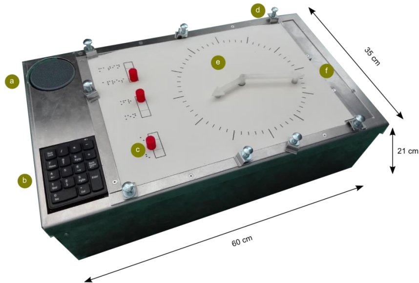
Figure 4.1. Overview of the Tangible Box. a) speaker; b) keyboard; c) a tangible object, composed of two parts (one above the surface, in red, and one below the surface); d) one element of the fastening system that holds the supports in place; e) support used for the activity (here, a raised-line clock); f) dedicated area where unused tangible objects can be placed.
