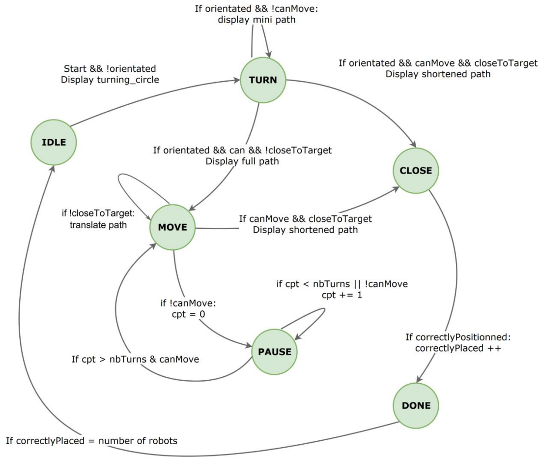
Figure C. 3. State-machine summarizing how the application handles the robots.
