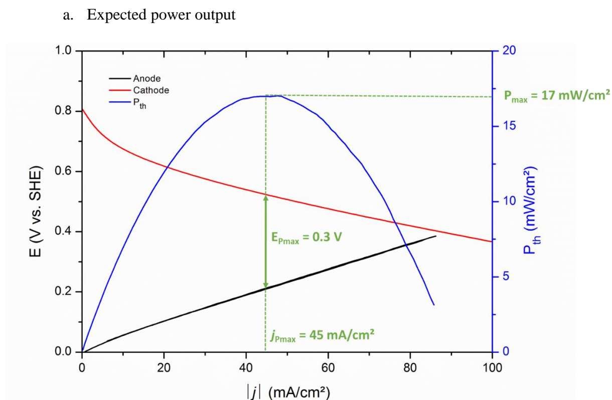
Figure 4. Polarization curves of a CyArg anode (black) and CoNC cathode (red), and extrapolated power output of an ideal fuel cell. Conditions for anode (MWNT-COOH/CyArg): S = 0.063 \text{ cm}^2 , electrolyte is \text{H}_2\text{SO}_4 0.5 M in \text{H}_2\text{O} , pH 0.3, 298K and P_{\text{H}_2} = 1 \text{ atm} . Conditions for cathode: S = 0.063 \text{ cm}^2 , electrolyte is \text{H}_2\text{SO}_4 0.5 M in \text{H}_2\text{O} , pH 0.3, 298K and P_{\text{O}_2} = 1 \text{ atm} .
