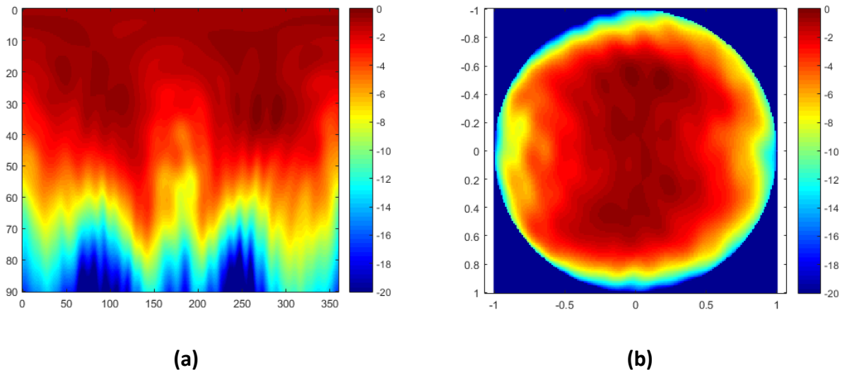
Fig. 2. 17 Element pattern from FEKO simulation of a one ring array of connected spirals (see Fig. 2. 13 for an array with 4 rings) with 14 elements per polarization and a radius of 16.95 cm with one of the spirals on while matching the other spirals to 220 ohm resistances. The element pattern is shown at 5GHz ((a) theta phi space and (b) uv space).
