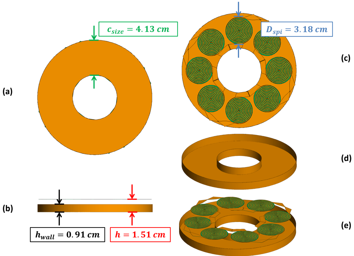
Fig. 2. 12 FEKO model of the cavity behind the ring array of connected spirals: top view (a) and isometric view (d). FEKO model of a ring array of connecting spirals: side view (b), top view (c) and isometric view (e). Spiral diameter ( D_{spi} ) highlighted in blue, cavity size ( c_{size} ) in green, height of the wall of the cavity ( h_{wall} ) in black and distance between the spirals and the bottom of the cavity ( h ) in red.
