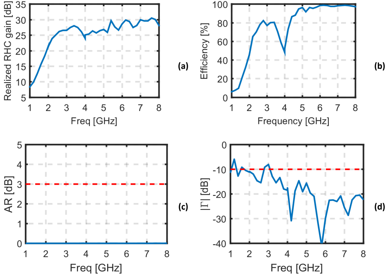
Fig. 2. 7 FEKO simulation of the concentric ring array of Fig. 2. 6 from (Hinojosa et al., 2014) with added connections between spirals at broadside ((a) Gain, (b) Efficiency, (c) AR and (d) |\Gamma| typical case). The dashed red lines indicate the limit from the specifications.
