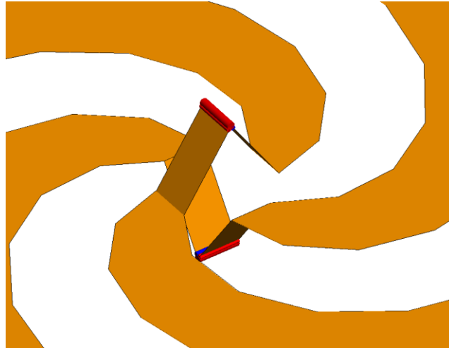
Fig. 3. 13 Feed of the simulated self-complementary 4-arms connecting spirals in FEKO.
