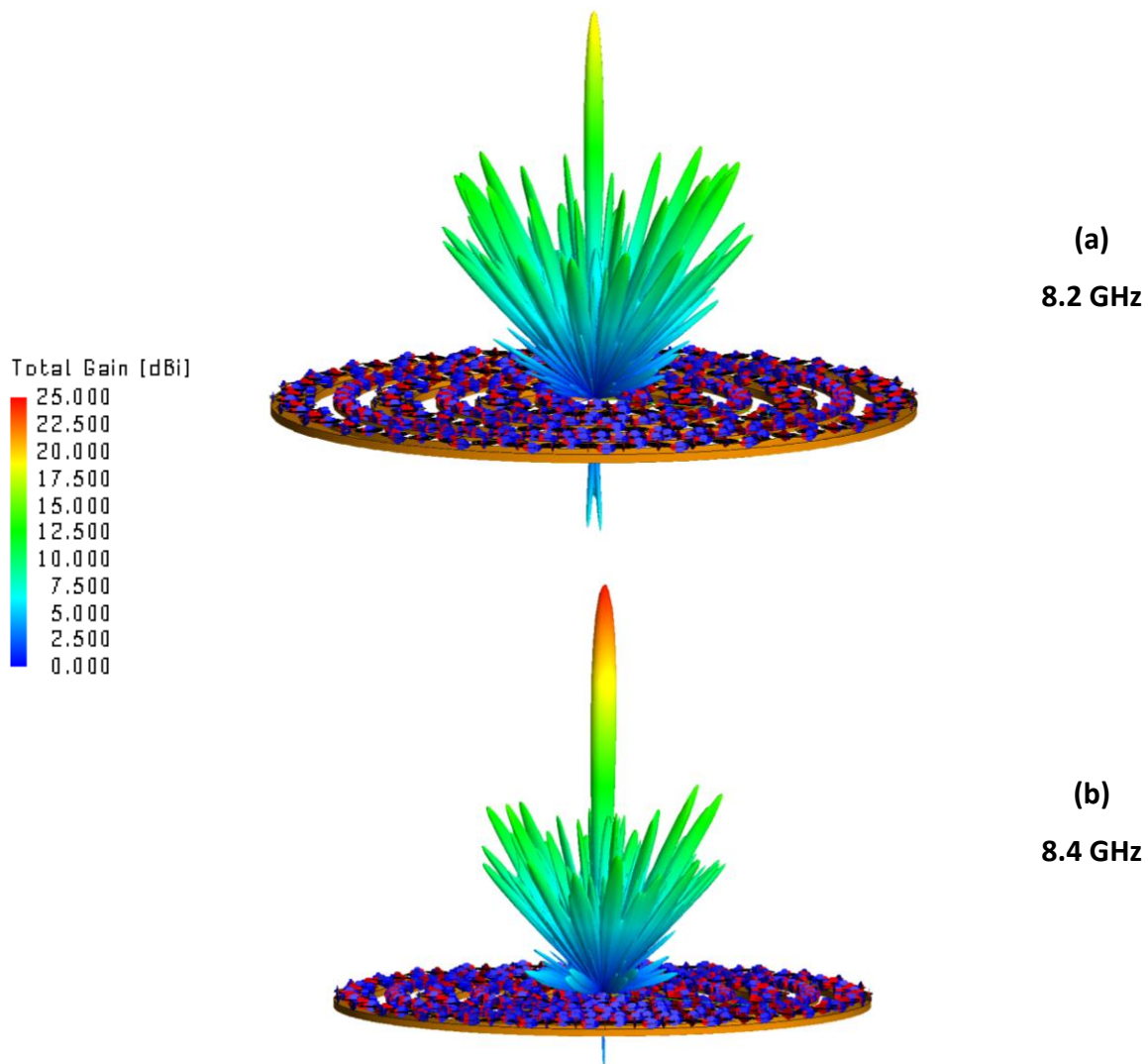
Fig. 2. 49 Radiating Pattern from the FEKO simulation of the optimized Concentric Ring Array of connecting Spirals with interleaved WAVES of Fig. 2. 44 with all elements turned on at broadside. In (a) we have the Radiating Pattern at 8.2 GHz and in (b) at 8.4 GHz.
