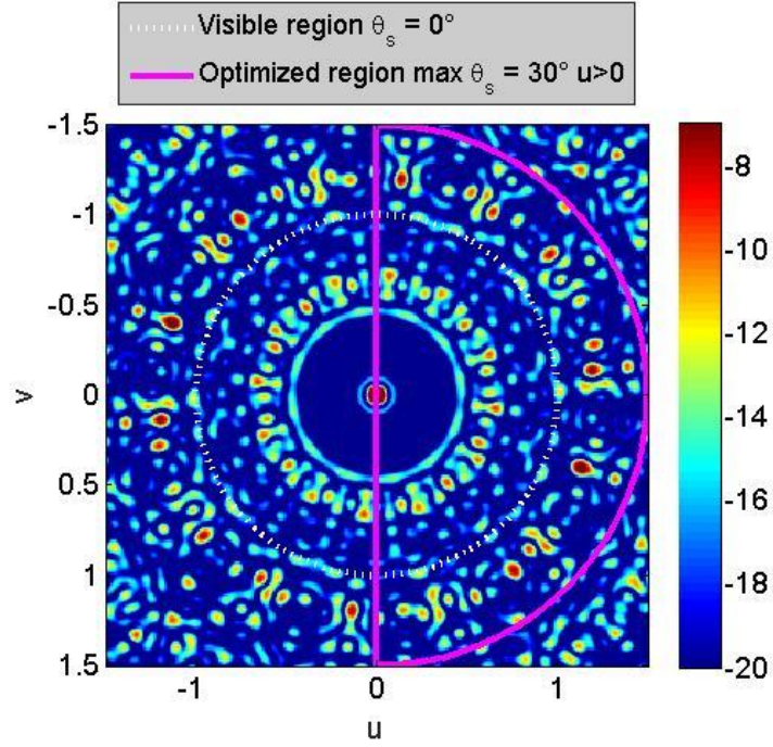
Fig. 2. 15 Array factor of the example array at 6.9 GHz. The visible region is inside the highlighted white dotted line. The zone in which we search the highest sidelobe to use in the cost function for our optimization of the concentric ring array is inside the highlighted purple line.
