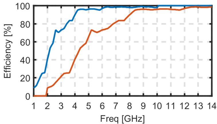
Fig. 2. 45 Efficiency model for the spiral antennas in the Concentric Ring Array with scaled WAVES of Fig. 2. 44. The blue curve is the efficiency of the normal sized spirals, obtained from Fig. 2. 30. The red curve is the efficiency of the smaller spiral antennas, obtained from scaling the results from the larger elements.
