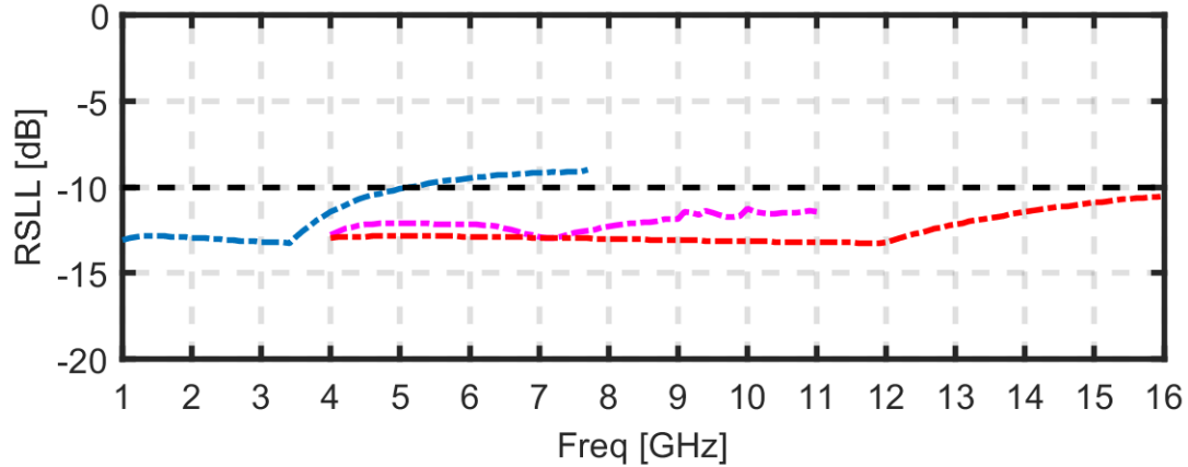
Fig. 2.43 RSLL obtained using equation (2.13) for the Concentric Ring Array with scaled WAVES weighting the 1 st lobe in the optimization (Table 2.14). The blue curve is the RSLL for the larger elements alone. The purple curve is the RSLL for both the smaller and the larger elements turned on together. The red curve is the RSLL when we have only the smaller elements turned on. The dashed black line is the limit from the specifications.
