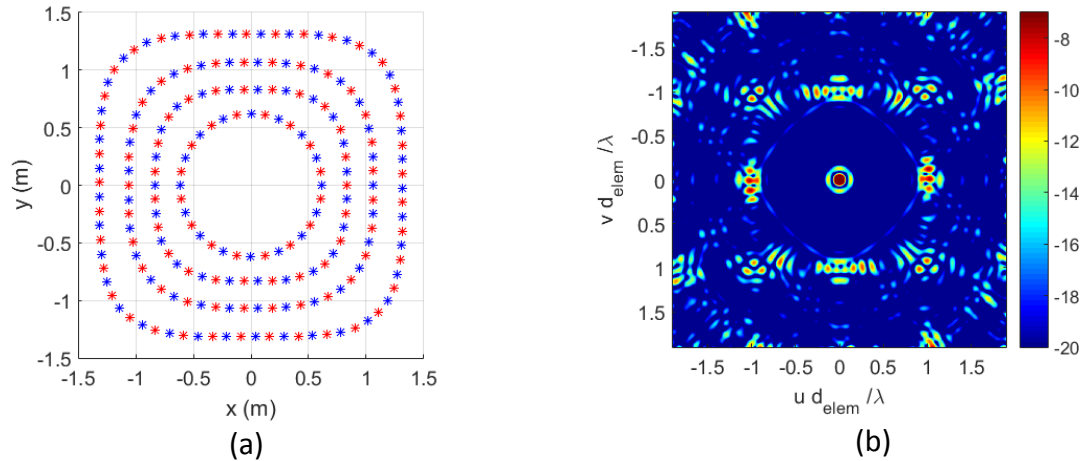
Fig. 1 Concentric superellipse ring array example. In (a) we have the elements positioning with the RHC polarized elements in blue and the LHC polarized elements in red. The first ring have a superellipse with degree 2 (a circle), both the intermediate ring have a degree of 3 and the largest ring has a degree of 4, thus being the one closer to a square. In (b) we have the array factor of the array with the axis normalized by d_{elem}/\lambda , with d_{elem} = 24.34 cm being the distance between two elements of the same polarization in a ring.
