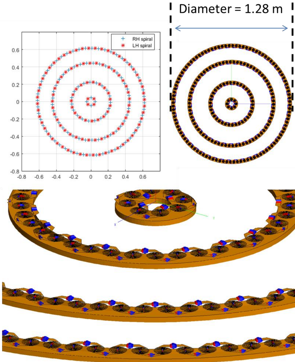
Fig. 2. 6 Element locations, Top view of the FEKO model and isometric view of the FEKO model for the concentric ring array from (Hinostroza et al., 2014) with added connections between spirals.
