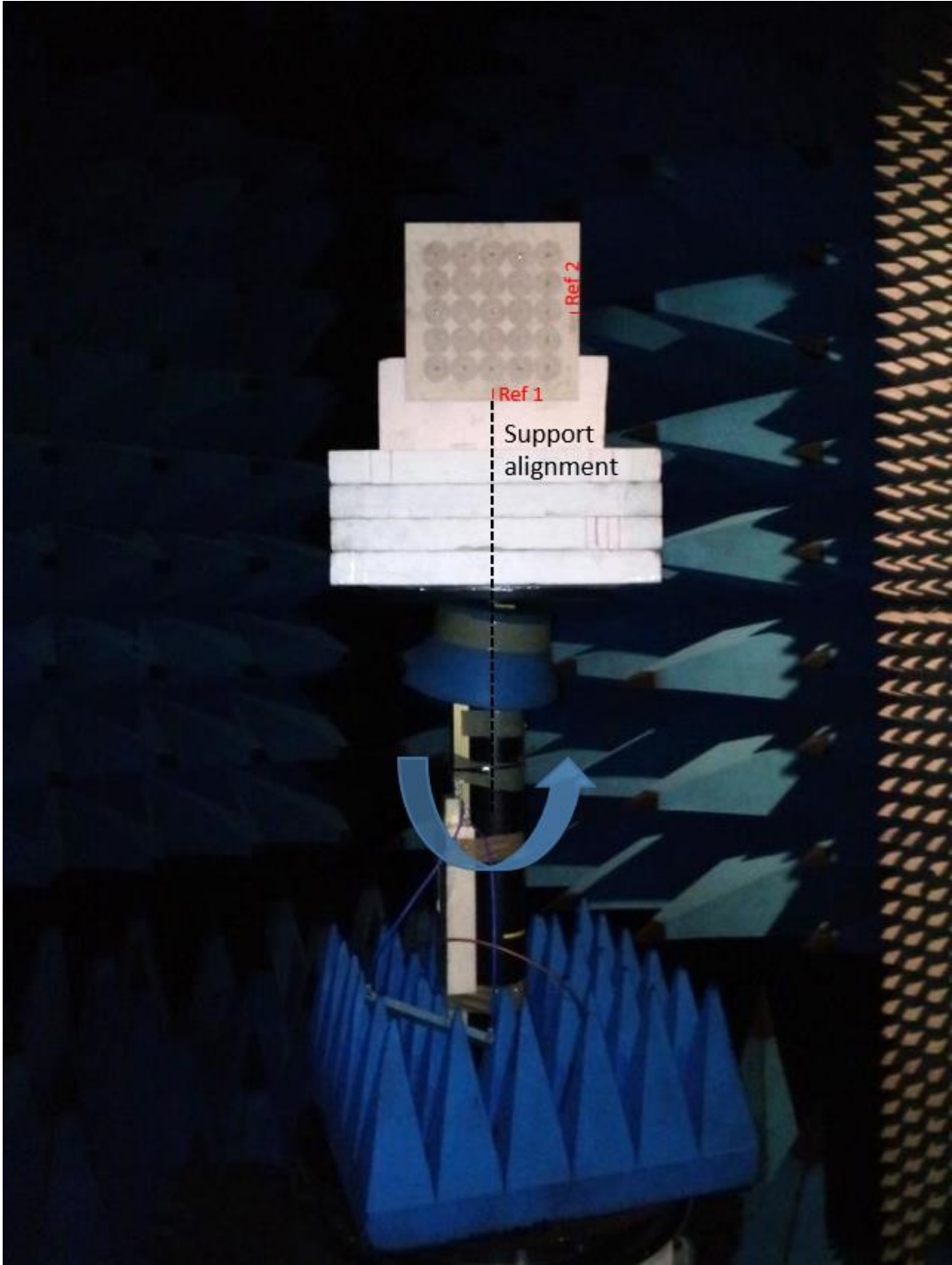
Fig. 3. 23 Antenna array Under Test on anechoic chamber.
