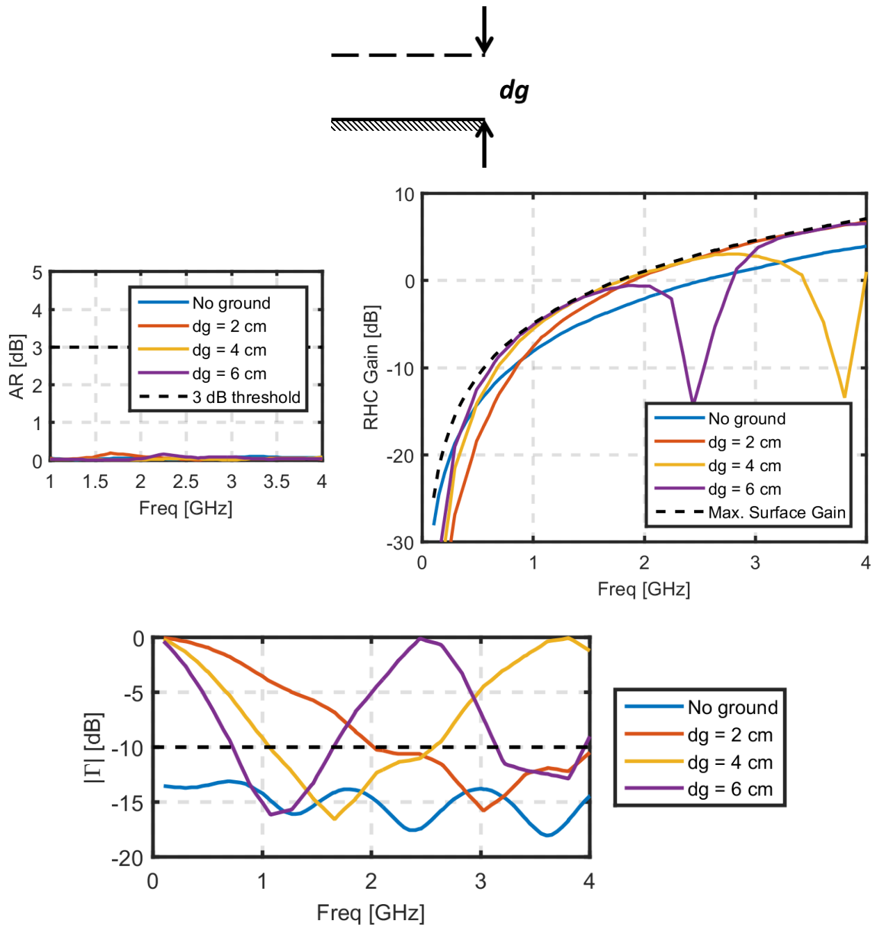
Fig. 3. 12 Axial Ratio, RHC Gain and Reflection coefficient obtained from infinite array simulations of a 4 arm connecting spiral array using FEKO. In blue there is no ground plane, in red there is a ground plane 2 cm away from the spirals, in yellow 4 cm away and in purple 6 cm away.
