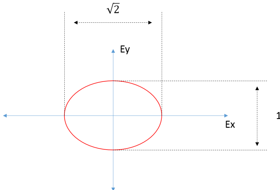
Fig. 1. 1 Polarization ellipse of an electric field with an Axial Ratio of 3 dB, which corresponds to a Cross Polarization Ratio of 15 dB
