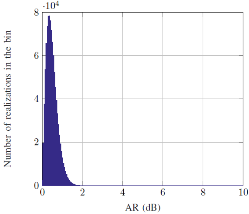
Fig. A. 2 Histogram of the Monte Carlo simulations of the AR calculations without approximations for 25 crossed dipoles elements looking at broadside. The bins in the histogram have a 0.05 dB width.
