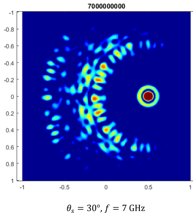
Fig. 2. 22 Radiating pattern of the optimized array from Table 2. 7, steered to 30^\circ , at 7GHz,calculated using the equations (2.10) and (2.12).
