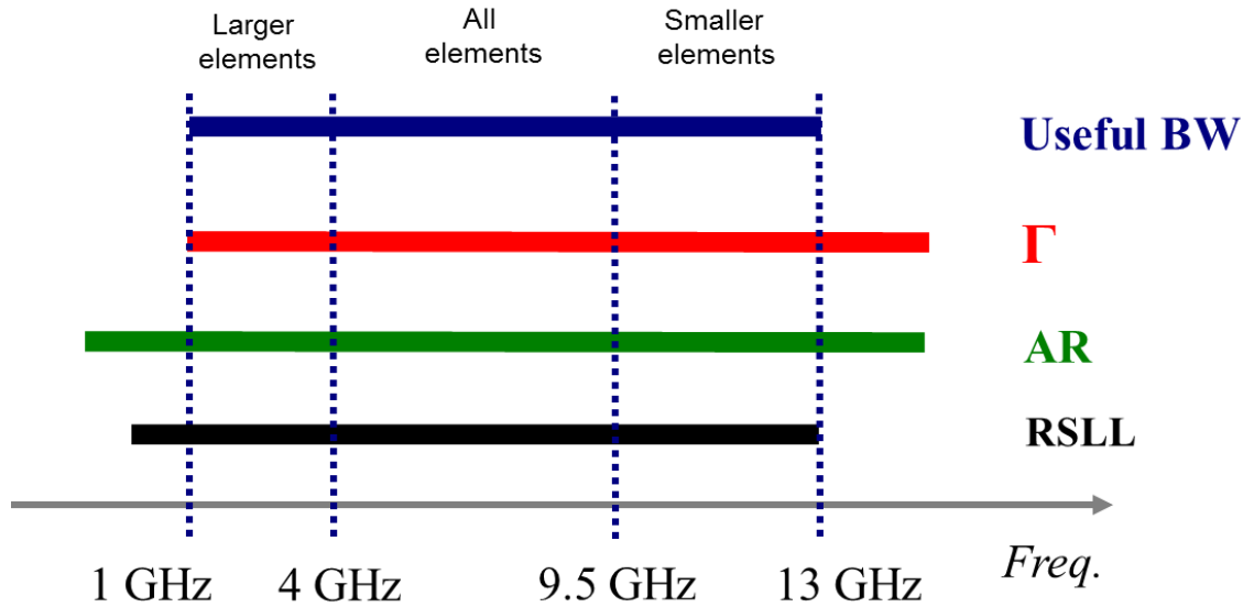
Fig. 2. 41 Frequency range of acceptable performance. The bars correspond to the bandwidth definitions listed. In red we have the bar corresponding to the reflection coefficient, in green the axial ratio and in black the relative sidelobe level. The overall useful bandwidth is the intersection of these three bandwidths.
