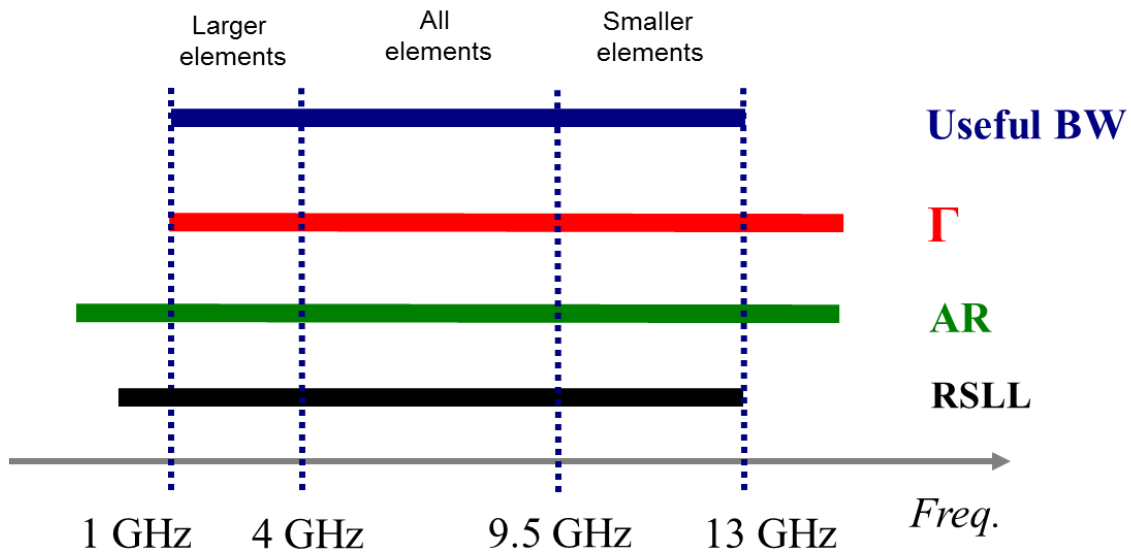
Fig. 2. 54 The bars correspond to the bandwidth definitions listed. In red we have the bar corresponding to the reflection coefficient, in green the axial ratio and in black the relative sidelobe level. The overall useful bandwidth is the intersection of these three bandwidths.
