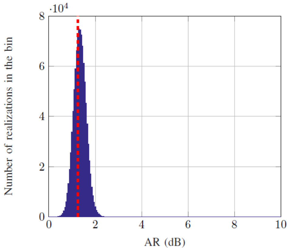
Fig. A. 4 Histogram of the Monte Carlo simulations of the AR calculations without approximations for 25 crossed dipoles elements scanned to 30°. In dashed red we have the AR without errors (1.25 dB). The bins in the histogram have a 0.05 dB width.
