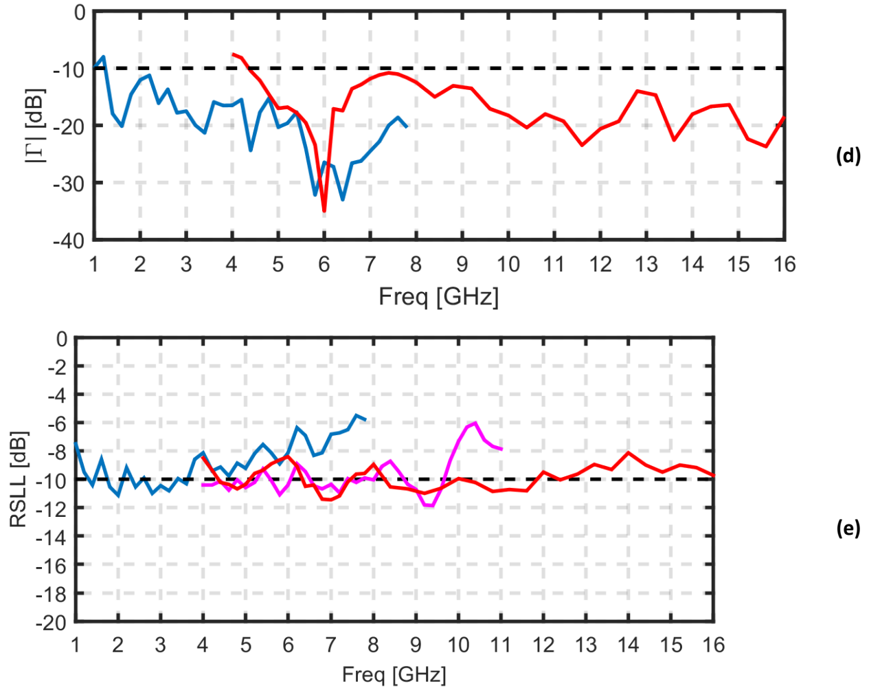
Fig. 2. 40 FEKO simulation of the optimized Concentric Ring Array of connecting Spirals with scaled WAVES of Fig. 2. 34 steering to [\theta_s, \varphi_s] = [30^\circ, 0^\circ] . In blue we have the larger elements alone. In purple we have both the smaller and the larger elements turned on together. In red we have only the smaller elements turned on. The dashed black lines indicate the limits from the specifications.
