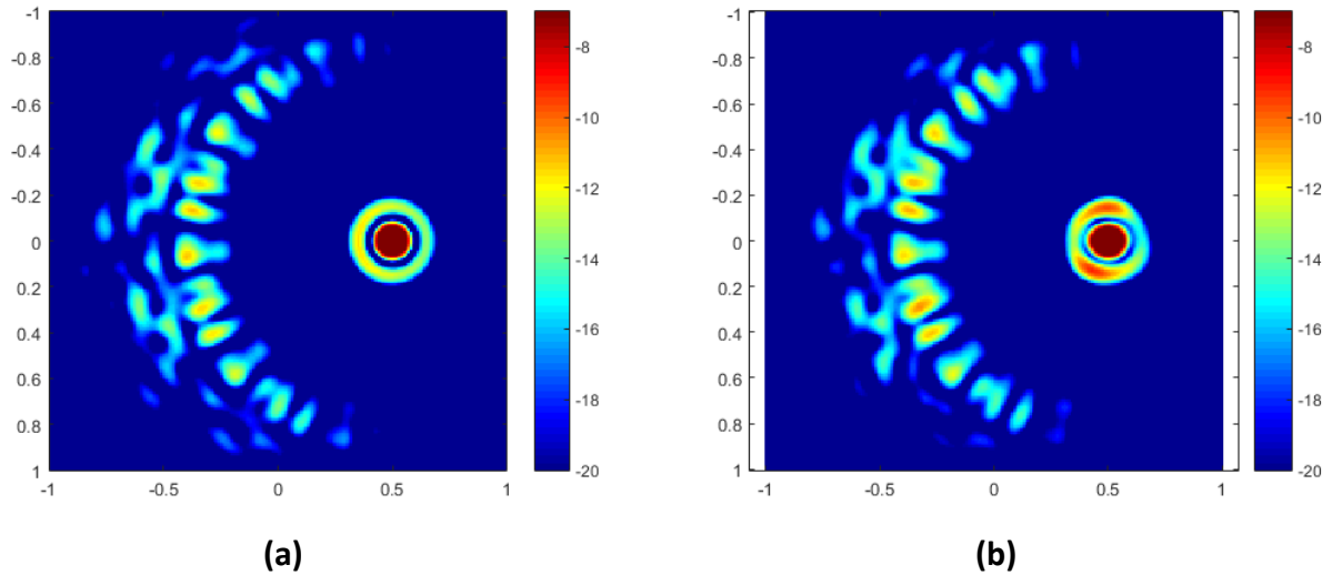
Fig. 2. 26 Electric field radiated from the concentric ring array from Table 2. 9 at 5 GHz, steered to 30^\circ , in the u v space. In (a) we have the electric field obtained with equations (2.10) and (2.12) and in (b) the electric field obtained from a FEKO simulation.
