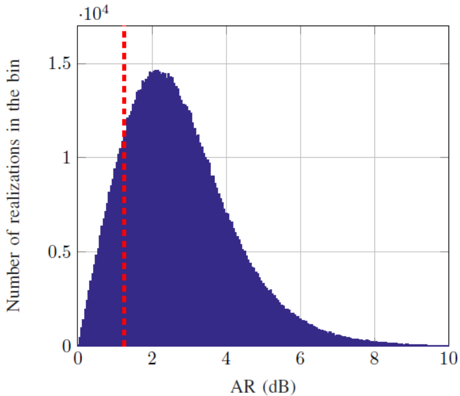
Fig. A. 3 Histogram of the Monte Carlo simulations of the AR calculations without approximations for a single crossed dipoles element at 30°. In dashed red we have the AR without errors (1.25 dB). The bins in the histogram have a 0.05 dB width.
