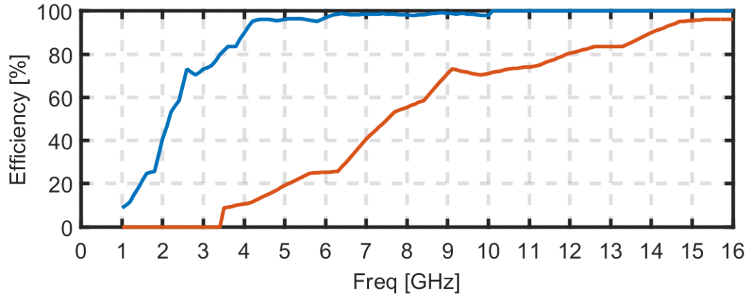
Fig. 2.37 Efficiency model for the spiral antennas in the Concentric Ring Array with scaled WAVES (see Fig. 2.34). The blue curve is the efficiency of the normal sized spirals, obtained from Fig. 2.30. The red curve is the efficiency of the smaller spiral antennas, obtained from scaling the results from the larger elements.
