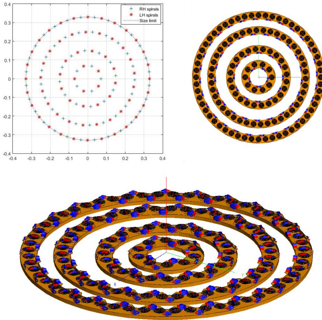
Fig. 2. 13 Elements locations of the example array (top left), Top view of the FEKO model (top right) and isometric view of the FEKO model for the example array (bottom).
