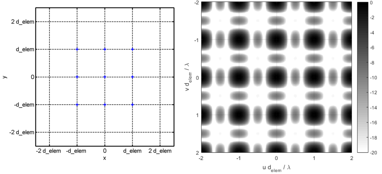
Fig. 1. 5 Elements positions of a 3x3 uniform array with a spacing of d_{elem} (left) and the corresponding AF with the axis normalized by d_{elem}/\lambda (right). The positions in the array factor where both u d_{elem}/\lambda and v d_{elem}/\lambda are integer are grating lobes.
