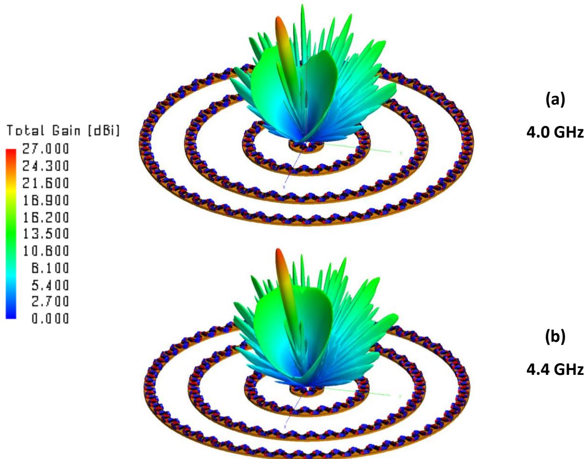
Fig. 2. 10 Radiating Pattern from the FEKO simulation of the concentric ring array of Fig. 2. 6 from (Hinojosa et al., 2014) with added connections between spirals steered to 30°. In (a) we have the Radiating Pattern at 4 GHz and in (b) at 4.4 GHz.
