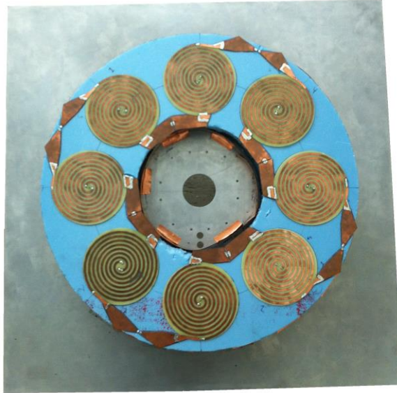
Fig. 1. 17 Ring array of connecting spirals with cavity (Hinostroza et al., 2016).
