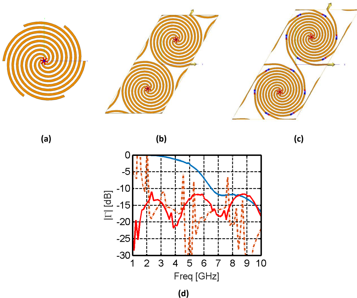
Fig. 3. Reflection coefficient from FEKO simulation of a 6-arms connecting spirals infinite array with (geometry in (c), dashed red curve) and without (geometry in (b), red curve) small resistances in the arms to break resonances and of a single 6 arms spiral (geometry in (a), blue curve) using FEKO. The spirals have a radius equal to 1 cm and the spacing between neighboring spirals in the arrays is 2 cm for that without resistances and 2.5 cm for the one with resistances.
