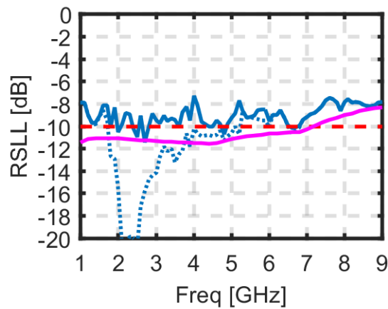
Fig. 2. 25 RSL vs freq. for the compact concentric ring array 2 nd optimization. The purple curve is the RSL calculated using a \cos^q approximation for the element pattern. The blue curve is the RSL obtained from a FEKO simulation of the array. The dotted blue curve is the RSL from the same FEKO simulation but disregarding the sidelobe closest to the main beam (Fig. 2. 26) The dashed red line is the limit from the specifications.
