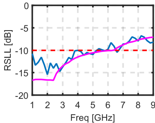
Fig. 2. 28 RSSL vs freq. for the compact concentric ring array 3 rd optimization. The purple curve is the RSSL calculated using a \cos^9 approximation for the element pattern. The blue curve is the RSSL obtained from a FEKO simulation of the array. The dashed red line is the limit from the specifications.
