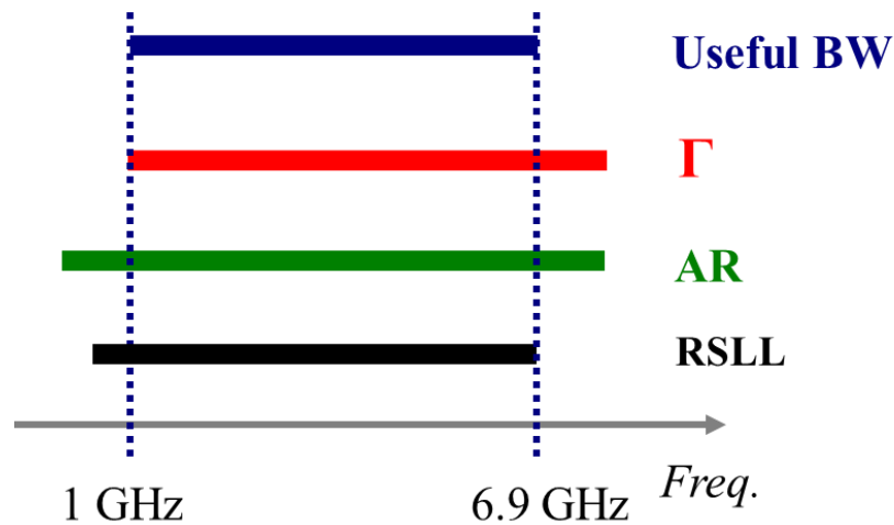
Fig. 2. 31 The bars correspond to the bandwidth definitions listed. In red we have the bar corresponding to the reflection coefficient, in green the axial ratio and in black the relative sidelobe level. The overall useful bandwidth is the intersection of these three bandwidths.
