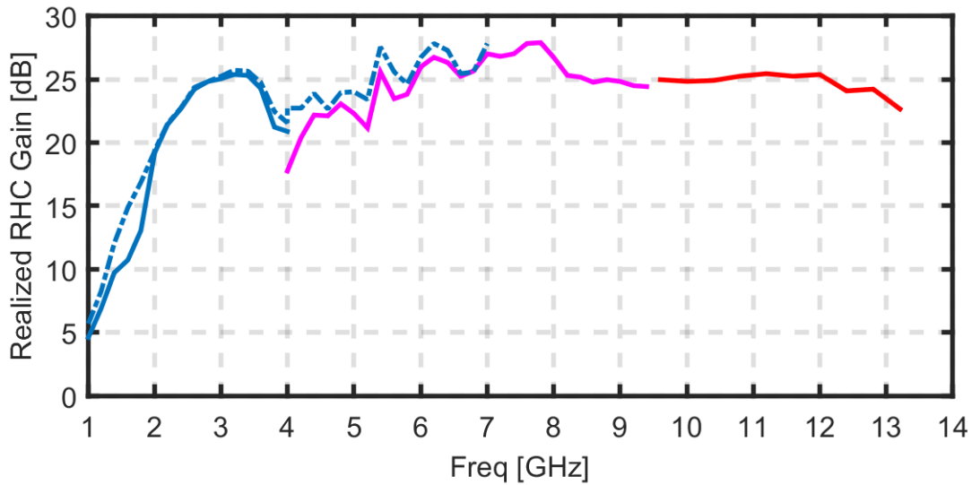
Fig. 2. 51 Realized RHC gain curves when pointing at broadside from the Concentric Ring Array of Table 2. 10 from section 2.3.3 (blue dashed line) and from the Concentric Ring Array with scaled WAVES of Fig. 2. 34 from section 2.4.1 with only the larger elements turned on (blue), both the larger and the smaller on at the same time (purple) and only the smaller elements on (red).
