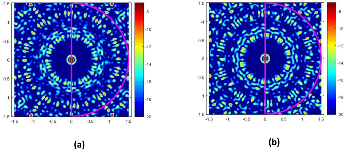
Fig. 2. 16 Array factor of the optimized compact concentric ring array at 6.9 GHz, in (a) from the RH polarized elements and in (b) from the LH polarized ones. In purple we highlight the zone in which we searched for the highest sidelobe for our optimization.
