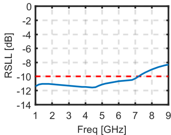
Fig. 2. 24 RSLL vs freq. for the compact concentric ring array 2 nd optimization using a \cos^q approximation for the element pattern. The dotted red line is the limit from the specifications.
