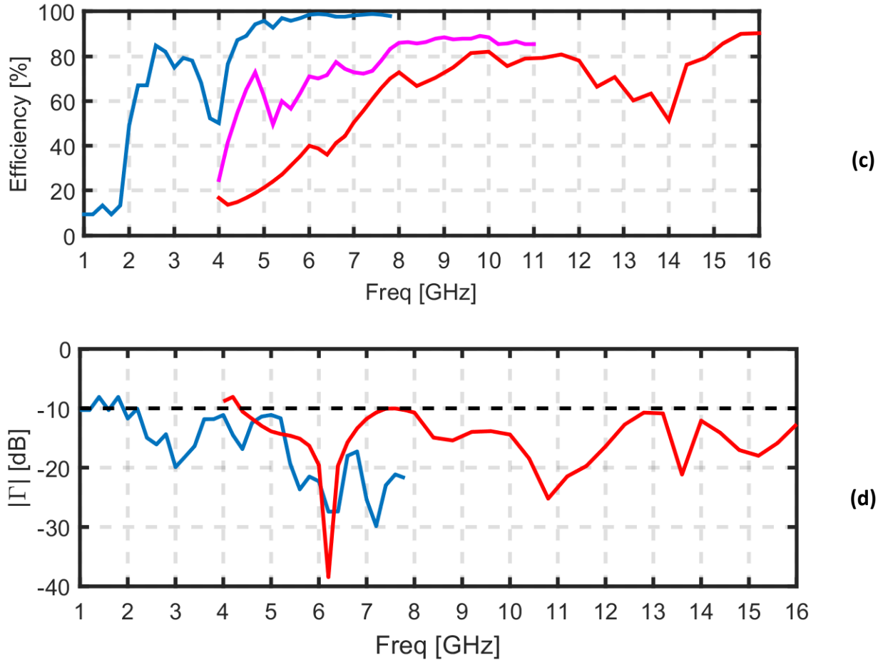
Fig. 2. 39 FEKO simulation of the optimized Concentric Ring Array of connecting Spirals with scaled WAVES of Fig. 2. 34 at broadside. In blue we have the larger elements alone. In purple we have both the smaller and the larger elements turned on together. In red we have only the smaller elements turned on. The dashed black lines indicate the limits from the specifications.
