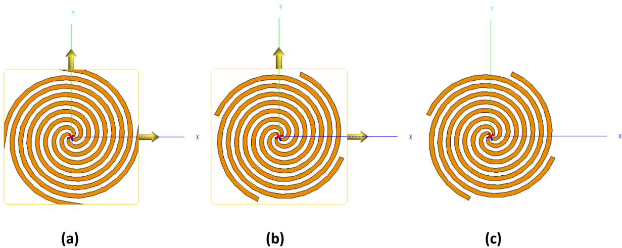
Fig. 3. 4 FEKO models of, from the left to the right, 4-arms connecting spirals infinite array (a), 4 arms disconnected spirals infinite array (b) and single 4 arms spiral (c). The spirals have a radius equal to 2.4 cm.
