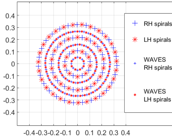
Fig. 2. 44 Elements position for the optimized concentric ring array with interleaved WAVES.
