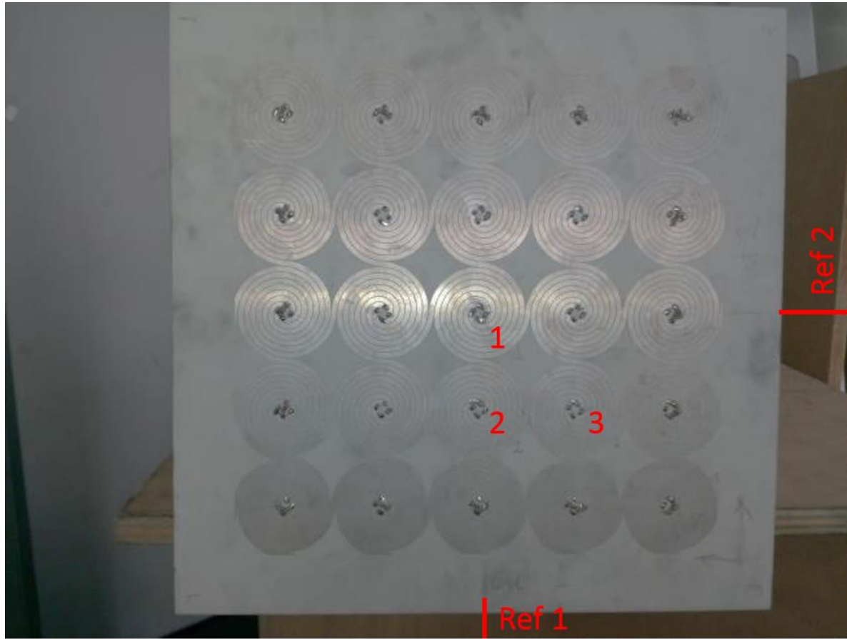
Fig. 3. 22 Antenna array Under Test. The marks Ref 1 and Ref 2 indicate that during the measurement (always the AUT is the one rotating, see Fig. 3. 24) the said Ref X is aligned to the base center marked in the support (Fig. 3. 23).
