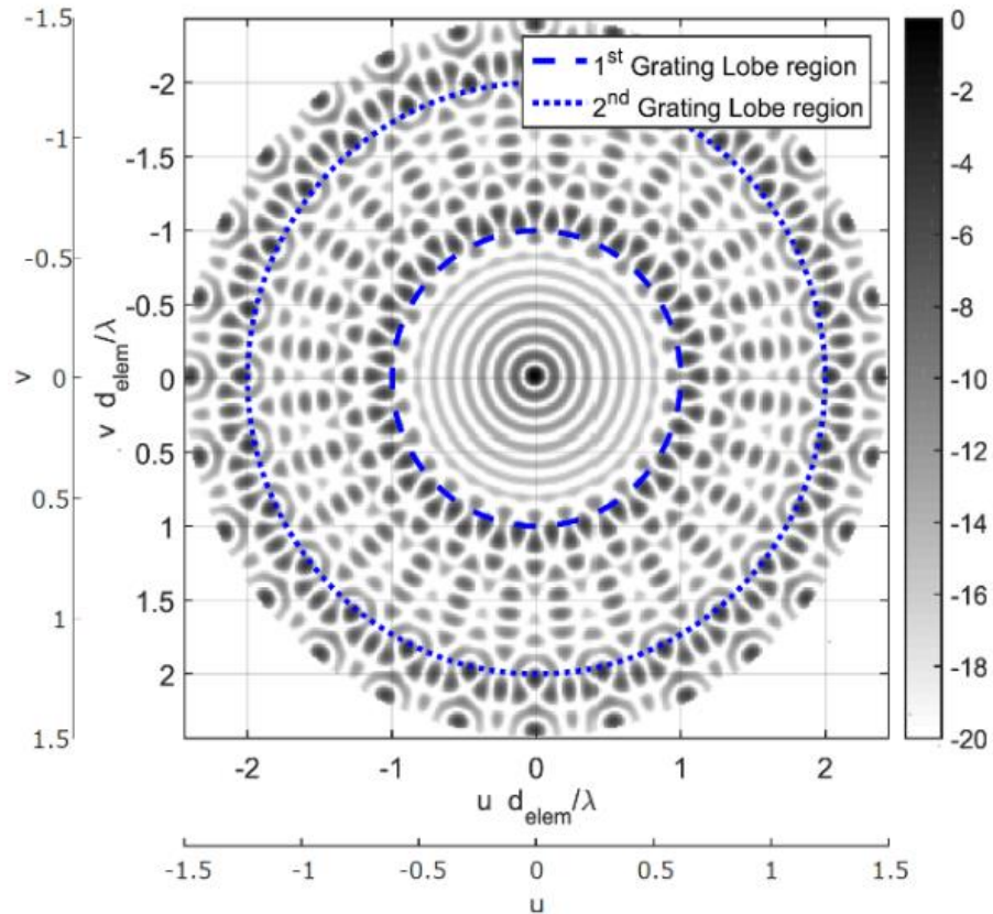
Fig. 1. 6 Array Factor of a one ring array with a radius of 1.085 m and 28 elements uniformly spaced, showing all sidelobes that appear in the visible zone at 2 GHz for a maximal steering of \theta_s = 30^\circ . The u - v axes are shown for the AF at 2 GHz, as well as the axis normalized by d_{elem}/\lambda . The 1 st (dashed) and 2 nd (dotted) Grating Lobe (GL) regions are highlighted in the Array Factor.
