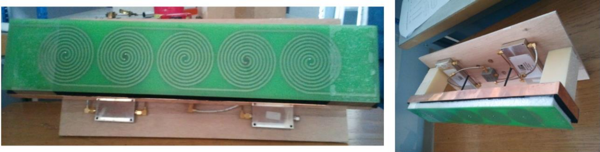
Fig. 1. 16 Linear array of connecting spirals with cavity (Guinvarc'h et al., 2012).
