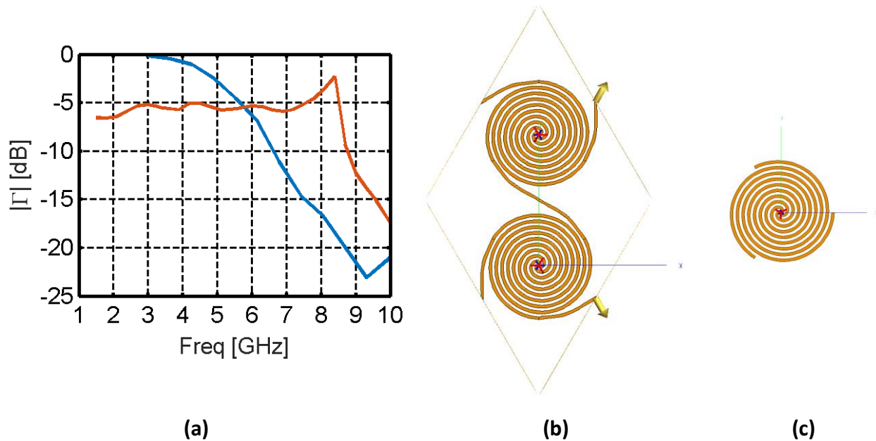
Fig. 3. 1 Reflection coefficient from FEKO simulation of a 3-arms connecting spirals infinite array (geometry in (b), red curve) and of a single 3 arms spiral (geometry in (c), blue curve) using FEKO. The spirals have radius equal to 1 cm and the spacing between neighboring spirals in the array is 2.33 cm.
