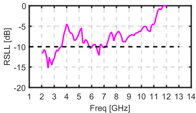
Fig. 2. 47 FEKO simulation of the optimized Concentric Ring Array of connecting Spirals with interleaved WAVES of Fig. 2. 44 with all elements turned on at broadside (in (a) the realized RHC gain and in (b) the RSLL) and steering to 30° (in (c) the realized RHC gain and in (d) the RSLL). The dashed black lines indicate the limits from the specifications.
