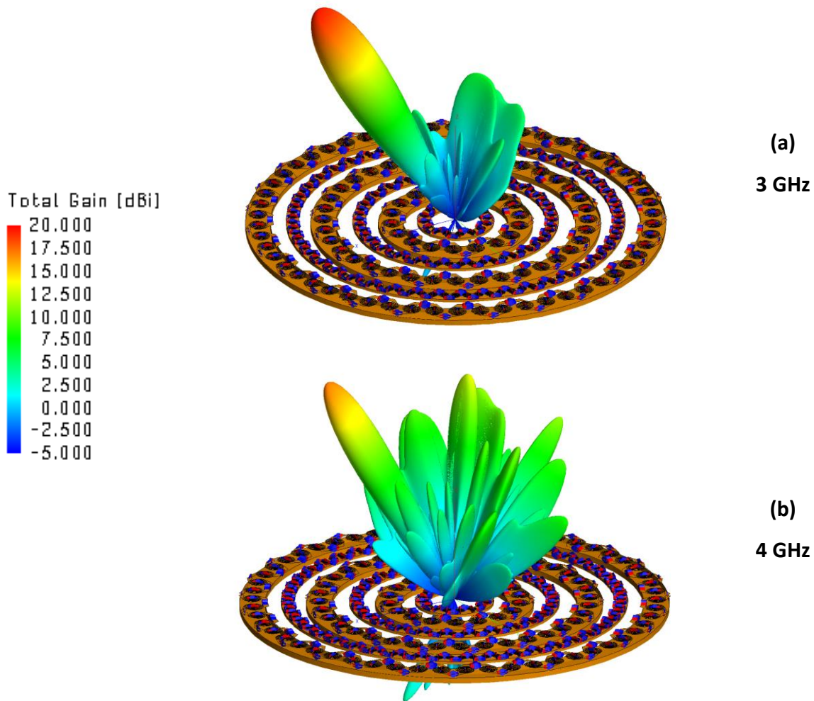
Fig. 2. 50 Radiating Pattern from the FEKO simulation of the optimized Concentric Ring Array of connecting Spirals with interleaved WAVES of Fig. 2. 44 with all elements turned on steered to 30°. In (a) we have the Radiating Pattern at 3 GHz and in (b) at 4 GHz.
