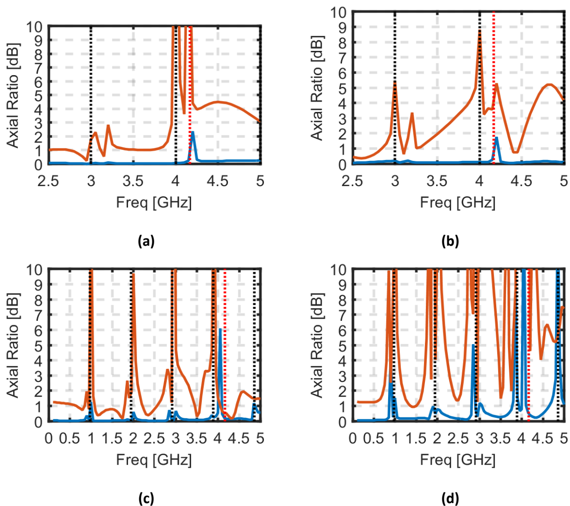
Fig. 3. 9 Axial Ratio of the 4 arm disconnected spirals infinite array in (a) and (b) and of the 4-arm connecting spirals infinite array in (c) and (d). In blue the array is steering to 5 degrees and in red to 30 degrees. In (a) and (c) we show the main polarization (mode 1) and in (b) and (d) we show the opposite polarization (mode -1). The black dotted vertical lines show the periodic spiral resonances and the red dotted vertical lines show the frequency in which the grating lobes appear when steering to 30^\circ .
