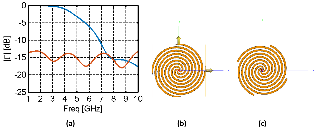
Fig. 3. 2 Reflection coefficient from FEKO simulation of a 4-arms connecting spirals infinite array (geometry in (b), red curve) and of a single 4 arms spiral (geometry in (c), blue curve) using FEKO. The spirals have a radius equal to 1 cm and the spacing between neighboring spirals in the array is 2 cm.
