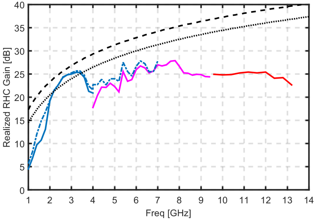
Fig. 2. 55 Realized RHC gain curves when pointing at broadside from the Concentric Ring Array from section 2.3.3 (blue dashed line) and from the Concentric Ring Array with scaled WAVES from section 2.4.1 with only the larger elements turned on (blue), both the larger and the smaller on at the same time (purple) and only the smaller elements on (red). Superposed we have the maximal surface gain corresponding to the 35 \text{ cm} circle in which the arrays are circumscribed, which has an area of 0.38 \text{ m}^2 , (black dashed line) and corresponding to the area occupied by the cavities of the CRA or the CRA with scaled WAVES, both which have 0.2 \text{ m}^2 (dotted black line).
