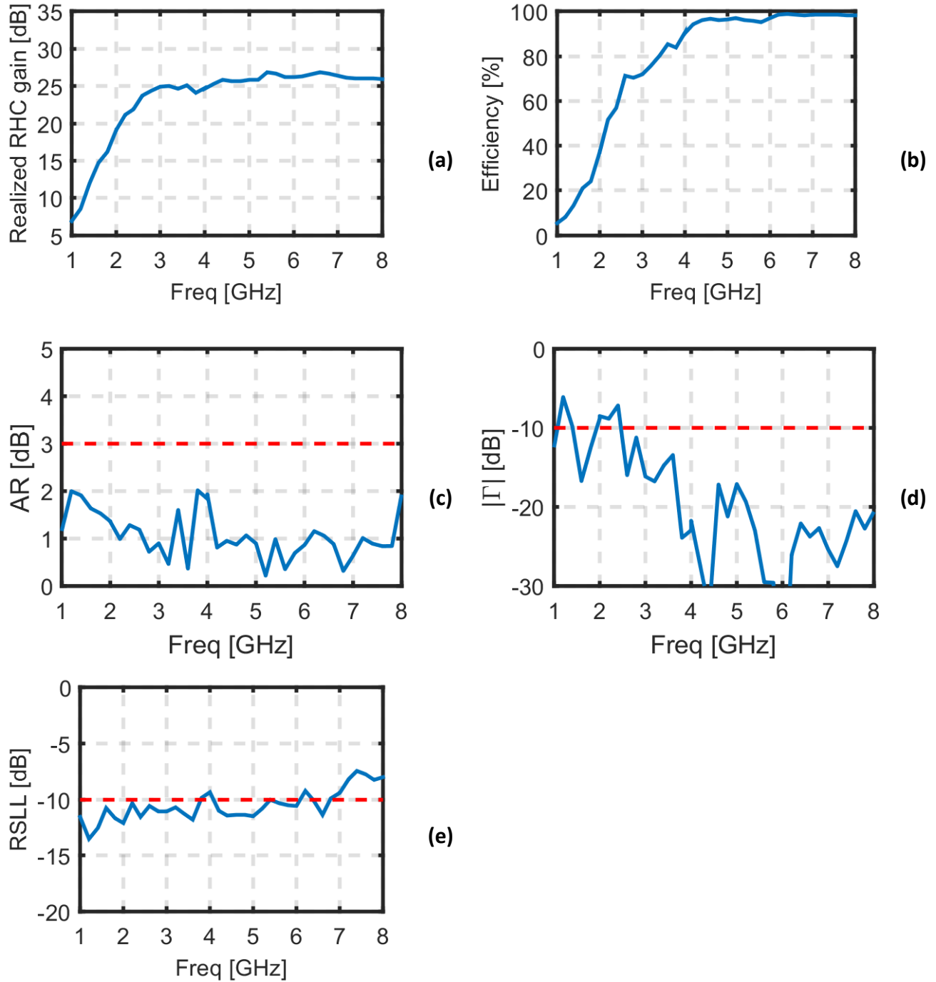
Fig. 2.9 FEKO simulation of the concentric ring array of Fig. 2.6 from (Hinostroza et al., 2014) with added connections between spirals steered to 30^\circ ((a) Gain, (b) Efficiency, (c) AR, (d) |\Gamma| typical case and (e) RSL). The dashed red lines indicate the limit from the specifications.
