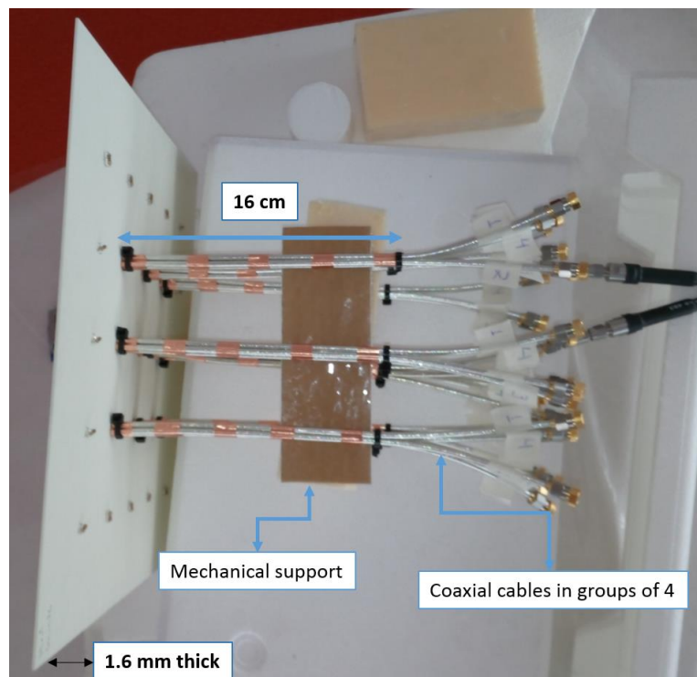
Fig. 3. 18 Photos of the prototype 4-arm connecting spirals array. In (a) we have the front view with the elements with soldered coaxial cables highlighted in blue and the dimensions indicated. In (b) we have the side view showing the soldered coaxial cables and the dimensions indicated as well.
