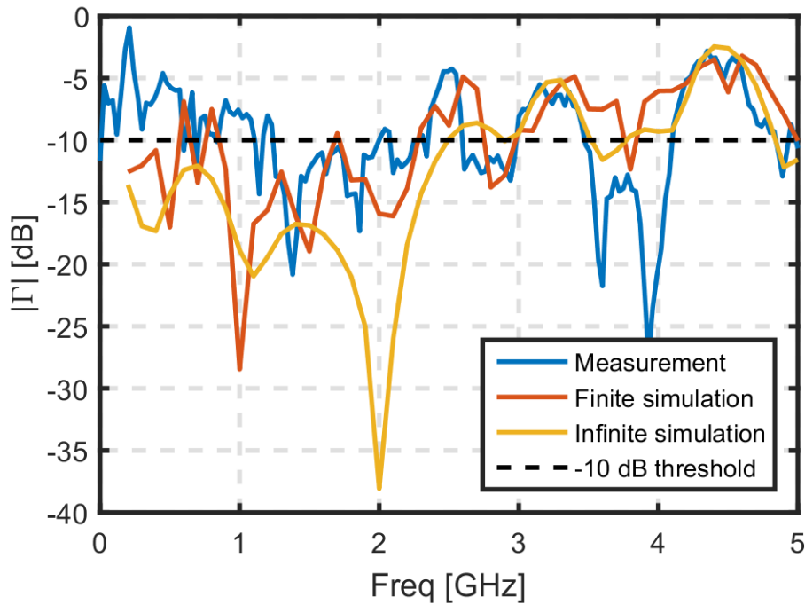
Fig. 3. 21 Reflection Coefficient from the prototype array (Fig. 3. 18), from the FEKO simulation of the 3x3 4-arm connecting non-complementary spirals array with one layer of elements with matching resistances of 100 \Omega (Fig. 3. 20) and from the FEKO simulation of the infinite 4-arm connecting non-complementary spirals array. In (a) we have the RH polarized array (mode 1) and in (b) we have the LH polarized array (mode -1).
