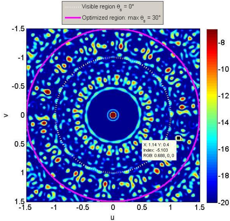
Fig. 2. 14 Array factor of the example array at 6.9 GHz. The visible region is highlighted in the white dotted line. The zone that corresponds to the union of the visible zones when steering up to \theta_s = 30^\circ and all \varphi_s is highlighted in purple.
