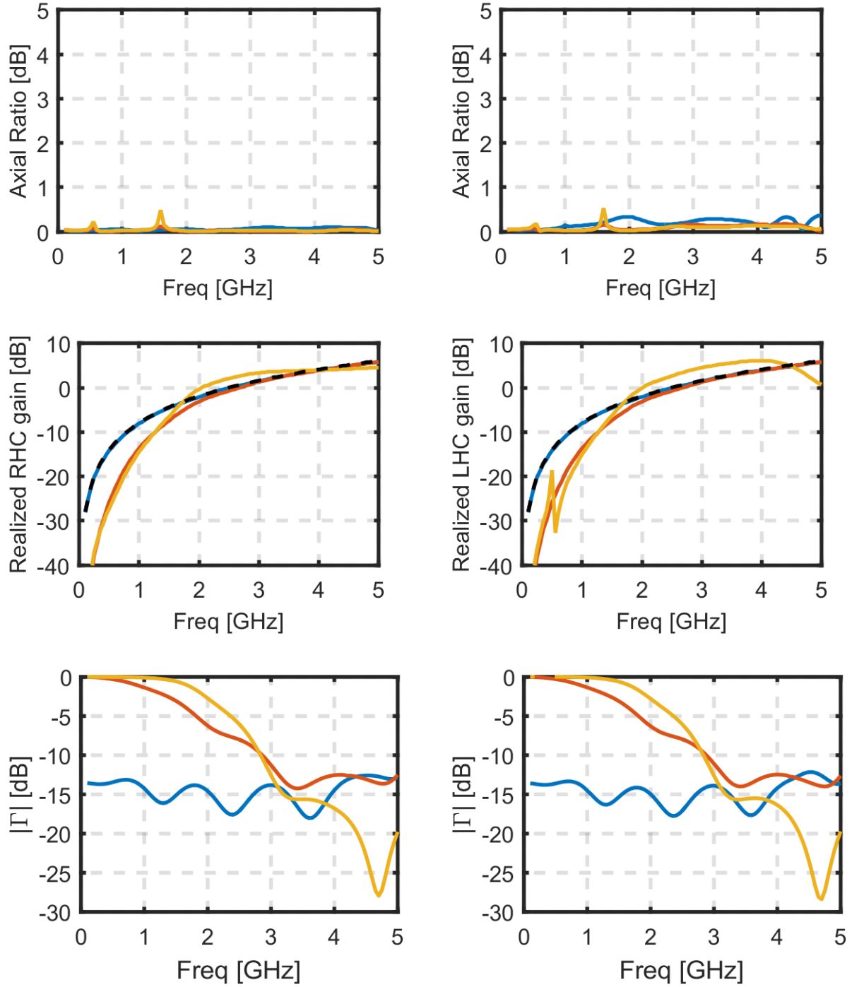
Fig. 3. 5 FEKO simulation of the 4-arms connecting spirals infinite array (blue), 4 arms disconnected spirals infinite array (red) and single 4 arms spiral (yellow). Main polarization (mode 1) on the curves to the left and secondary polarization (mode -1) on the curves to the right. In dashed black we have the maximal surface gain corresponding to the regions enclosed by the periodic boundaries, subtracting 3 dB as the antennas radiates to both sides.
