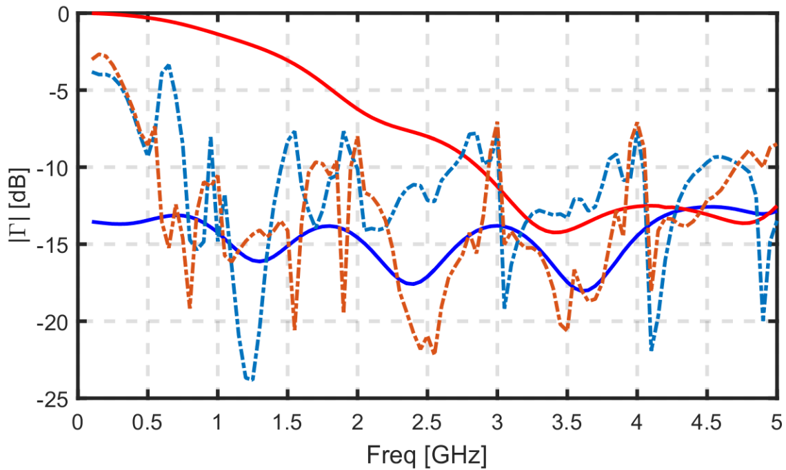
Fig. 3. 8 Reflection coefficient for the 3x3 (dash-dotted blue) and the 5x5 (dash-dotted red) 4-arms connecting spiral arrays, one layer of elements with matching resistances of 290 \Omega . The reflection coefficient was calculate using the S parameters of the arrays, which were obtained from S parameter simulations using FEKO. We also have the reflection coefficient of the 4-arms connecting spirals infinite array (solid blue) and 4 arm disconnected spirals infinite array (solid red) for comparison.
