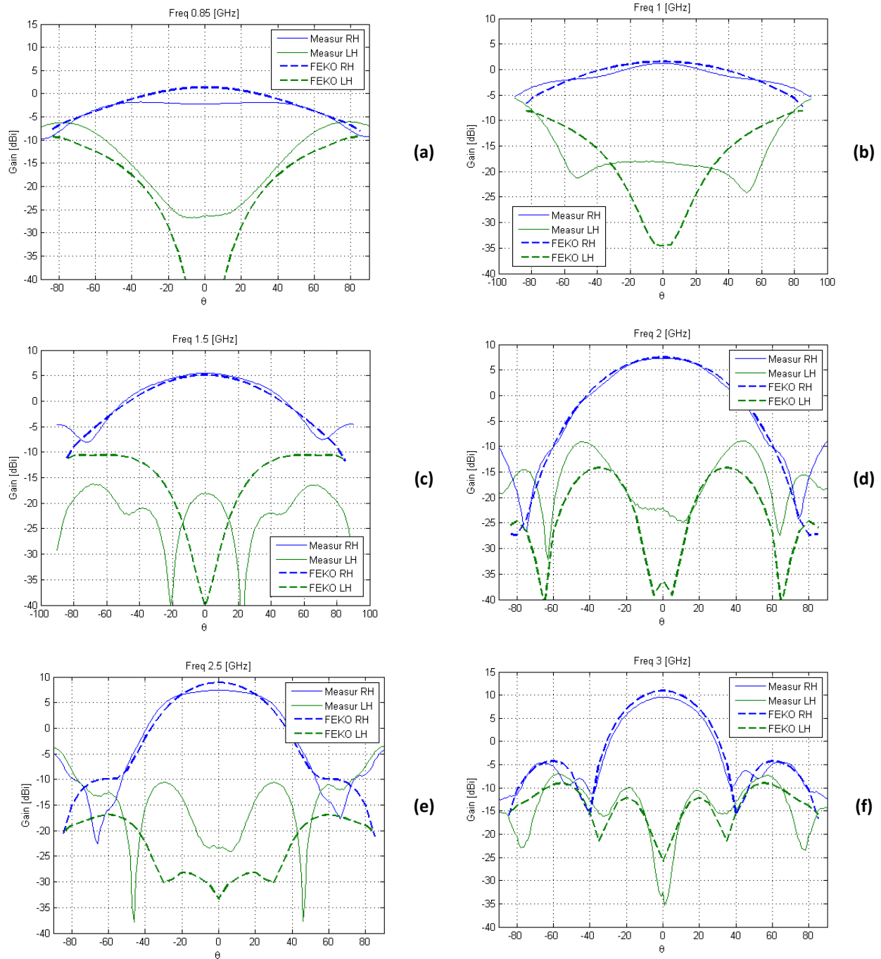
Fig. 3. 26 RH polarization (mode 1) electric field horizontal cuts from the prototype array (Fig. 3. 18) and from the FEKO simulation of the 3x3 4-arm connecting non-complementary spirals array with one layer of elements with matching resistances of 100 \Omega (Fig. 3. 20). In (a), (b), (c), (d), (e) and (f) we have, respectively, the fields at 0.85 GHz, 1 GHz, 1.5 GHz, 2 GHz, 2.5 GHz and 3 GHz.
