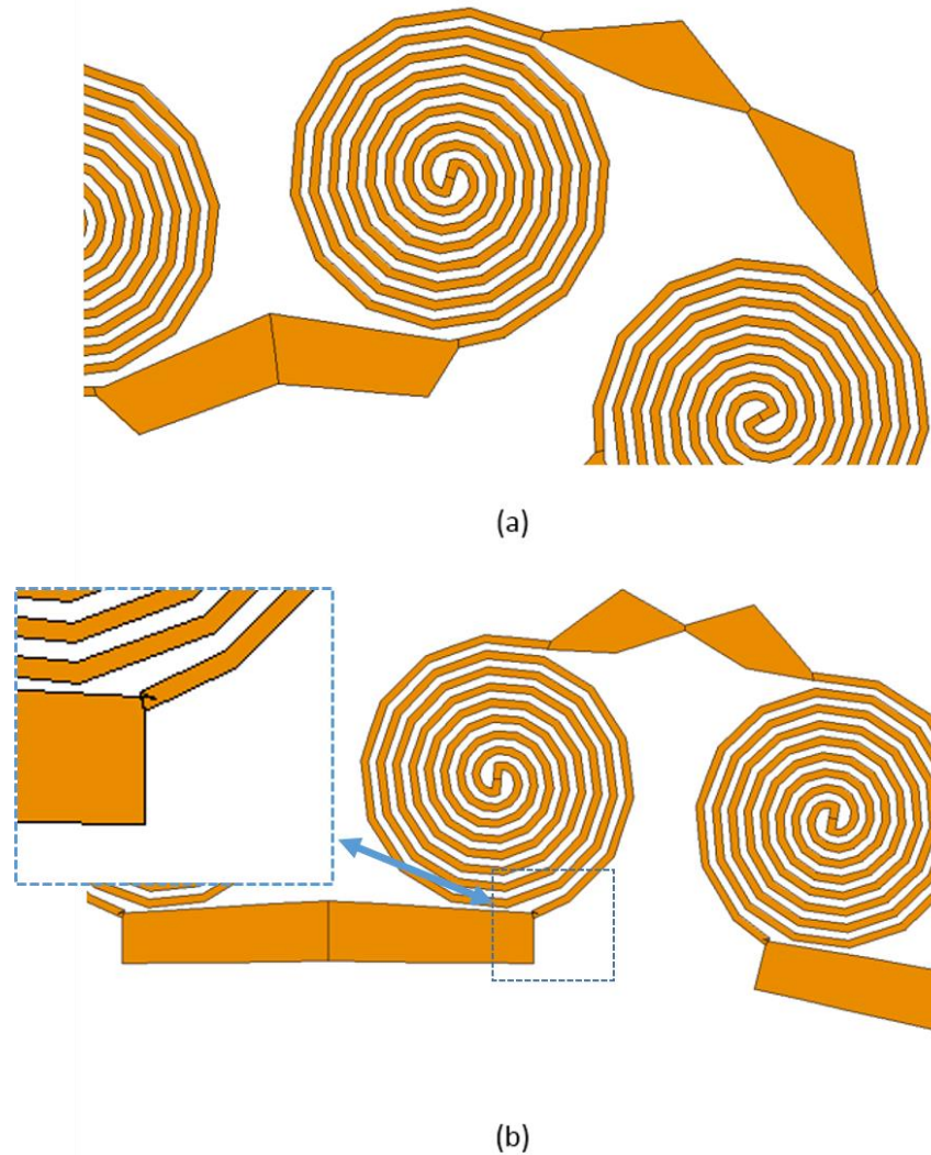
Fig. 2. 5 Connections between spirals in a ring array for an array with 4 spirals per polarization (a) and for an array with 27 elements per polarization (b). The parameters used for the connections are listed in Table 2. 3.
