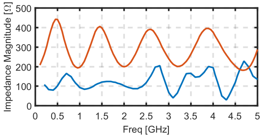
Fig. 3. 17 Simulated impedance (magnitude) from the simulated infinite array of self-complementary spirals in free space (red) and non-complementary spirals with substrate RO4350B, \epsilon_r = 3.66 (blue).
