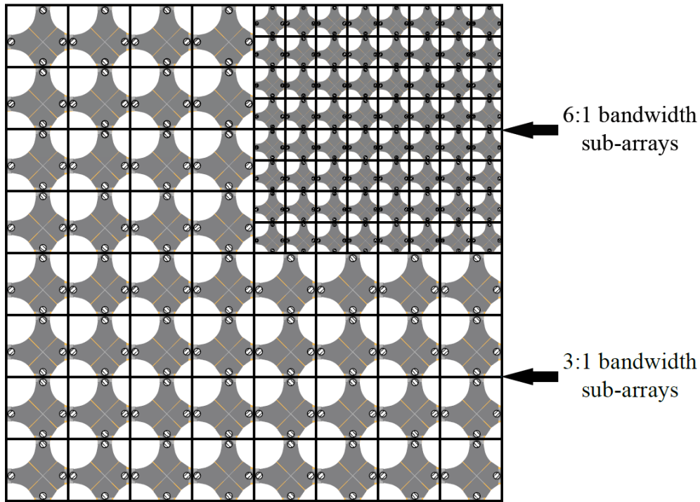
Fig. 1. 19 Sub-array view of a PUMA wavelength-scaled array (L-shape configuration) consisting of a 8 \times 8 6:1 PUMA sub-array with three 4 \times 4 3:1 PUMA sub-arrays (Lee et al., 2016).
