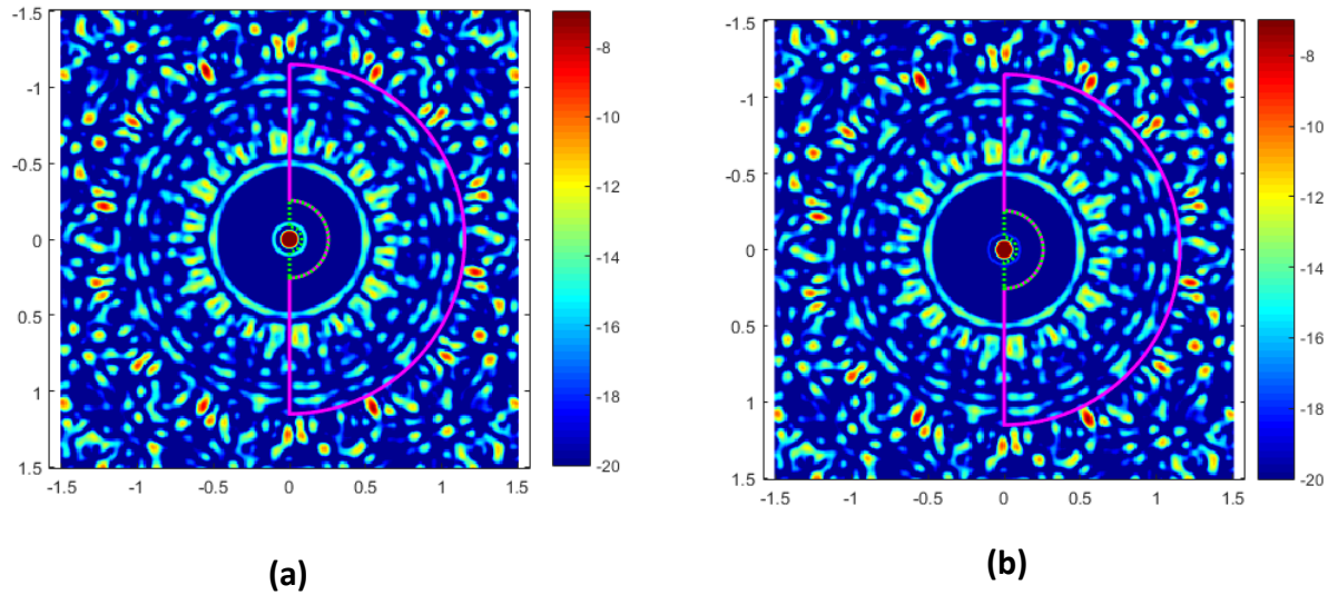
Fig. 2. 27 Array factor of the optimized compact concentric ring array using a smaller RSSL search zone for the cost function and weighting the first sidelobe by \sqrt{2} , at 6.9 GHz. In purple we highlight the zone in which we searched for the highest sidelobe excluding the first sidelobe and in dotted green we highlight the zone that was weighted by \sqrt{2} . In (a) the Array Factor of the optimal array with the weighting and in (b) without the weighting.
