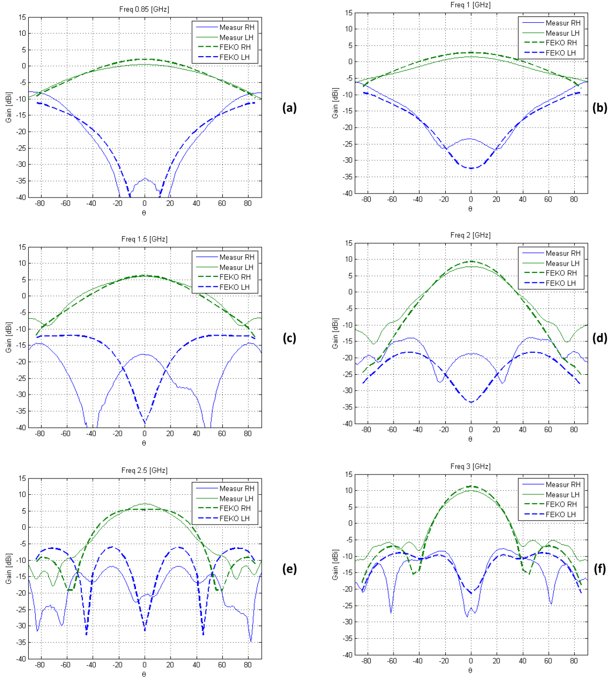
Fig. 3. 27 LH polarization (mode -1) electric field horizontal cuts from the prototype array (Fig. 3. 18) and from the FEKO simulation of the 3x3 4-arm connecting non-complementary spirals array with one layer of elements with matching resistances of 100 \Omega (Fig. 3. 20). In (a), (b), (c), (d), (e) and (f) we have, respectively, the fields at 0.85 GHz, 1 GHz, 1.5 GHz, 2 GHz, 2.5 GHz and 3 GHz.
