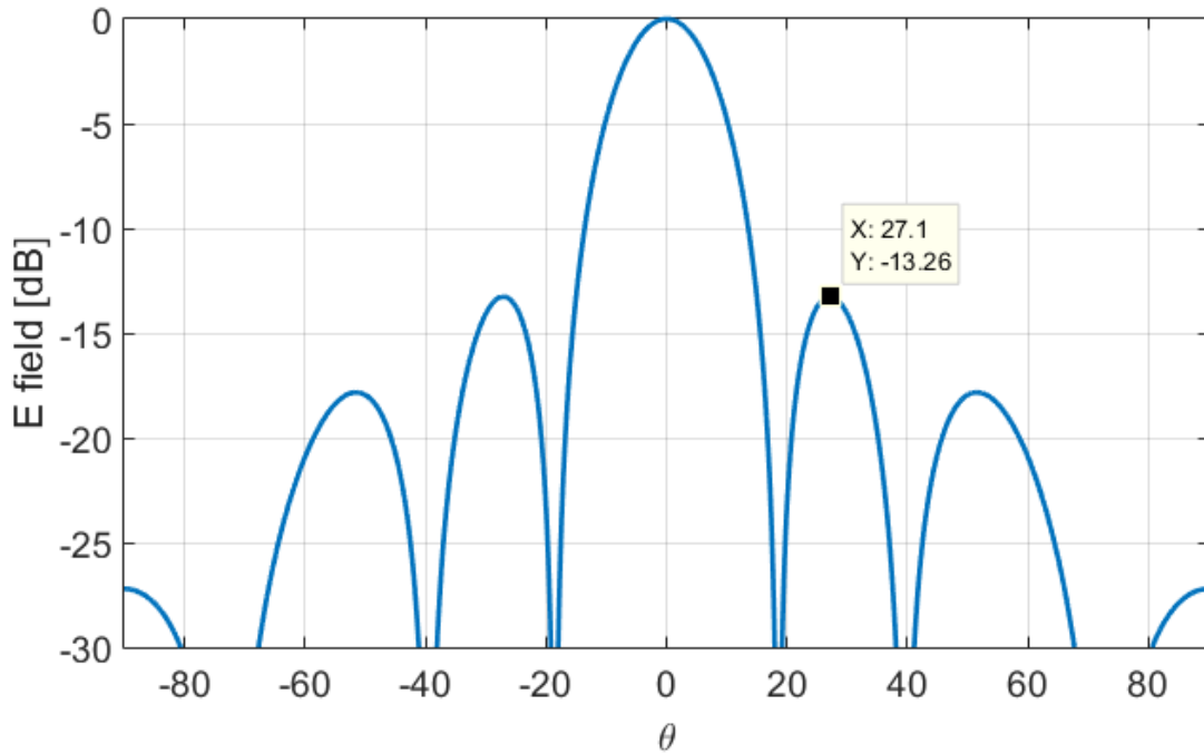
Fig. 1. 3 Arbitrary electric field elevation cut normalized by the main lobe. The relative sidelobe level (RSL) is equal to -13.26 dB as highlighted.
