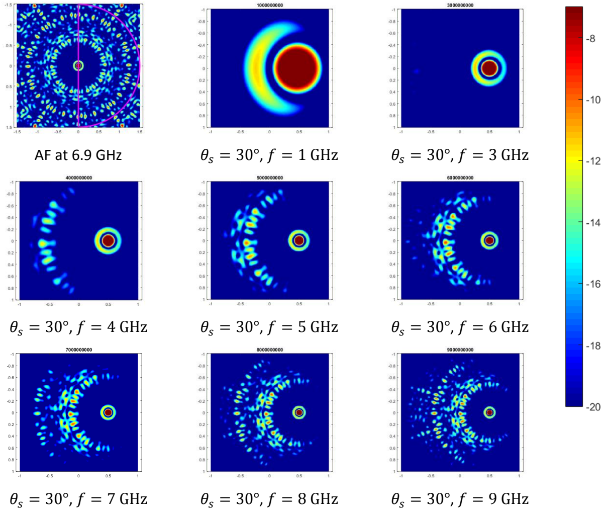
Fig. 2. 21 Array Factor of the optimized array from Table 2. 7 at 6.9 GHz (Top Left). On the other figure we have the radiating pattern of the same array steered to 30^\circ at several frequencies (from 1 to 9 GHz) using the equations (2.10) and (2.12).
