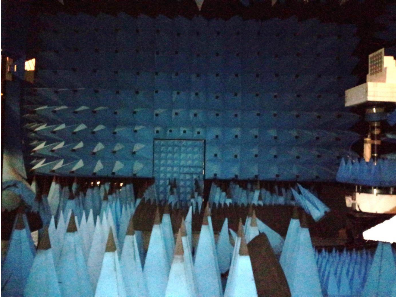
Fig. 3. 24 Spatial configuration of reference antenna and AUT. Distance between antennas is 4.3 m.
