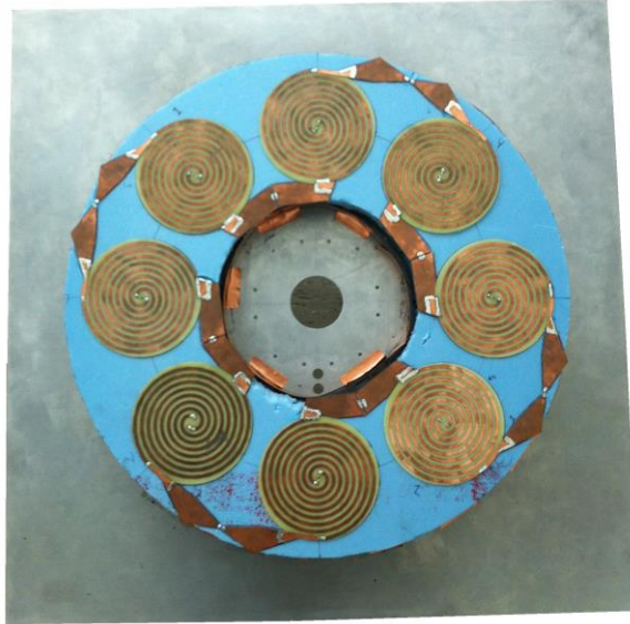
Fig. 2. 2 Ring array of connecting spirals with cavity (Hinostrroza et al., 2016).
