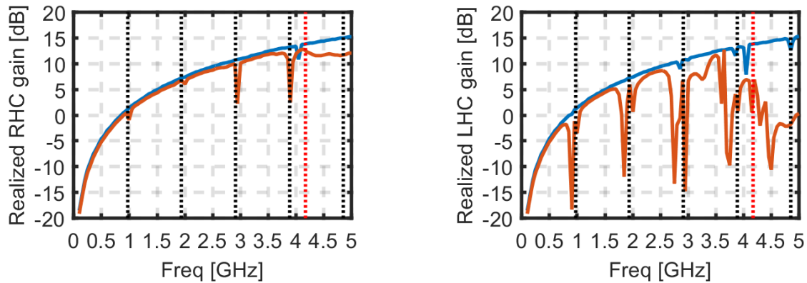
Fig. 3.10 Realized Gain of the 4-arm connecting spirals infinite array. In blue the array is steering to 5 degrees and in red to 30 degrees. The curve to the left shows the main polarization (mode 1) and the curve to the right the opposite polarization (mode -1). The gain curves are traced considering the element pattern from the infinite simulation in FEKO in a 3x3 array. The black dotted vertical lines show the periodic spiral resonances and the red dotted vertical lines show the frequency in which the grating lobes appear when steering to 30°.
