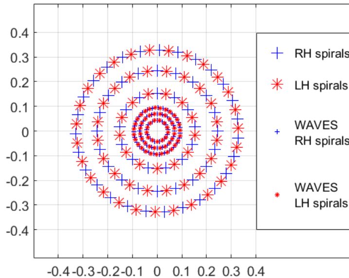
Fig. 2. 34 Elements positions for the Concentric Ring Array of connecting spirals with scaled down WAVES from Table 2. 12.
