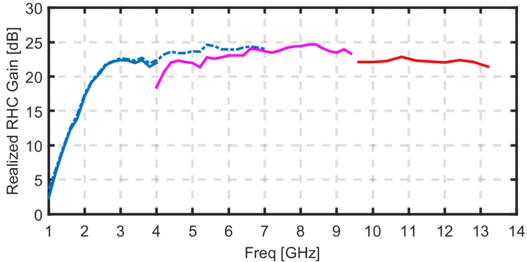
Fig. 2. 52 Realized RHC gain curves when steering to 30^\circ from the Concentric Ring Array of Table 2. 10 from section 2.3.3 (blue dashed line) and from the Concentric Ring Array with scaled WAVES of Fig. 2. 34 from section 2.4.1 with only the larger elements turned on (blue), both the larger and the smaller on at the same time (purple) and only the smaller elements on (red).
