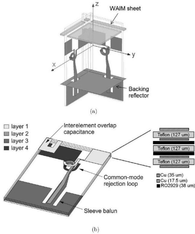
Fig. 1. 10 (a) Three-dimensional view of the array unit cell and (b) components of the dipole and the feed structure in the multilayer PCB. (Bolt et al., 2016)
