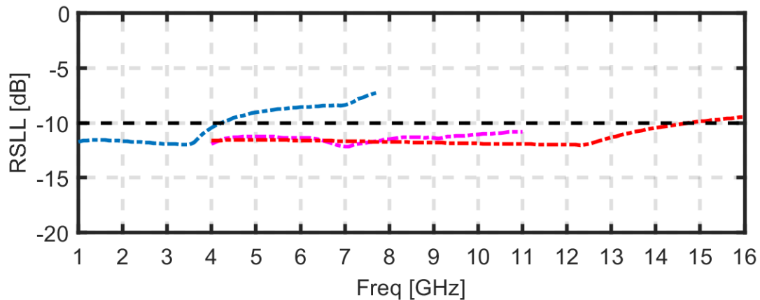
Fig. 2.38 RSLL for the Concentric Ring Array with scaled WAVES using equation (2.13). The blue curve is the RSLL for the larger elements alone. The purple curve is the RSLL for both the smaller and the larger elements turned on together. The red curve is the RSLL when we have only the smaller elements turned on. The dashed black line is the limit from the specifications.
