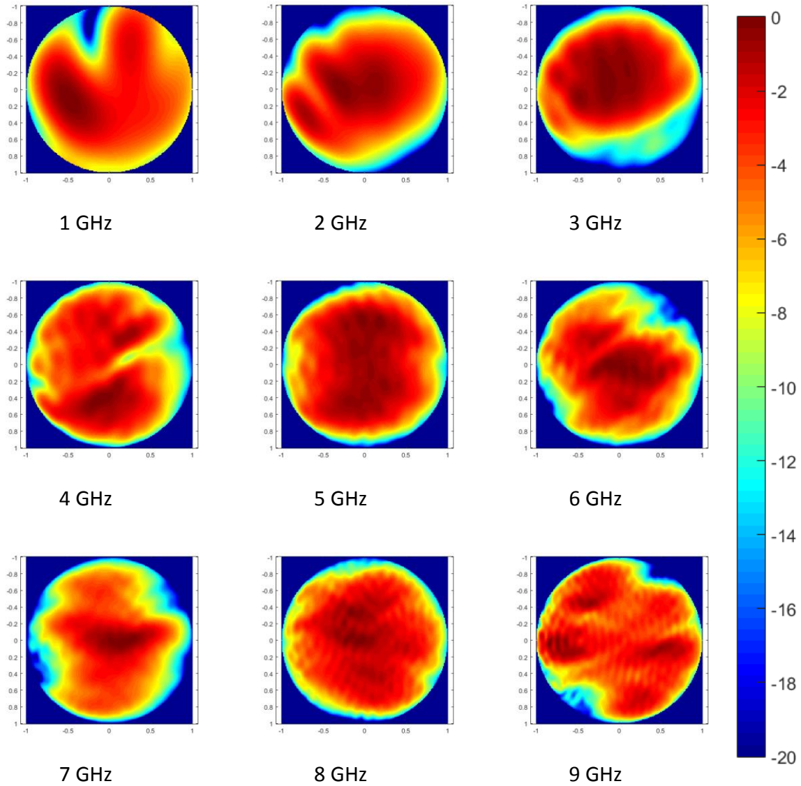
Fig. 2. 19 Element pattern from FEKO simulation of a one ring array of connecting spirals with a radius on 16.95 cm and 14 elements per polarization, with only one element connected to a feeding source and the other adapted by matching resistances, from 1 to 9 GHz in the u v space.
