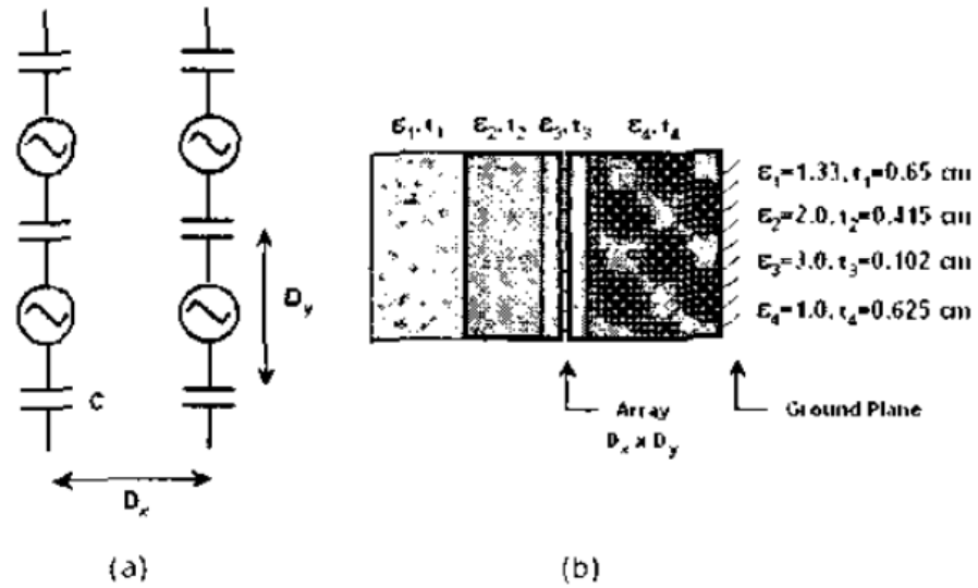
Fig. 1. 7 (a) Circuit model (b) Dielectric Profile (Munk et al., 2003)
