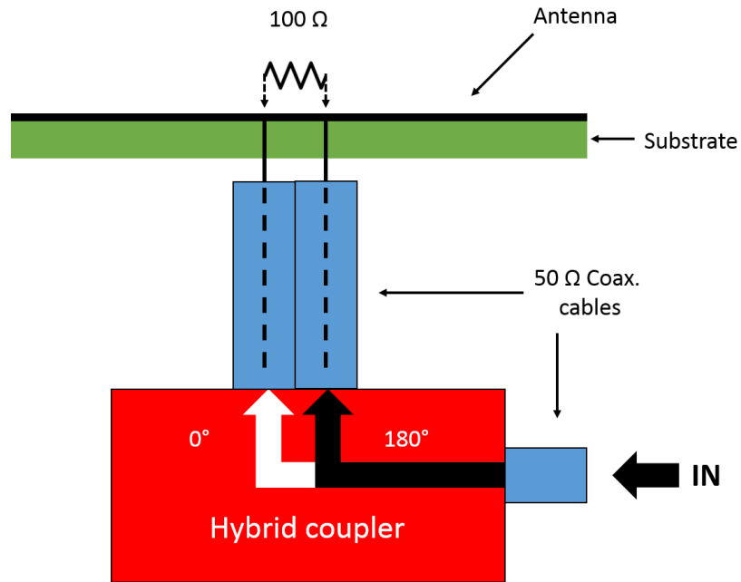
Fig. 3. 14 A simple balun with an impedance transformation from 100\ \Omega to 50\ \Omega using a hybrid coupler.
