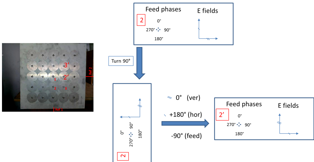
Fig. 2. 56 Scheme showing how to obtain the all the antennas radiation from the measured antennas thanks to the array symmetry. At first we have the antenna numbered 2 (3), and we rotate the fields by 90°. This way the originally vertical cut becomes the horizontal cut (one tick) and the originally horizontal cut becomes the vertical cut (two ticks). Finally, we take the negative of the horizontal cut (one tick) and we compensate the extra rotation on the feeding phases by adding a 90° phase to both cuts, resulting in 2' (3'). Subsequent rotations can provide the fields from the other antennas.
