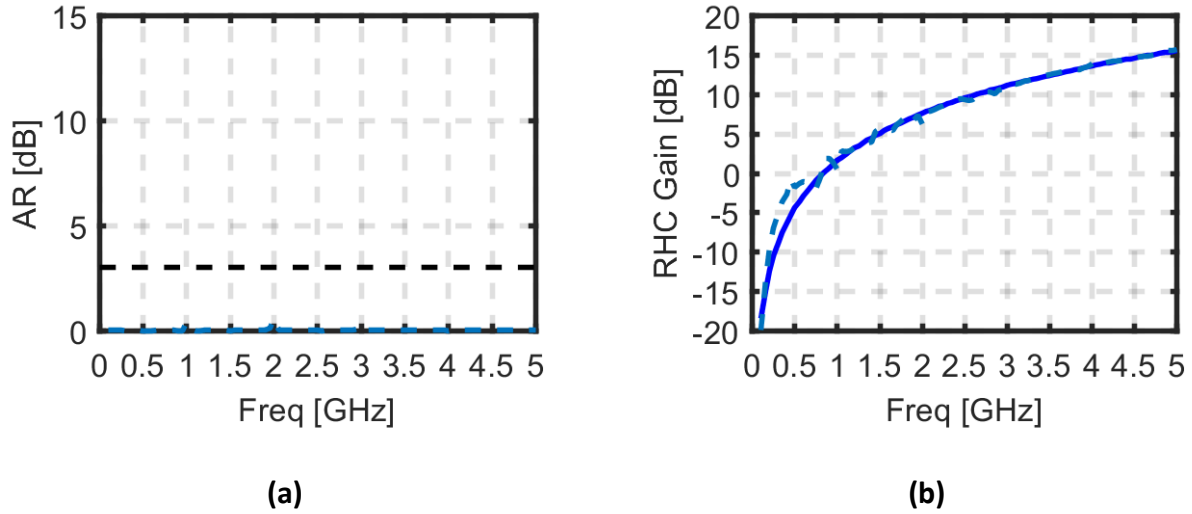
Fig. 3. 7 FEKO simulation of the 3x3 (dash-dotted blue) 4-arms connecting spiral arrays with one layer of elements with matching resistances of 290 \Omega . In (a) we show the AR of the finite array and in (b) the RHC gain. The solid blue line in (b) comes from the 3x3 array of connected spirals using the embedded element pattern from the infinite simulation of the 4-arms connecting spirals infinite array for comparison.
