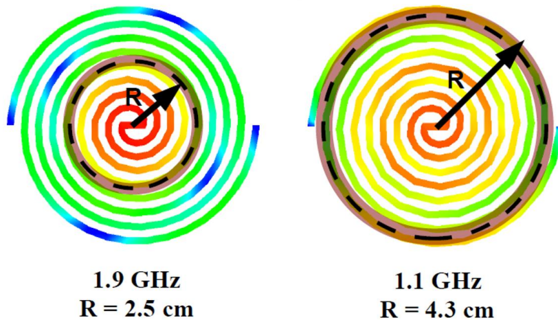
Fig. 1. 4 Normalized current density (30 dB dynamic range from red to blue) along the arms of an Archimedean spiral antenna for different frequencies of operation.
