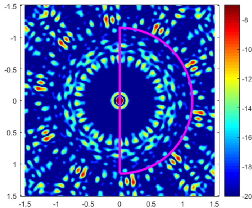
Fig. 2. 23 Array factor of the optimized compact concentric ring array using a smaller RSLL search zone for the cost function, at 6.9 GHz. In purple we highlight the zone in which we searched for the highest sidelobe for our optimization.
