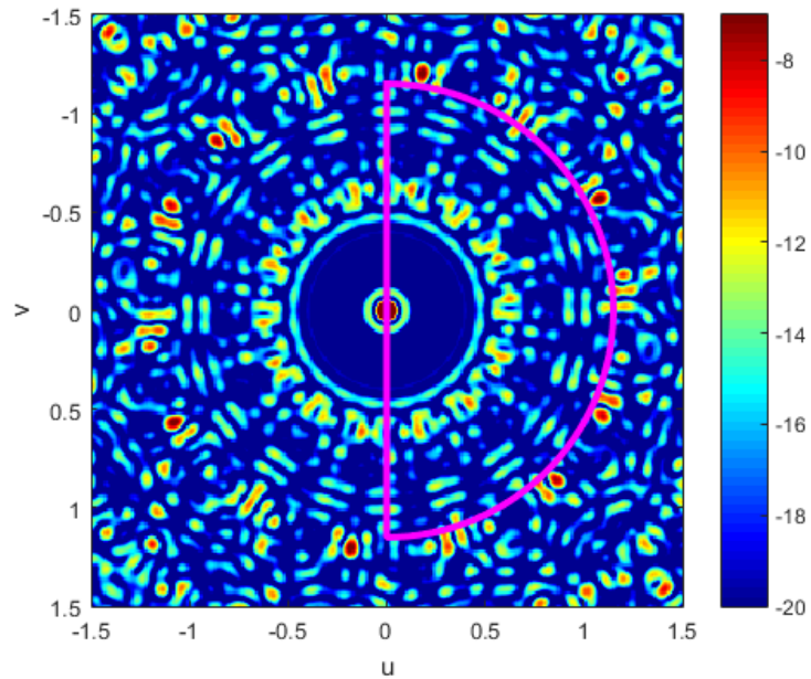
Fig. 2. 35 AF of the larger elements in the optimized Concentric Ring Array with scaled WAVES from Table 2. 12 at 6.9 GHz. In purple we highlight the region in which the sidelobes were optimized.
