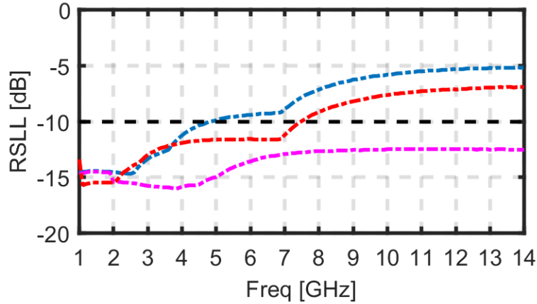
Fig. 2. 46 RSLL for the Concentric Ring Array with interleaved WAVES of Fig. 2. 44 using equation (2.13). The blue curve is the RSLL for the larger elements alone. The purple curve is the RSLL for both the smaller and the larger elements turned on together. The red curve is the RSLL when we have only the smaller elements turned on. The dashed black line is the limit from the specifications.
