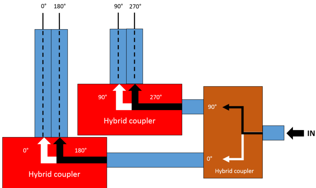
Fig. 3. 15 Connection scheme using 90^\circ and 180^\circ hybrid couplers to obtain 0^\circ , 90^\circ , 180^\circ and 270^\circ phases for a balanced feed for a 4-arm spiral antenna.
