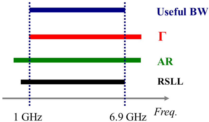
Fig. 2. 53 The bars correspond to the bandwidth definitions listed. In red we have the bar corresponding to the reflection coefficient, in green the axial ratio and in black the relative sidelobe level. The overall useful bandwidth is the intersection of these three bandwidths.
