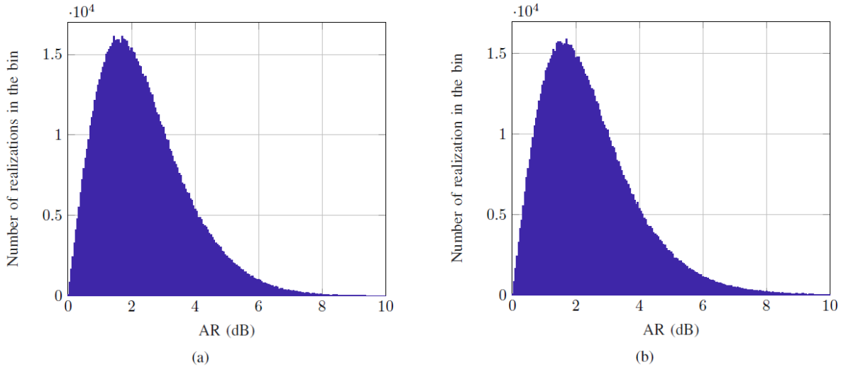
Fig. A. 1 Histogram of the Monte Carlo simulations of the AR calculations for a single crossed dipoles element at broadside. (a) with approximations in (A.24) (b) without approximations. The bins in the histogram have a 0.05 dB width.
