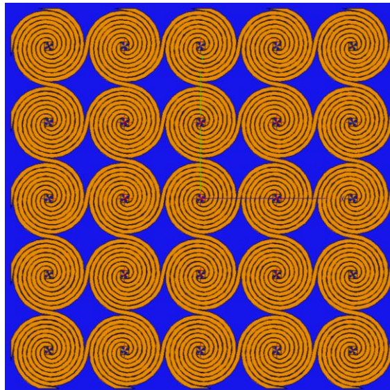
Fig. 3. 20 FEKO model of 4-arm connected spirals 5x5 array.
