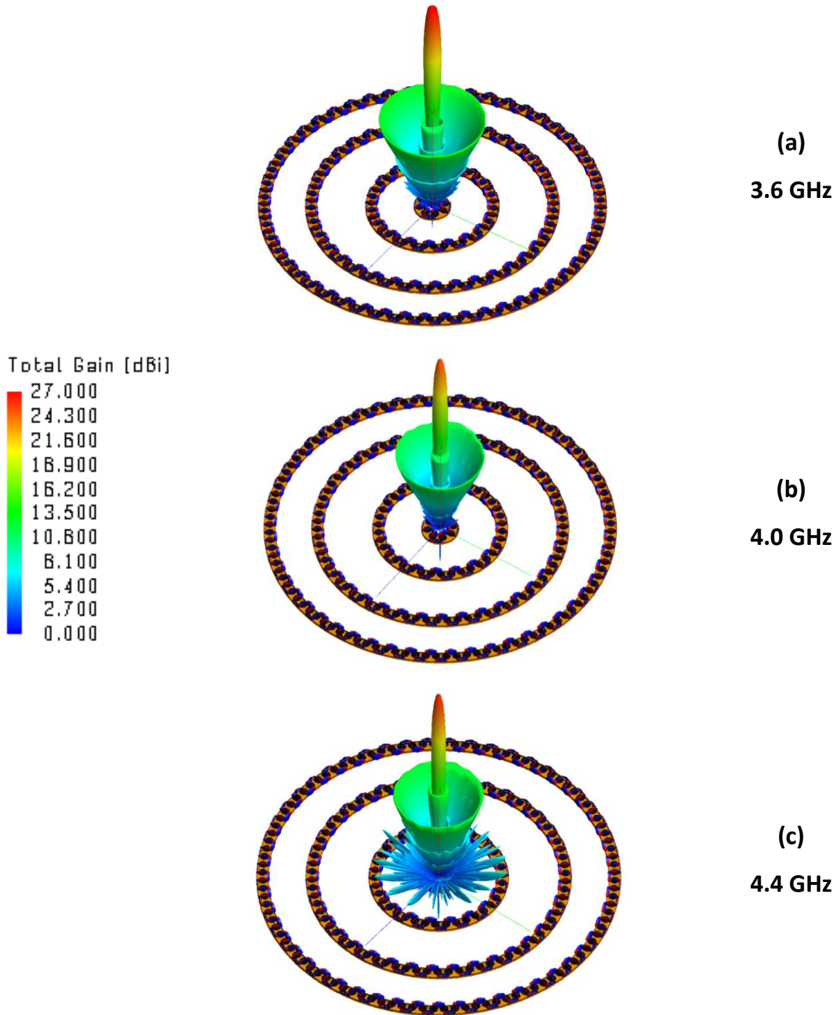
Fig. 2. 8 Radiating Pattern from the FEKO simulation of the concentric ring array of Fig. 2. 6 from (Hinojosa et al., 2014) with added connections between spirals at broadside. In (a) we have the Radiating Pattern at 3.6 GHz, in (b) at 4 GHz and in (c) at 4.4 GHz.
