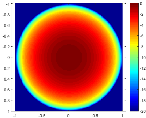
Fig. 2. 18 Element pattern from equation (2.10) in the u v space.
