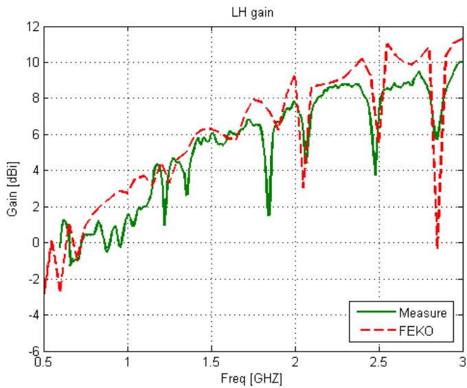
Fig. 3. 25 RHC gain (a) and LHC gain (b) from the prototype array (Fig. 3. 18) and from the FEKO simulation of the 3x3 4-arm connecting non-complementary spirals array with one layer of elements with matching resistances of 100 \Omega (Fig. 3. 20).
