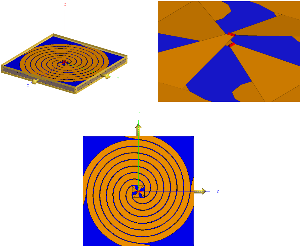
Fig. 3. 16 Unitary cell of the infinite array of non-complementary 4-arms connecting spirals over a RO4350B substrate, \epsilon_r = 3.66 .
