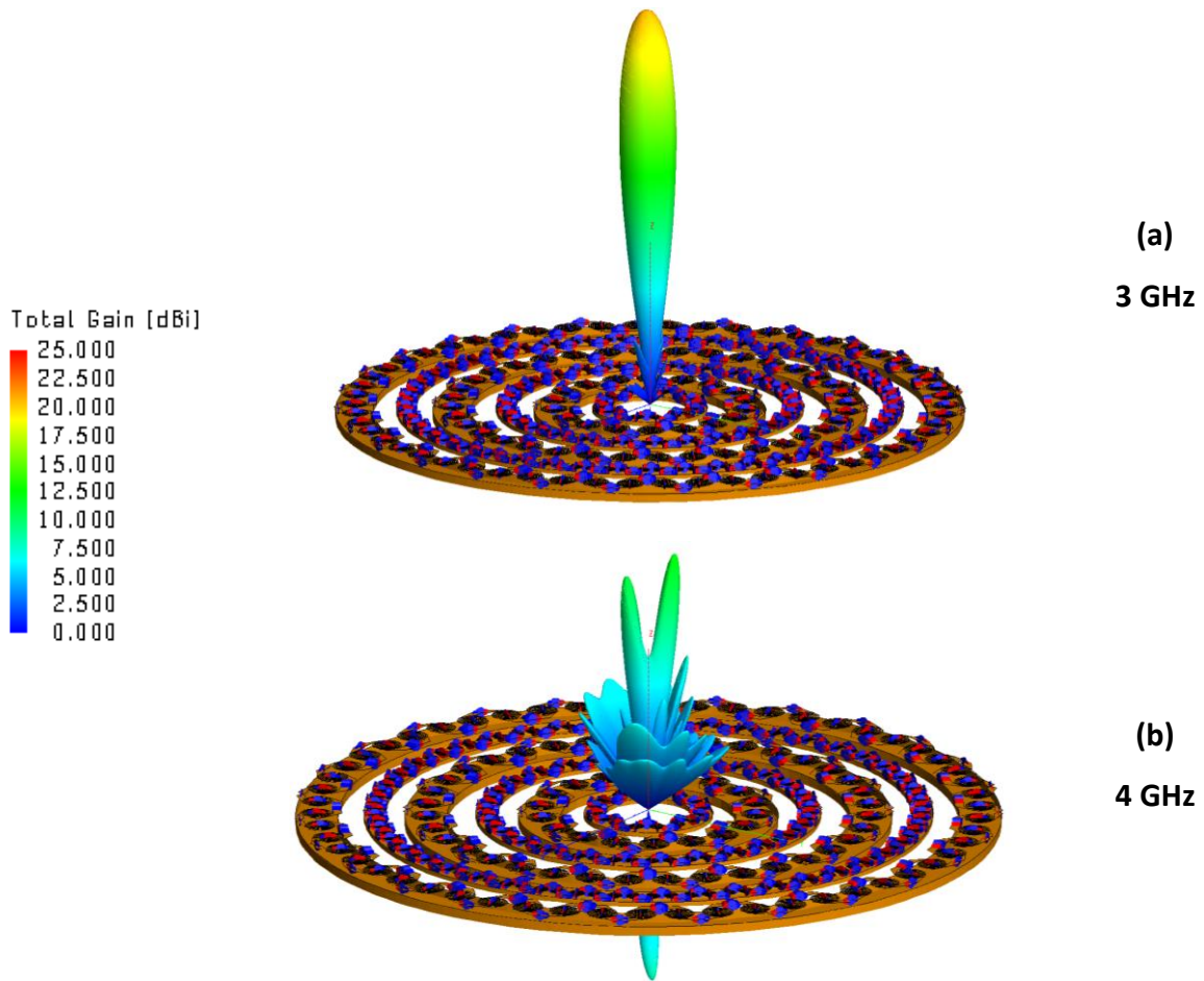
Fig. 2. 48 Radiating Pattern from the FEKO simulation of the optimized Concentric Ring Array of connecting Spirals with interleaved WAVES of Fig. 2. 44 with all elements turned on at broadside. In (a) we have the Radiating Pattern at 3 GHz and in (b) at 4 GHz.
