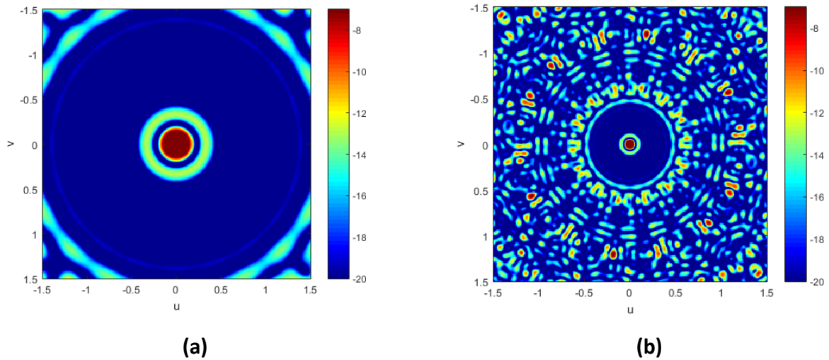
Fig. 2. 36 AF of the smaller elements in the optimized Concentric Ring Array with scaled WAVES from Table 2. 12 at 6.9 GHz (a) and 24.15 GHz (b).
