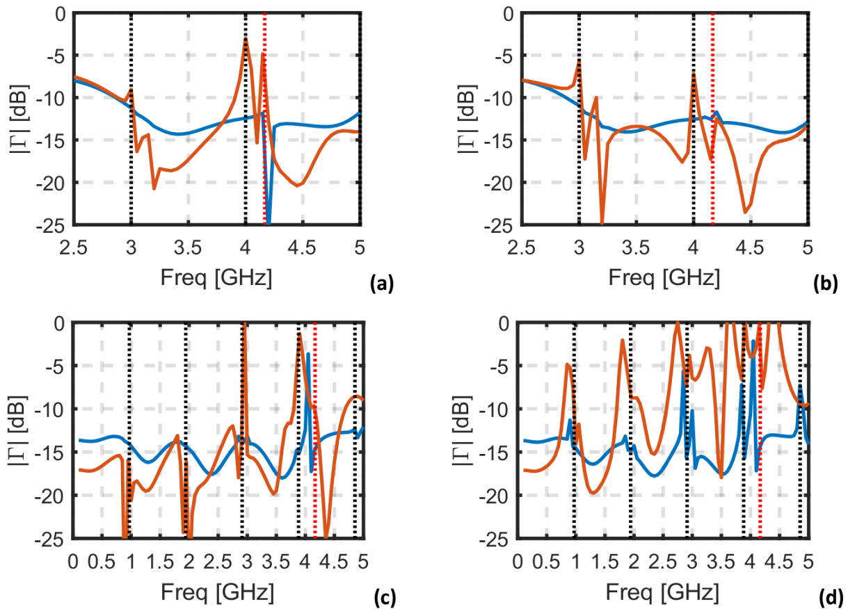
Fig. 3.11 Reflection Coefficient of the 4 arm disconnected spirals infinite array in (a) and (b) and of the 4-arm connecting spirals infinite array in (c) and (d). In blue the array is steering to 5 degrees and in red to 30 degrees. In (a) and (c) we show the main polarization (mode 1), and in (b) and (d) we show the opposite polarization (mode -1). The black dotted vertical lines show the periodic spiral resonances and the red dotted vertical lines show the frequency in which the grating lobes appear when steering to 30°.
