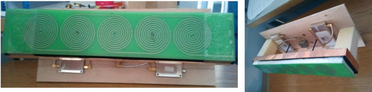
Fig. 2. 1 Linear array of connecting spirals with cavity (Guinvarc'h et al., 2012).
