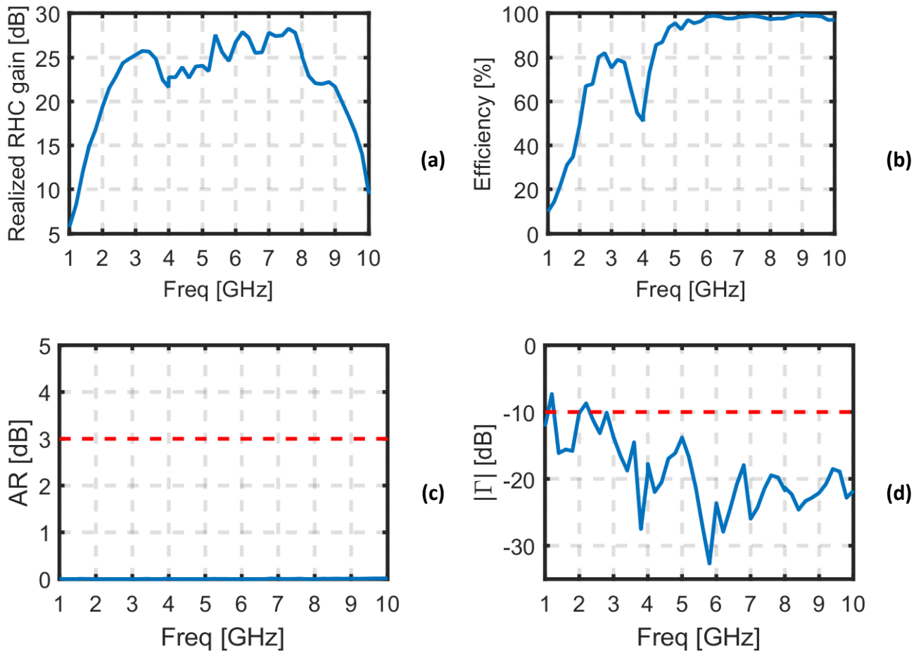
Fig. 2. 29 FEKO simulation of the concentric ring array of connecting spirals from the 3 rd optimization (Table 2. 10) at broadside ((a) Gain, (b) Efficiency, (c) AR and (d) |\Gamma| typical case). The dashed red lines indicate the limit from the specifications.
