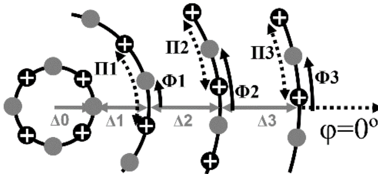
Fig. 2. 3 Concentric ring array: filled and cross circles represent RH and LH polarized spirals, respectively. Interleaved spirals make the array sparse, so high lobes (“grating lobes”) appear in the radiating visible zone. Concentric rings with radius and relative rotations optimized to reduce those lobes can enhance the RSSL in higher frequencies.
