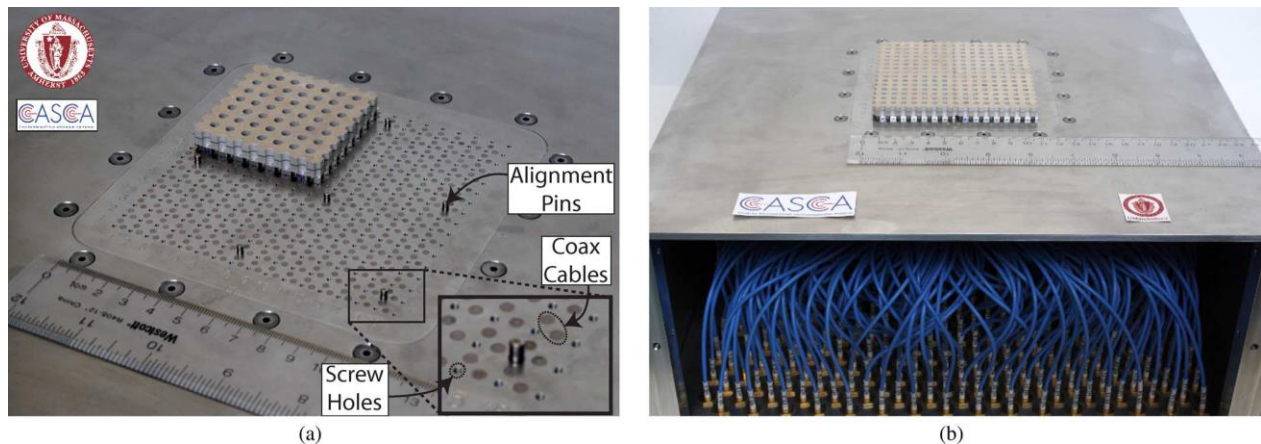
Fig. 1. 13 Modular and solderless assembly of a 16x16 dual-polarized PUMA array prototype on the measurement fixture. (a) Top plate of the fixture and the mounting of an 8x8 module. (b) Full array mounted on measurement fixture, with the side panel removed to show the coaxial cables exiting the top plate and terminating in SMA connectors on the backside of the fixture (Holland et al. , October 2012).
