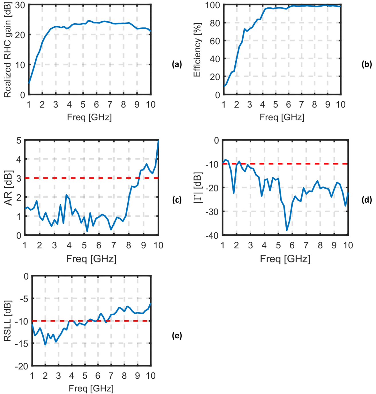
Fig. 2. 30 FEKO simulation of the concentric ring array of connecting spirals from the 3 rd optimization (Table 2. 10) steered to 30° ((a) Gain, (b) Efficiency, (c) AR and (d) |\Gamma| typical case and (e) RSLI). The dashed red lines indicate the limit from the specifications.
