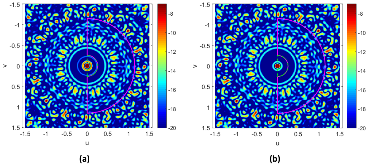
Fig. 2. 42 Array factor of the larger elements in the optimized concentric ring array with scaled WAVES weighting the first sidelobe by 1.6 (see Table 2. 14), at 6.9 GHz. In purple we highlight the zone in which we searched for the highest sidelobe excluding the first sidelobe and in dotted green we highlight the zone that was weighted by 1.6. In (a) the Array Factor of the optimal array with the weighting and in (b) without the weighting.
