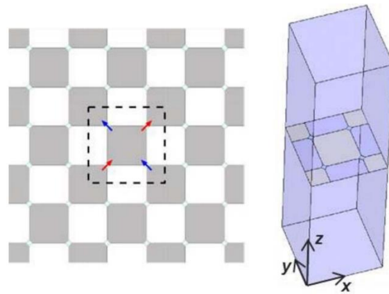
Fig. 1. 12 Self-complementary connected array aperture and unit cell (Varault et al. , 2017).
