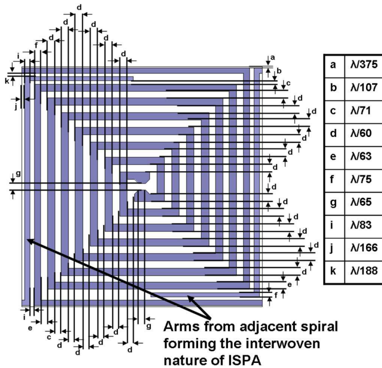
Fig. 1. 15 Interwoven Spiral Array (ISPA) unit cell and its dimensions in wavelengths. The element is fed at the center. (Tzanidis et al., 2011)
