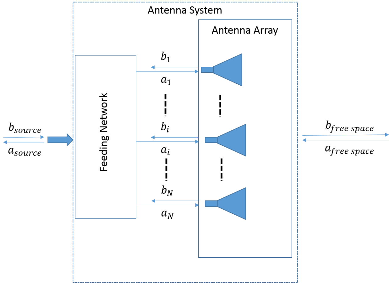
Fig. 1. 2 Scheme of an antenna system with a feeding network and an antenna array.
