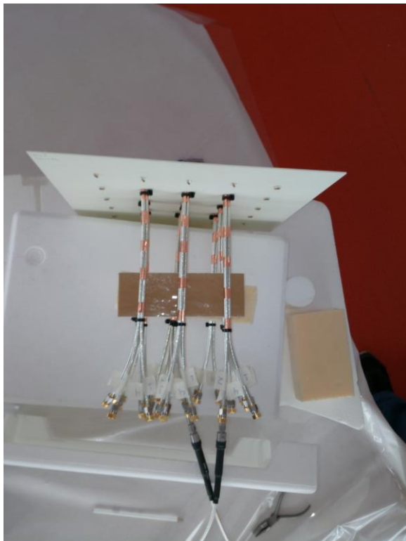
Fig. 3. 19 Measurement of the S parameters of the prototype array of 4 arms connecting non-complementary spirals.
