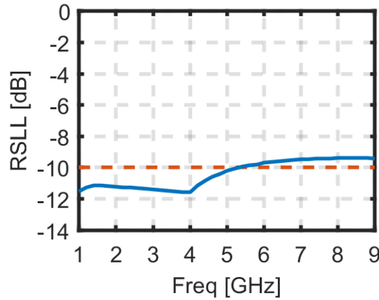
Fig. 2. 20 RSLL vs freq. for the compact concentric ring array 1 st optimization using a \cos^q approximation for the element pattern. The dotted red line is the limit from the specifications.
