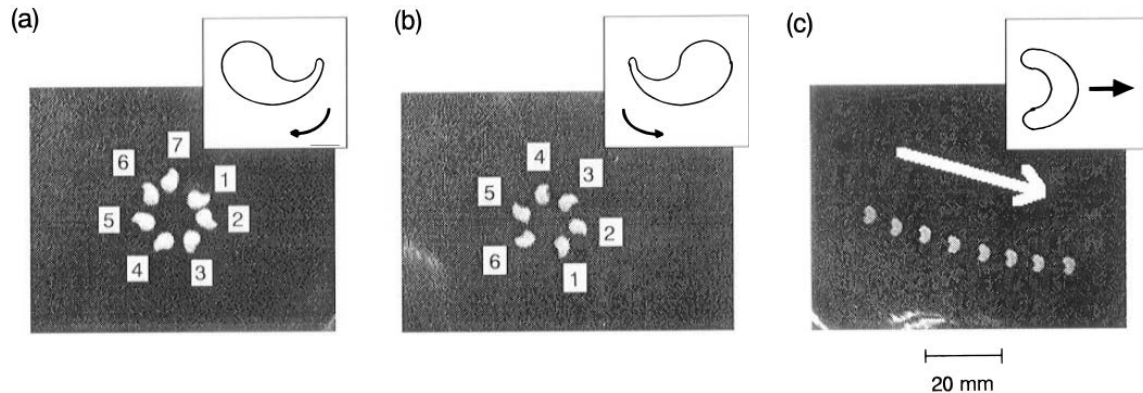
Figure 1.15: Camphor systems on liquid surfaces. A: Motion of camphor scraggings with different geometries that lead to different kind of motions (Figure taken from [37]).
