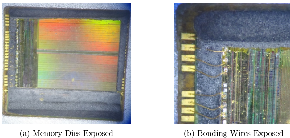
Figure 5.21: eMMC Decapsulated
