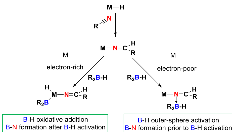
Scheme 1-21: General considerations for the hydroboration of nitriles with metal hydride complexes
