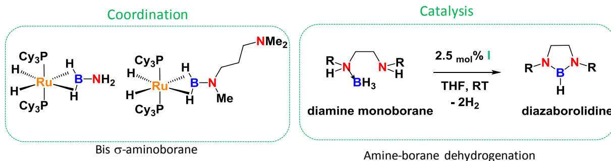
Scheme 1-24: Amine-borane coordination to RuH_2(H_2)_2(PR_3)_2 (left) and related catalysis (right)
