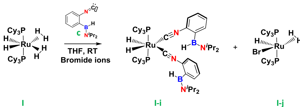
Scheme 3-18: Products from the addition of \text{RuH}_2(\text{H}_2)_2(\text{PCy}_3)_2 in the crude mixture containing c
