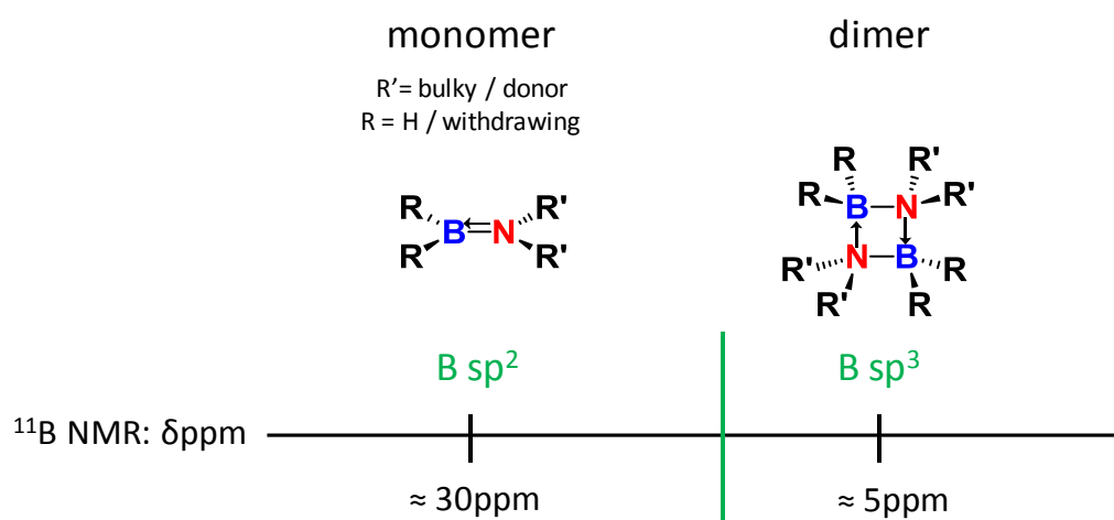
Figure 1-3: ^{11}\text{B} NMR generic values for monomeric and dimeric aminoboranes
