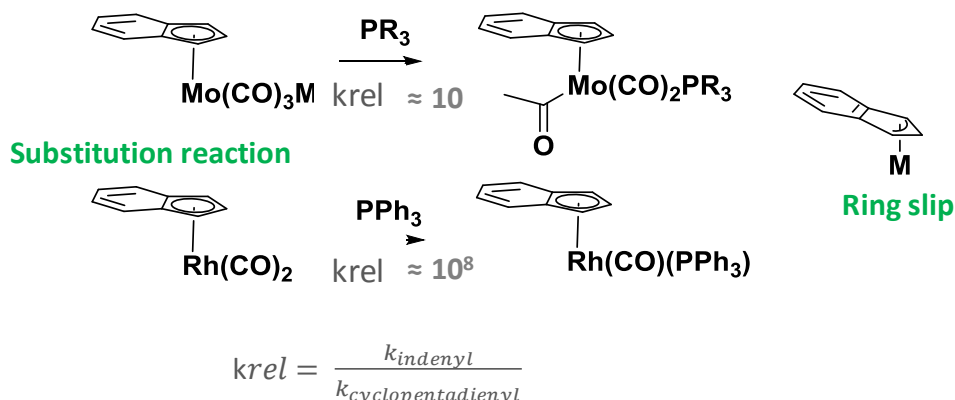
Scheme 1-4: Rate acceleration of ligand-induced migratory insertion and substitution reaction of indenyl complexes compared to the cyclopentadienyl analogues (k rel = relative reaction rate constant)
