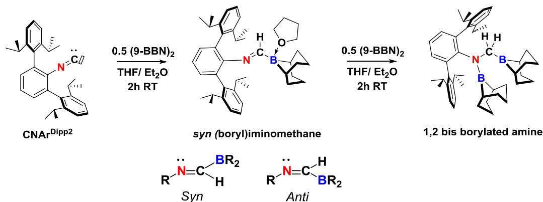
Scheme 1-14: Hydroboration of \text{CNAr}^{\text{Dipp}2} isocyanide with 9-BBN
