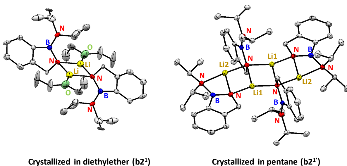
Figure 4-1: Asymmetric unit of b2 1 and b2 1' crystals
