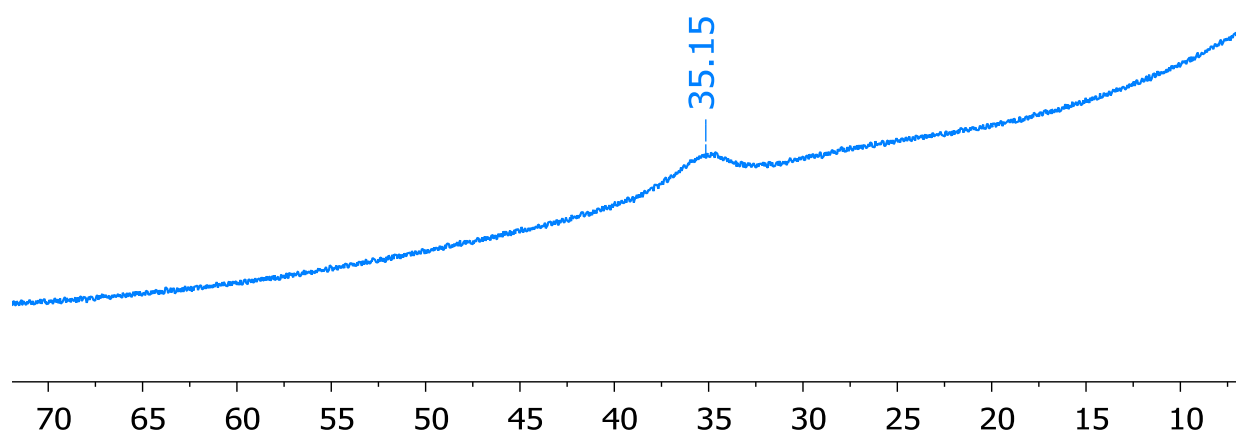
^{11}\text{B} NMR spectrum of compound d2 (toluene d_8 , 128.39 MHz, 298K)
