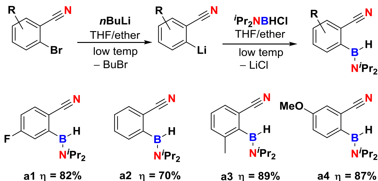
Scheme 2-1: Synthetic procedure towards aryl(cyano)(aminoborane) derivatives
