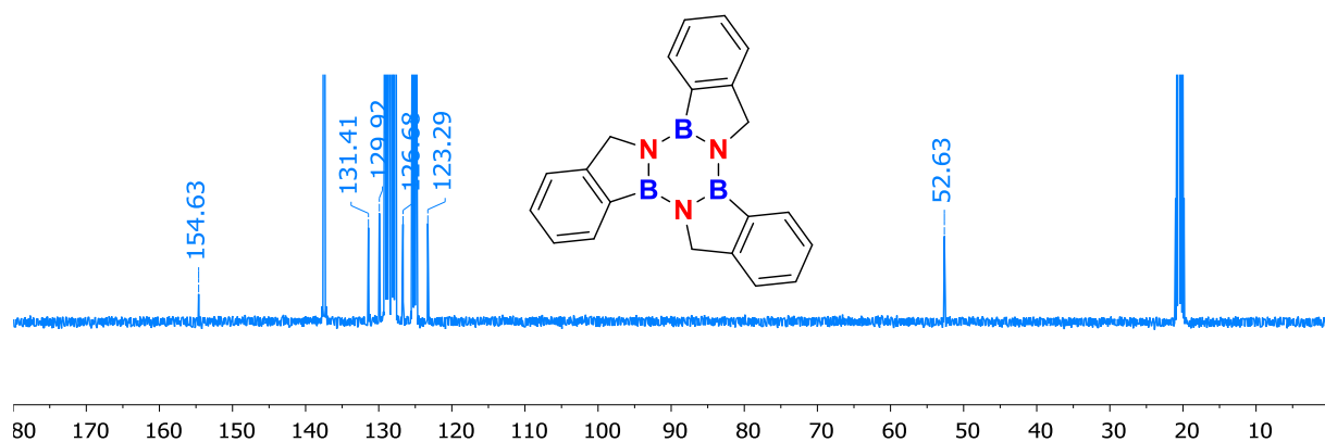
^{13}\text{C}\{^1\text{H}\} NMR spectrum of compound d2 (toluene d_8 , 100.63 MHz, 298K)
