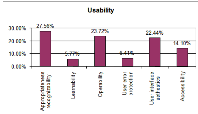
Figure 5.11: Distribution of usability metrics
