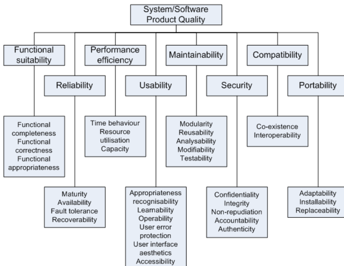
Figure 2.4: Quality model in ISO 25010
