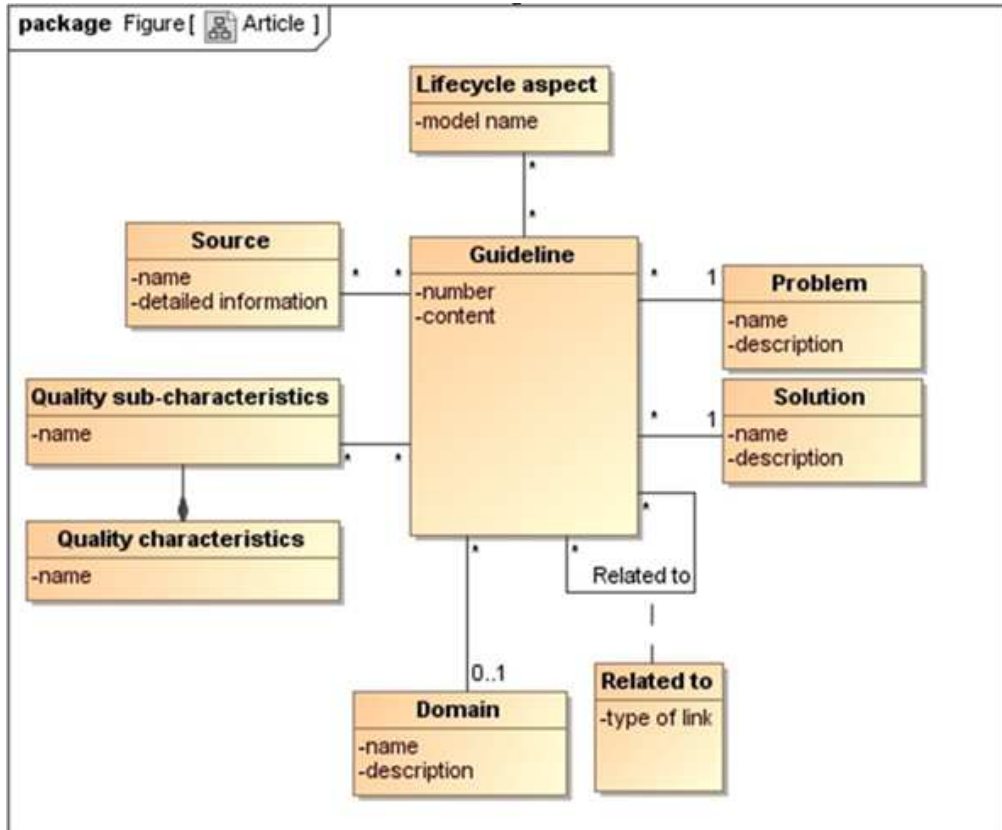
Figure 6.4: The meta-model of guidelines
