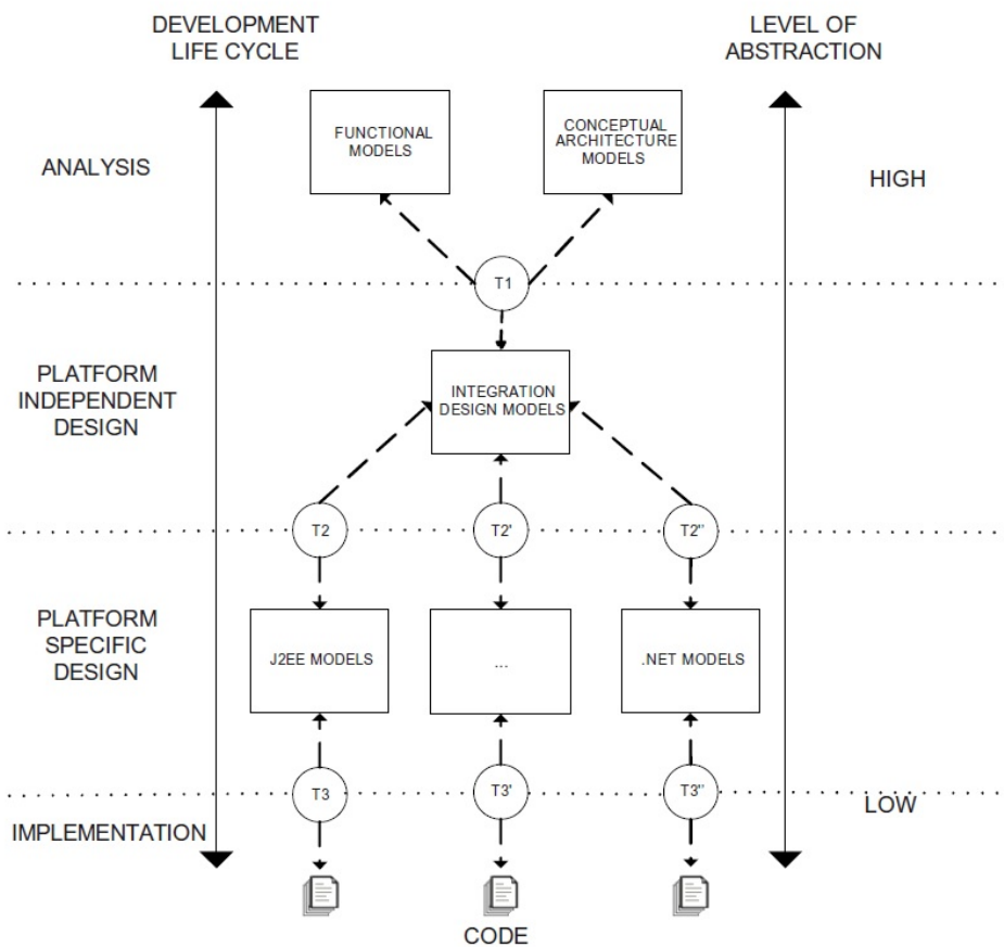
Figure 2.6: WebSA Web development process [Beigbeder and Cachero 2004]
