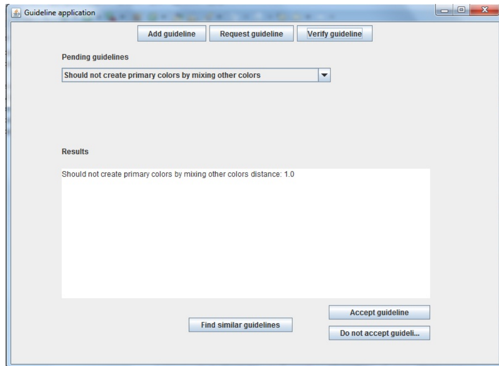
Figure 6.10: Verifying guidelines
