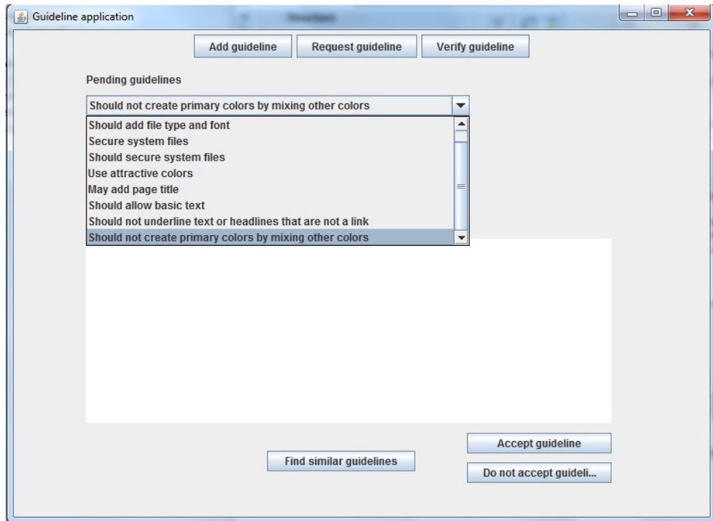
Figure 6.9: Check guidelines
