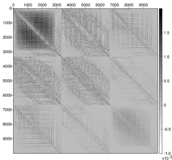
Figure 3.3 – Hessian operator H(m_0) corresponding to a 2D frequency-domain multi-parameter FWI problem for the reconstruction of the P -wave velocity, the density, and an attenuation parameter.
