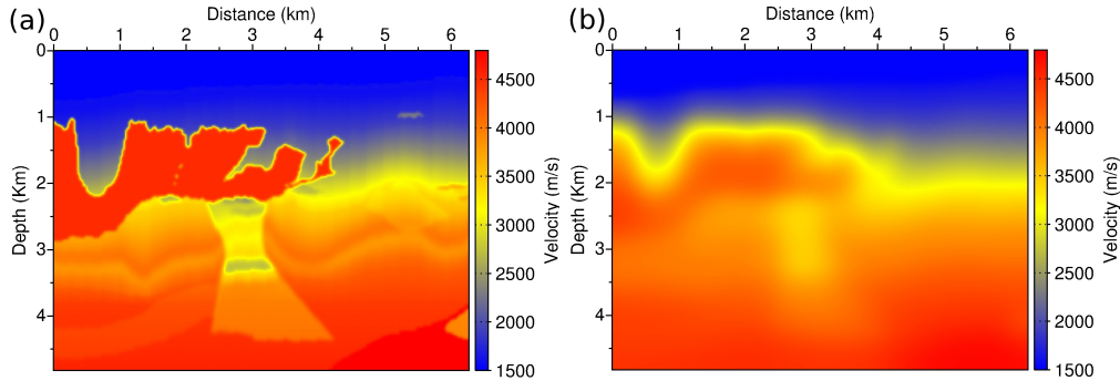
Figure 3.10 – BP 2004 synthetic exact model (a), initial model (b).
