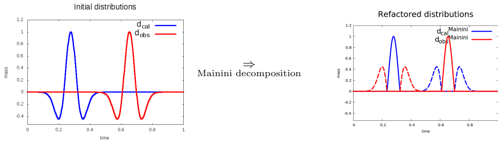
Figure 2.1 – Mainini decomposition.
