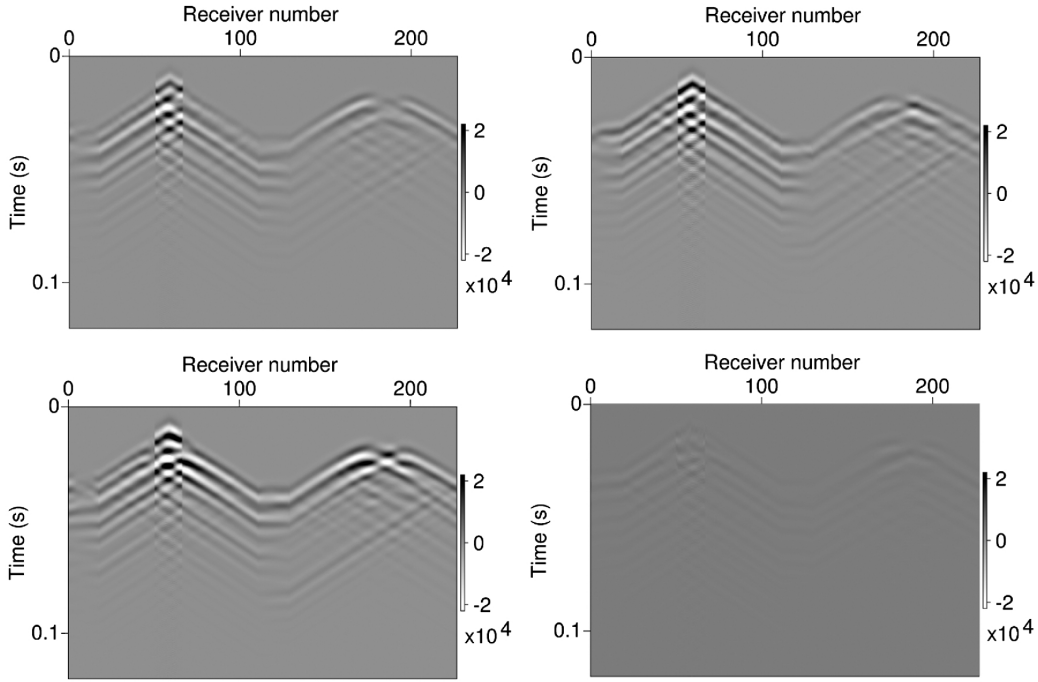
Figure 3.9 – Residuals associated with the estimated models. Steepest-descent (top left), l -BFGS (top right), Gauss-Newton (bottom left), Newton (bottom right).
