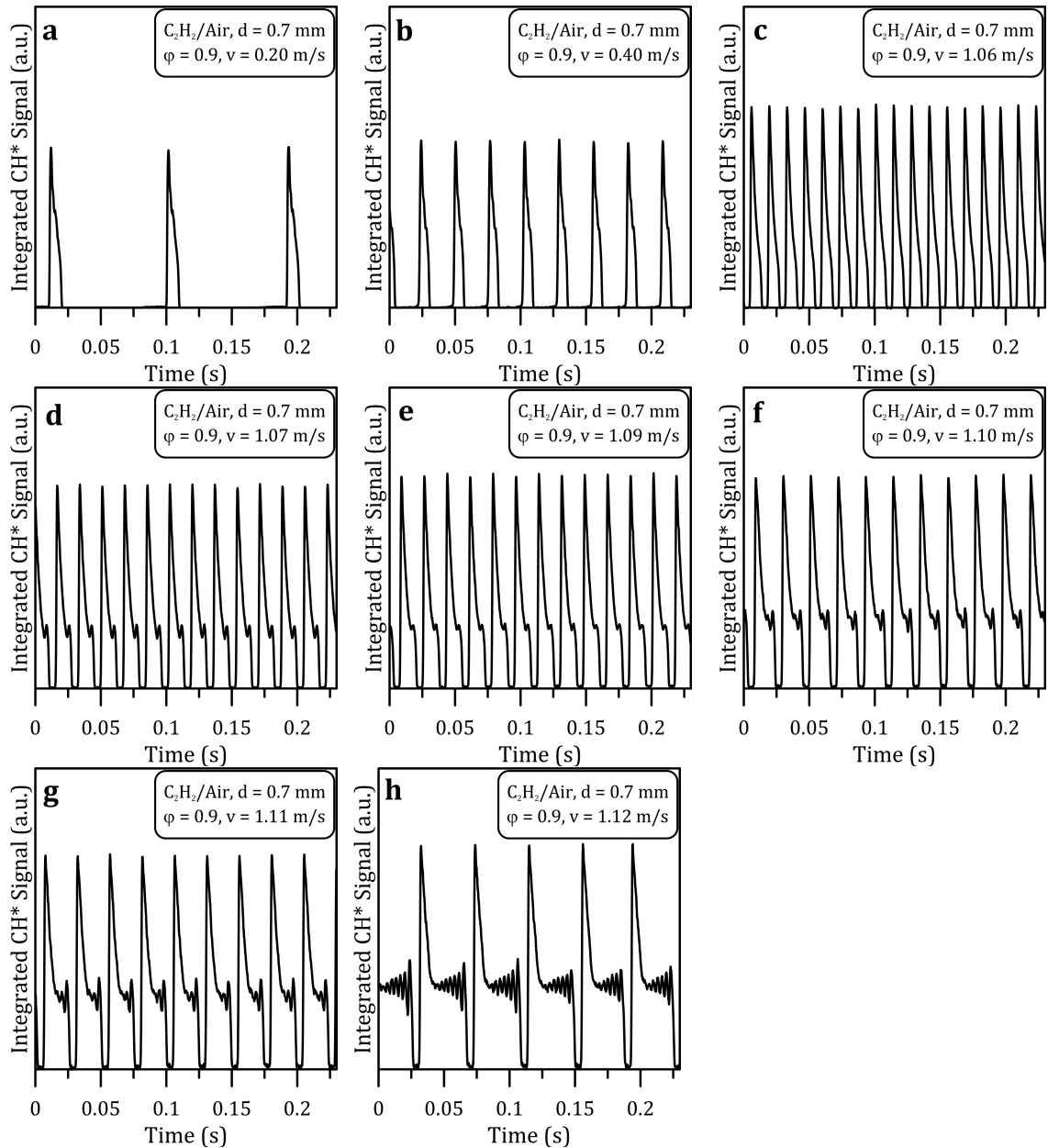
Figure E10: Temporal evolution of \text{C}_2\text{H}_2/\text{Air} unstable flames at \phi = 0.9 . a) v = 0.20 m/s, Fr = 10.9 Hz (FREI), b) v = 0.40 m/s, Fr = 30.7 Hz (FREI), c) v = 1.06 m/s, Fr = 73.9 Hz (FREI), d) v = 1.07 m/s, Fr = 58.3 Hz (Oscillating FREI), e) v = 1.09 m/s, Fr = 57.2 Hz (Oscillating FREI), f) v = 1.10 m/s, Fr = 47.6 Hz (Oscillating FREI), g) v = 1.11 m/s, Fr = 40.6 Hz (Oscillating FREI), h) v = 1.12 m/s (Oscillating FREI).
