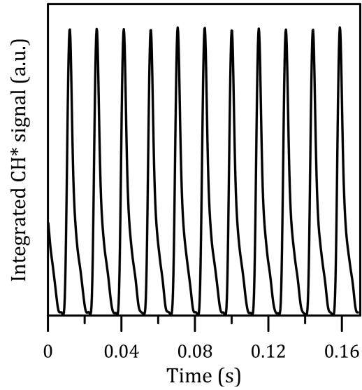
Figure B10: Spatially integrated \text{CH}^* signal at v = 0.32 \text{ m/s} ( \text{CH}_4/\text{air} , \varphi = 1 , d = 2.15 \text{ mm} ).
