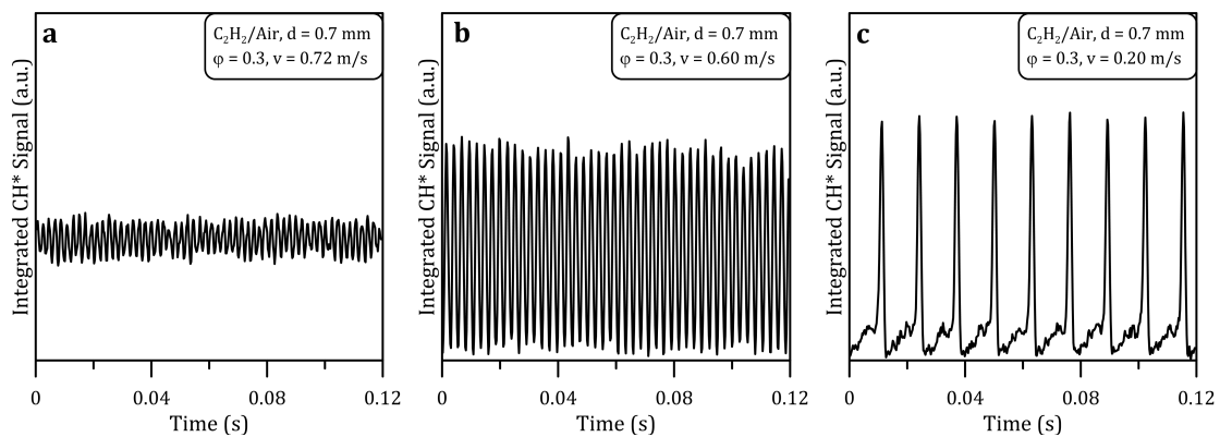
Figure 4.28: Spatially integrated \text{CH}^* signals obtained at \phi = 0.3 . a) v = 0.72 m/s (Oscillating FREI), b) v = 0.60 m/s (Oscillating FREI), c) v = 0.20 m/s (FREI).
