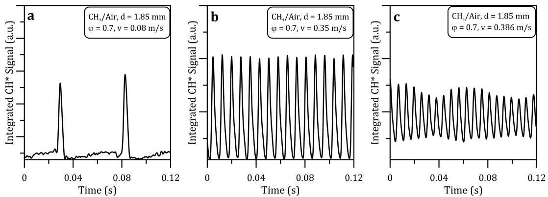
Figure D1: Temporal evolution of \text{CH}_4/\text{Air} unstable flames at \varphi = 0.7 . a) v = 0.08 \text{ m/s} , \text{Fr} = 19.8 \text{ Hz} (FREI), b) v = 0.35 \text{ m/s} , \text{Fr} = 131.1 \text{ Hz} (FREI), c) v = 0.386 \text{ m/s} , \text{Fr} = 160.0 \text{ Hz} (Oscillating FREI).
