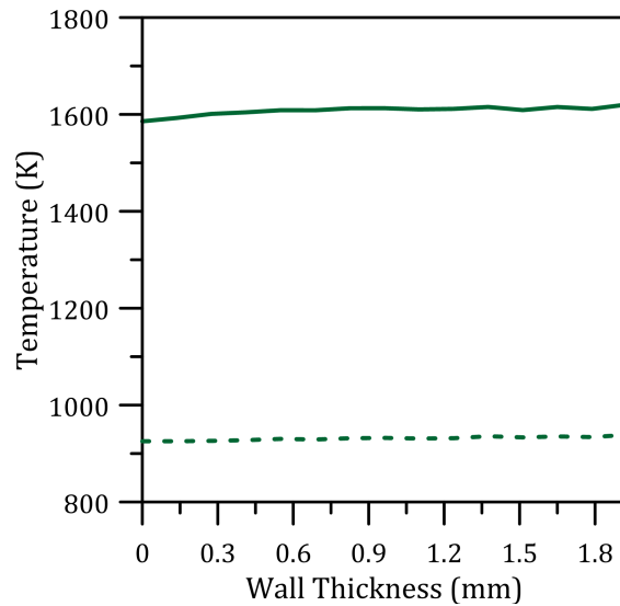
Figure 2.32: Temperature profile along the wall thickness.
