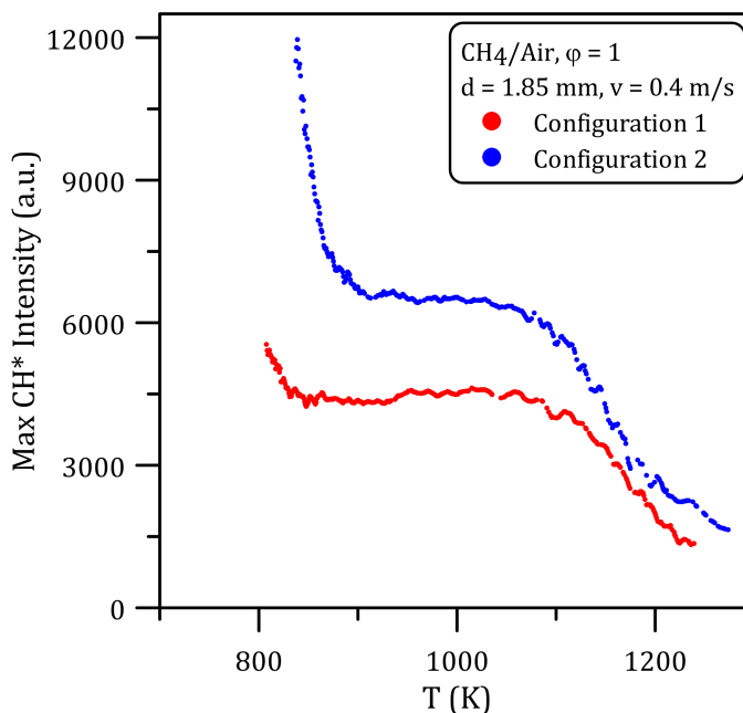
Figure 2.16: \text{CH}^* progression obtained with the two configurations employed.
