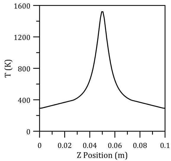
Figure C2: Temperature profile at the wall.
