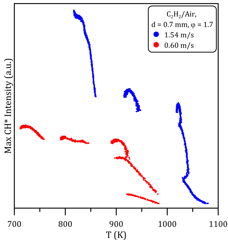
Figure 4.32: Maximum \text{CH}^* progression at \phi = 1.7 at high ( v = 1.54 \text{ m/s} ) and low ( v = 0.60 \text{ m/s} ) inlet velocity.
