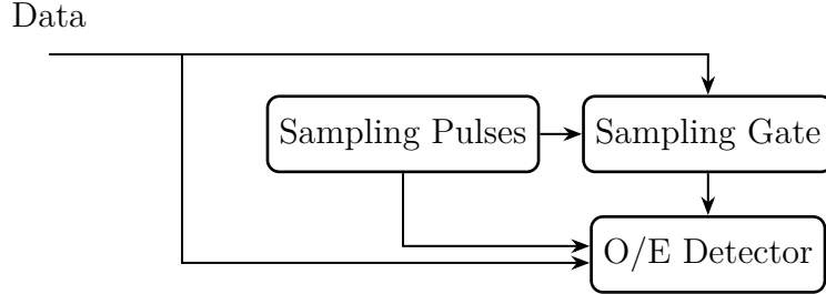
Figure 2.20: Random sampling
