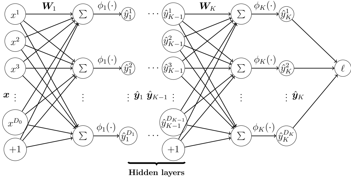
Fig. 1.4 Multilayer perceptron. (Notation: D_k, k = 1, \dots, K is the dimension of the output of the layer k . D_0 = D is the dimension of the input \mathbf{x} of the network. D_K = M is the dimension of the output \hat{\mathbf{y}} of the network, i.e., M . x^i is the i^{\text{th}} component of \mathbf{x} . \hat{y}_k^j is the j^{\text{th}} component of the output representation \hat{\mathbf{y}}_k at the layer k ).
