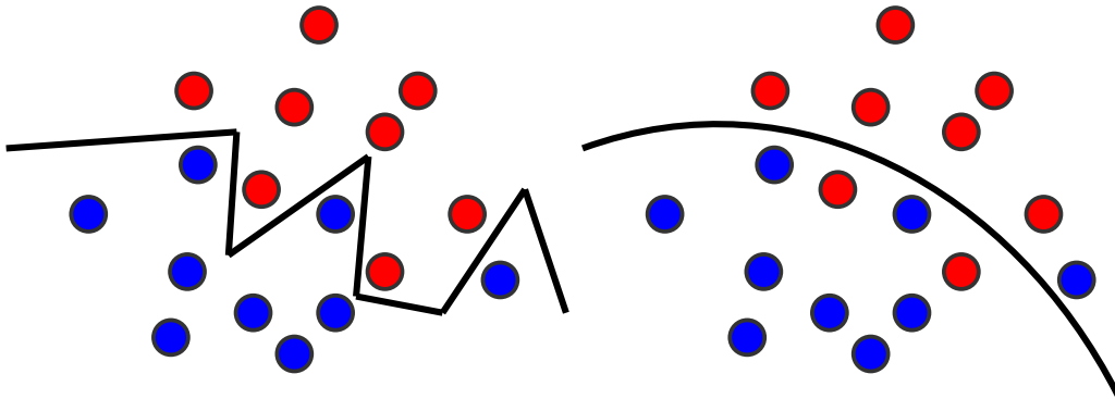
Fig. A.1 The zig-zag line on the left panel is consistent over the blue and red training samples, but it is a complex separation surface that is not likely to generalize well to unseen data. In contrast, the decision surface on the right panel is simpler and might generalize better in spite of its misclassification of few points of the training samples. (Reference: [305])
