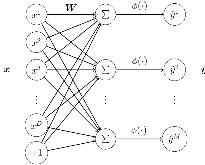
Fig. 1.3 Multiclass perceptron. (Notation: x^i is the i^{th} component of \mathbf{x} . \hat{y}^j is the j^{th} component of \hat{\mathbf{y}} ).
