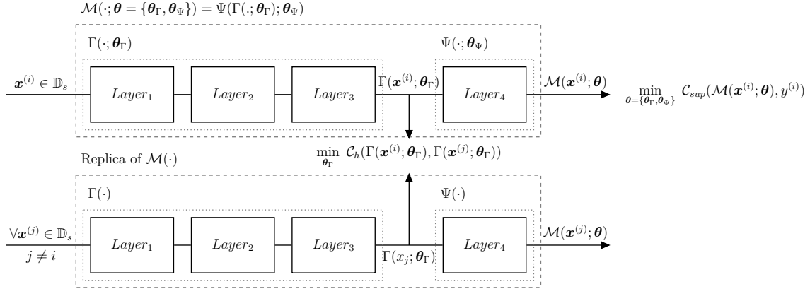
Fig. 3.3 Constraining the intermediate learned representations to be similar over a decomposed network \mathcal{M}(\cdot) during the training phase.
