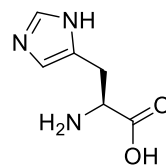
L-Histidine (His)
