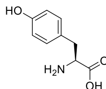
L-Tyrosine (Tyr)
