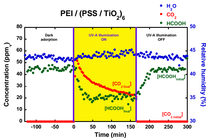
Figure 37: Photocatalytic activity of a PEI/(PSS/TiO 2 ) 6 LbL film
