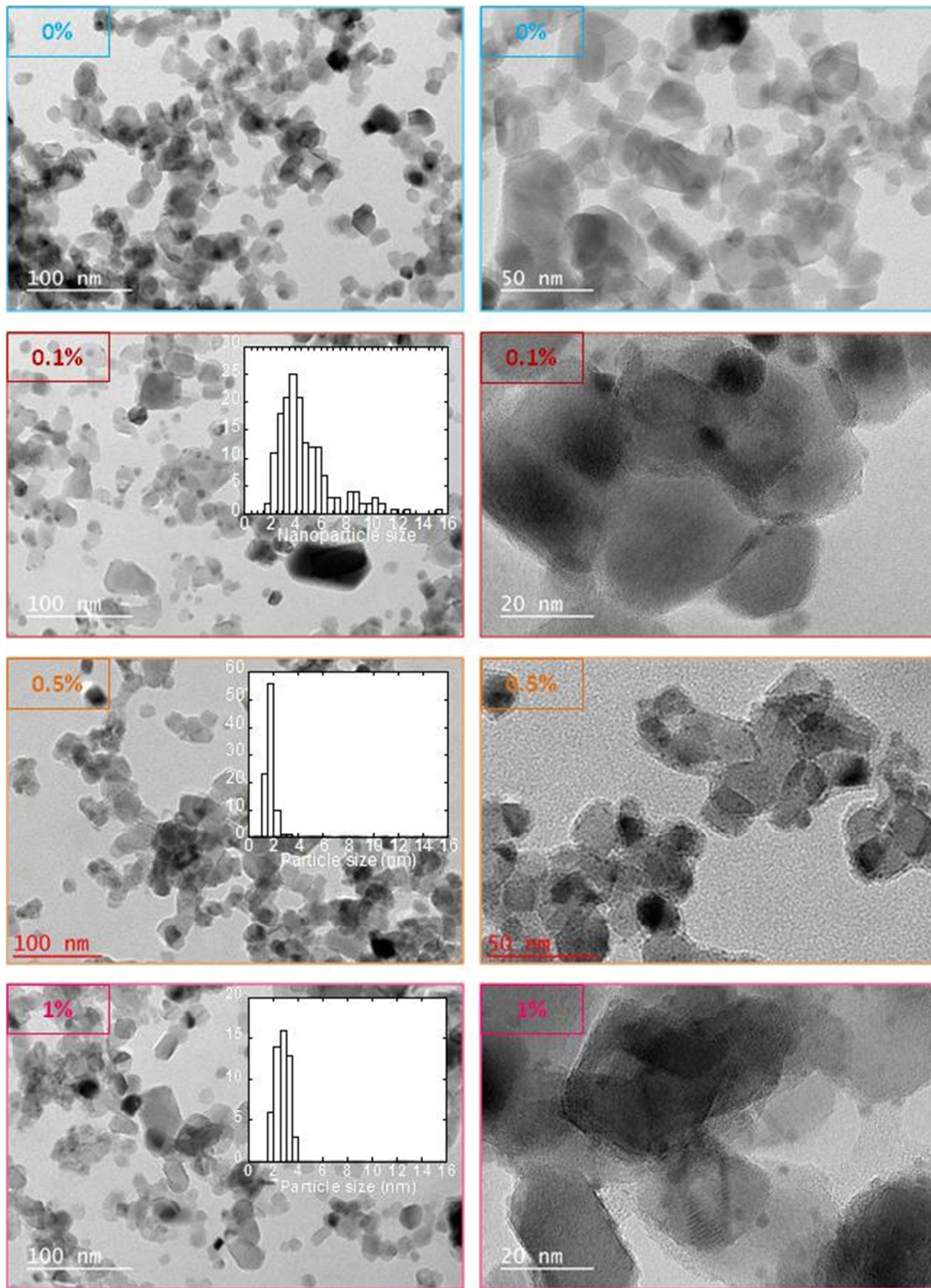
Figure 73 : TEM images of PEI/PSS/TiO 2 /x%Ag films. x = 0%, 0.1%, 0.5% and 1%. The size distribution was assessed only on 56 nanoparticles for the sample with x=1%.
