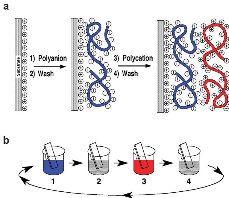
Figure 14: (a) Construction of polyelectrolyte LbL films on a charged flat surface. Once the polyanion (in blue) and the polycation (in red) are successively deposited, a pair of layers has been constructed. (b) LbL thin film construction via the dipping deposition technique. The substrate is alternately immersed in the polyanion solution (1) and in the polycation solution (3), with a rinsing step between each immersion (2 & 4) [17], [18].
