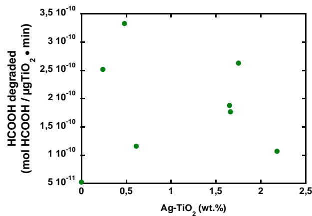
Appendix 10 : Degradation of HCOOH per μg TiO 2 • min, in regards to the silver content in PEI/PSS/(x%Ag-TiO 2 ) films.
