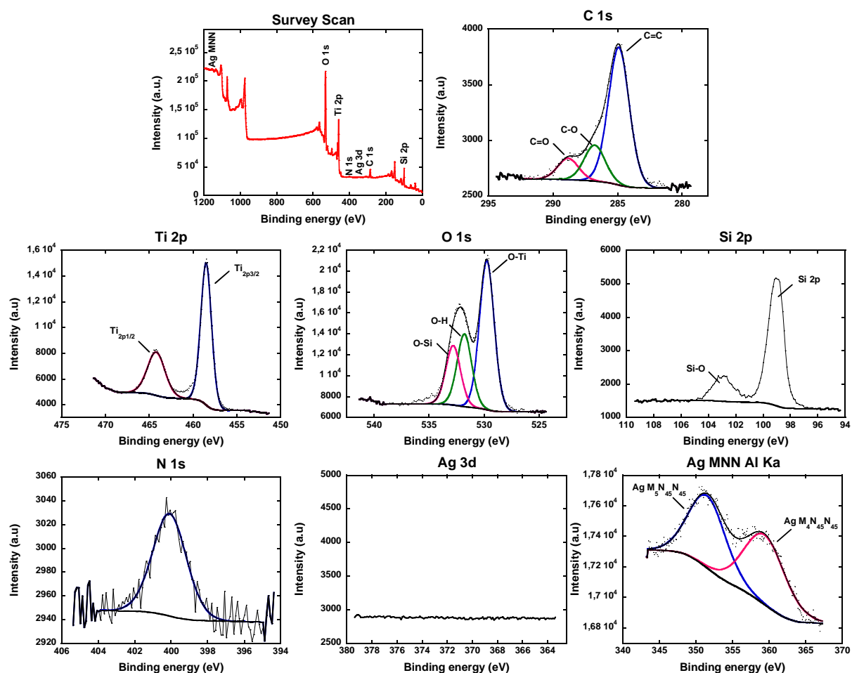
Figure 83 : XPS characterisations of PEI/PSS/(1%Ag-TiO 2 ) LbL film
