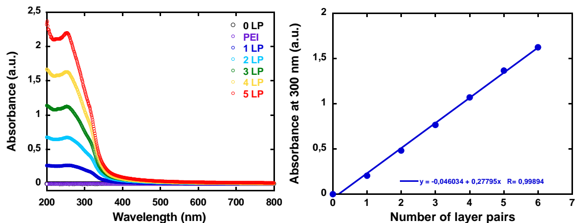
Figure 44: Transmission UV-Visible photospectrophotometry characterisation of PEI/(PSS/TiO 2 ) n film. (Left) film deposition on quartz slide with absorbance increment after each layer pairs deposited. (Right) reported absorbance at 300 nm in regards to the number of layer pairs deposited.
