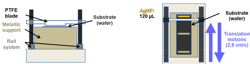
Figure 67: Schematic of the Doctor Blade device (not to scale). (Left) side view of the device, with a substrate placed on the metallic support and below the PTFE blade. (Right) top view of the device with 120 μL of AgNP suspension (yellow lines, 3x40μL) placed onto the substrate.
