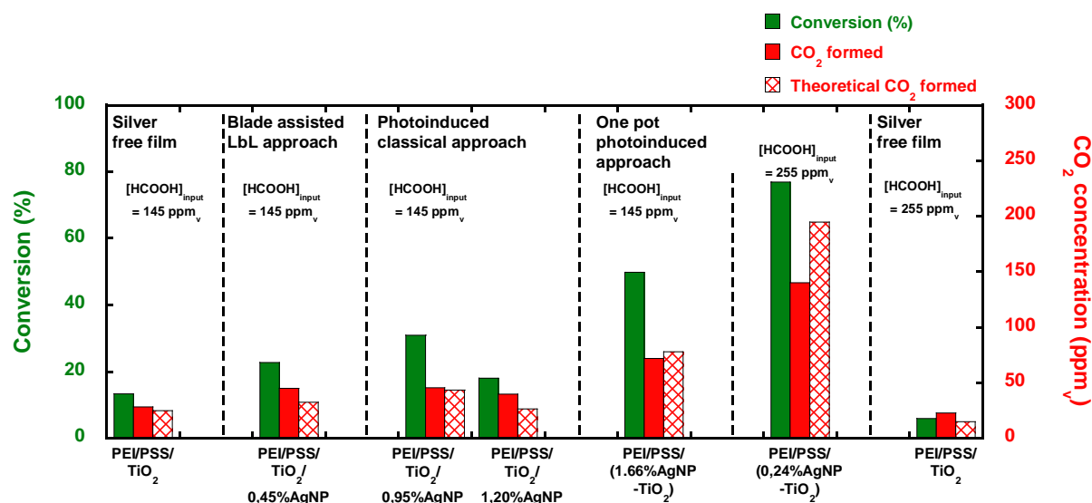
Figure 90: Comparison of the photocatalytic performances shown by Ag-TiO 2 films prepared via the three approaches.
