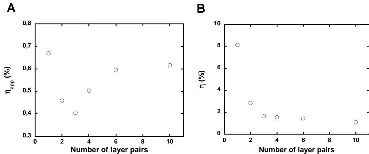
Figure 55: (A) Apparent quantum yield, \eta_{app} ; (B) Quantum yield \eta .
