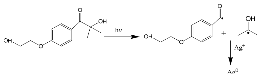
Figure 10 : Photo-cleavage mechanism of Iragure 2959 chromophore and reduction of silver cations [100].
