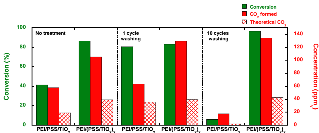
Figure 109 : Photocatalytic performances of functionalised textiles before and after 1 and 10 cycles washing. Experimental parameters: [HCOOH] = 45 ppm v , air flow = 20 mL/min, speed = 0.7 cm/s, UV-A irradiance = 2.5 mW/cm 2 , films built on polyester textile.
