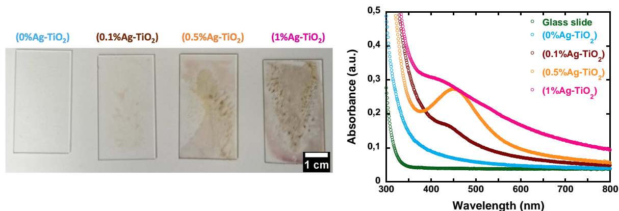
Figure 77: Characterisations of photoinduced AgNP synthesised on glass slide with TiO 2 -based x%AgNO 3 -TiO 2 photosensitive suspensions, containing different amounts of AgNO 3 . (Left) Pictures of the photosensitive suspensions on glass slides after UV irradiation. (Right) Corresponding transmission mode UV-Visible spectra.
