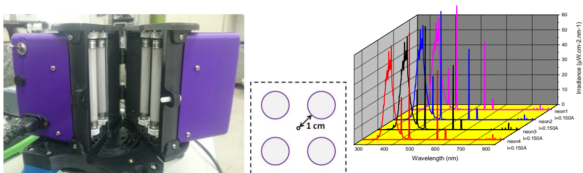
Figure 32: (Left) photo of irradiation box when being open. (Middle) schematic of a cross section viewed from the top of the closed irradiation box. The quartz cavity is located in the middle of the box with 4 UV-A lamps with a distance of 1 cm. (Right), the irradiance spectra of the 4 UV-A lamps used for illumination of functionalised capillaries.
