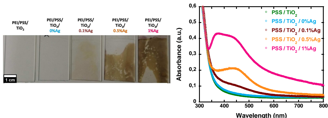
Figure 72: Classical photoinduced AgNP synthesis on PEI/PSS/ \text{TiO}_2 films on glass slides (left) and the UV-Visible characterisation of PEI/PSS/ \text{TiO}_2 /x%Ag films in transmission mode (right).
