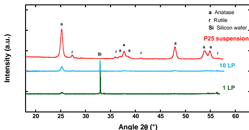
Figure 41 : XRD analysis of titania and polyelectrolytes LbL films.
