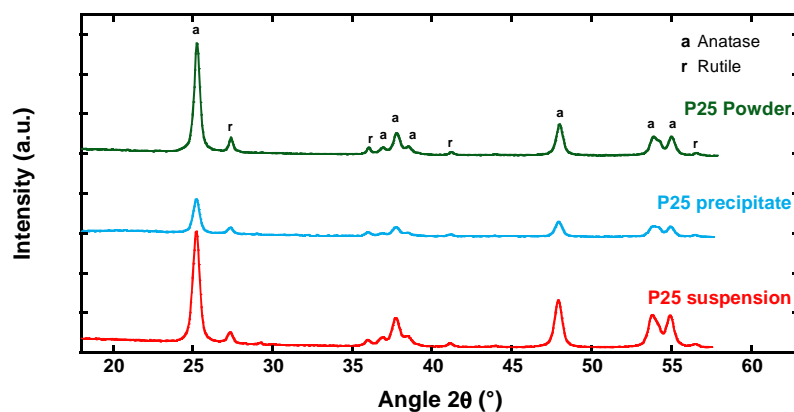
Figure 39 : XRD analysis of TiO 2 P25 as powder, precipitate and from the LbL suspension. a and r correspond to peak associated to anatase and rutile phase respectively.
