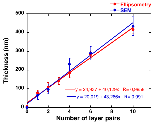
Figure 48 : Increase in thickness of PEI/(PSS/TiO 2 ) n LbL films obtained by ellipsometry and SEM characterisations.
