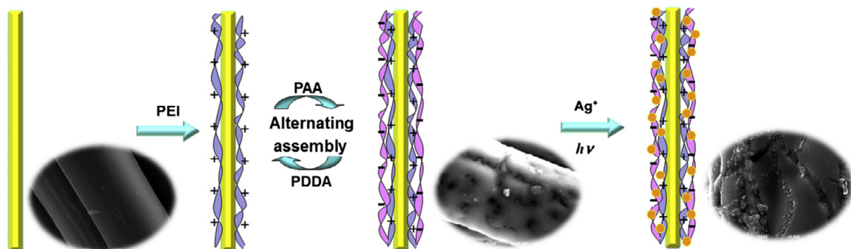
Figure 18: AgNP photoinduced synthesis on PEI/(PAA/PDDA) 8 LbL film constructed on silk fibers [193].
