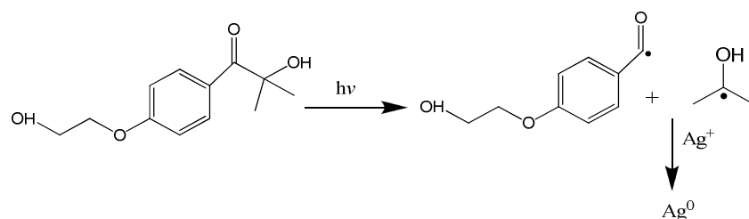
Figure 10 : Photo-cleavage mechanism of Irigure 2959 chromophore and reduction of silver cations [100].
