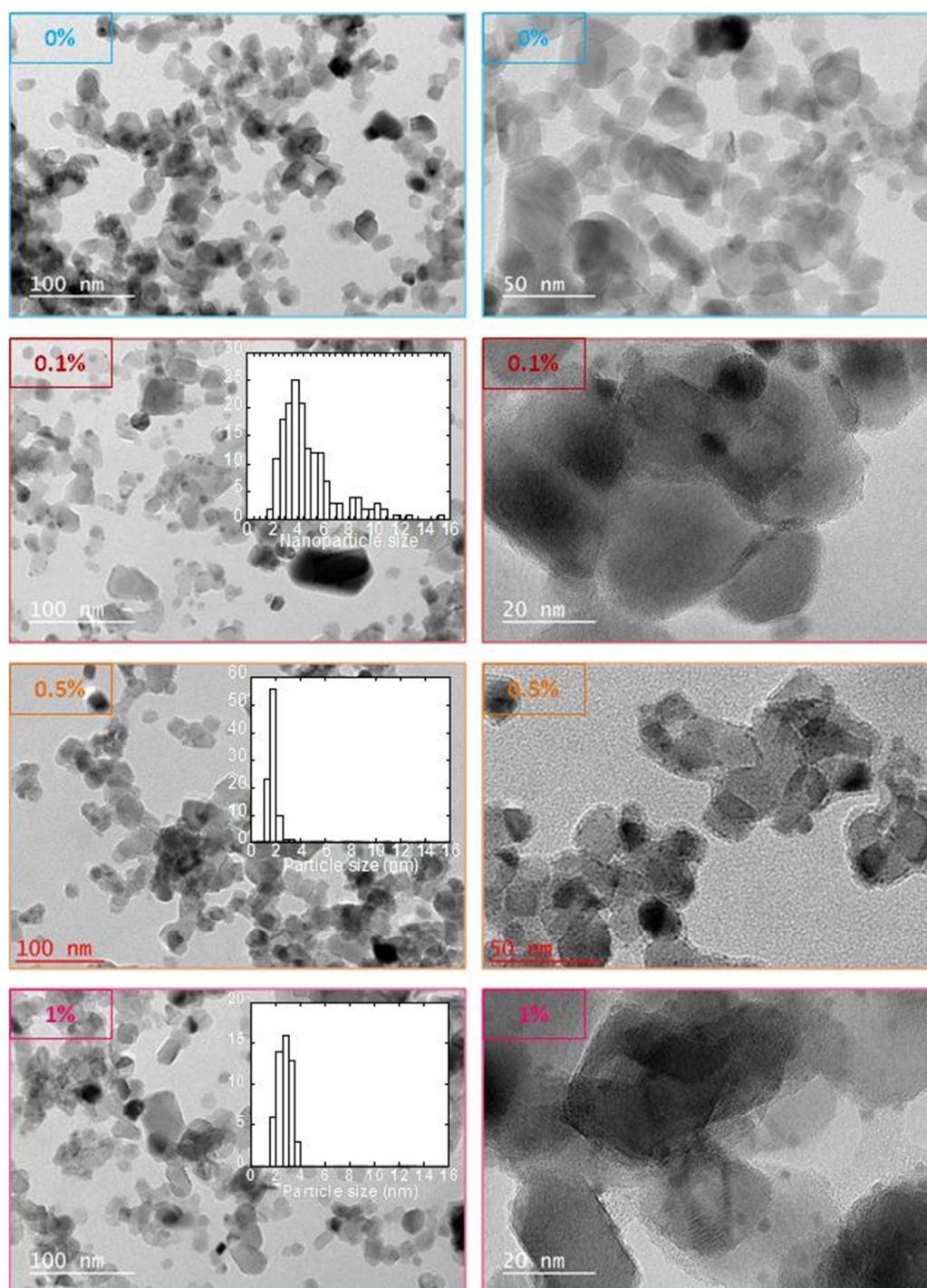
Figure 73 : TEM images of PEI/PSS/TiO 2 /x%Ag films. x = 0%, 0.1%, 0.5% and 1%. The size distribution was assessed only on 56 nanoparticles for the sample with x=1%.
