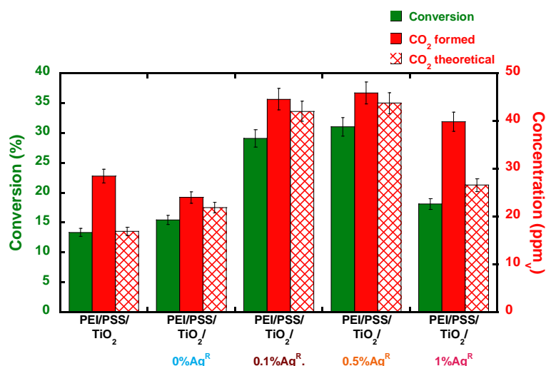
Figure 76: Photocatalytic performance of PEI/PSS/TiO 2 /x%Ag R films (with additional rinsing steps prior UV irradiation for AgNP photoinduced synthesis). Experimental parameters: [HCOOH] = 145 ppm v , air flow = 20 mL/min, speed = 0.7 cm/s, UV-A irradiance = 2.5 mW/cm 2 , films built on 36 cm 2 silicon wafers.
