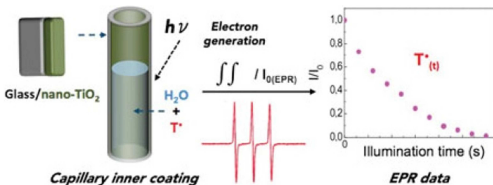
Figure 33 : Summary of EPR characterisations of LbL titania film constructed in capillary. Tempol (T•) solution is introduced in the functionalised capillary and EPR signal is acquired after each UV-A irradiation (hv). Double integrate is applied on the first EPR spectra peak to calculate intensity, and is normalised in regards to initial intensity. Normalised intensity values are reported afterwards in regards to illumination time [207].
