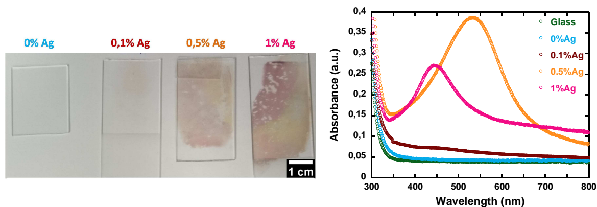
Figure 71 : Characterisations of photoinduced AgNP synthesised with photosensitive formulation containing different amounts of \text{AgNO}_3 . (Left) Pictures of irradiated photosensitive formulations deposited on glass slides. (Right) UV-Visible spectroscopy characterisation of photoinduced AgNP, in transmission mode. Photosensitive formulations: x wt.% \text{AgNO}_3 , 0,5 wt.% Irgacure and water (100 wt.%).
