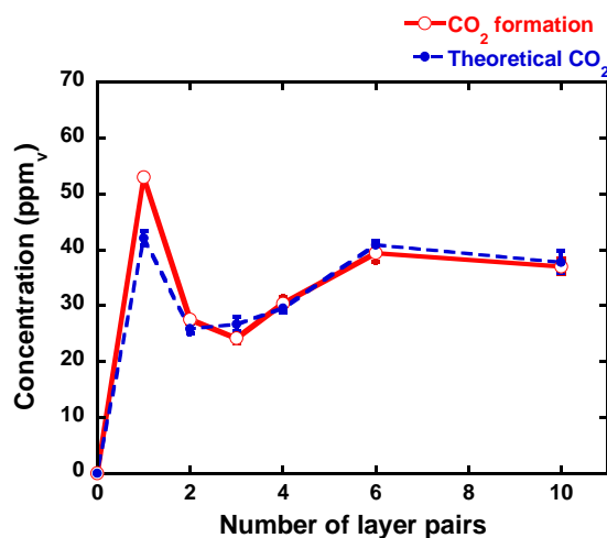
Figure 53: CO 2 formation on TiO 2 LbL films in regards to number of layer pairs during photocatalysis test with formic acid.
