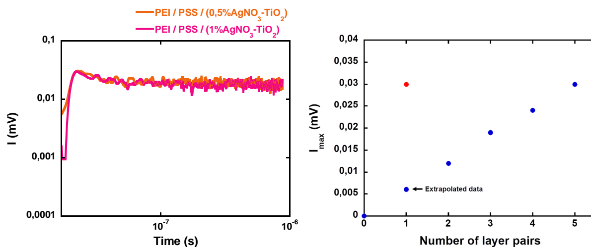
Figure 89: (Left) TRMC characterisations of PEI/PSS/(0.5%Ag-TiO 2 ) and PEI/PSS/(1%Ag-TiO 2 ) films. (Right) I_{\max} values for the PEI/(PSS/TiO 2 ) n films (●) and Ag-TiO 2 hybrid film I_{\max} value (●).
