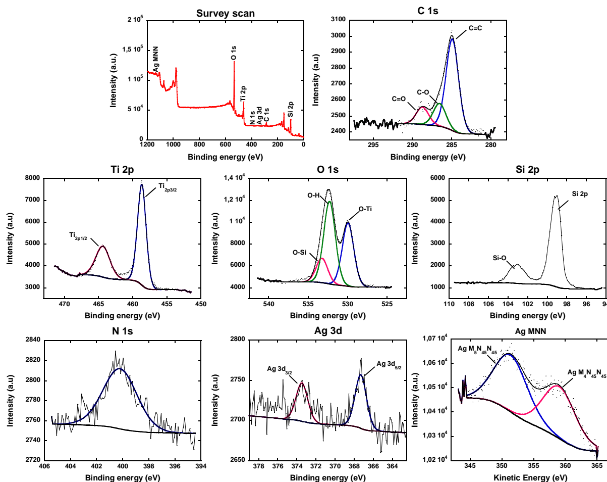
Figure 82: XPS characterisations of PEI/PSS/(0.2%Ag-TiO 2 ) LbL film
