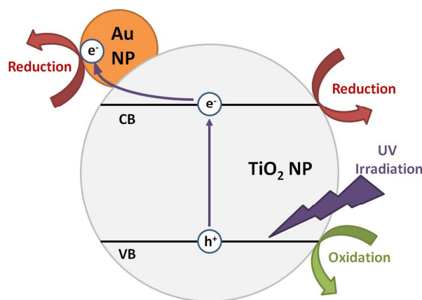
Figure 9: Association of \text{TiO}_2 with gold nanoparticles (AuNP) which act as an electron trap once \text{TiO}_2 is irradiated by UV light. The figure is based on schematic of Friehs et al. [93].
