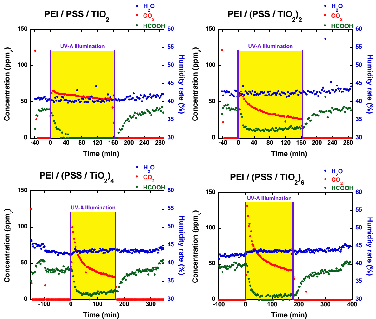
Appendix 6: Evolution of CO 2 and HCOOH concentration curve of LbL film under UV-A illumination.
