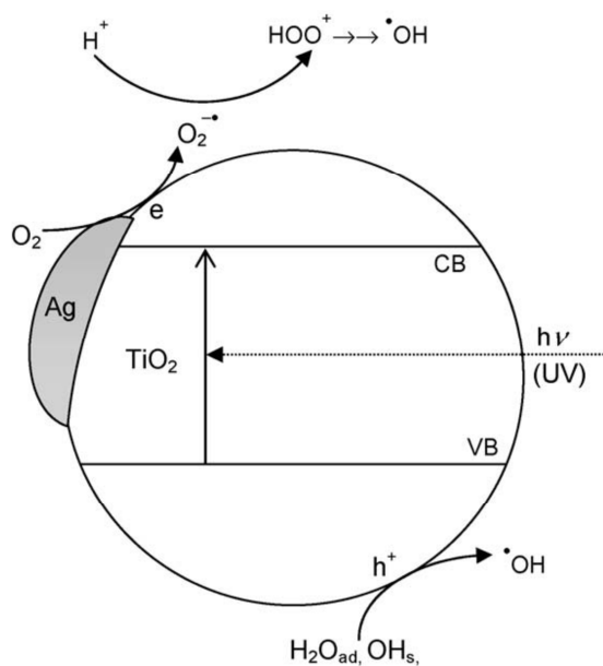
Figure 13: Photocatalytic pathway of TiO 2 -silver nanocomposite under UV-irradiation [130].
