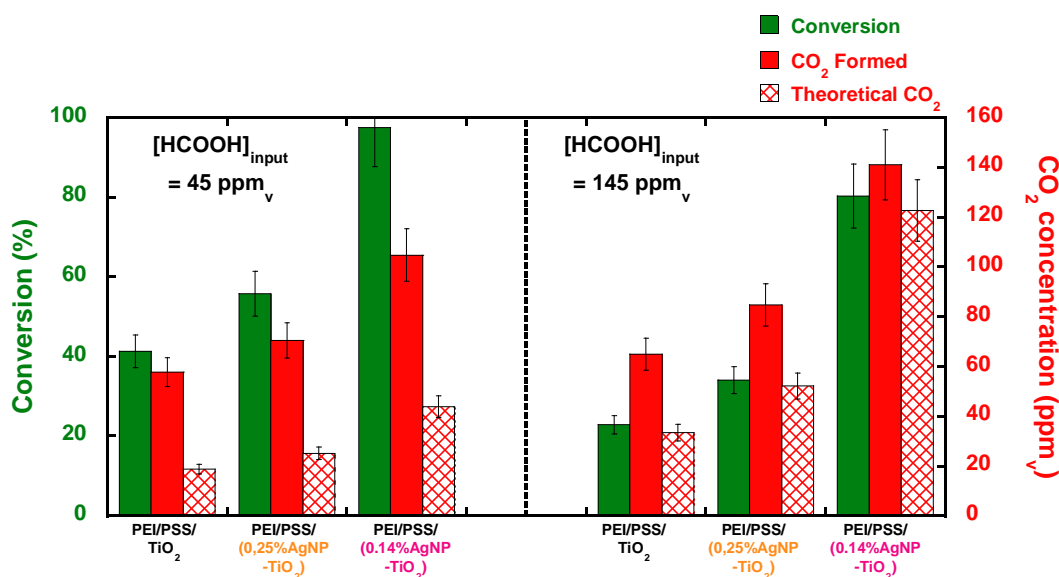
Figure 99 : Comparison of photocatalytic results of PEI/PSS/(AgNP-TiO 2 ) films obtained at different input HCOOH concentrations. Experimental parameters: [HCOOH] = (left) 45 and (right) 145 ppm v , air flow = 20 mL/min, speed = 0.7 cm/s, UV-A irradiance = 2.5 mW/cm 2 , films built on polyester textile.
