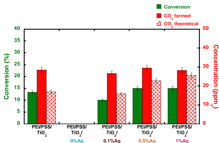
Figure 75 : Photocatalytic performance of PEI/PSS/TiO 2 /x%Ag films towards the degradation of gas phase HCOOH. Experimental parameters: [HCOOH] = 145 ppm v , air flow = 20 mL/min, speed = 0.7 cm/s, UV-A irradiance = 2.5 mW/cm 2 , films built on 36 cm 2 silicon wafers.
