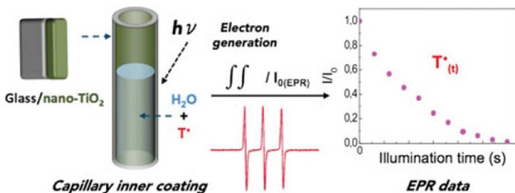
Figure 33 : Summary of EPR characterisations of LbL titania film constructed in capillary. Tempol ( T^\bullet ) solution is introduced in the functionalised capillary and EPR signal is acquired after each UV-A irradiation ( h\nu ). Double integrate is applied on the first EPR spectra peak to calculate intensity, and is normalised in regards to initial intensity. Normalised intensity values are reported afterwards in regards to illumination time [207].
