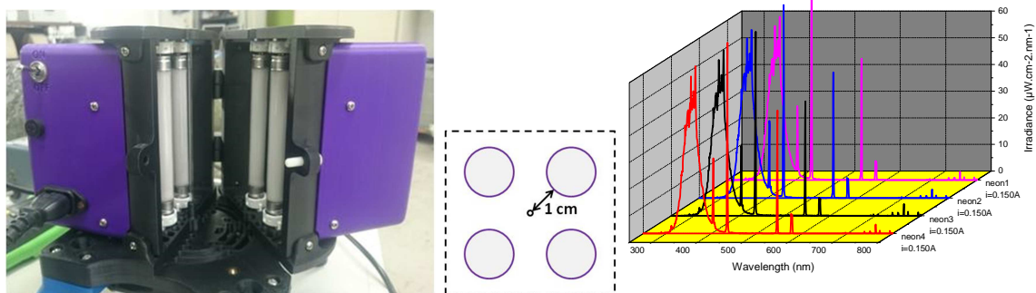
Figure 32: (Left) photo of irradiation box when being open. (Middle) schematic of a cross section viewed from the top of the closed irradiation box. The quartz cavity is located in the middle of the box with 4 UV-A lamps with a distance of 1 cm. (Right), the irradiance spectra of the 4 UV-A lamps used for illumination of functionalised capillaries.
