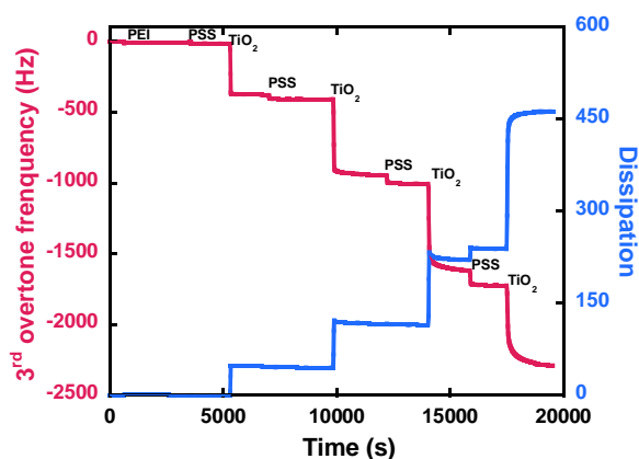
Figure 45: Monitoring PEI/(PSS/TiO 2 ) n film construction by QCM-D at the 3 rd overtone. 4 PSS/TiO 2 layer pairs were deposited.
