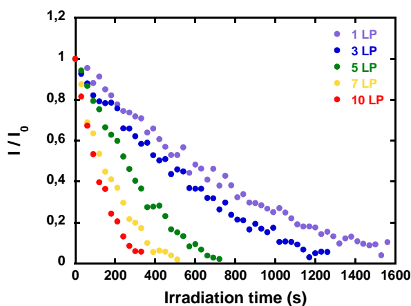
Figure 58: Tempol spin-scavenging by PEI/(PSS/TiO 2 ) n films, monitored by EPR.
