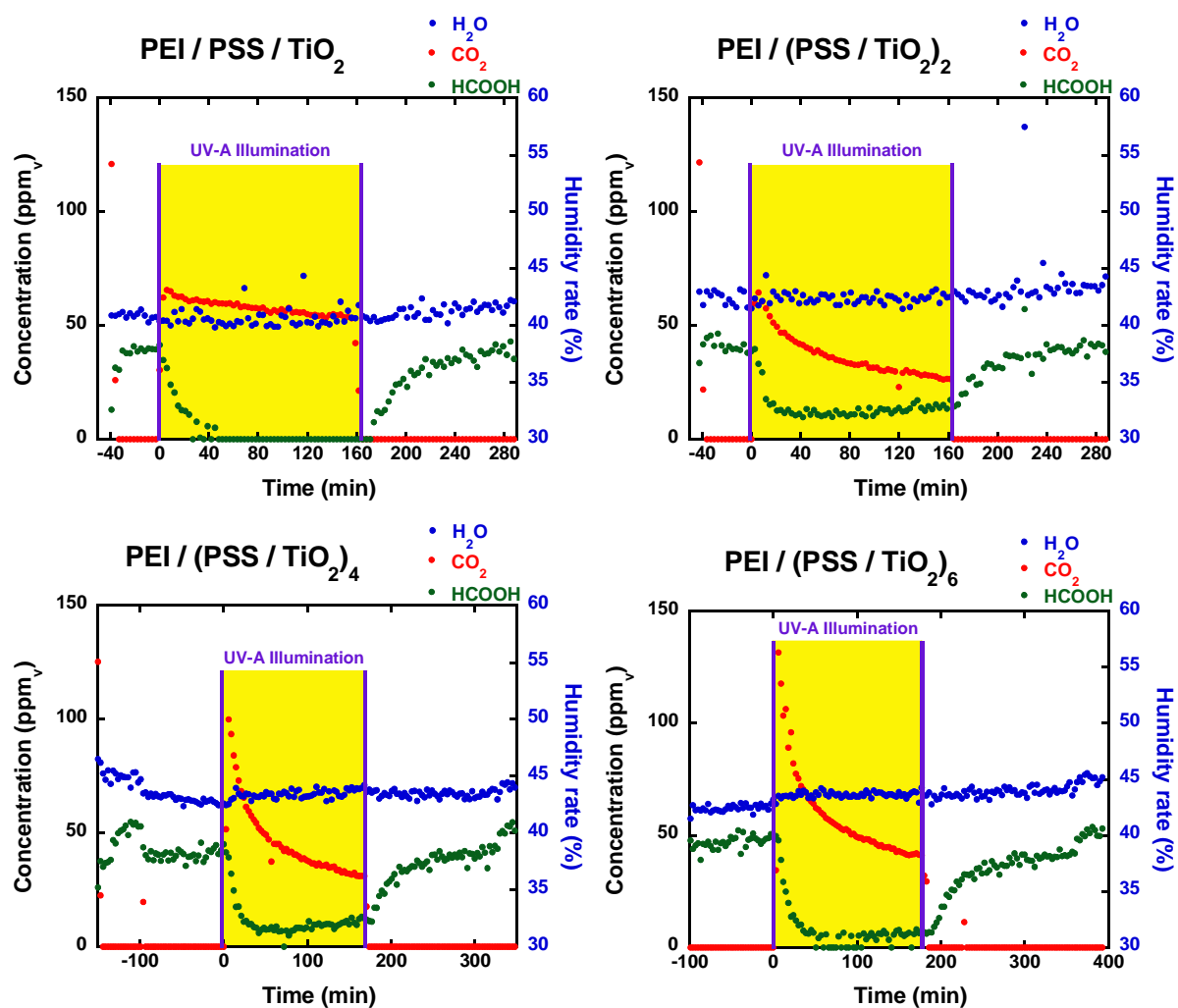
Appendix 6: Evolution of \text{CO}_2 and \text{HCOOH} concentration curve of LbL film under UV-A illumination.
