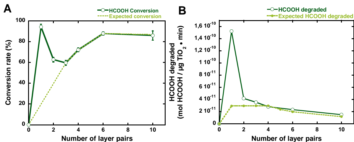
Figure 52: (A) Evolution of HCOOH conversion in regards to the number of layer pairs deposited in LbL films. (B) HCOOH degraded in mol per μg of TiO 2 per min in regards to the number of layer pairs. Experimental parameters: [HCOOH] = 45 ppm v , air flow = 20 mL/min, speed = 0.7 cm/s, UV-A irradiance = 2.5 mW/cm 2 , films built on 36 cm 2 silicon wafers.
