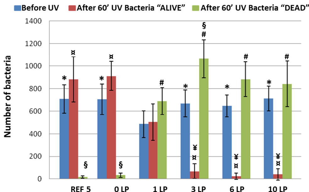
Figure 65: Bacteria assay on \text{PEI}/(\text{PSS}/\text{TiO}_2)_n films, with REF 5 and 0LP used as control samples. Tested bacteria: Escherichia Coli , UV-A irradiance = 2.5 \text{ mW}/\text{cm}^2 , irradiation time = 60 min, films built on 2 \text{ cm}^2 silicon wafers. (*) significantly different than 1 LP before UV ( p -value < 0.05); (α) significantly different than 1 LP after UV (ALIVE) ( p -value < 0.05); (¥) significantly different than 0 LP, 1 LP and REF 5 after UV (ALIVE) ( p -value < 0.05); (#) significantly different than 0 LP after UV (DEAD) ( p -value < 0.05); (§) significantly different than 1 LP after UV (DEAD) ( p -value < 0.05).
