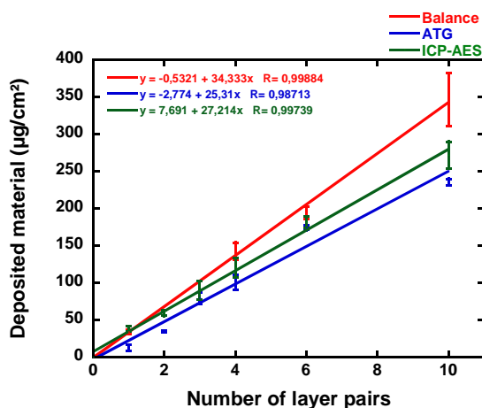
Figure 95 : Comparison of the amount of deposited material on textile surface using different characterisation methods.
