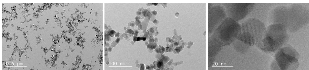
Figure 49: TEM images of a PEI/PSS/TiO 2 LbL film (single layer pair).
