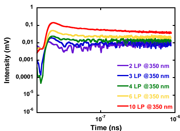
Figure 56: TRMC characterisations of PEI/(PSS/TiO 2 ) n films.
