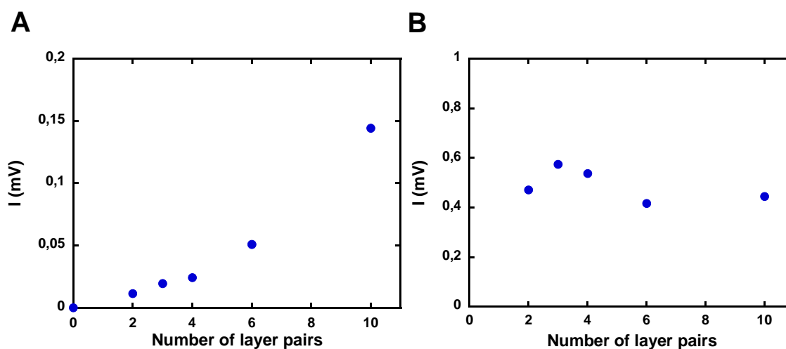
Figure 57: Information on charge carriers in regards to number of layer pairs deposited. A: I_{\max} ; B: I_{40}/I_{\max} .
