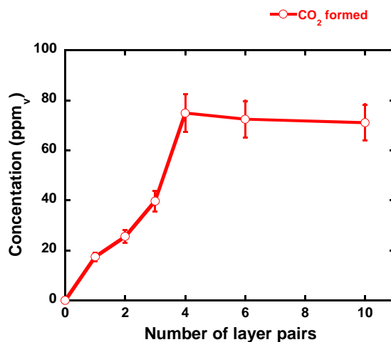
Figure 98 : Evolution of CO 2 formation UV-A irradiation, in the absence of HCOOH, in regards to the number of layer pairs deposited on textile surfaces. Experimental parameters: [HCOOH] = 0 ppm v , air flow = 20 mL/min, speed = 0.7 cm/s, UV-A irradiance = 2.5 mW/cm 2 , films built on polyester textile.
