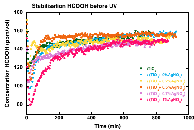
Appendix 9 : Stabilisation of PEI/PSS/(x%Ag-TiO 2 ) samples prior UV-A irradiation of the films. Experimental parameters: [HCOOH] = 145 ppm v , air flow = 20 mL/min, speed = 0.7 cm/s, UV-A irradiance = 2.5 mW/cm 2 , films built on 36 cm 2 silicon wafers
