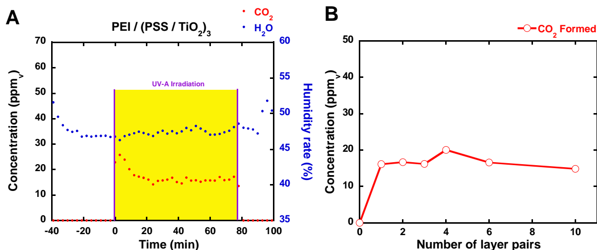
Figure 54: (A) Evolution of concentration curve for a 3 layer pairs LbL film; stabilisation is reached after 18 min. (B) Results of CO 2 concentration formed during UV-A irradiation in regards to the number of layer pairs deposited.
