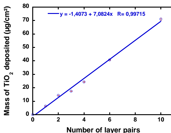
Figure 51: Mass of TiO 2 deposited investigated by chemical analysis ICP-AES. Error bars are too small to be clearly shown on the graph.
