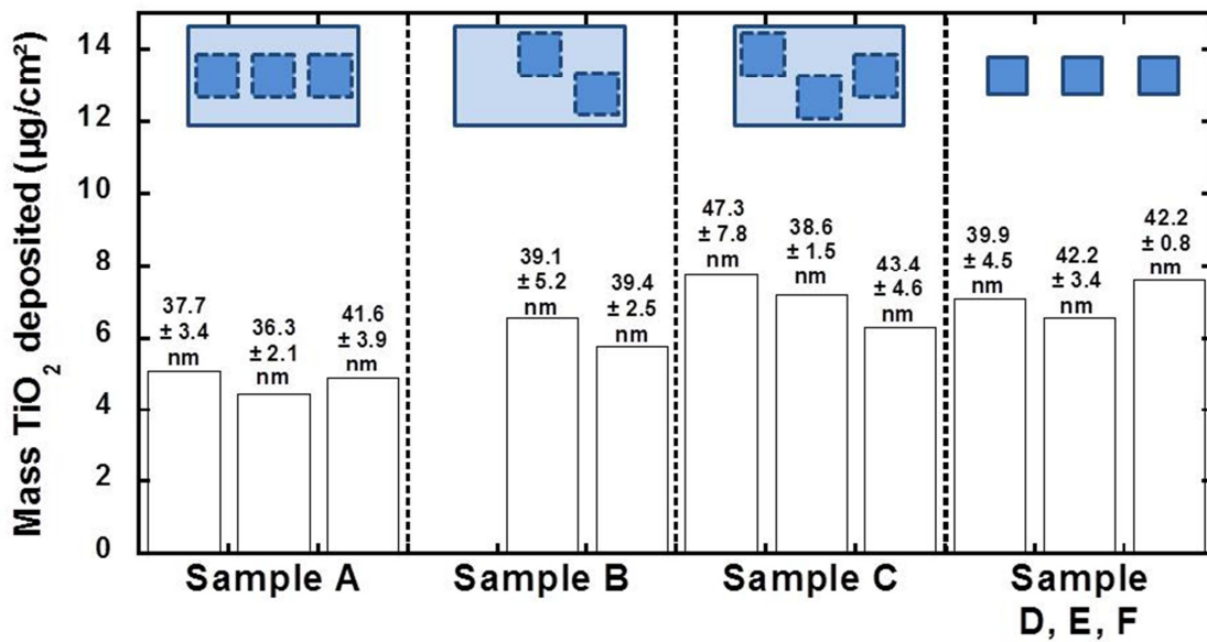
Appendix 4 : Amount of TiO 2 deposited in single layer pair films investigated by ICP-AES. Blue rectangles above every set of samples represent a 36 cm 2 silicon wafer and dash lines are the area where 4 cm 2 samples were cut for chemical analysis. Sample D, E and F were directly constructed on 4 cm 2 silicon wafer. Film thickness is reported above each histogram (measured by ellipsometry).
