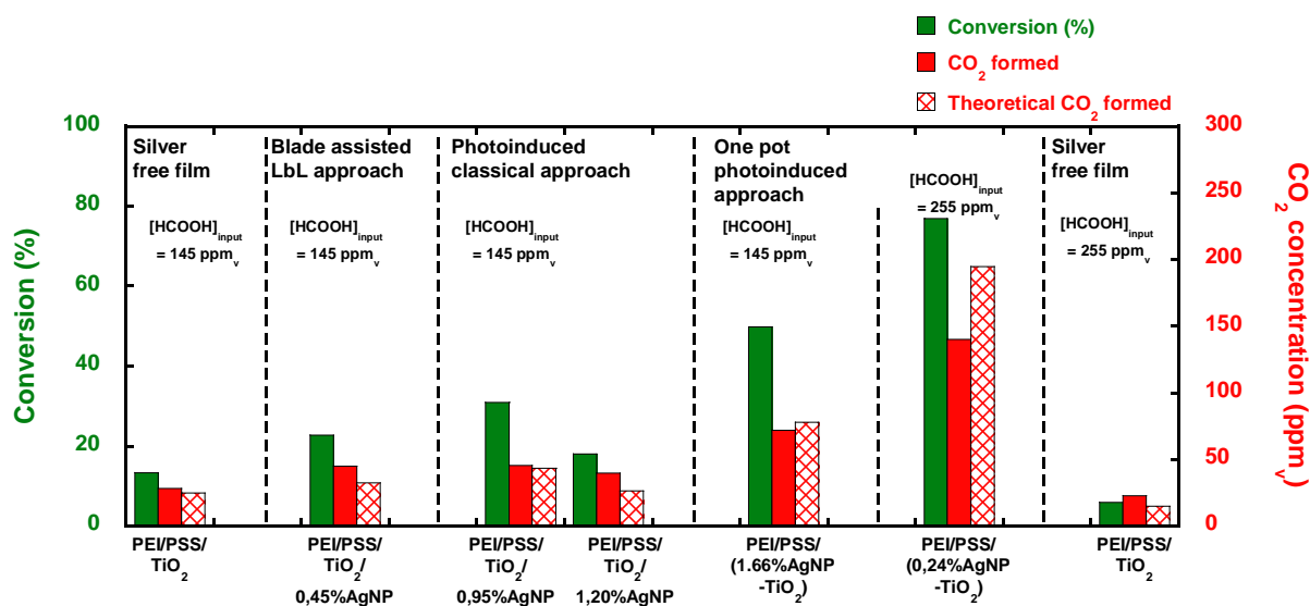
Figure 90: Comparison of the photocatalytic performances shown by Ag-TiO 2 films prepared via the three approaches.
