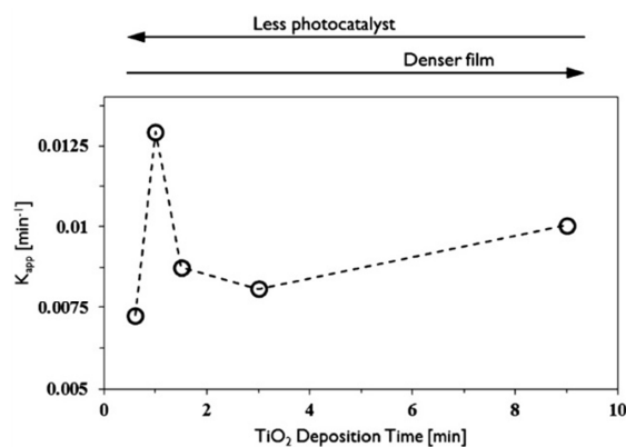
Figure 62: Methylene blue oxidation activity for LbL films with 5 layer pairs, prepared using different \text{TiO}_2 deposition times [149].
