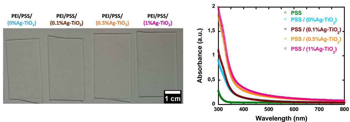
Figure 79 : Characterisations of PEI/PSS/(x%Ag-TiO 2 ) film, with x = 0, 0.1, 0.5 and 1wt% AgNO 3 . (Left) Pictures of irradiated films constructed on glass slides. (Right) Transmission mode UV-Visible spectra of the films after being UV irradiated for AgNP one-pot synthesis.
