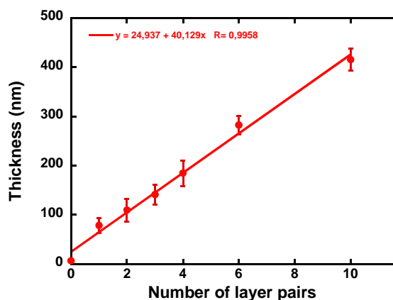
Figure 43: Ellipsometry characterisation of PEI/(PSS/TiO 2 ) n films. A linear increase in thickness is observed after deposition of each PSS/TiO 2 layer pair.
