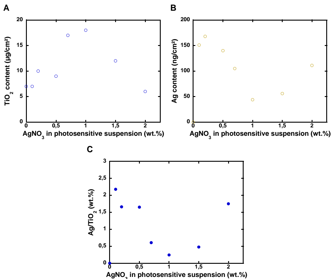
Figure 80 : (A) \text{TiO}_2 and (B) Ag content in regards to the \text{AgNO}_3 concentration in the \text{TiO}_2 photosensitive suspension. (C) Ag/ \text{TiO}_2 wt.% in Ag- \text{TiO}_2 hybrid films in regards to the \text{AgNO}_3 concentration in \text{TiO}_2 photosensitive suspension.
