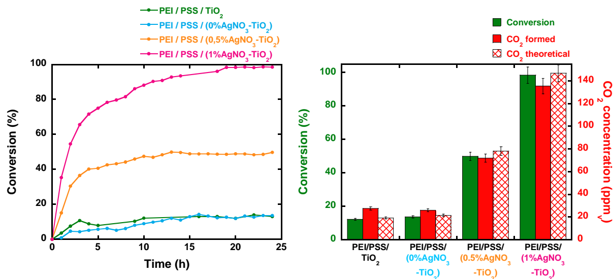
Figure 85 : (Left) Evolution of gas-phase HCOOH conversion during UV-A irradiation of PEI/PSS/(x%Ag-TiO 2 ) films. (Right) Photocatalytic performance of PEI/PSS/(x%Ag-TiO 2 ) films. Experimental parameters: [HCOOH] = 145 ppm v , air flow = 20 mL/min, speed = 0.7 cm/s, UV-A irradiance = 2.5 mW/cm 2 , films built on 36 cm 2 silicon wafers.
