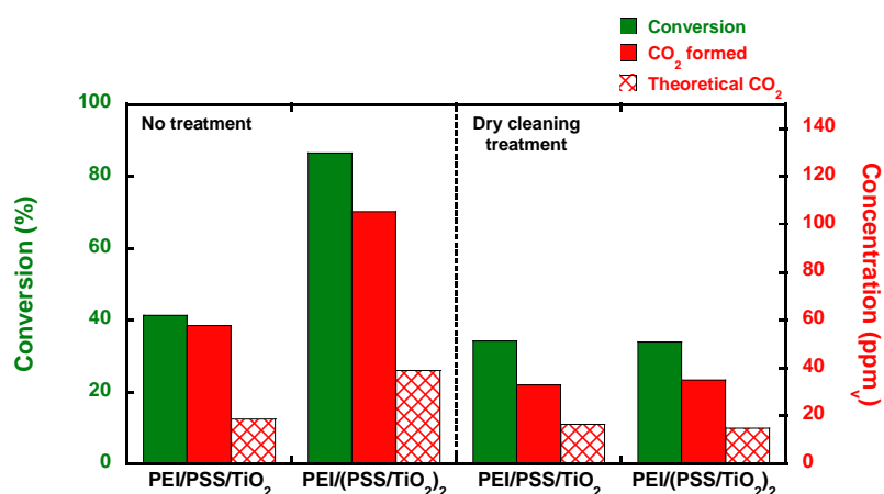
Figure 112 : Photocatalytic performances of functionalised textiles before and after dry cleaning treatment. Experimental parameters: [HCOOH] = 45 ppm v , air flow = 20 mL/min, speed = 0.7 cm/s, UV-A irradiance = 2.5 mW/cm 2 , films built on polyester textile.
