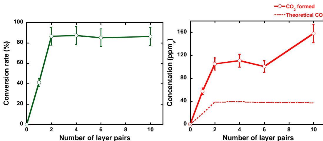
Figure 97 : (Left) Evolution of HCOOH conversion in regards to the number of layer pairs deposited in LbL films. (Right) Evolution of CO 2 formed upon irradiation of LbL films, in regards to the number of layer pairs. Experimental parameters: [HCOOH] = 45 ppm v , air flow = 20 mL/min, speed = 0.7 cm/s, UV-A irradiance = 2.5 mW/cm 2 , films built on polyester textile.
