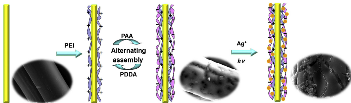
Figure 18: AgNP photoinduced synthesis on PEI/(PAA/PDDA) 8 LbL film constructed on silk fibers [193].
