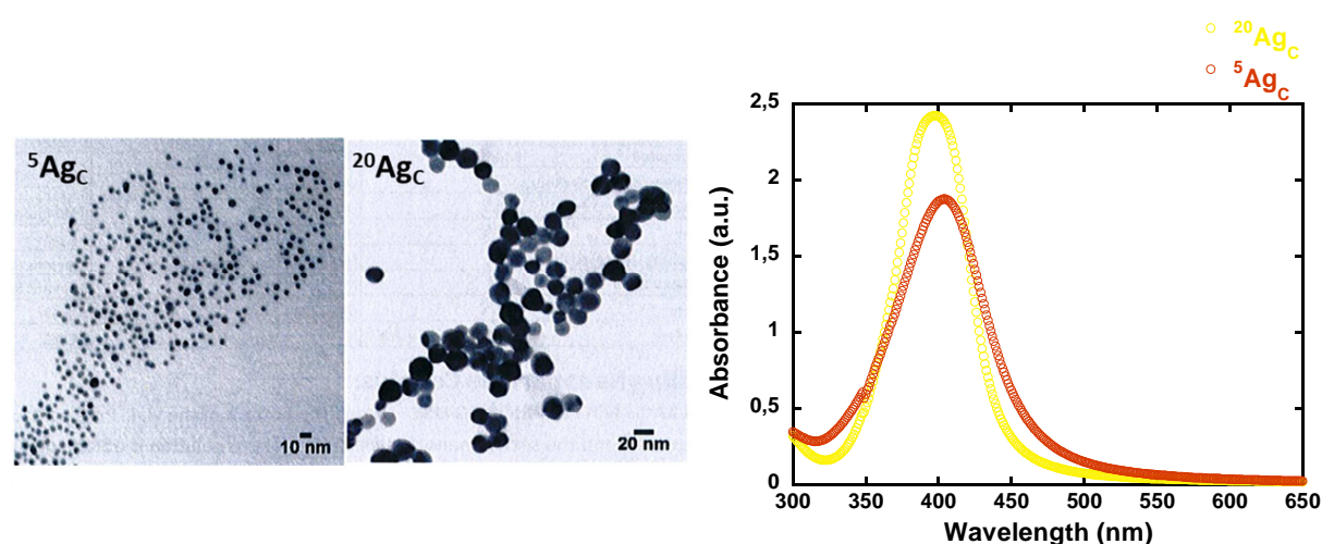
Figure 66: Characterisations of AgNP suspensions with TEM images taken from NanoXact (left), and UV-Visible spectroscopy in transmission (right).
