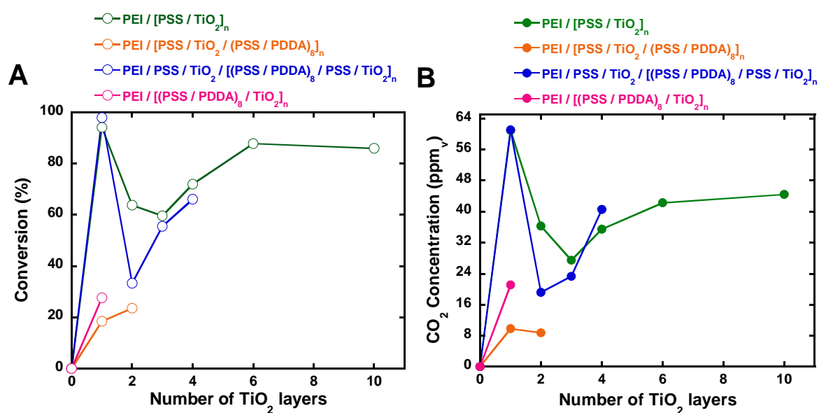
Figure 60 : Degradation of gas-phase HCOOH under UV-A light using LbL titania film with different types of architecture. (A) HCOOH conversion rate in regards of number of TiO 2 layers deposited; (B) CO 2 formation in regards of number of TiO 2 layers deposited. Experimental parameters: [HCOOH] = 45 ppm v , air flow = 20 mL/min, speed = 0.7 cm/s, UV-A irradiance = 2.5 mW/cm 2 , films built on 36 cm 2 silicon wafers.
