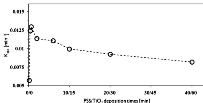
Figure 61: Methylene blue oxidation activity for LbL films with 5 layer pairs, prepared using different deposition times [149].
