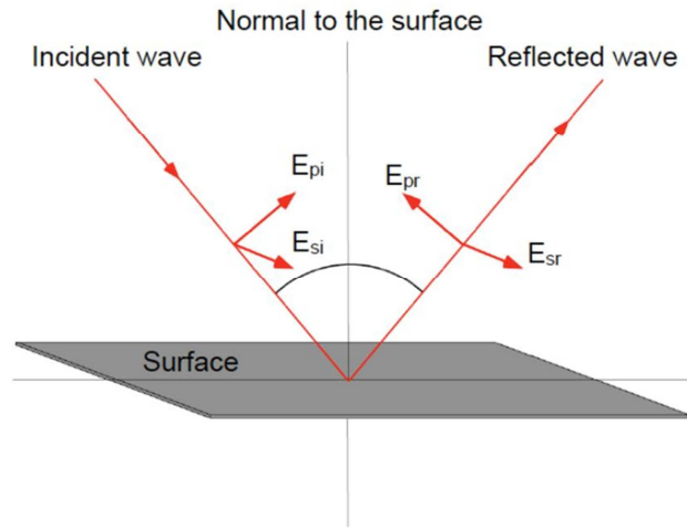
Figure 22: Schematic representation of an electromagnetic wave reflecting off a surface.
