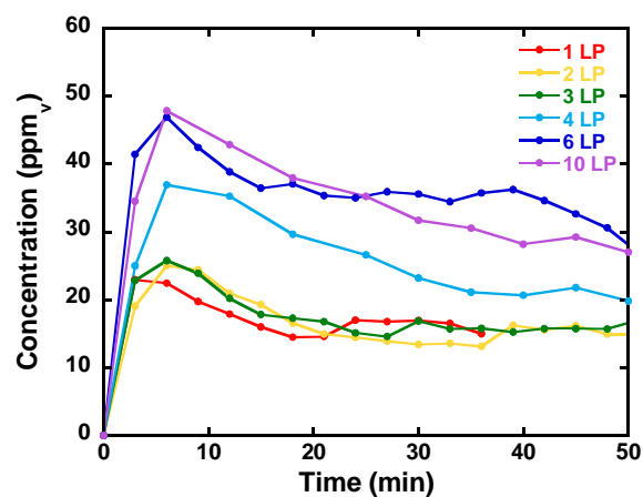
Appendix 5 : Evolution of \text{CO}_2 formation during photocatalysis tests without \text{HCOOH}
