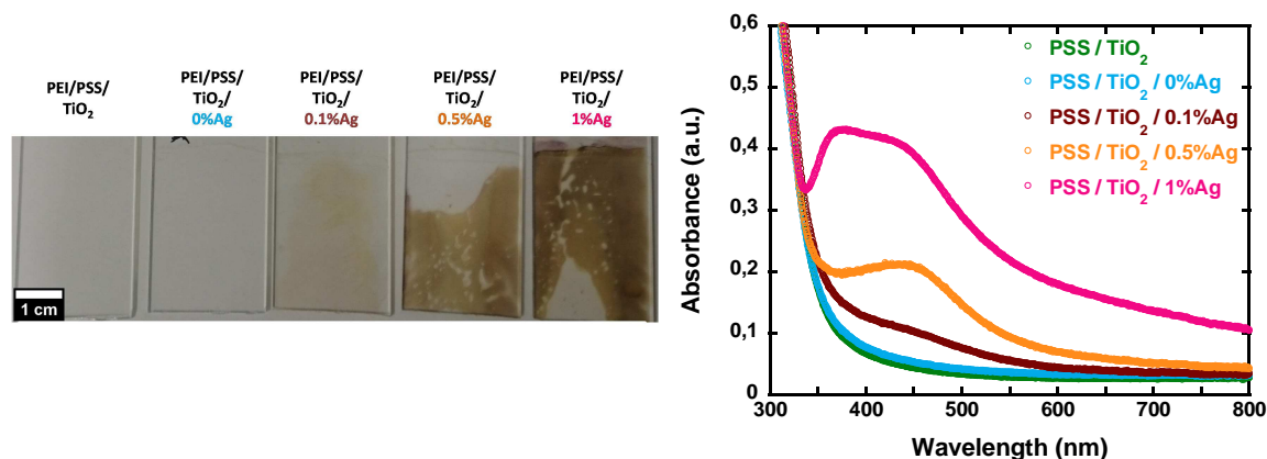
Figure 72: Classical photoinduced AgNP synthesis on PEI/PSS/TiO 2 films on glass slides (left) and the UV-Visible characterisation of PEI/PSS/TiO 2 /x%Ag films in transmission mode (right).
