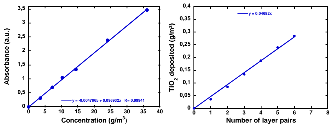
Figure 50: Amount of \text{TiO}_2 deposited per layer calculated from UV-Visible spectrophotometry data. Absorbance of \text{TiO}_2 suspension in regards to \text{TiO}_2 concentration (left); amount of \text{TiO}_2 deposited per layer pairs calculated from Dontsova's equation (right).
