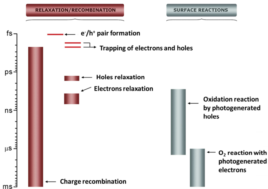
Figure 4: Time scale range of the main processes taking place in the irradiated semiconductor material. Schematic based on the diagram of Kubacka et al [61].
