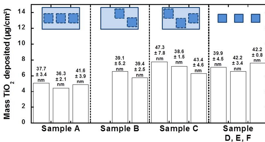
Appendix 4 : Amount of TiO 2 deposited in single layer pair films investigated by ICP-AES. Blue rectangles above every set of samples represent a 36 cm 2 silicon wafer and dash lines are the area where 4 cm 2 samples were cut for chemical analysis. Sample D, E and F were directly constructed on 4 cm 2 silicon wafer. Film thickness is reported above each histogram (measured by ellipsometry).
