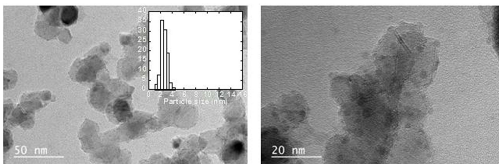
Figure 78 : TEM images of the Ag- \text{TiO}_2 system obtained after irradiation of the 0.5% \text{AgNO}_3\text{-TiO}_2 photosensitive suspension.
