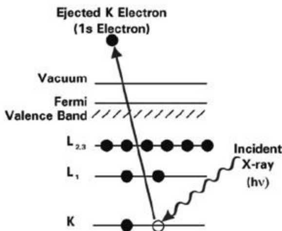
Figure 26 : Photoemission process involved during XPS surface analysis. Dark and white dots represent electrons and bars represent the energy levels within the analysed material.
