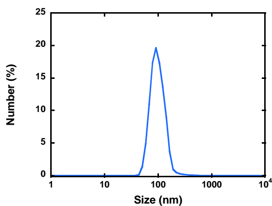
Figure 40 : Dynamic light scattering characterisation of the TiO 2 P25 suspension used for LbL films construction.
