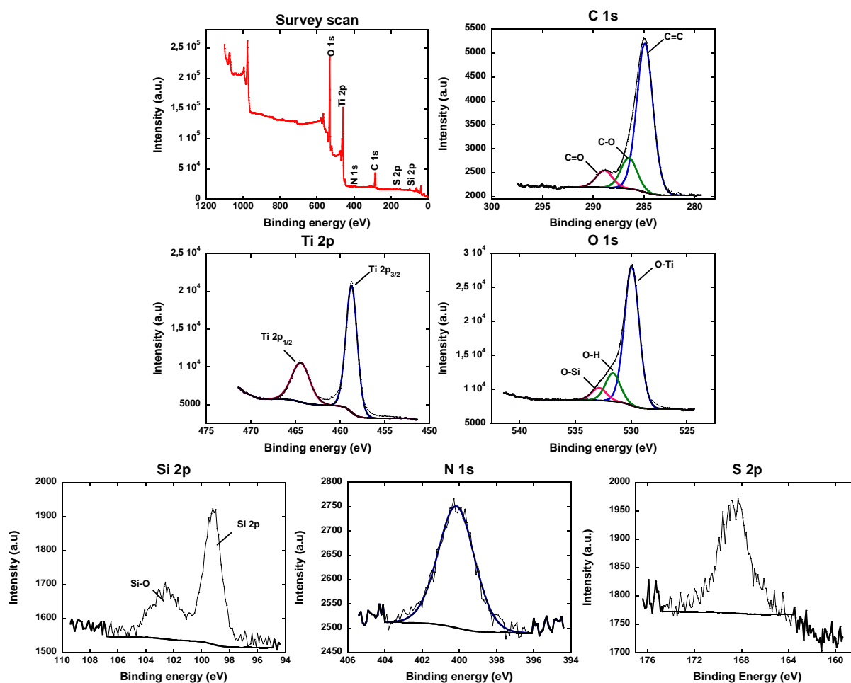
Figure 81 : XPS characterisation of the PEI/(PSS/TiO 2 ) 10 LbL film.
