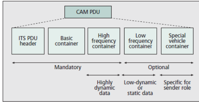
Figure 2.4: CAM structure (ETSI EN 302 637-2) [2, 3].
