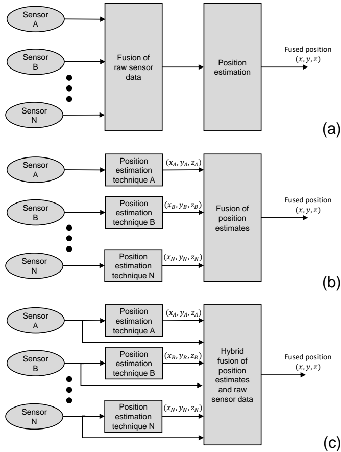
Figure D.1: Generic fusion architectures: (a) centralized (low-level), (b) autonomous (high-level), (c) hybrid (partial reproduction and simplification of [1]).
