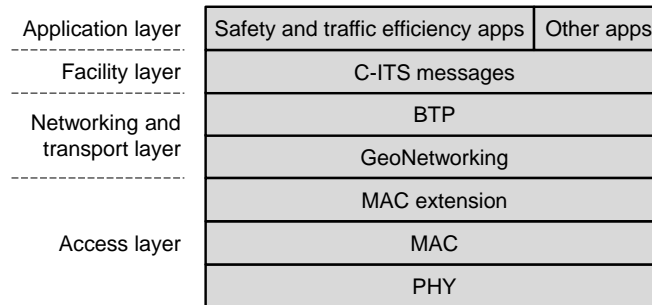
Figure 2.3: The C-ITS protocol stack (partial reproduction of [8, 10]).
