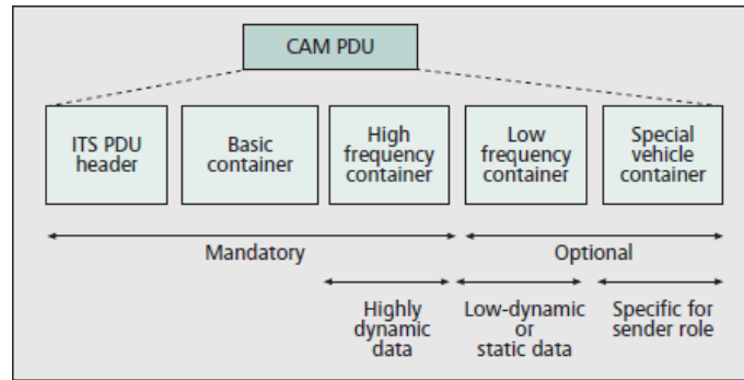
Figure 2.4: CAM structure (ETSI EN 302 637-2) [10, 21].
