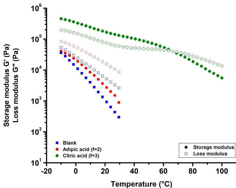
Figure 39. Evolution of the storage and loss modulus ( G' and G'' ) as a function of temperature for the films prepared from WNIPU4 and 100 mol. % of different functional carboxylic acids.
