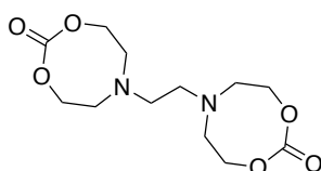
Scheme 15. Structure of the 8-membered cyclic carbonate bearing tertiary amines in its structure (bis-N-8-C).
