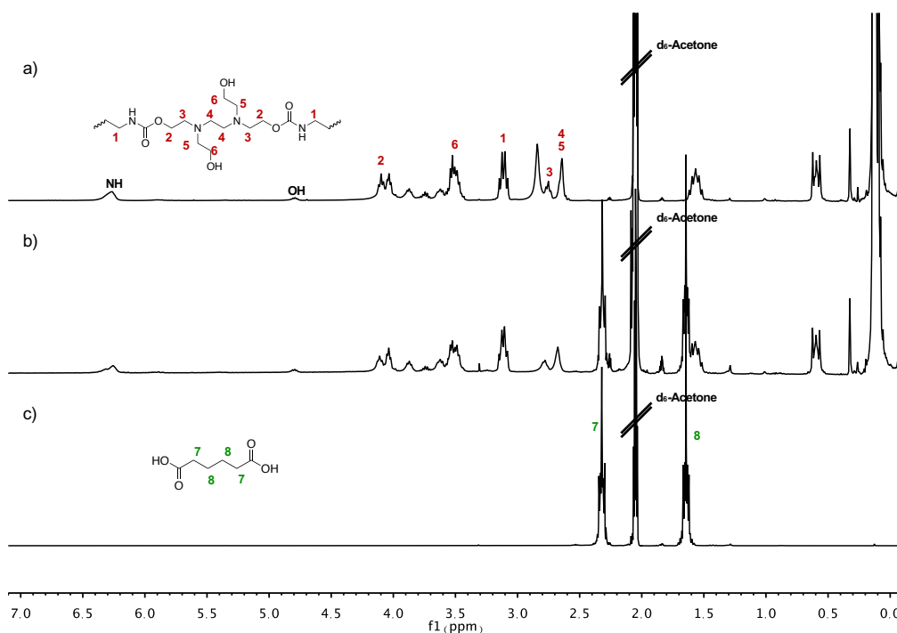
Figure S40. 1 H NMR (300 MHz, d 6 -acetone) of a) WNIPU4, b) WNIPU4/adipic acid film and c) adipic acid showing no proton shift associated with the formation of ionic hydrogen bonds.
