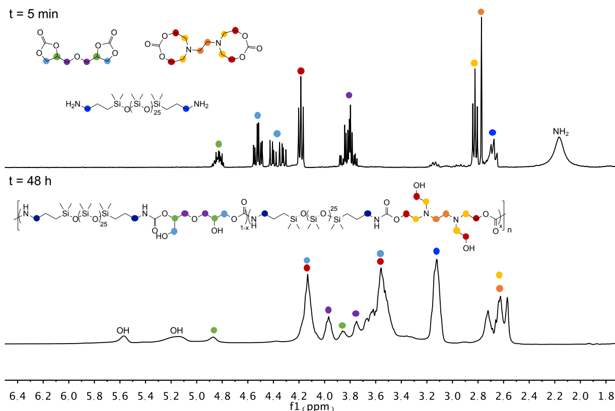
Figure 30. Expanded 1 H NMR (300 MHz, CDCl 3 ) of the poly(hydroxyurethane) based on DGC, bis-N-8-C and PDMS diamine after 5 min and 48 h. WNIPU4 (x = 0.3).
