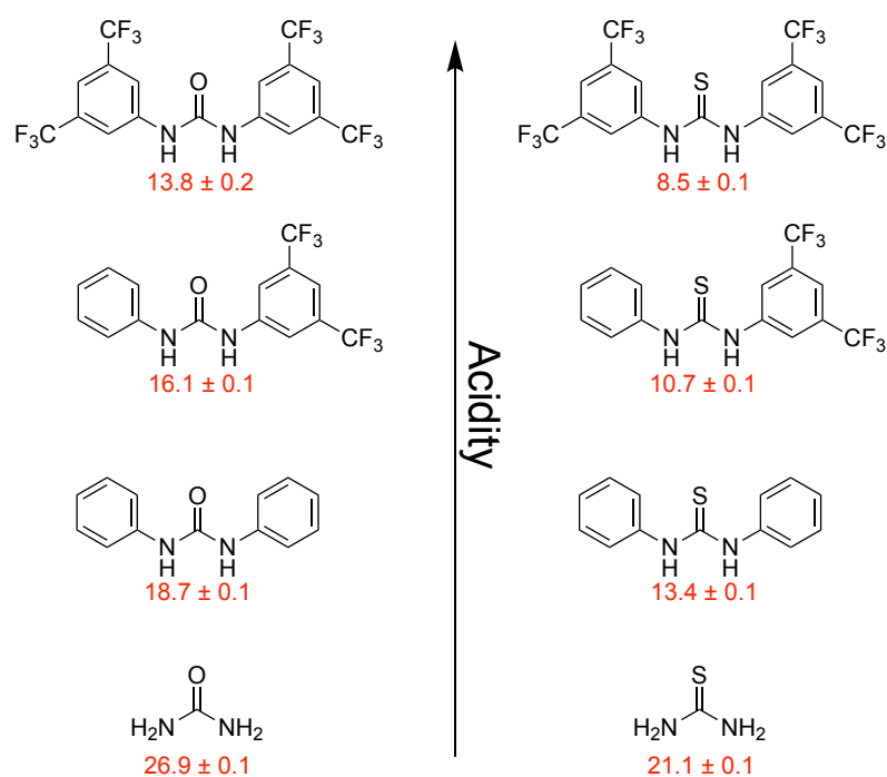
Figure 7. The effect of the 3,5-bis(trifluoromethyl)phenyl rings on the acidity of various ureas and thioureas. pKa values determined in DMSO; adapted from ref. 92
