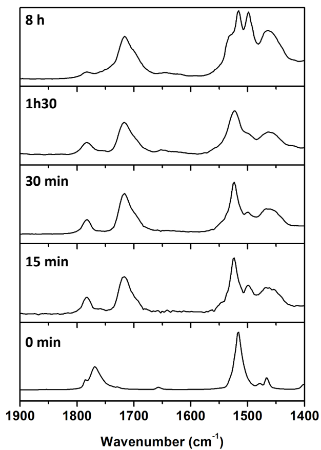
Figure S53. Scale expanded FTIR at different reaction times of the polymerization between Monomer A and PEG diamine in interfacial condition (80 % \text{H}_2\text{O} / 20 % DCM) as example.
