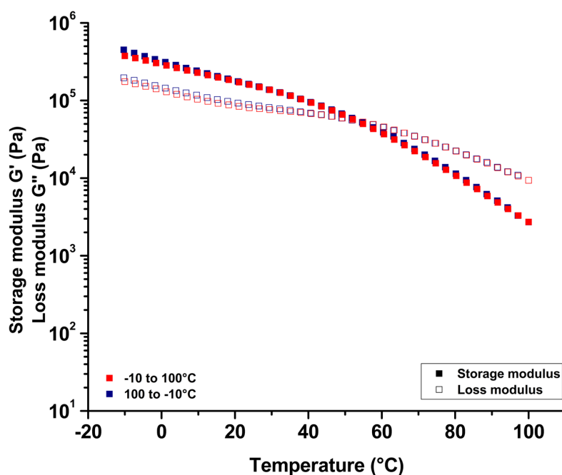
Figure 40. Evolution of the storage and the loss modulus ( G' and G'' ) in reverse temperature sweep between -10 and 100 ^{\circ}\text{C} of films prepared from WNIPU4 and citric acid.
