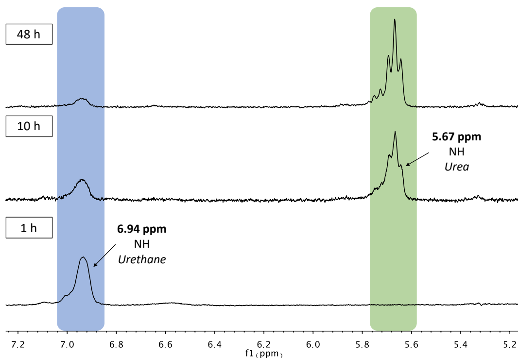
Figure 10. 1 H NMR (300 MHz, DMSO-d 6 ) in the area 5–7 ppm of the products obtained at different times from the step-growth polymerization of DGC with Jeffamine ED-2003 performed at 120 °C using TBD as catalyst showing the change in the shifts of the NH protons.
