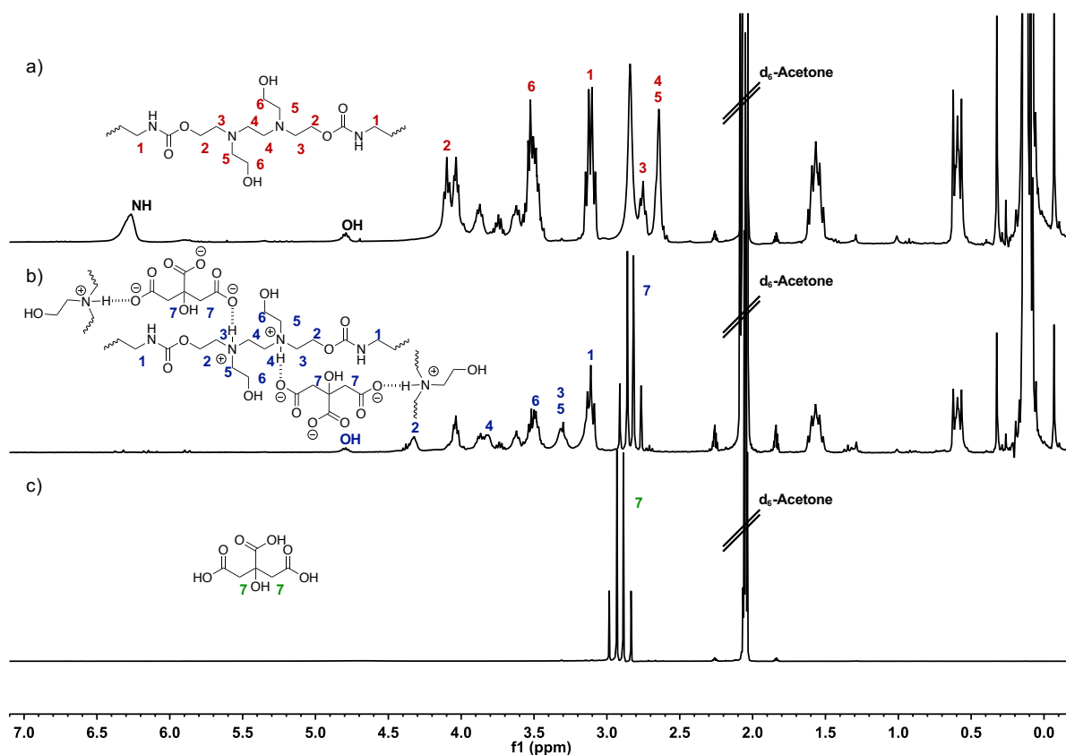
Figure 38. ^1\text{H} NMR (300 MHz, \text{d}_6 -acetone) of: a) WNIPU4; b) WNIPU4/citric acid film; c) citric acid showing the proton shift associated with the formation of ionic bonds.
