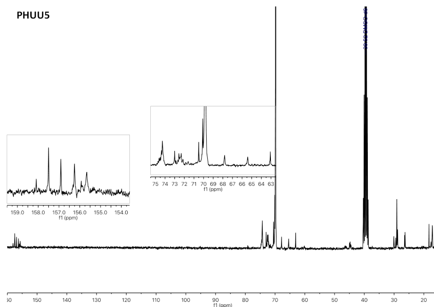
Figure S10. ^{13}\text{C} NMR of PHUU5 (75 MHz, \text{DMSO-d}_6 ) \delta (ppm) = 158.1, 157.5, 156.9 ( -\text{NH}-(\text{C}=\text{O})-\text{NH}- ), 156.3, 155.9, 155.7 ( -\text{NH}-(\text{C}=\text{O})-\text{O}- ), 74.7-74.0 (m), 73.0-71.6 (m), 70.5, 70.1, 67.8, 65.4, 63.1 ( \text{CH}_2\text{O} and \text{CHO} ), 46.5, 46.3, 46.2, 46.0, 44.9, 44.8, 44.7, 44.6, 44.5 ( \text{CH}_2\text{NH} ), 30.1, 29.4, 29.1, 28.9, 28.8, 26.5, 26.3, 18.3, 17.6, 17.2, 17.1 ( \text{CH}_3 ).
