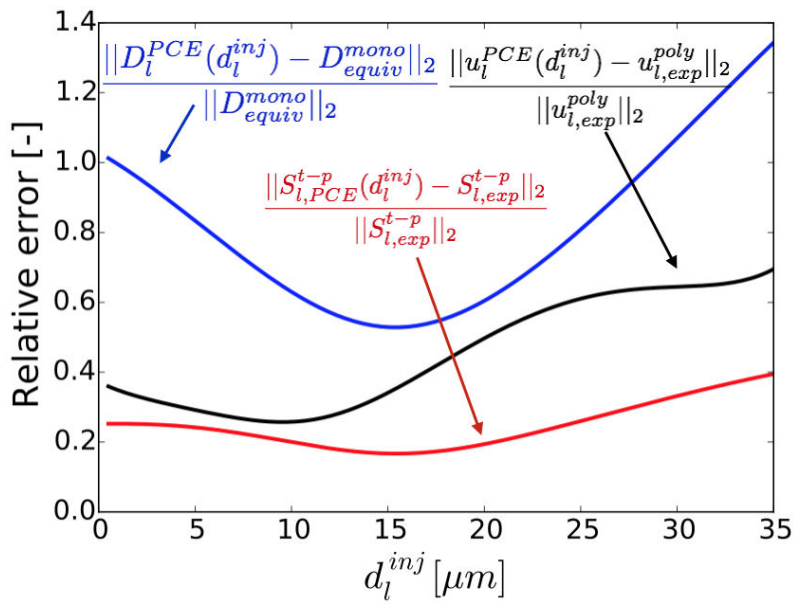
Figure 2.16: Normalised L^2 -norm of the different error criteria at x = 7.5 mm. Black curve: error on liquid axial velocity, blue curve: error on the liquid equivalent diameter and red curve: error on the two-phase laminar flame speed.
