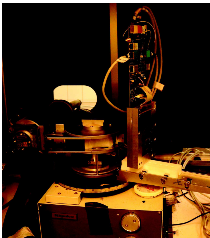
Figure 5.2: A PIPPER-2 proxy in its watercooled aluminum box coupled to its auxiliary board installed in the X-ray generator with a copper tube installed.
