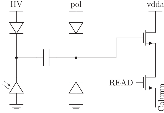
Figure 4.3: Schematic of the PIPPER-2 pixel. The substrate is biased from the top through a forward bias diode and the collecting diode. The collection node is AC-coupled to a source follower. A set of diodes after the coupling at the input of the amplifier is used to set the DC point.
