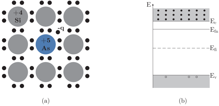
Figure 2.2: (a) Schematic two-dimensional representation of n-type silicon with its donor (arsenic). (b) Schematic of the energy bands structure of a n-type semiconductor
