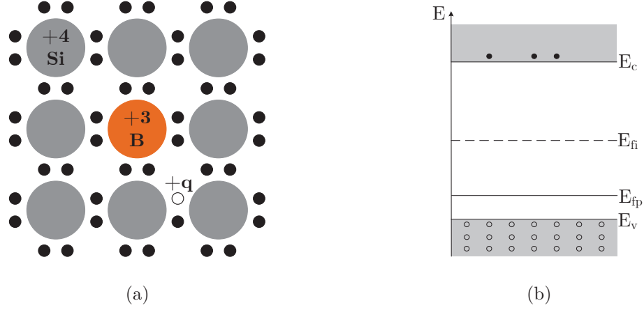
Figure 2.3: (a) Schematic two-dimensional representation of p-type silicon with its acceptor (boron). (b) Schematic of the energy bands structure of a p-type semiconductor
