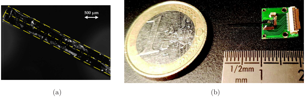
Figure 8.10: Two IMIC sensors each thinned to 250\ \mu\text{m} and glued back to back (8.10a). Picture by L. Ammour (IMNC). The double sided probe wirebonded on each side of its PCB and protected by globtop coating (8.10b). Picture by F. Gensolen (CPPM).
