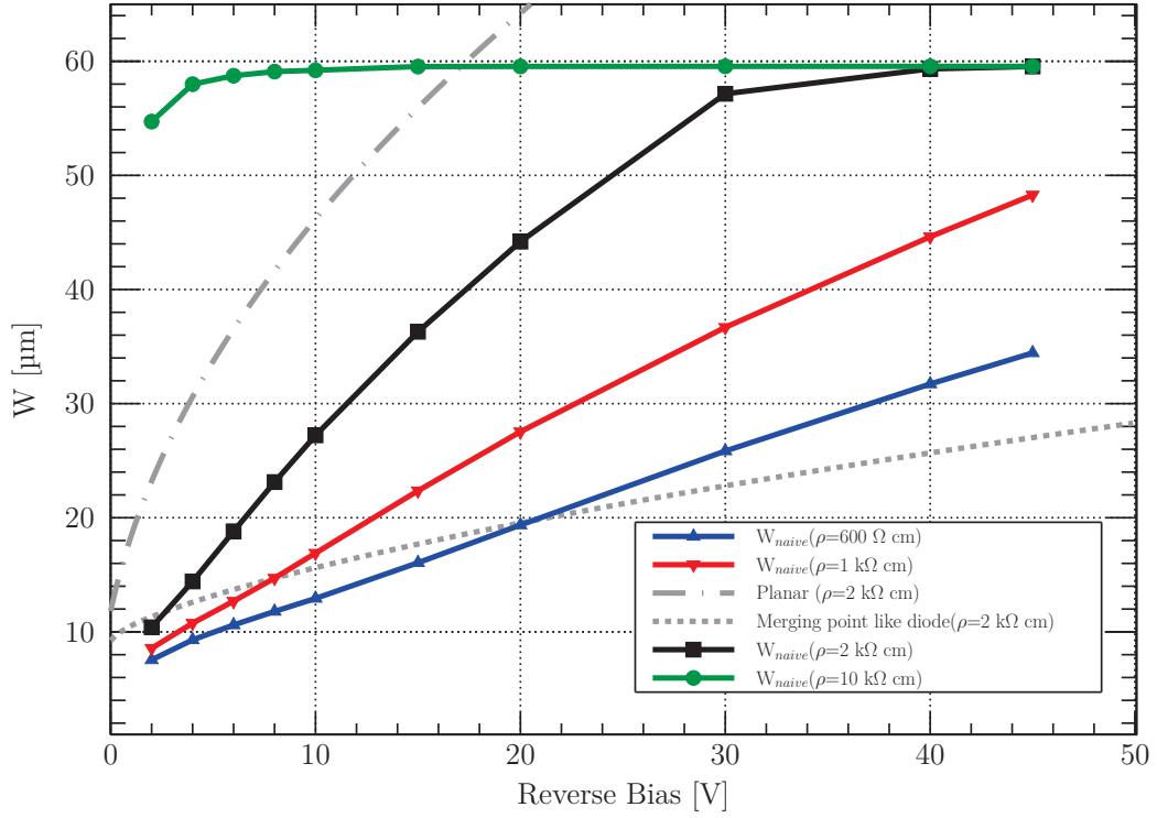
Figure 4.14: TCAD simulated depletion depth reached in a simplified PIPPER-2 structure at various resistivities: 600 \Omega \text{ cm} , 1 \text{k}\Omega \text{ cm} , 2 \text{k}\Omega \text{ cm} , and >10 \text{ k}\Omega \text{ cm} compared to the depth calculated for a 2 \text{k}\Omega \text{ cm} with the planar equation (equation 2.52) and with the merging point like-diode equation (equation 4.19).
