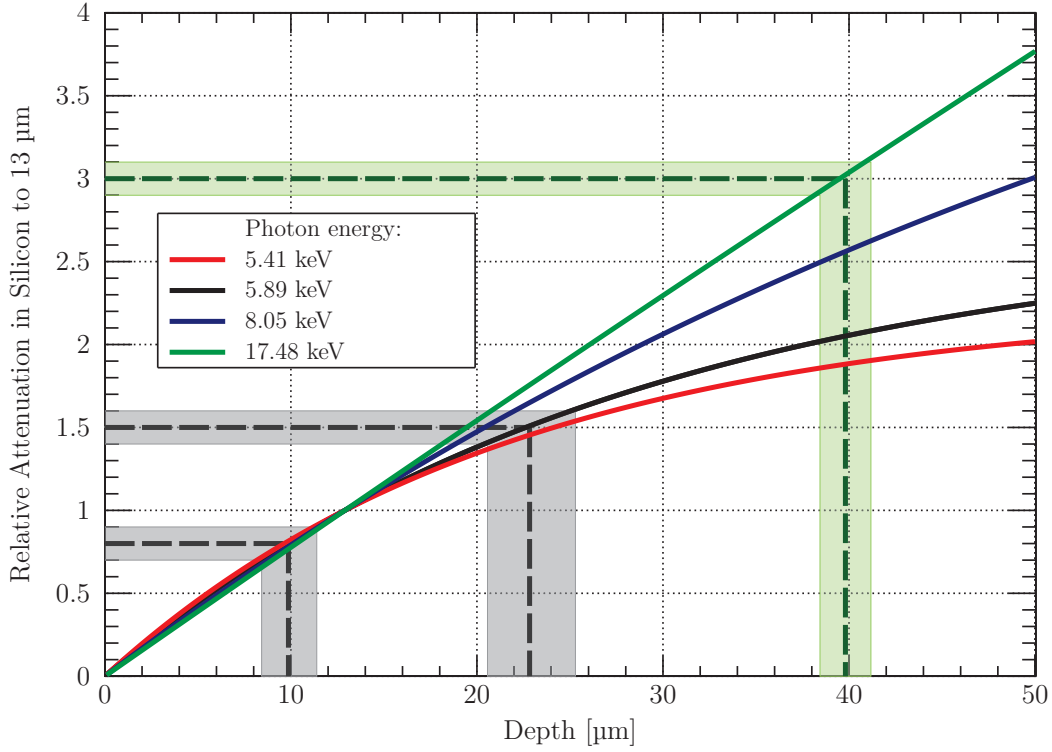
Figure 6.1: Relative attenuation to a fixed thickness ( x_0=13\text{ }\mu\text{m} ) for each sources used to characterize the sensitive thickness of the PIPPER-2 sensor. A relative attenuation below 1 between two different measurements suggests a sensitive depth below the fixed thickness while a relative attenuation above one between two measurements suggest a thicker depleted volume. With ^{55}\text{Fe} ( \mu(5.9\text{ keV})=154.82\text{ cm}^2\text{ g}^{-1} ), a relative attenuation of 0.8 evaluates the sensitive depth to x_1=10\text{ }\mu\text{m} when an attenuation of 1.5 gives a thickness of x_1\approx 23\text{ }\mu\text{m}
