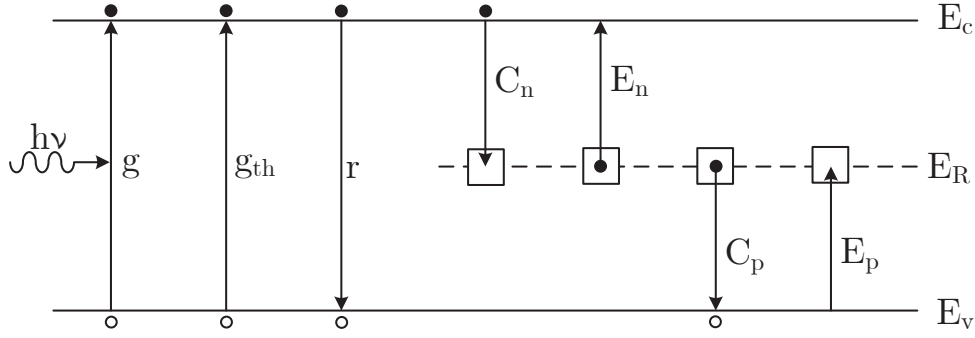
Figure 2.5: Generation and recombination processes under illumination
