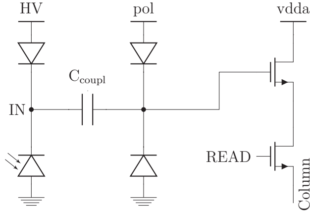
Figure 7.1: Schematics of the PIPPER-2 pixel. The substrate is polarized from the top through a forward bias diode and the collecting diode. The collection node is AC-coupled ( C_{\text{coup}} ) to a source follower. A set of diodes after the coupling at the input of the amplifier is used to set the DC point.
