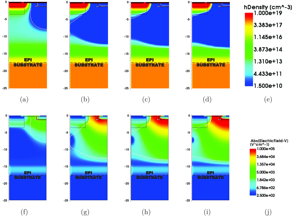
Figure 4.15: Behaviour of the depletion depth with the realistic HR18 model biased at (a) 2 V, (b) 20 V, (c) 30 V, and (d) 45 V. The 25 \mu m thick substrate is defined using the doping profile presented in figure 4.9. The total thickness is 25 \mu m thick with a 22 \mu m pitch (half of the pitch is displayed since only a quarter of the pixel is simulated). The diode located at the center of the pixel area is visible on the top right corner of each cross-section. The dark blue area in (a–d) is where the density of holes is below 5 % of the acceptors concentration. The electric field in the epitaxial layer for the same conditions as (a–d) are (f–i)
