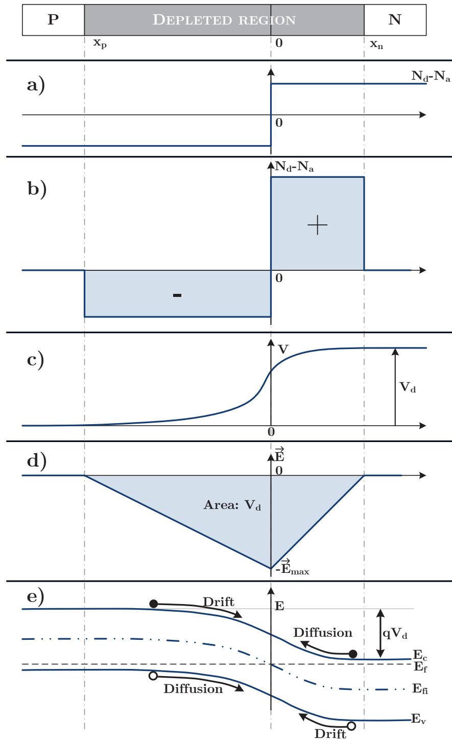
Figure 2.7: (a) Dopants (b) Charge (c) Potential. From 0 to the built-in potential across the junction (d) Electric field. The integration of the area represents the built-in voltage (e) Band diagram and effect on electrons and holes
