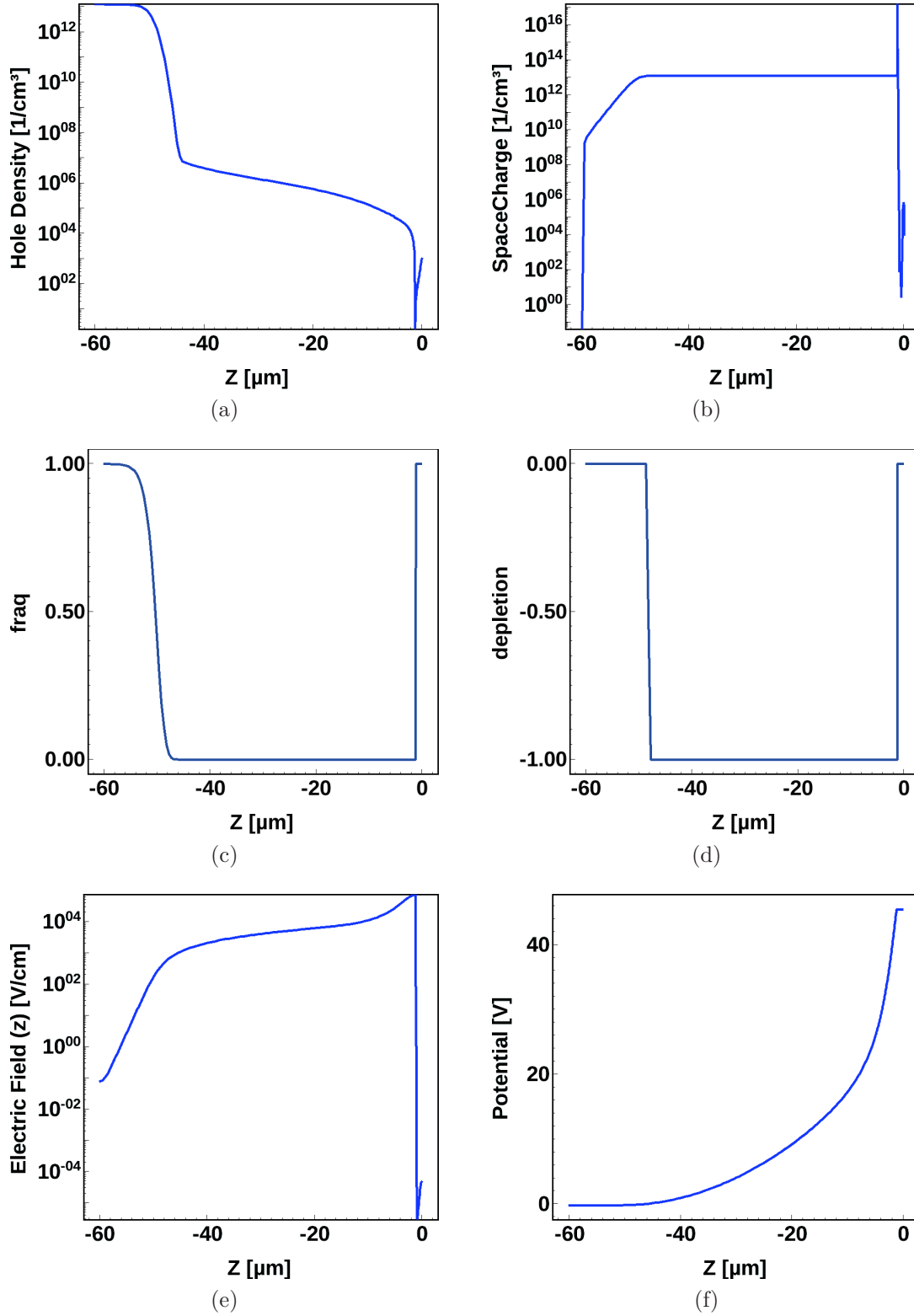
Figure 4.11: Simulation results of a simplified structure with a substrate resistivity of 600 \, \Omega \text{ cm} biased at 45 \text{ V} . The collecting diode is between 0 and -1.5 \, \mu\text{m} . (a) Hole density. (b) Q_{SC} (equation 4.20). (c) V_D (equation 4.21). (d) D (equation 4.22). (e) Electric field. (f) Potential
