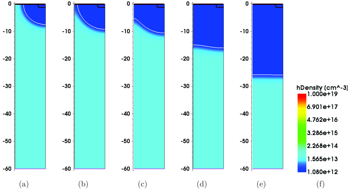
Figure 4.13: Behaviour of the depletion depth with the simplified model using a 600 \Omega \text{ cm} substrate biased at (a) 2 V, (b) 4 V, (c) 6 V, (d) 15 V, and (e) 30 V. The simulated substrate is 60 \mu\text{m} thick with a 22 \mu\text{m} pitch (half of the pitch is displayed since only a quarter of the pixel is simulated). The diode located at the center of the pixel area is visible on the top right corner of each cross-section. The dark blue area is where the density of holes is below 5 % of the acceptors concentration.
