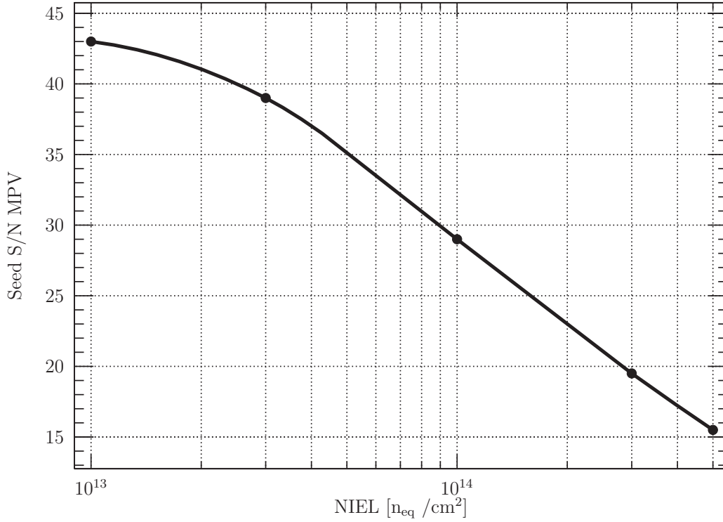
Figure 5.21: Seed signal to noise ratio MPV versus neutron fluence of PIPPER-2 fabricated on an 18 \mu m thick epitaxial layer biased at 20 V and cooled at -20 °C. Reproduced from A. Perez Perez in [156]
