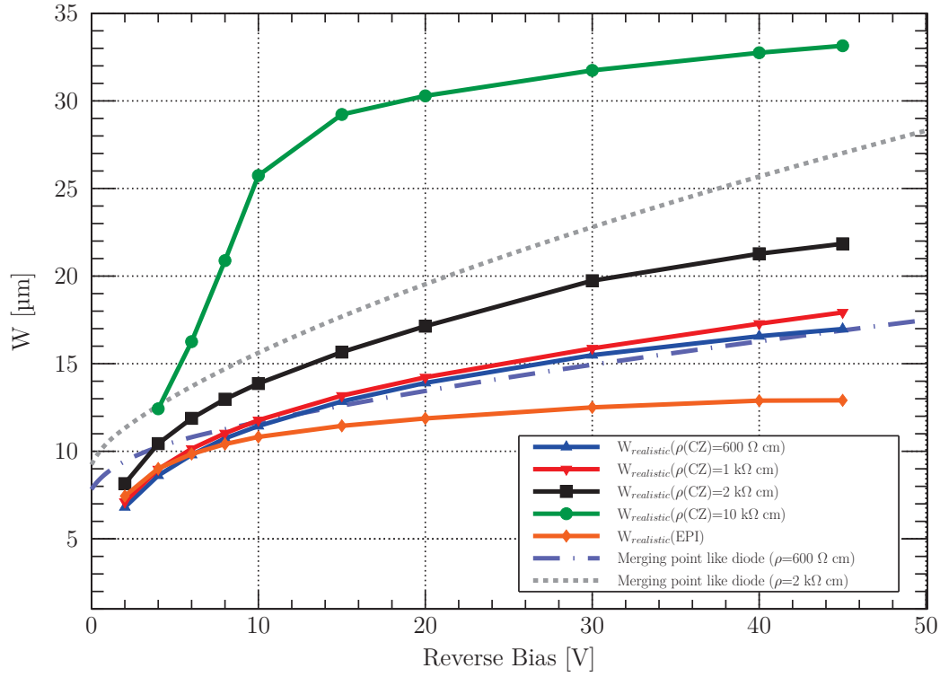
Figure 4.17: TCAD simulated depletion depth reached in a realistic PIPPER-2 bulk structure at various resistivities: 600 \Omega \text{ cm} , 1 k \Omega \text{ cm} , 2 k \Omega \text{ cm} , and >10 k \Omega \text{ cm} and in the HR18 structure. The simulations are compared to the point like diode equation for a bulk resistivity of 600 \Omega \text{ cm} , and of 2 k \Omega \text{ cm}
