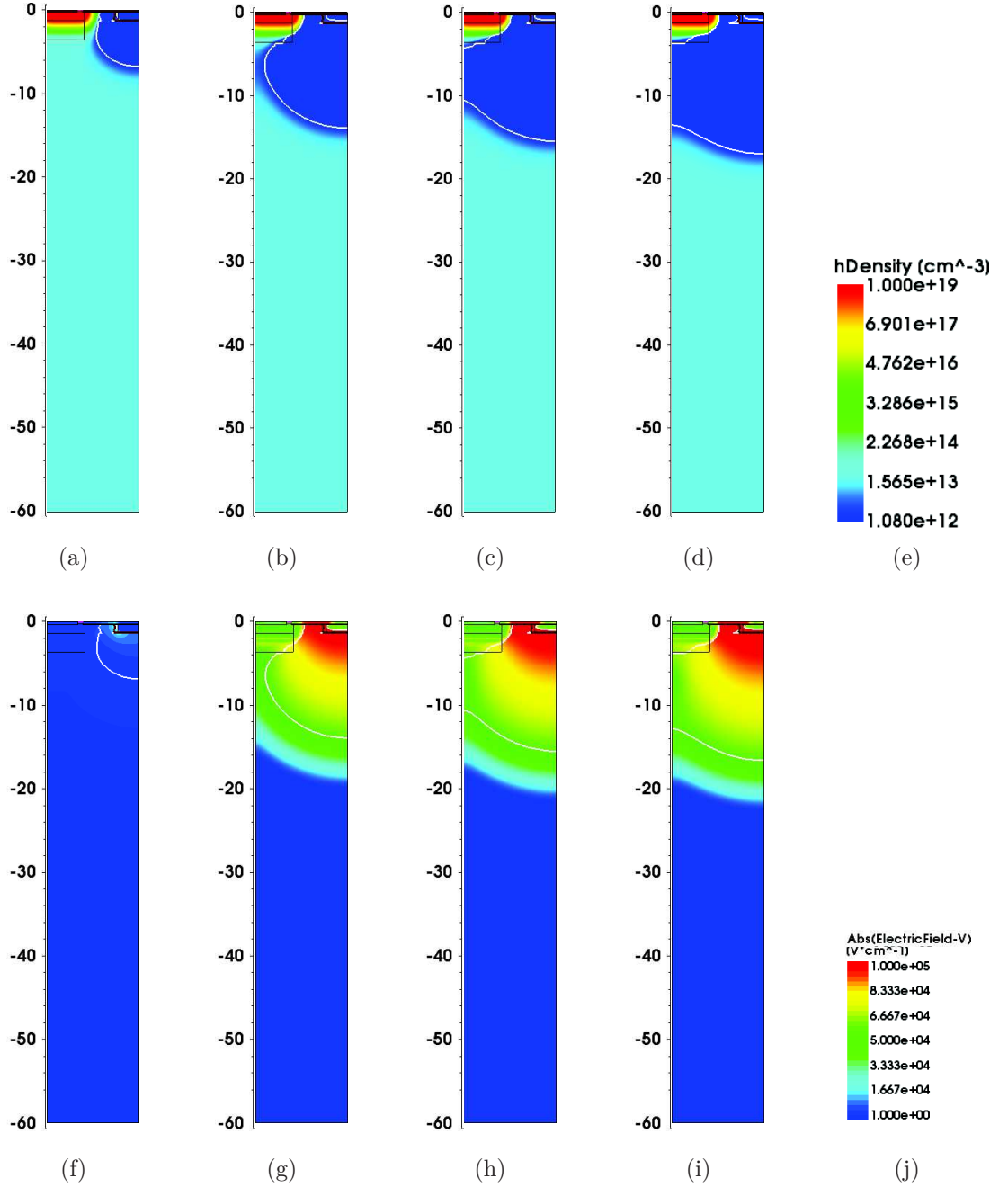
Figure 4.16: Behaviour of the depletion depth with the realistic CZ model using a 600\ \Omega\ \text{cm} substrate biased at (a) 2 V, (b) 20 V, (c) 30 V, and (d) 45 V. The simulated substrate is 60\ \mu\text{m} thick with a 22\ \mu\text{m} pitch (half of the pitch is displayed since only a quarter of the pixel is simulated). The diode located at the center of the pixel area is visible on the top right corner of each cross-section. The dark blue area is where the density of holes is below 5 % of the acceptors concentration.
