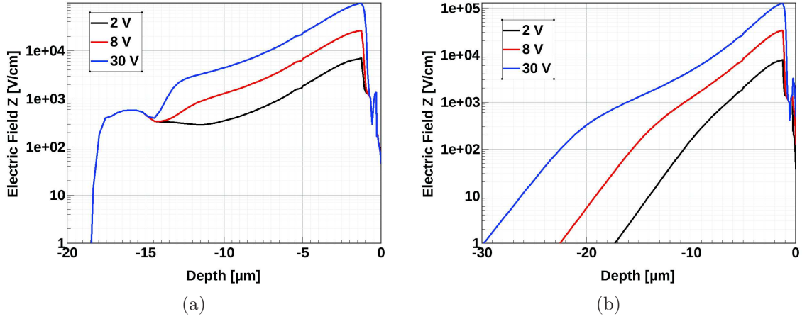
Figure 4.18: Simulations of the electric field along the Z-axis for different diode bias voltage (2 V, 8 V, and 30 V) in the (a) HR18 structure, and the (b) realistic CZ with a 2 kΩ cm structure
