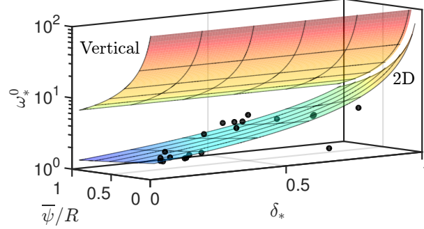
Figure 4.15: Resonant reduced frequency \omega_3^0 as a function of the dimensionless stand-off distance \bar{\psi}/R and the dimensionless diffusion layer thickness \delta_* according to the vertical mechanism from Eq. (4.9) (upper surface) and the bidimensional mechanism from Eq. (4.11) (lower surface). Experimental values corresponding to all flames described in Table 2.1 are represented as black spheres.
