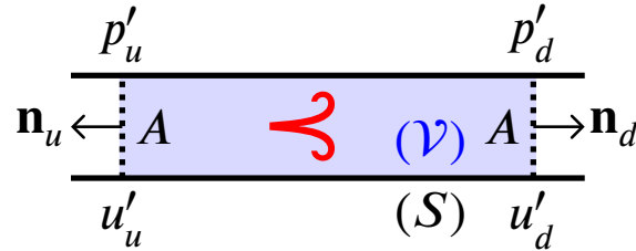
Figure 8.1: Sketch of a compact flame stabilized in a low-Mach flow within a straight duct. The acoustic pressure and acoustic velocity at the duct inlet are denoted by p'_u and u'_u respectively. The acoustic pressure and acoustic velocity at the duct outlet are denoted by p'_d and u'_d respectively. The control volume ( \mathcal{V} ) retained here is bounded by a surface ( S ).
