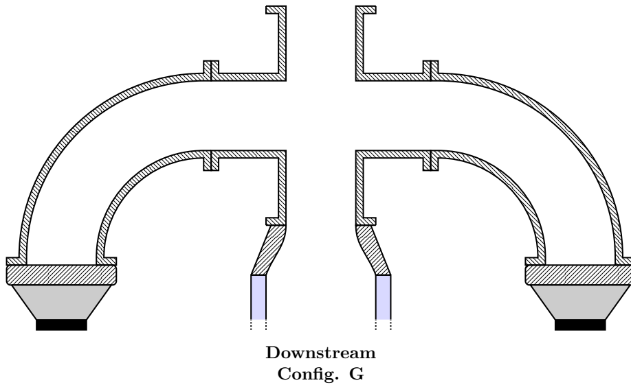
Figure 5.9: Active downstream configuration of the NoiseDyn burner : Configuration G . The elements placed above the loudspeakers are water-cooled in order to protect the loudspeakers' membranes.
