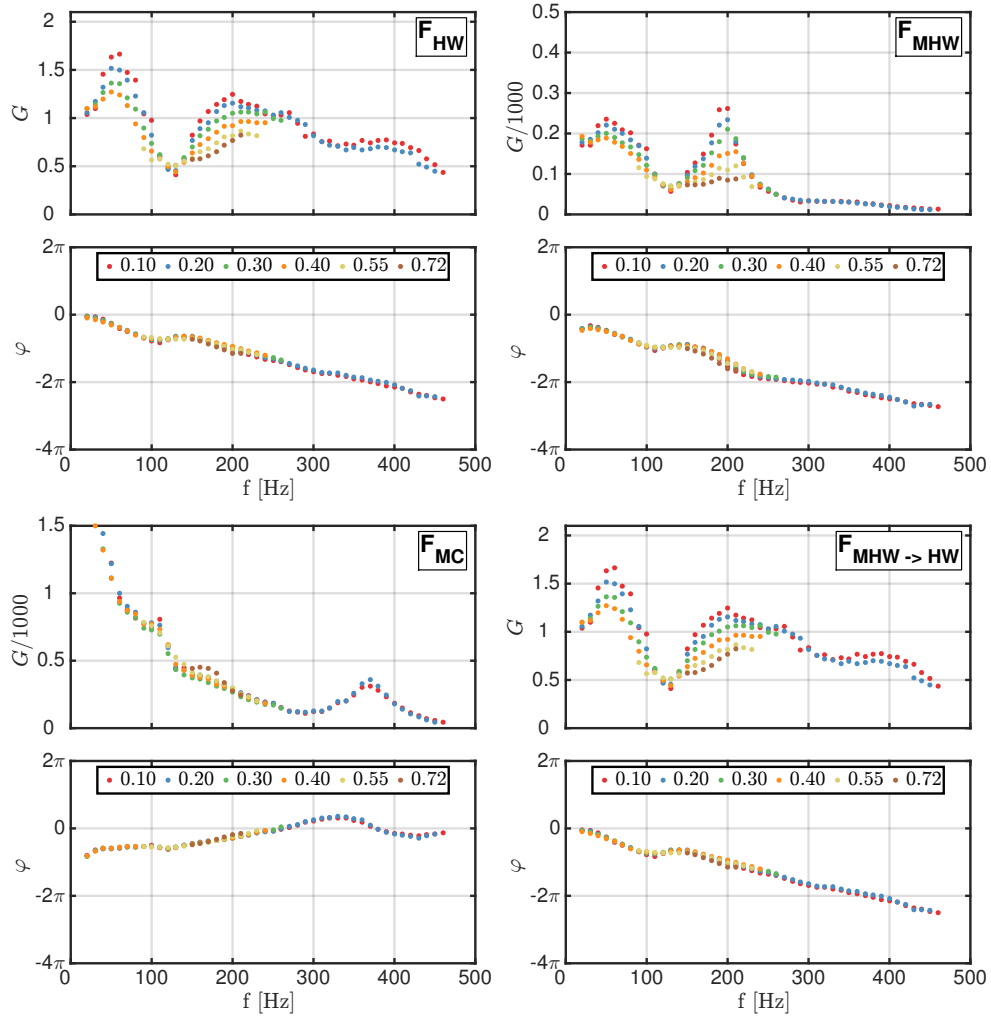
Figure 9.7: Describing functions of a fully premixed confined swirling flame obtained with upstream forcing for six different forcing levels |u'_0|/\bar{u}_0 measured at the hot wire location. F_{HW} : (\dot{Q}'/\bar{Q})/(u'_0/\bar{u}_0) . F_{MHW} : (\dot{Q}'/\bar{Q})/(p'_0/\bar{p}_0) . F_{MC} : (\dot{Q}'/\bar{Q})/(p'_s/\bar{p}_s) . F_{MHW \rightarrow HW} = Z_s \bar{u}_0 F_{MHW}/\bar{p}_0 .
