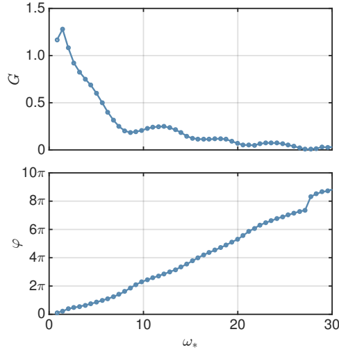
Figure 4.5: Gain (Top) and phase (Bottom) of the FTF of a premixed laminar conical \text{CH}_4/\text{air} flame with \phi = 1.00 , \bar{h}/R = 4 , R = 7 \text{ mm} , Le = 0.93 and T_* = 6.42 ( FS15 ).
