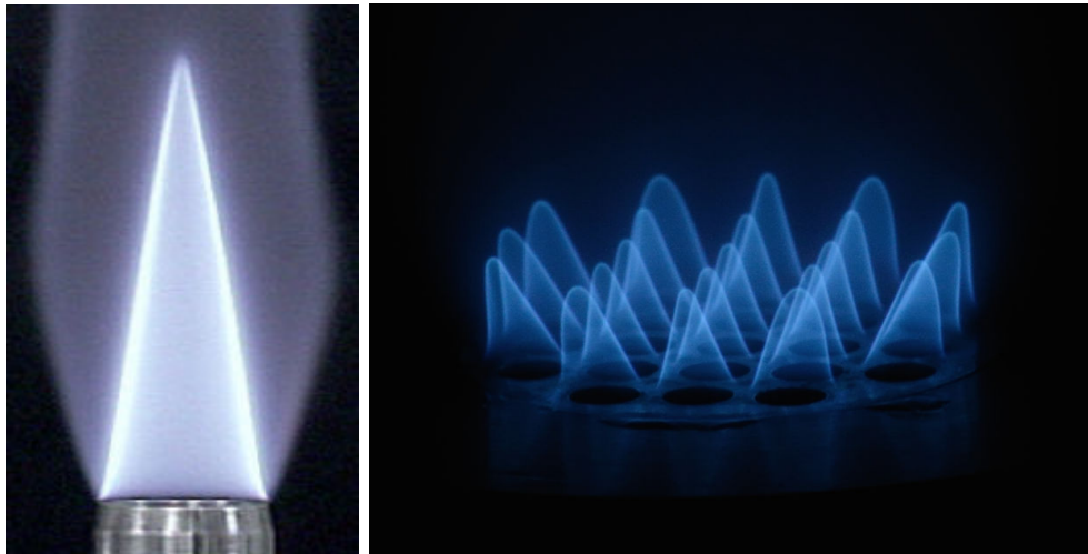
Figure 1.4: (Left): Example of a large premixed laminar conical \text{CH}_4/\text{Air} flame of equivalence ratio \phi = 0.95 obtained with an injector of radius R = 11 mm traversed by a fresh reactant stream of bulk velocity \bar{u}_b = 2.5 m/s, reproduced from Durox et al. (2004). (Right): Example of a collection of small premixed laminar conical \text{CH}_4/\text{Air} flames at stoichiometry stabilized on a plate featuring 21 holes of radius R = 1.5 mm traversed by a fresh reactant stream of bulk velocity \bar{u}_b = 1.48 m/s.
