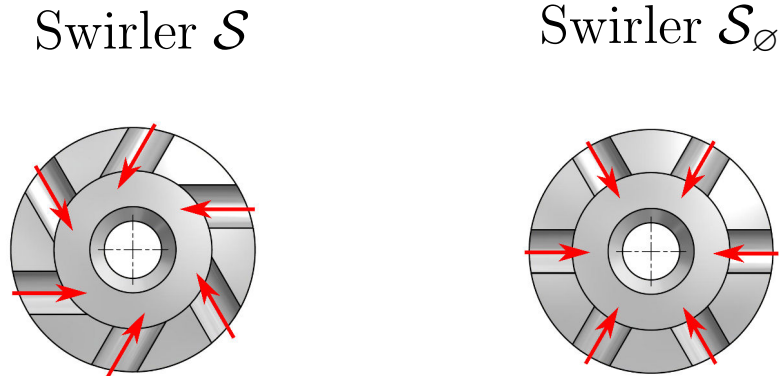
Figure 5.4: Cross-sectional top view of the swirlers used in the NoiseDyn burner. A cylindrical bluff body fills the central aperture. The premixed gases flow from the outer to the inner regions of the swirler channels. (Left): Swirler \mathcal{S} that generates a swirling flow characterized by a Swirl number S = 0.8 . (Right): Swirler \mathcal{S}_\emptyset that generates a non-swirling flow.
