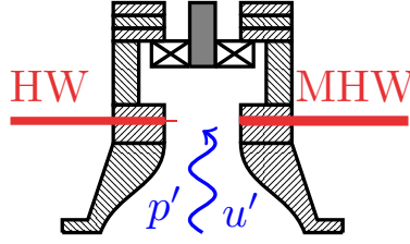
Figure 6.11: Acoustic impedance measurement with a hot wire probe and a microphone. The hot wire probe (HW) and microphone (MHW) are located at the same axial position and their signals are recorded simultaneously.
