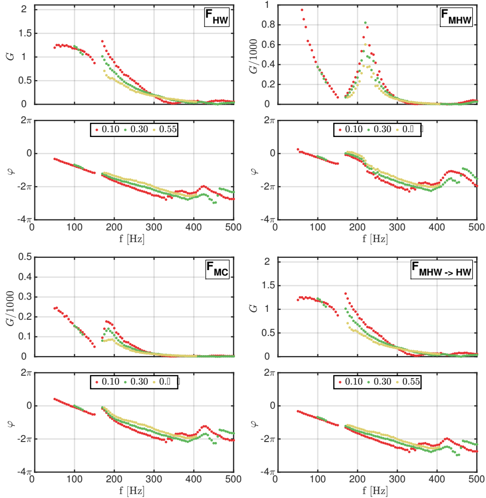
Figure 9.11: Describing functions of a fully premixed confined non-swirling flame obtained with downstream forcing for three different forcing levels |u'_0|/\bar{u}_0 measured at the hot wire location. F_{HW} : (\dot{Q}'/\bar{Q})/(u'_0/\bar{u}_0) . F_{MHW} : (\dot{Q}'/\bar{Q})/(p'_0/\bar{p}_0) . F_{MC} : (\dot{Q}'/\bar{Q})/(p'_8/\bar{p}_8) . F_{MHW \rightarrow HW} = Z_s \bar{u}_0 F_{MHW}/\bar{p}_0 .
