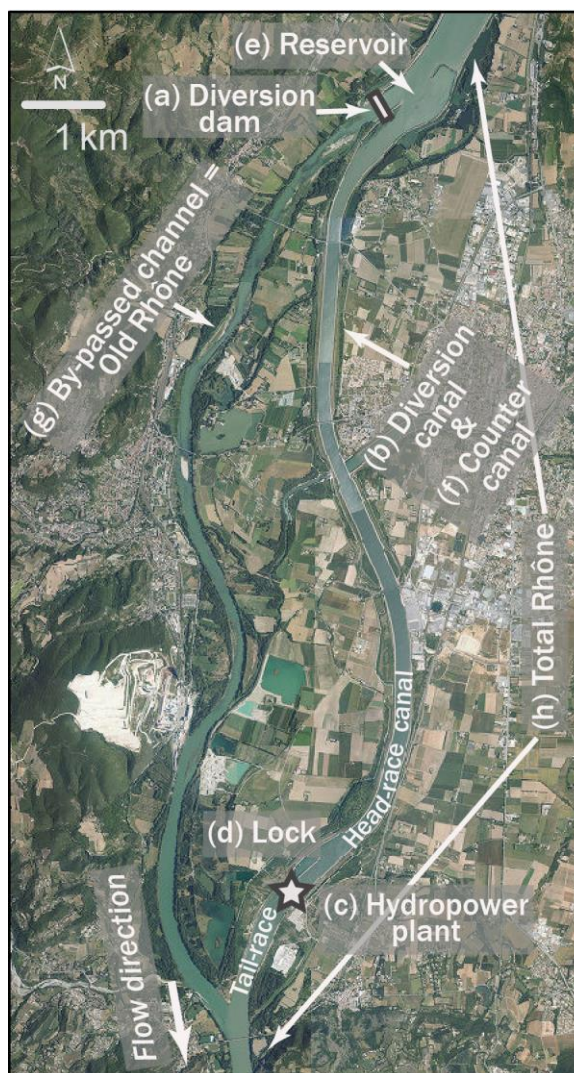
Figure II-5: Typical arrangement of a diversion scheme on the Rhône. Example of the by-passed reach of Péage de Roussillon.
