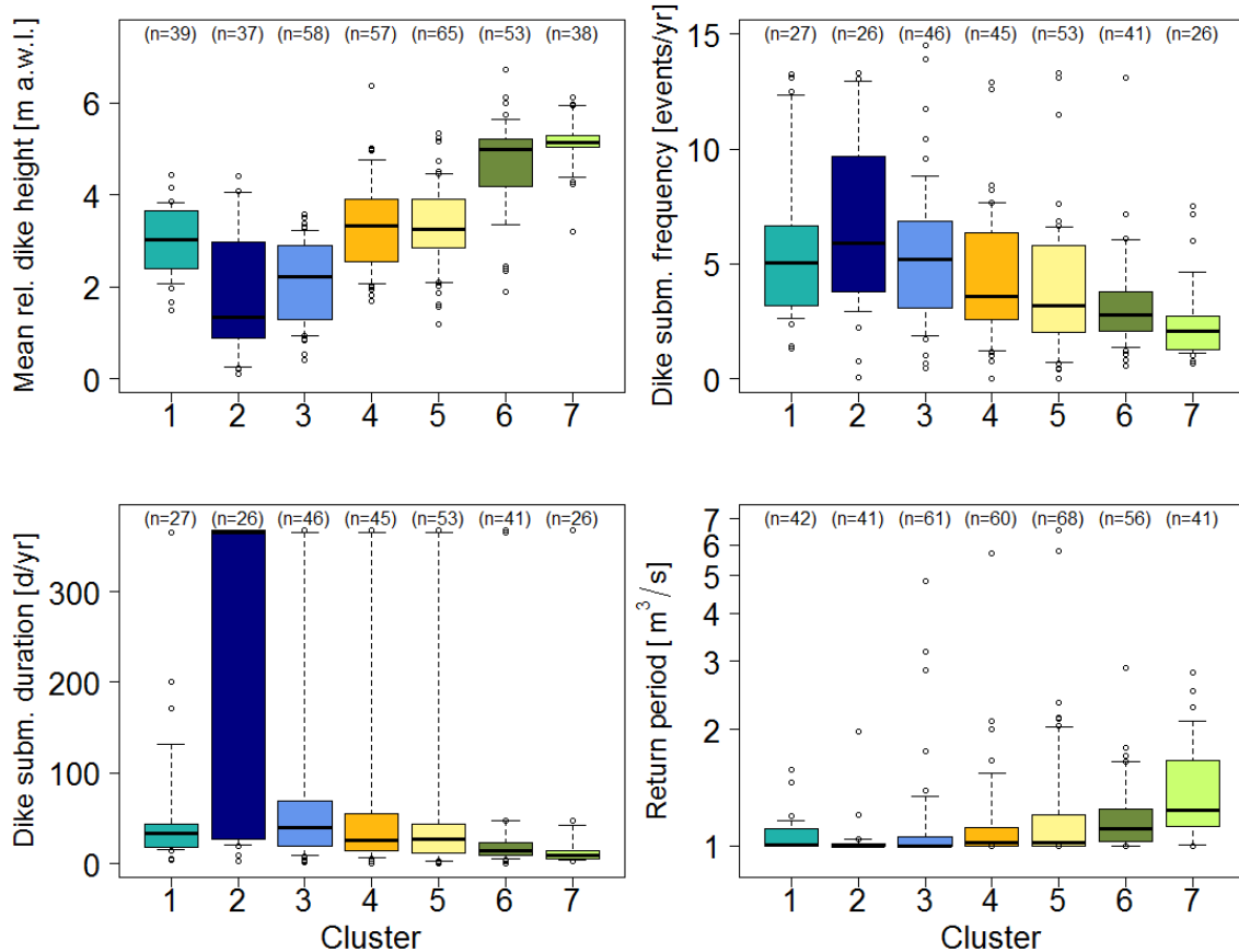
Figure IV–27: Comparison of connectivity variables between the seven morpho-topographical clusters.
