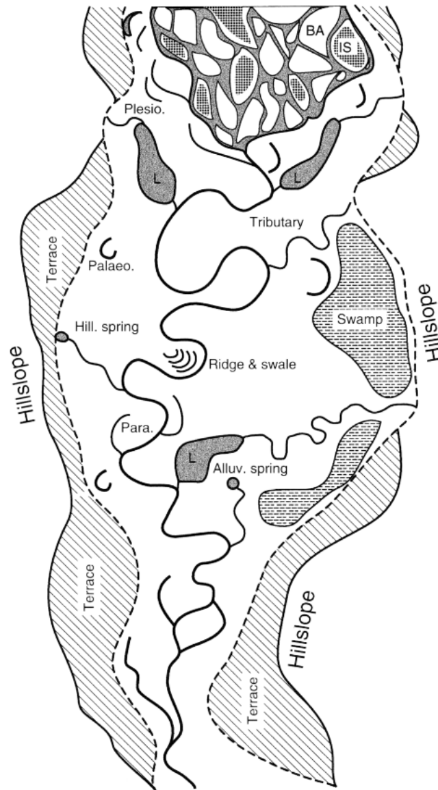
Figure I-1: Schematic example of geomorphic landforms of river-floodplain systems along a gradient of connectivity and successional stage (Ward et al., 2002, based on the classification from Amoros et al., 1982 and Amoros et al., 1987): lotic main and side channels (= eupotamon), tributary streams and alluvial springbrooks, semi-lentic cut-off channels connected to the main channel system at the downstream end (= parapotamon; e.g. abandoned braid channels close to the active channel), permanent or temporary lentic water bodies without permanent or direct connection to the main channel system but highly influenced by river discharge (= plesiopotamon), and permanent or temporary lentic water bodies without permanent or direct connection to the main channel system and only mildly influenced by river discharge (= paleopotamon; e.g. abandoned meander loops), terrestrial bars or levees.
