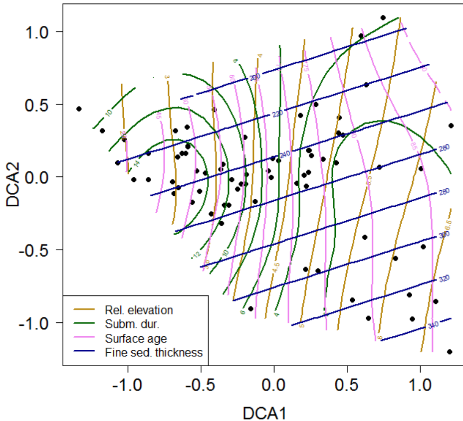
Figure VI-20: Surfaces of environmental variables fitted to ordinations of the DCA.
