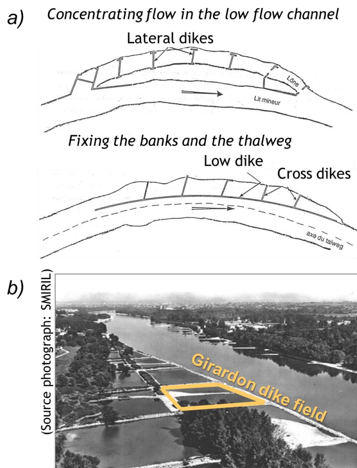
Figure II-3: What is a dike field? a) Idealised schemes of the arrangement of dikes in secondary channels (top) and in the main channel (bottom) (modified from Poinsart (1992) and b) the resulting dike fields.
