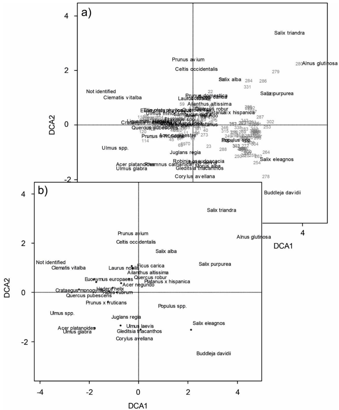
Figure VI-11: Results from a DCA on both dike fields and reference sites: biplots with a) species and samples, and b) a zoom on species for improved readability (overlapping labels deleted).
