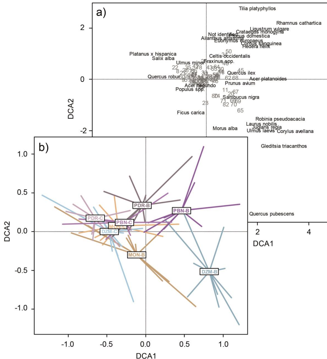
Figure VI-13: Results from a DCA on dike fields only: biplots with a) species and samples and b) samples coded by reach and pre- vs. post-dam surfaces.
