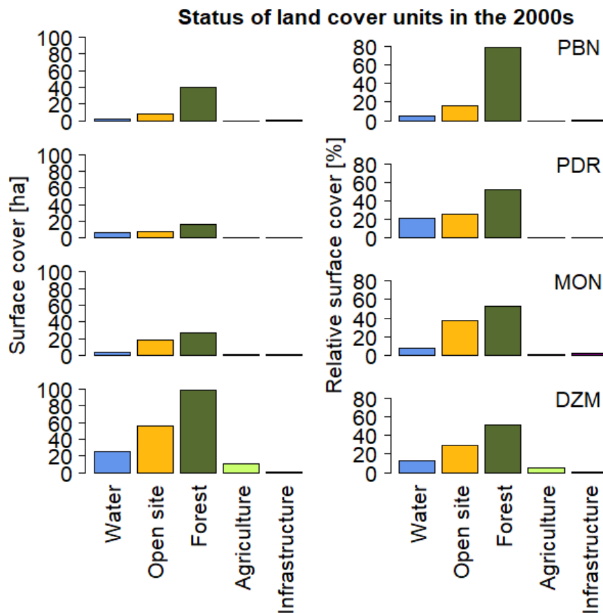
Figure IV–23: Contemporary distribution of land cover units in dike fields compared between the four reaches ( N_{PBN} = 113 , N_{PDR} = 73 , N_{MON} = 62 , N_{DZM} = 109 ).
