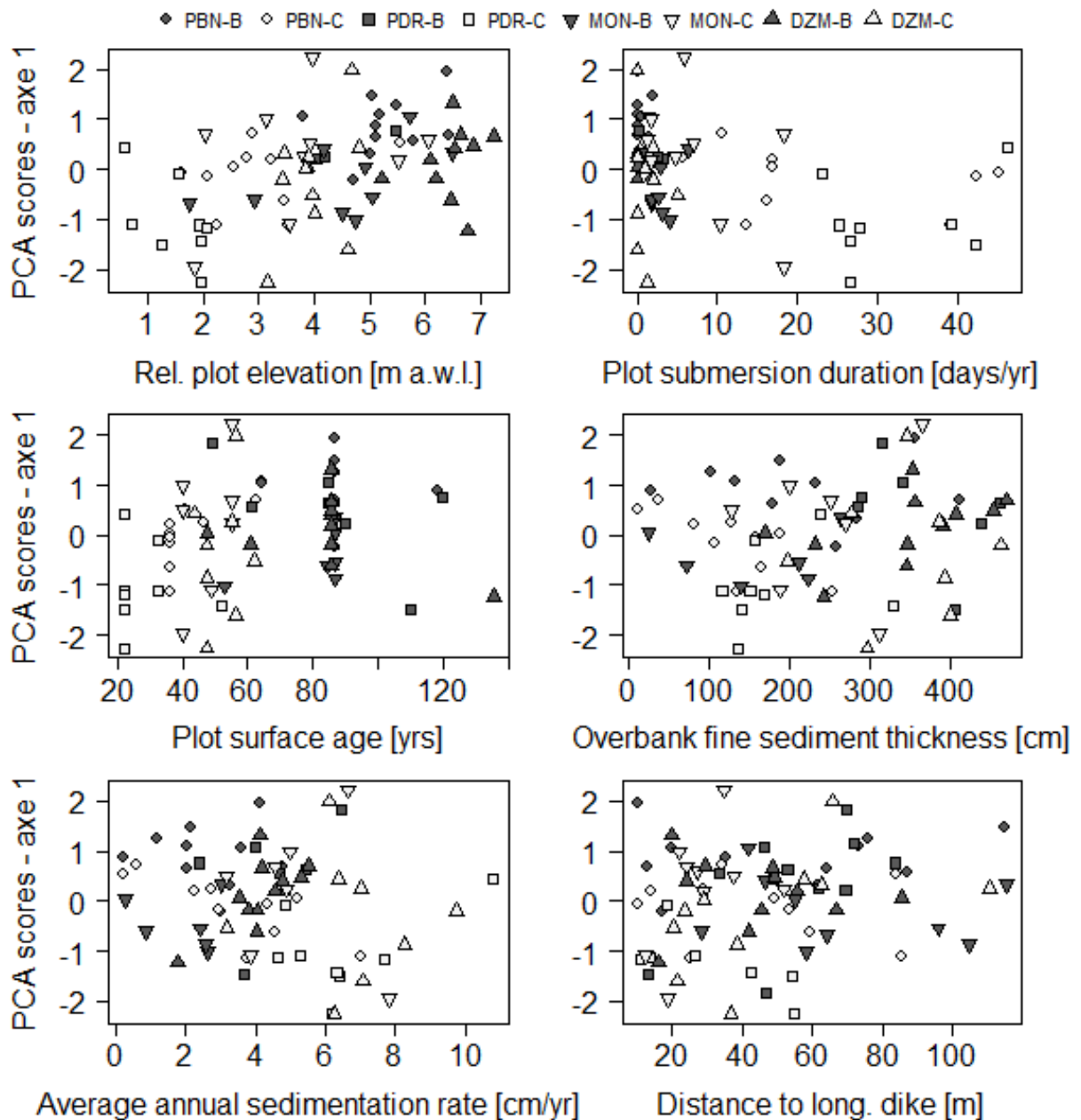
Figure VI–19: Relationship between control variables and PCA scores on axis 1.
