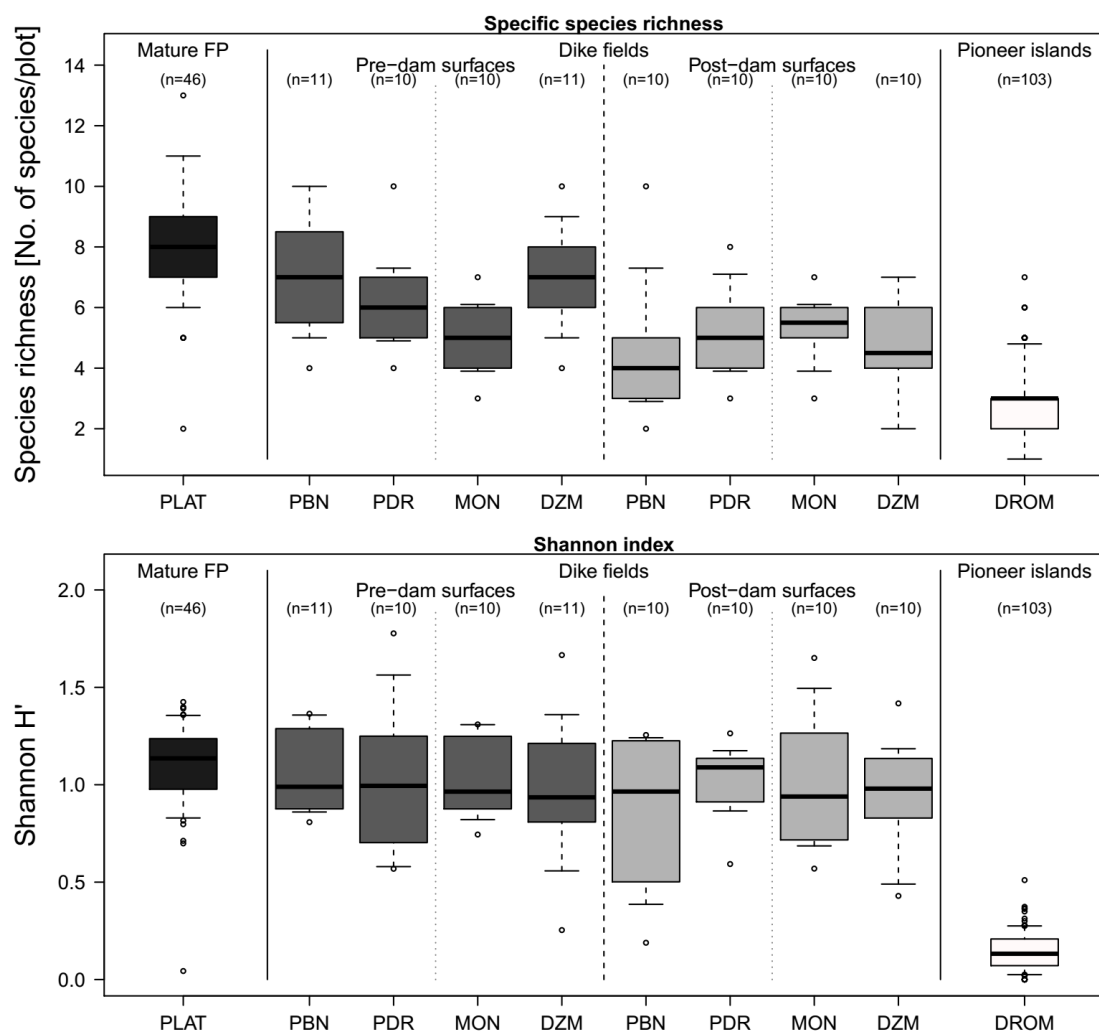
Figure VI-6: Comparison of compositional forest stand characteristics between dike fields and between dike fields and reference sites. Top: species richness, bottom: Shannon diversity index.
