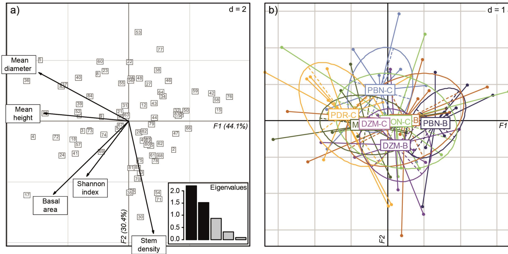
Figure VI-8: Results of the PCA on structural forest stand parameters. a) Factor map. b) Representation of the individual plots coloured by the study reach and period they belong to on the factor map. The four labels in the centre of the plot, which overlap, are from left to right: MON-B (dark green), DZM-C (light violet), MON-C (light green), and PDR-B (dark orange).
