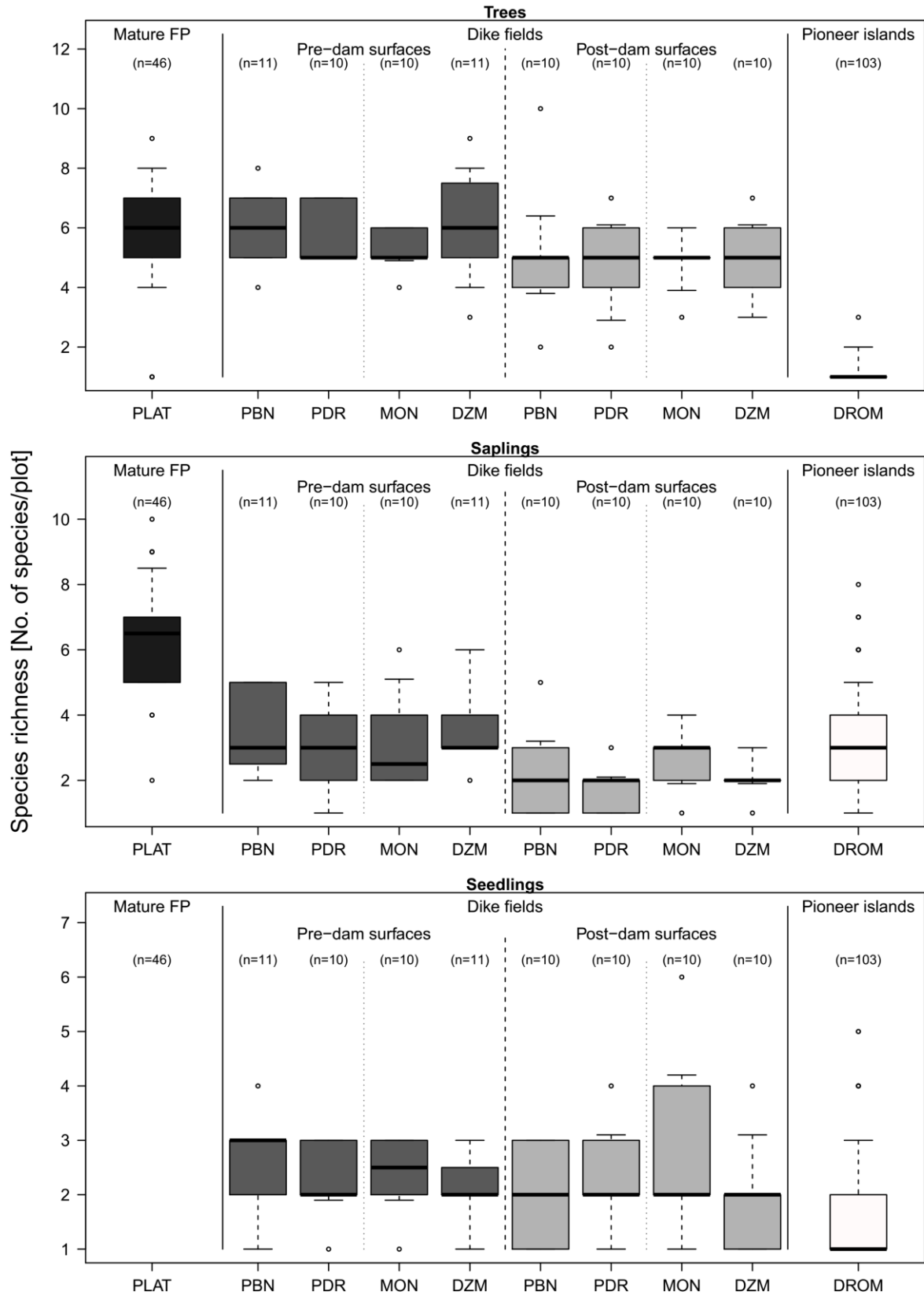
Figure A-III-5: Comparison of species richness per plot between dike fields and between dike fields and reference sites for each LHS separately.
