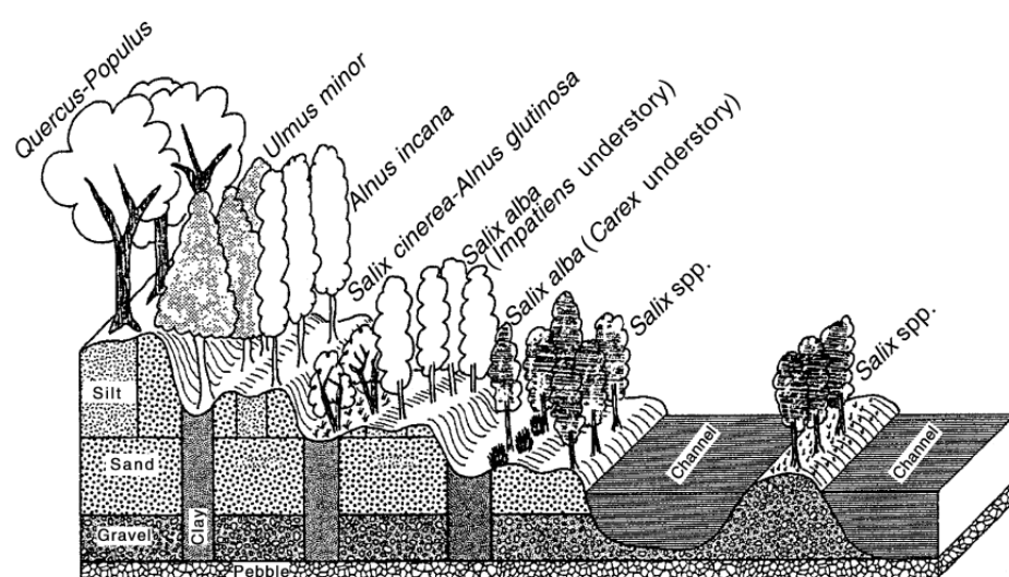
Figure I-2: Zonation of dominant species in woody riparian vegetation assemblages along a lateral transect on a braided reach of the Upper Rhône River (Ward et al., 2002, modified after Pautou, 1984).
