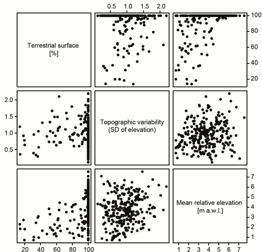
Figure IV–15: Binary relationships between PCA input variables.
