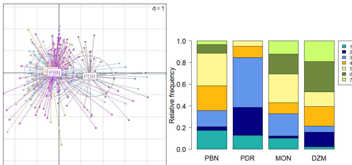
Figure IV-18: Reach-scale patterns behind the PCA and clustering results: colour coding the PCA factor map introduced in according to the study reach (left). Distribution of clusters between reaches (right).
