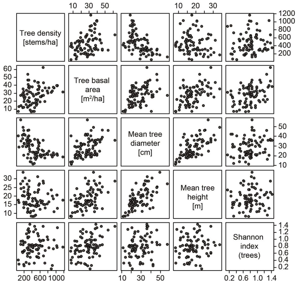
Figure VI-7: Bivariate relationships between PCA input variables.
