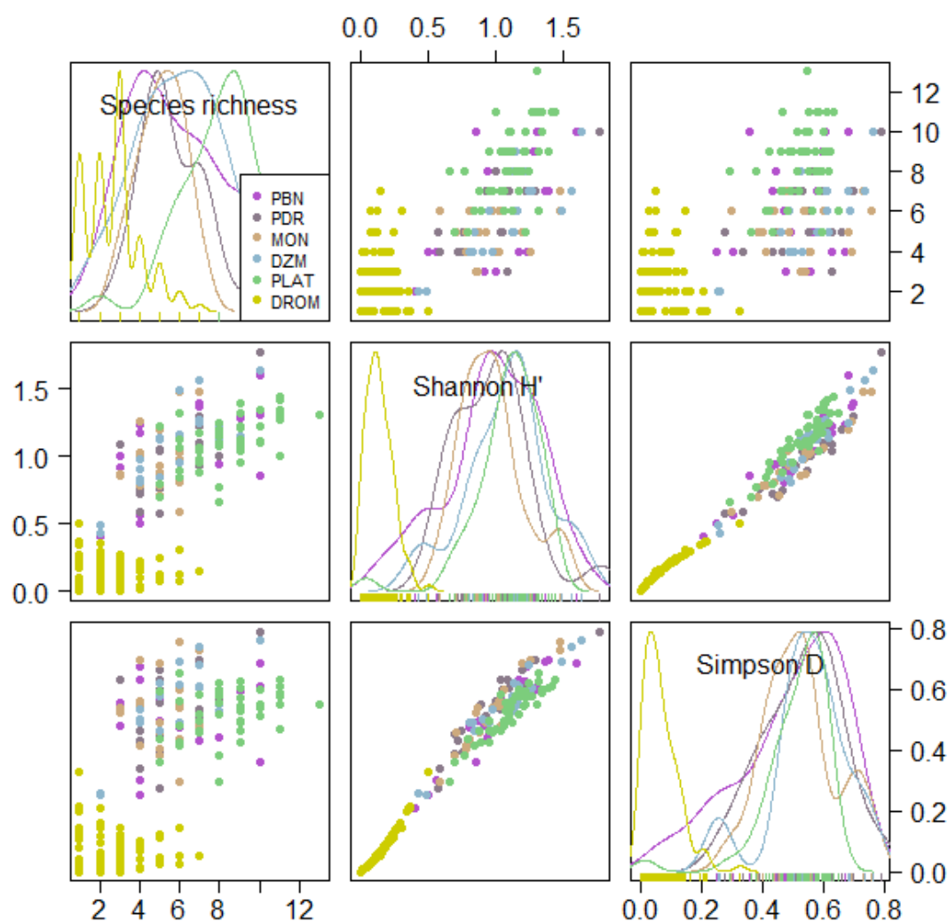
Figure VI-5: Scatter plots showing the relationships of the three variables describing the species richness of the six sites. The diagonal line represents density plots of each variable per site.
