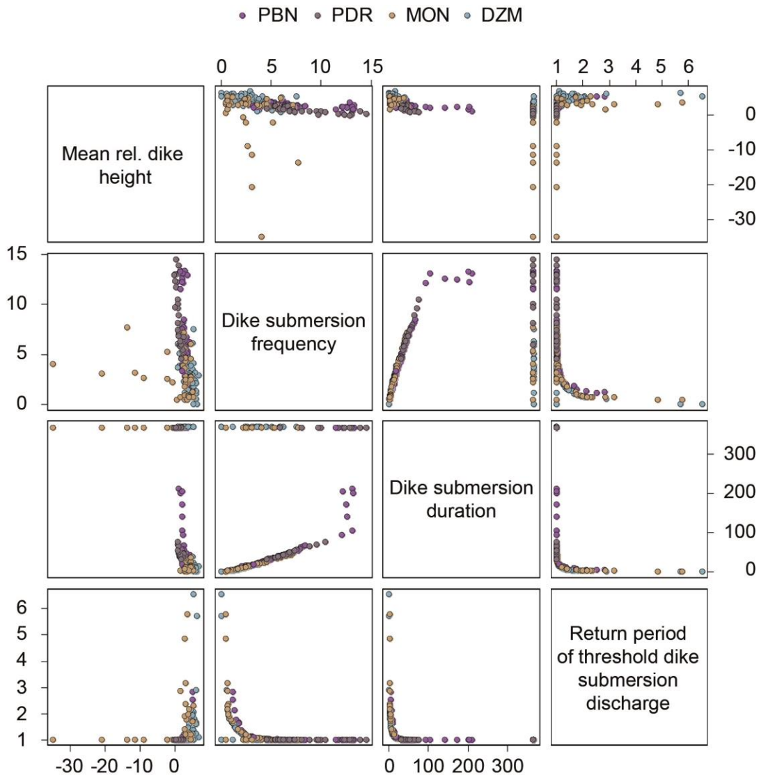
Figure IV-19: Bivariate relationships between the four variables used as proxies for hydrological connectivity of the dike fields.
