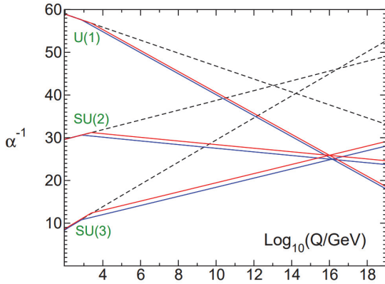
Inverse coupling constants evolution obtained by a two-loop renormalization performed in the Standard Model (dashed lines) and in the Minimal Supersymmetric Standard Model (solid lines). The masses of the heavy superpartners is varied between 750 GeV and 2.5 TeV. Supersymmetric coupling constants meet at the energy of 10^{16} GeV, whereas their usual equivalent never intersect. This figure is taken from [13]
