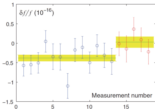
A. Relative shift in frequency of an atomic clock at the surface of the earth, then lifted by 33 cm.
