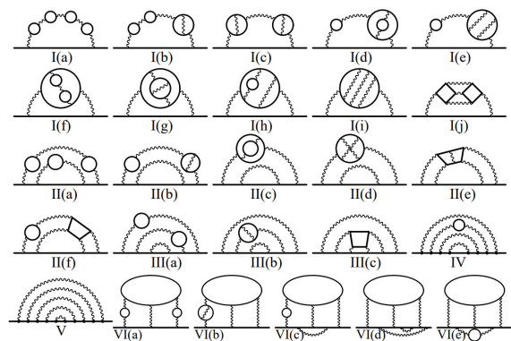
B. Sample of the Feynman diagrams calculated to obtain the anomalous magnetic moment of the electron a_e = 0.001156652181643(764)
