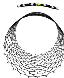
Figure 6. Structure of the ZnPc stacked at the outer surface of NT (17,0) from our DFT calculations.
