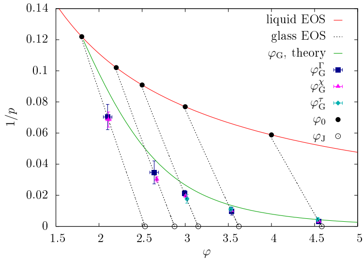
Figure 6.8. The Gardner transition points located with the three different estimators \varphi_G^T , \varphi_G^X and \varphi_G^J . The numerical estimate is robust and consistent with the theoretical prediction reported in chapter 4.
