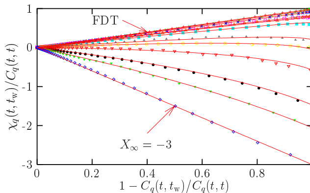
Figure 2.7. Susceptibility vs. correlation plots for the FA model in d = 3 . Symbols are numerical data while lines are theoretical calculations. Wave-numbers decrease from top to bottom, with the bottommost corresponding to q = 0 . A negative FDR is observed. Reprinted from [169].
