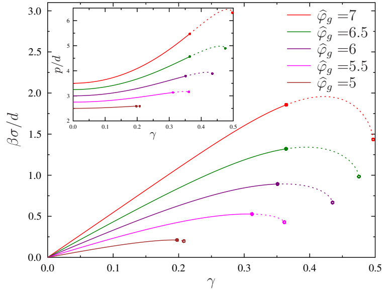
Figure 4.8. Following glassy states prepared at \hat{\varphi}_g upon applying a shear-strain \gamma . Shear-stress \sigma ( main panel ) and reduced pressure p ( inset ) as a function of strain for different \hat{\varphi}_g . Same styles as fig. 4.4. Upon increasing the strain, the states undergo a Gardner transition at \gamma_G(\hat{\varphi}_g) . For \gamma > \gamma_G our RS computation is unstable but predicts a stress overshoot followed by a spinodal point.
