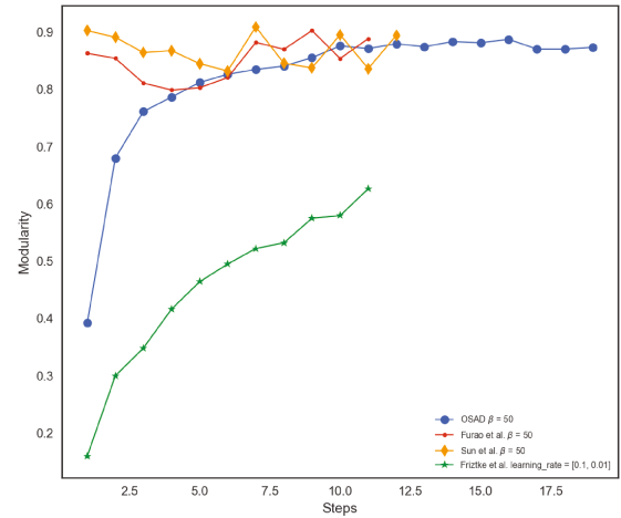
(b) Modularity
