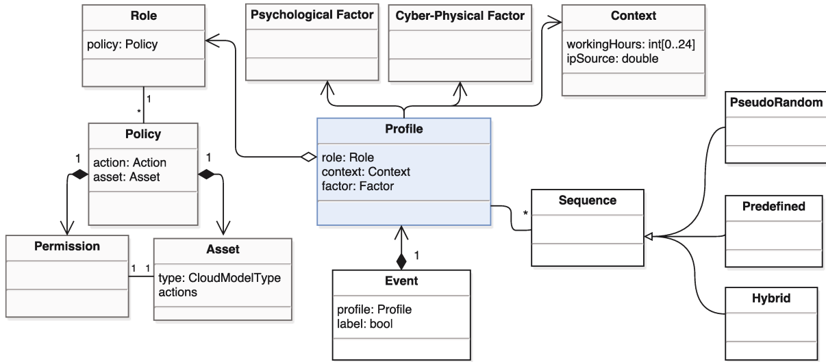
Figure 3.2 – Class models for generation of cloud insider threat dataset
