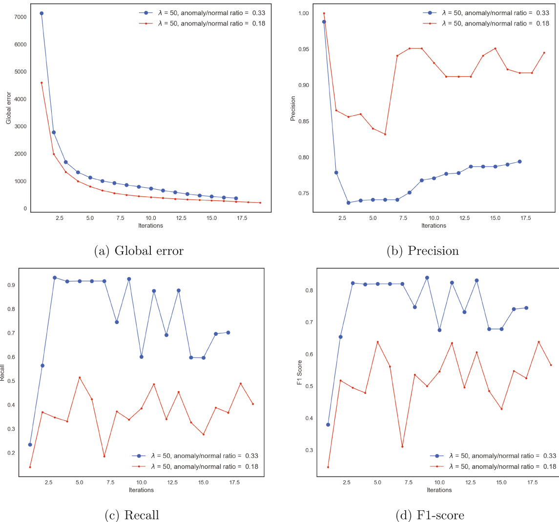
Figure 6.6 – External evaluation metrics for different anomaly/normal ratio with scenario 1
