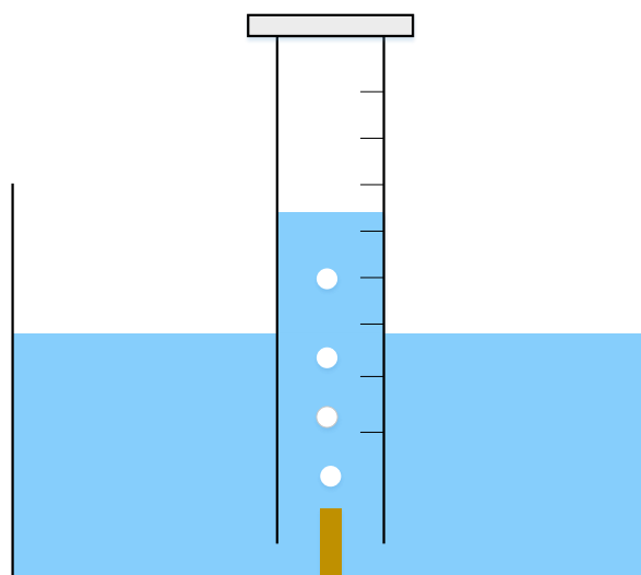
FIGURE 3.10: Bubble meter method to measure gas flow rate.
