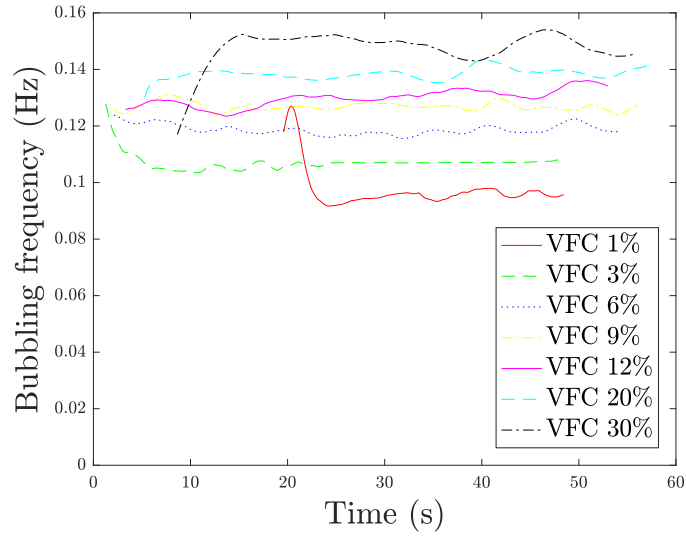
FIGURE 3.15: Bubbling frequency for all the flow rates.
