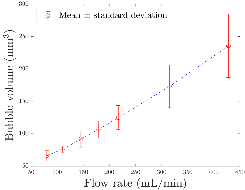
FIGURE 3.21: The mean and standard deviation of bubble volumes at steady state.
