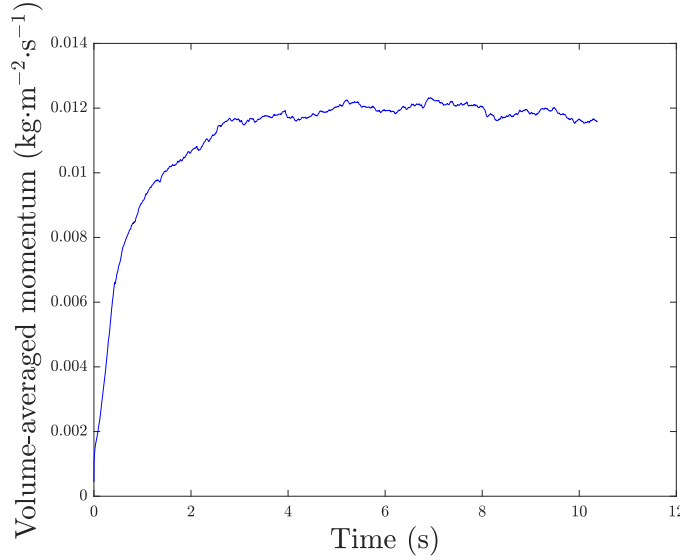
FIGURE 5.2: The evolution of volume-averaged momentum.
