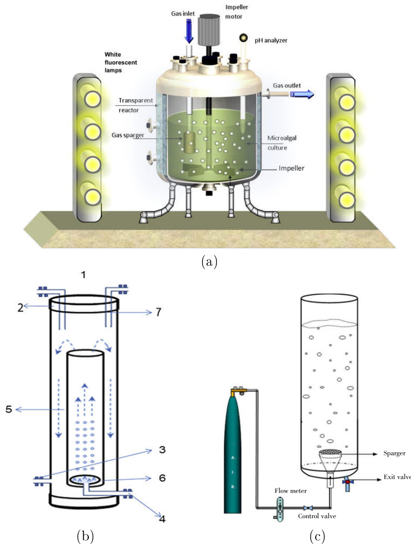
FIGURE 2.3: A schematic diagram of different types of photobioreactor: (a) stirred tank [28], (b) airlift [29], (c) bubble column [30].
