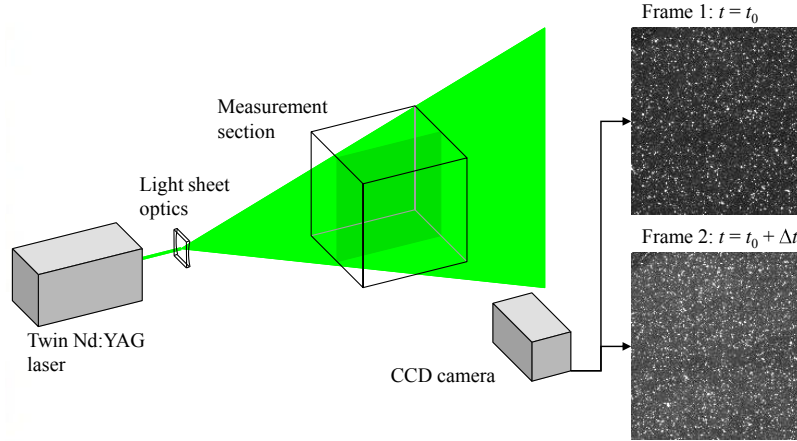
FIGURE 5.5: Schematic sketch of a PIV system, illustration from [183].
