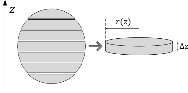
FIGURE 3.16: The horizontal segmentation method to calculate bubble volume.
