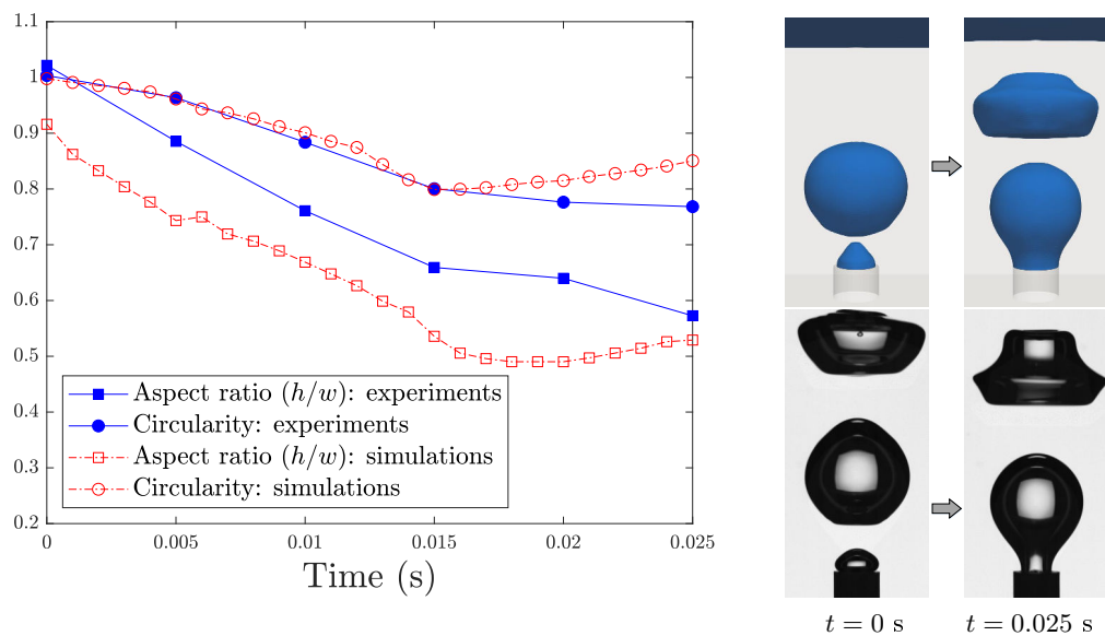
FIGURE 4.29: Evolution of bubble shape factors. The images have the same scale : 3 mm = 126 pixels. VFC: 20%.
