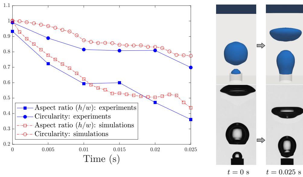
FIGURE 4.26: Evolution of bubble shape factors. The images have the same scale : 3 mm = 126 pixels. VFC: 6%.
