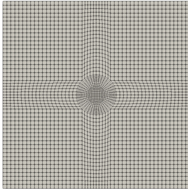
FIGURE 4.13: The bottom view of the meshed computational domain.
