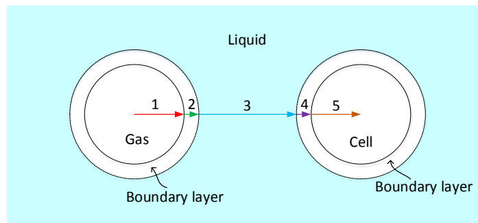
FIGURE 2.12: Chain of mass transfer in a photobioreactor.
