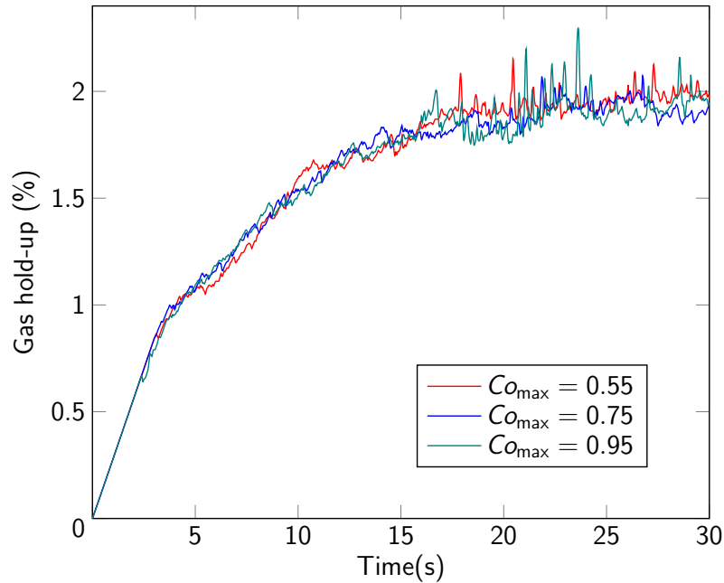
FIGURE 4.8: The influence of Courant number on gas hold-up, mesh size \Delta x = 1 mm.
