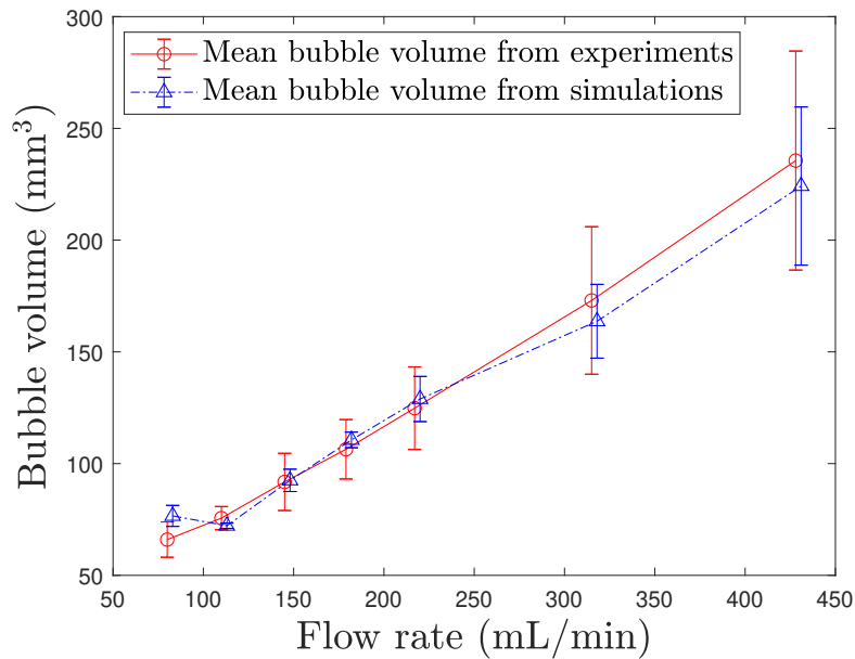
FIGURE 4.23: Comparison of bubble volumes obtained from simulations ( V_{\text{sim}} ) and experiments ( V_{\text{img}} ). The vertical bar is the standard deviation. The curve for simulations are slightly shifted to the right to better distinguish the two curves.
