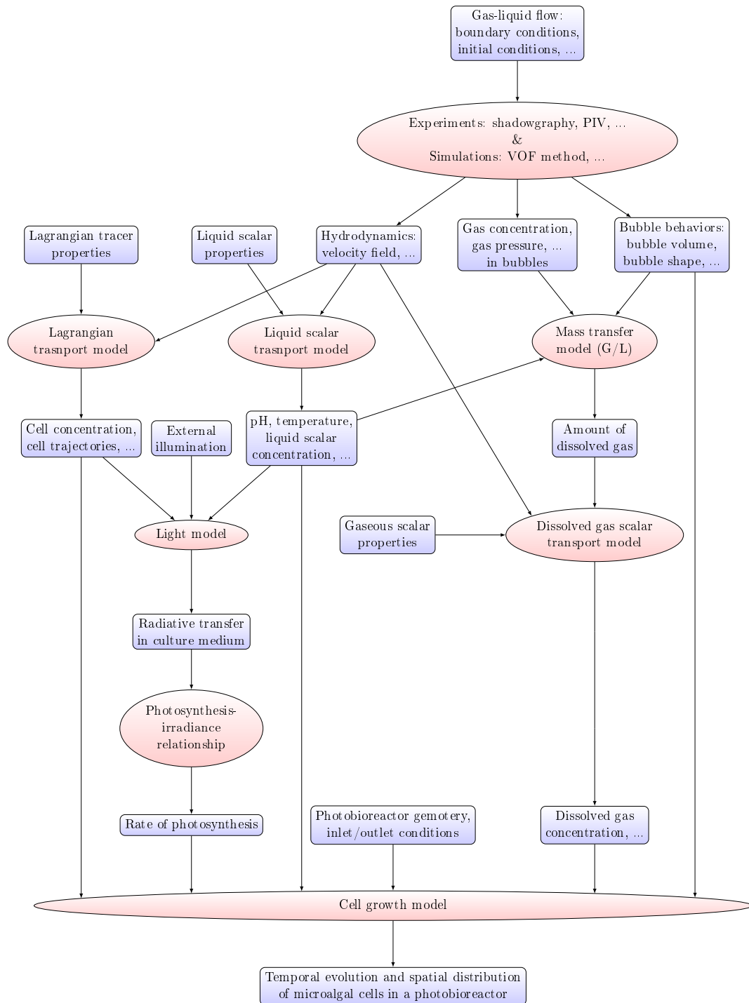
FIGURE 2.24: The basic structure of the complete model. An ellipse represents a model handling a specific problem, and a rectangle represents the inputs required by a model, or outputs yielded from a model.
