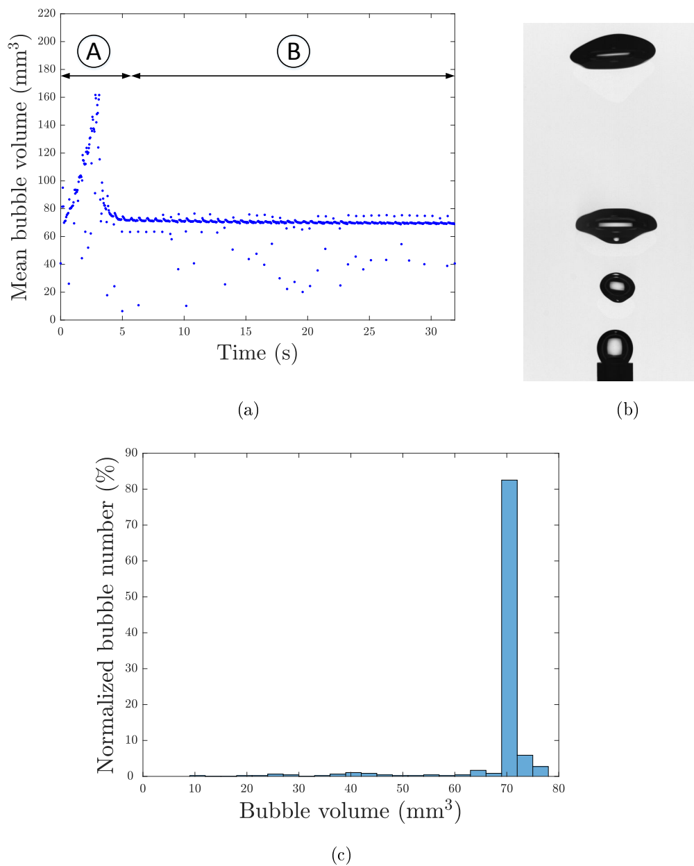
FIGURE 3.18: (a) the temporal distribution of bubble volume, (b) a small bubble occurred at t = 10.1 s at steady state, (c) histogram of bubble volume at steady state, bin width: 3 (VFC 1%).
