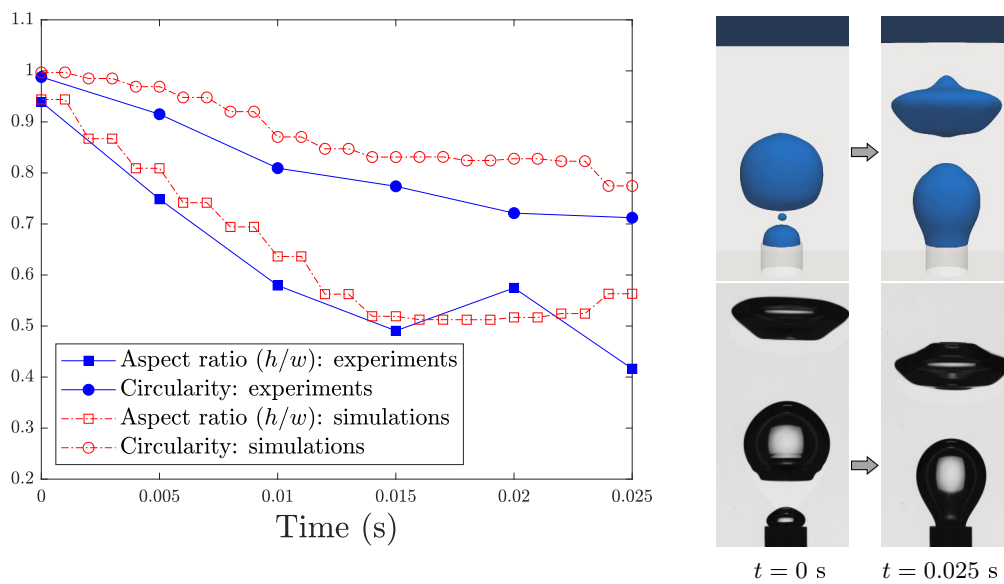
FIGURE 4.27: Evolution of bubble shape factors. The images have the same scale : 3 mm = 126 pixels. VFC: 9%.
