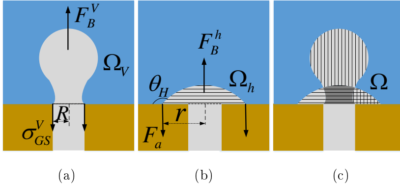
FIGURE 3.2: The method for calculating bubble volume. (a) \Omega_V is the maximum gas volume that can be supported by the vertical gas-solid interface. (b) During bubble spreading, \Omega_h is the gas volume that is held by the horizontal solid surface, its maximum value is \Omega_H = (\Omega_h)_{\max} . (c) The bubble volume is considered as a sum of the previous two maximum volumes. Noticing that the overlapping volume represented by the dark region appears twice in the total volume, thus the theoretical bubble volume is a little larger than the actual one.
