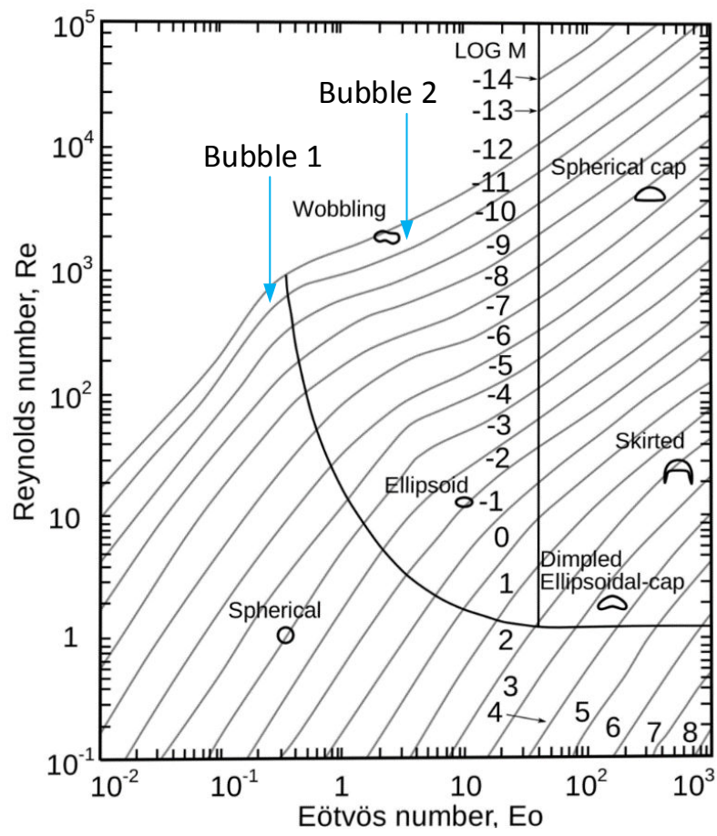
FIGURE 4.11: Shape regime map for bubbles and drops [166], illustration from [170].
