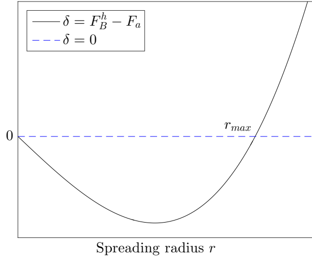
FIGURE 3.3: The difference between the buoyancy force F_B^h and the adhesive force F_a versus spreading radius r for the horizontal part. \delta = 0 indicates F_B^h = F_a , \delta < 0 indicates F_B^h < F_a . And r_{\max} is the maximum spreading radius.
