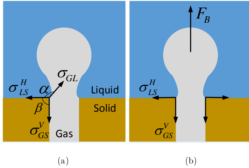
FIGURE 3.1: A bubble that does not spread beyond the orifice edge. (a) The three surface stresses \sigma act on the triple line located at the orifice edge. \alpha , \beta are the angles between the interfaces, and \beta is set to be \pi/2 . (b) The gas-liquid surface stress \sigma_{GL} does not appear in the forces acting on the bubble as a whole. The liquid-solid surface stress \sigma_{LS}^H pulls the bubble outwards and may make the bubble spread over the horizontal surface. The gas-solid surface stress \sigma_{GS}^V resists the buoyancy force F_B .
