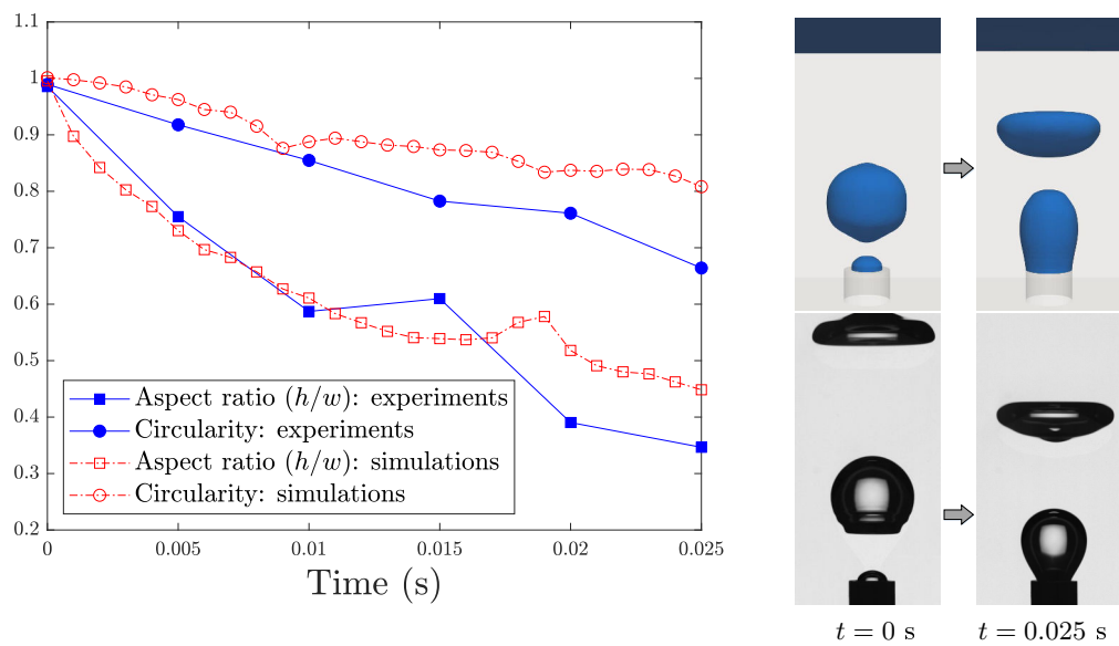
FIGURE 4.25: Evolution of bubble shape factors. The images have the same scale : 3 mm = 126 pixels. VFC: 3%.
