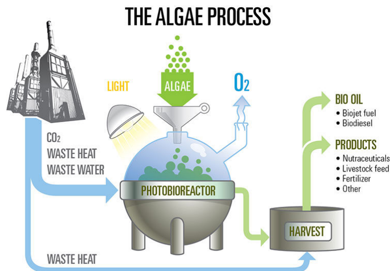
FIGURE 2.1: Illustration of Microalgae process from [26].
