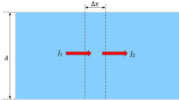
FIGURE 2.15: The volume element used to deduce Fick's second law of diffusion.
