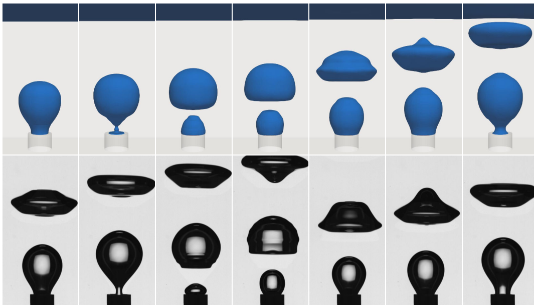
FIGURE 4.18: Comparison of bubble evolution in simulations and in experiments. Upper images are from simulations, lower images are from experiments, they have the same scale: 3 \text{ mm} = 126 \text{ pixels} . The nozzle diameter in simulations is the same as the one in experiments, i.e. 3 \text{ mm} . Time interval between images in upper and lower row is similar. VFC: 9%.
