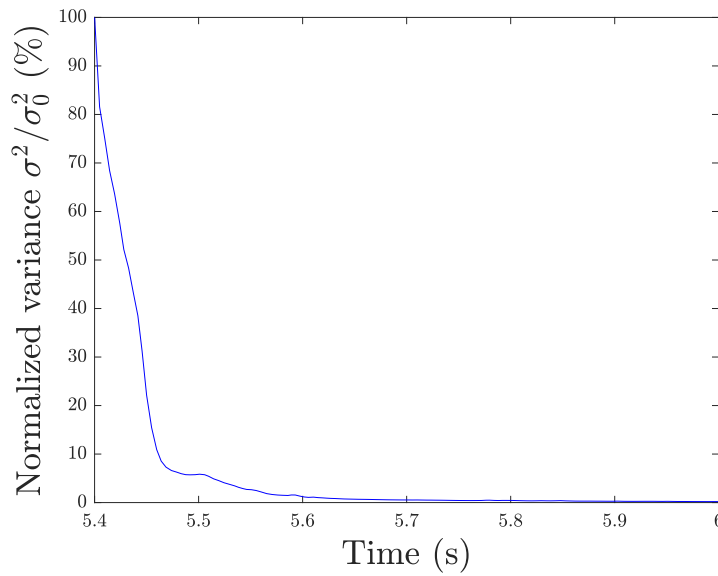
FIGURE 5.4: The evolution of normalized variance. The start time is the moment that tracer is injected, and the liquid already reaches quasi-steady state at that moment.
