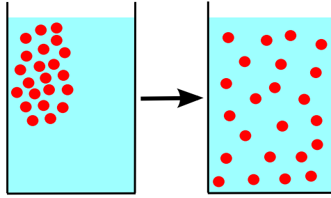
FIGURE 2.13: The process of diffusion, illustration from Wikipedia article Diffusion .
