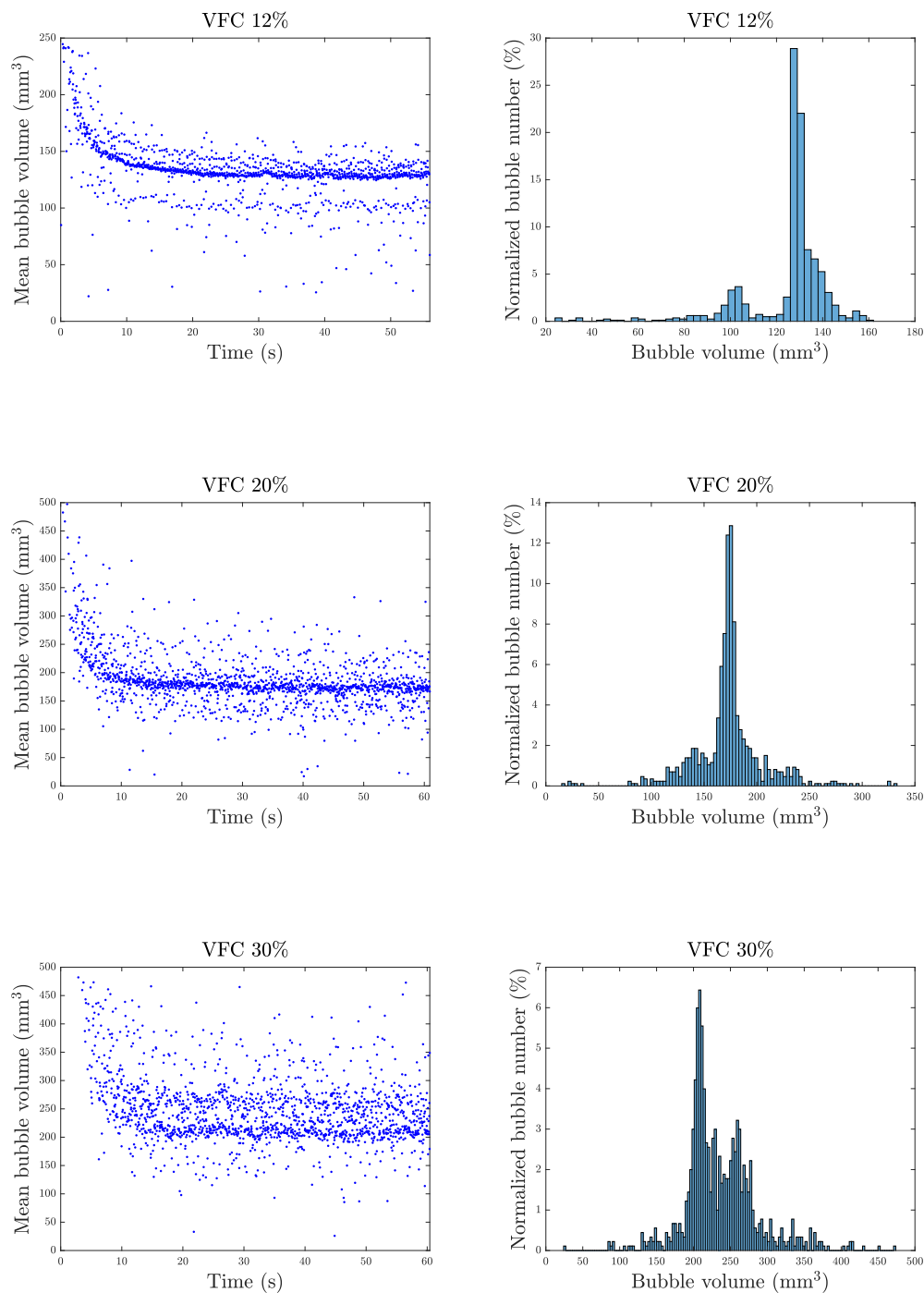
FIGURE 3.20: The temporal distribution (left column) and histogram (right column) of bubble volume at VFC 12%-30%, bin width: 3 .
