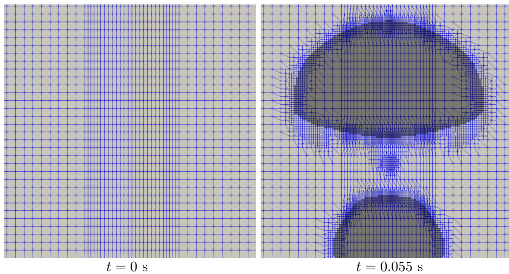
FIGURE 4.14: Dynamic mesh is “activated” as soon as the mesh meet the interface, illustration from simulation with VFC 3%.
