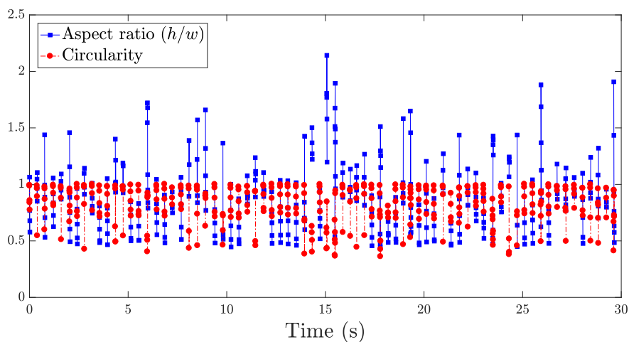
FIGURE 3.24: The evolution of aspect ratio and circularity of a population of bubbles at steady state (VFC 30%).
