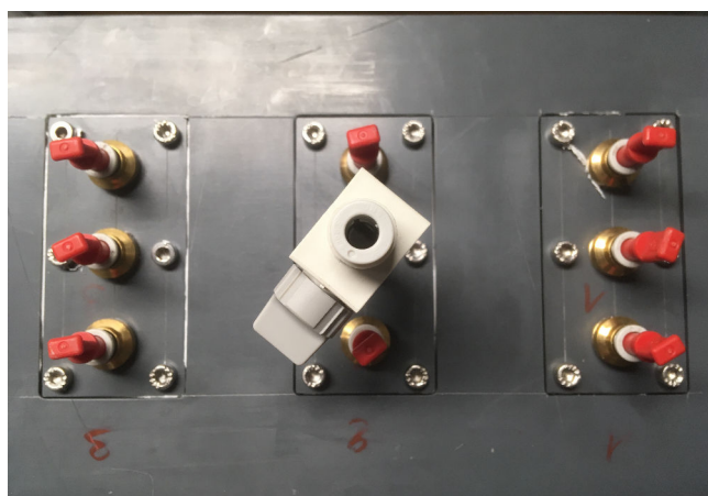
FIGURE 3.9: The 9 nozzles at the bottom of the reactor (the side connecting with gas source).
