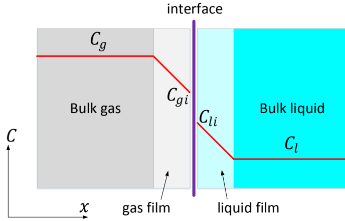
FIGURE 2.17: Two film model: films exist in both phases.
