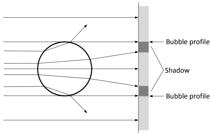
FIGURE 3.7: An annular-like shadow is formed on the recording plane when a light beam traveling in liquid meet a gas bubble due to the refraction.
