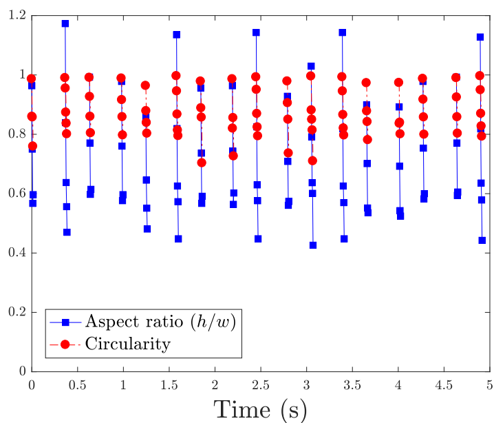
FIGURE 3.23: The evolution of aspect ratio and circularity of a population of bubbles at steady state (VFC 1%).
