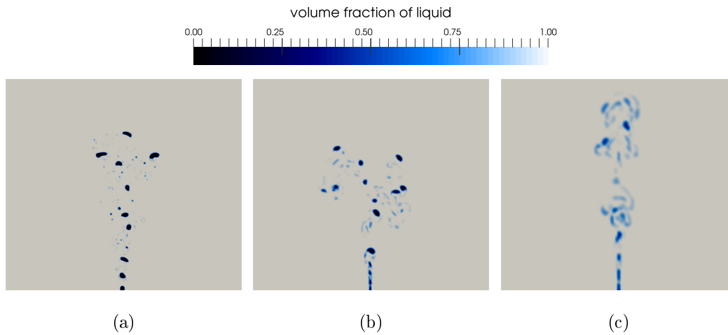
FIGURE 4.9: 2D simulations with different mesh sizes, at physical time t = 1 s. (a) \Delta x = 0.25d_s , (b) \Delta x = 0.5d_s , (c) \Delta x = d_s . d_s is the inner diameter of the sparger. (Scale: width of the numerical domain is 286 mm.)
