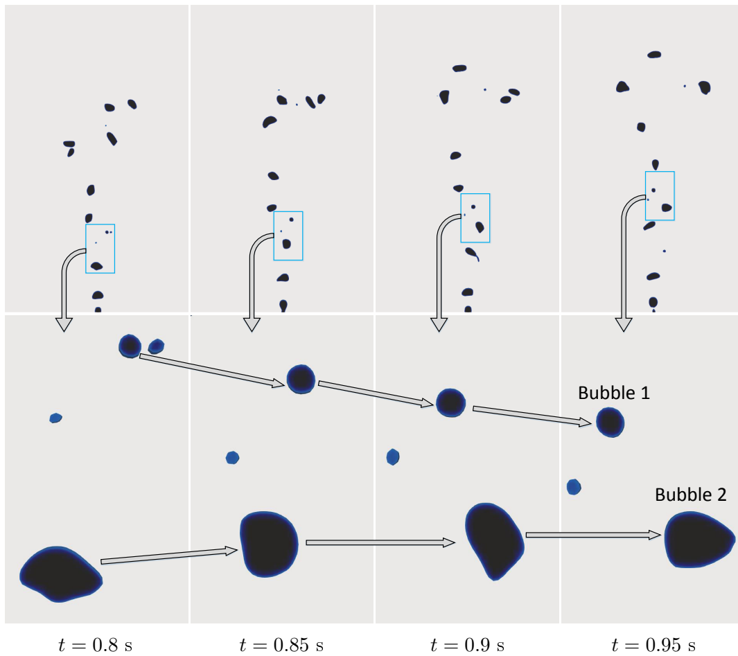
FIGURE 4.10: Two bubbles in different shape regime. Conditions: Co_{\max} = 0.75 , \Delta x = 0.5 mm, injecting gas velocity v_g = 0.2 m/s. The equivalent diameter d_1 \approx 1.5 mm, d_2 \approx 4.5 mm.
