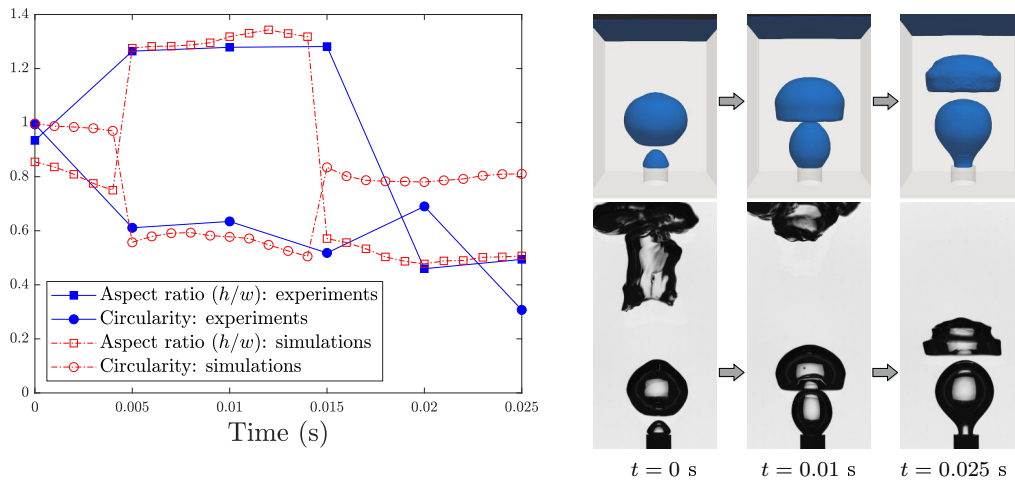
FIGURE 4.30: Evolution of bubble shape factors. The images have the same scale : 3 mm = 80 pixels. VFC: 30%.
