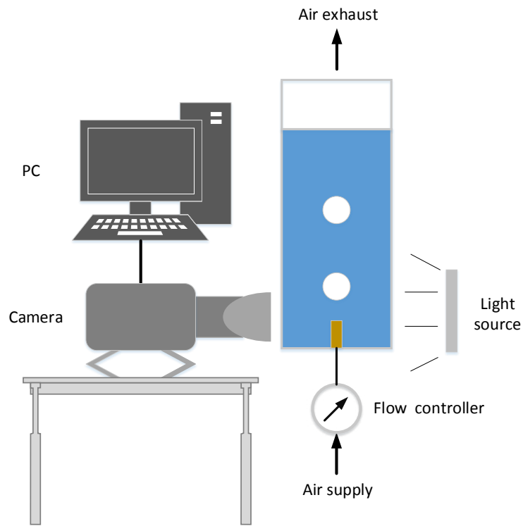
FIGURE 3.8: Schematic sketch of the experimental setup.
