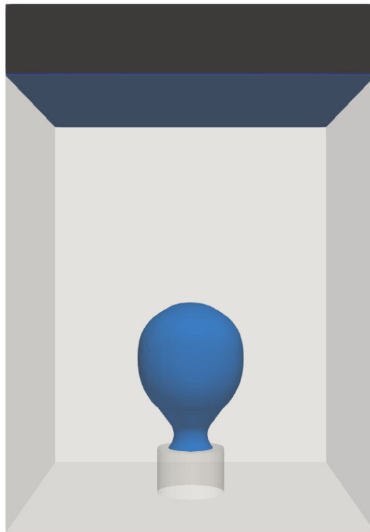
FIGURE 4.12: The mini-reactor in 3D simulations. (Numerical domain: 14 \times 14 \times 20 mm, exterior diameter of the nozzle: 3 mm.)
