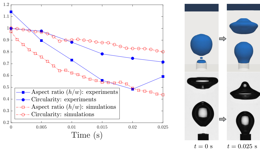
FIGURE 4.28: Evolution of bubble shape factors. The images have the same scale : 3 mm = 126 pixels. VFC: 12%.
