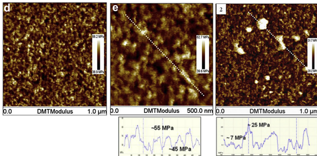
Figure 1.27 – DMT modulus maps of a PU surface containing 50% of soft segments; (d) 1 \times 1 \mu\text{m}^2 ; (e) 500 \times 500 \text{ nm}^2 ) scans with section analysis profile taken along the white dashed line. (2) Similar 1 \times 1 \mu\text{m}^2 modulus image with profile for a PU containing 70% of soft segments. [111].
