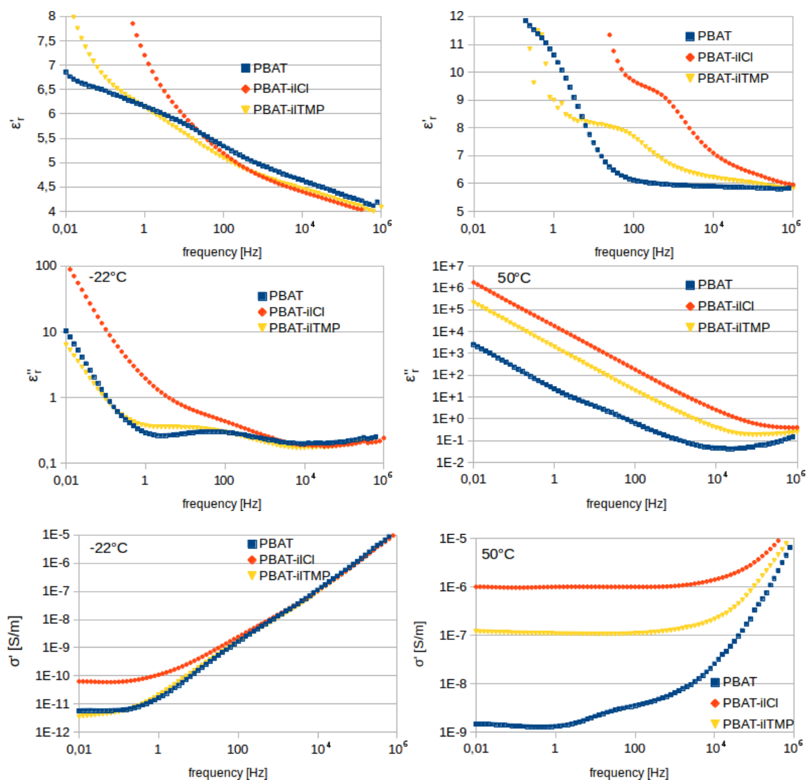
Figure 4.6 – Relative dielectric permittivity (top), loss (middle) and real conductivity (bottom) versus frequency, at -22°C (left) evidencing the \alpha relaxation around 100 Hz and at 50°C (right) showing conduction and the \alpha' relaxation. The latter corresponds to the conductivity step around 100 Hz for PBAT, and is overlapped by the conduction for the other blends (It corresponds anyway to the steps in \epsilon_r' and could be fitted properly).
