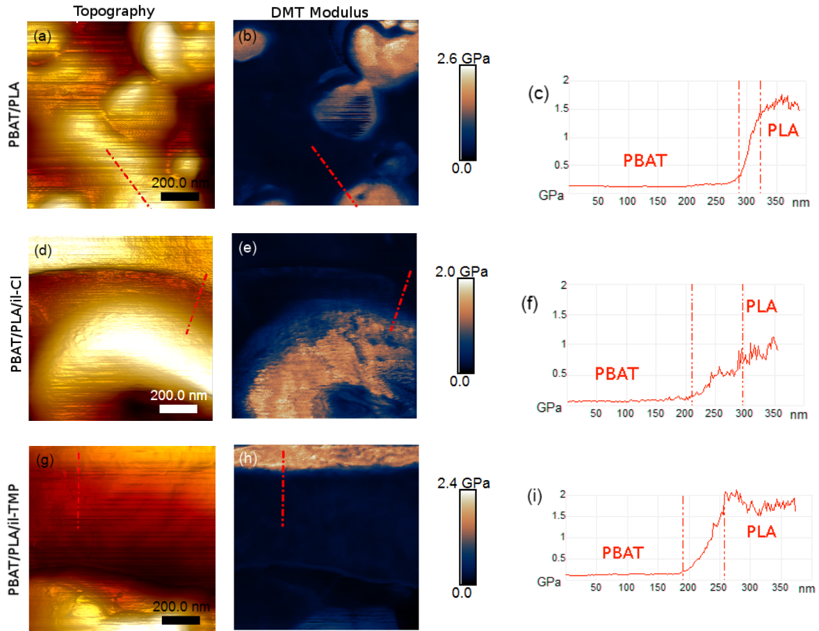
Figure 3.8 – AFM 1 × 1 μm 2 topography (left) and DMT modulus (center) images with corresponding modulus profiles for PBAT/PLA : (a), (b) and (c); PBAT/PLA/il-Cl : (d), (e) and (f); PBAT/PLA/il-TMP : (g), (h) and (i). The modulus profile are taken following the red dashed line in (b), (e) and (h).
