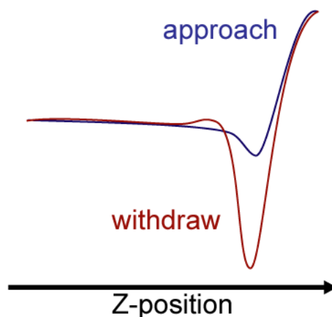
Figure 1.10 – Typical force curve: approach (blue) and withdraw (red) versus piezo Z (vertical) position. Source: Peak Force QNM User Guide [43].
