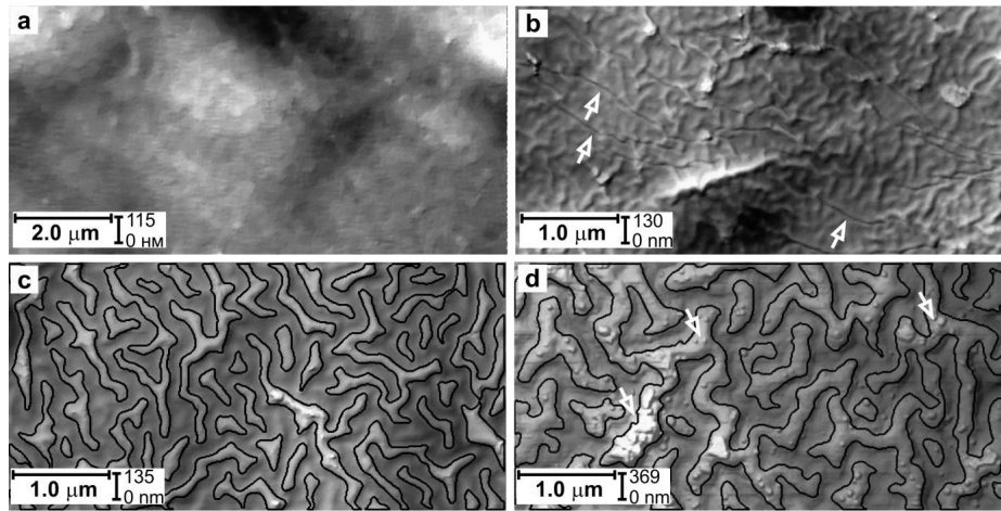
Figure 1.26 – AFM height images of PU: (a) – untreated PU; after plasma immersion N_2^+ ion implantation: (b) - 2 \cdot 10^{15} ions/cm 2 ; (c) - 2 \cdot 10^{16} ions/cm 2 ; (d) - 2 \cdot 10^{17} ions/cm 2 . In (c) and (d) the fractal structure is evidenced by black lines of constant height [105].
