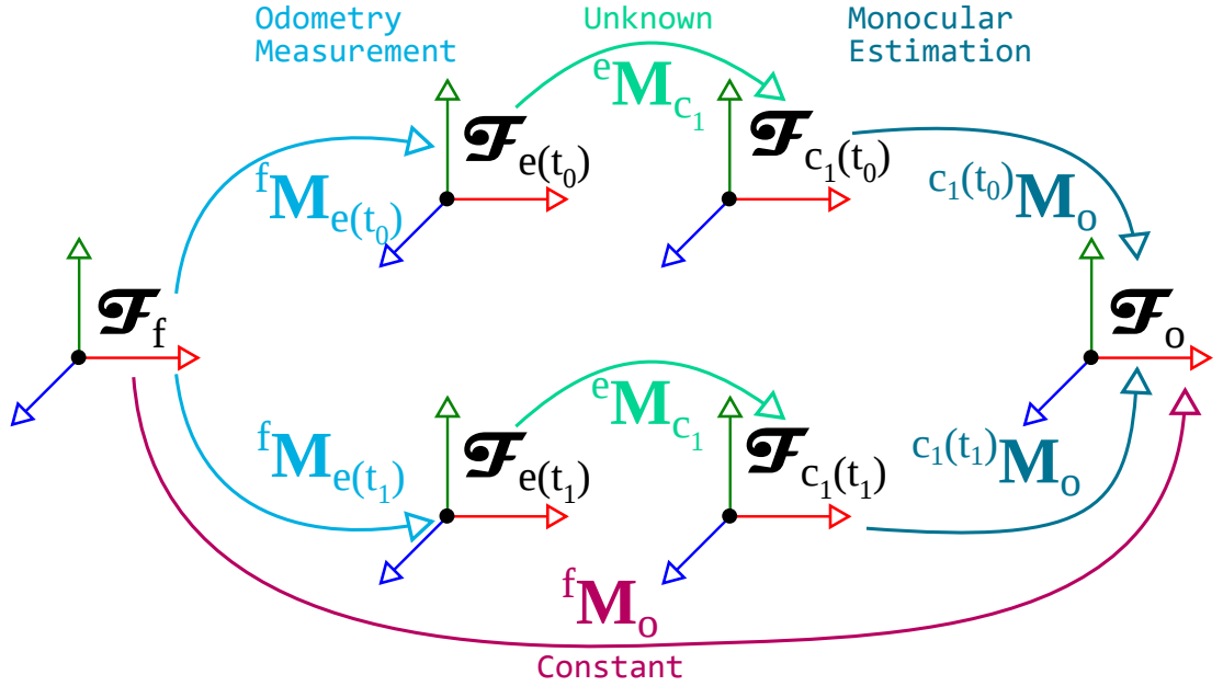
Figure 4.12 – Frame configuration for controlled camera calibration with 2 camera positions (in practice 4 positions were used). The only unknown matrix is e\mathbf{M}_{c_1} and its estimated thanks to the other matrices that are known.
