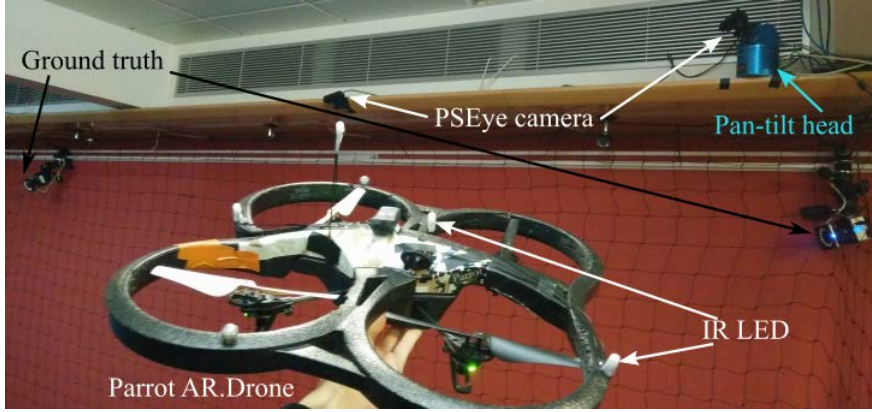
Figure 4.20 – Our optical tracking approach for UAV localization and for comparison with Vicon's optical tracking system.
