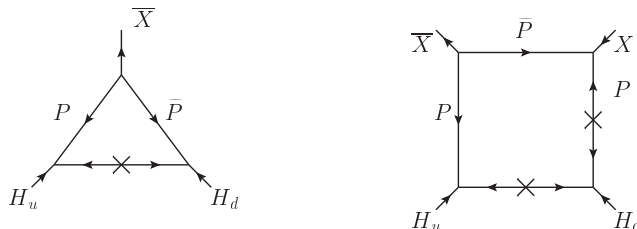
Figure 2.3: Left: Superfield graph inducing an effective \mu term at one loop. Right: Effective B\mu term which is also generated at one loop.
