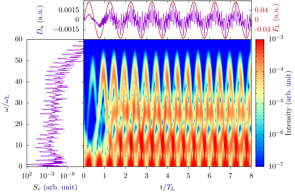
Figure II.7 Same as Figure II.6 with a trapezoidal laser pulse of 8 optical cycles with linear ramps of 1 optical cycle.
