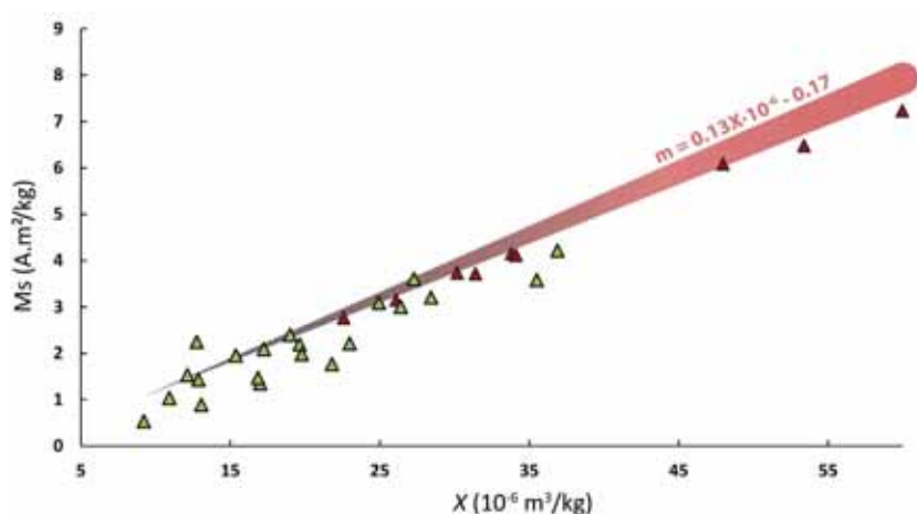
Fig. 10. Correlation between mass magnetic susceptibility ( \chi ) and saturation magnetization (Ms) for unaltered serpentinites (red) and hydrothermalized serpentinites (green). Relation between magnetite content ( m = M_{s_{sample}}/M_{s_{pure\ magnetite}} , 92 A.m 2 /kg; e.g. Oufi et al., 2002) and \chi is represented (in red). See data in Supplementary Material. (For interpretation of the references to colour in this figure legend, the reader is referred to the web version of this article.)
