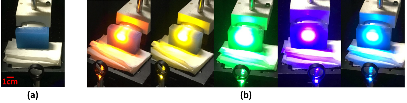
Figure 2.8: (a) Blue phantom in the set-up. (b) Blue phantom during the acquisition of the multispectral photoacoustic signals.
