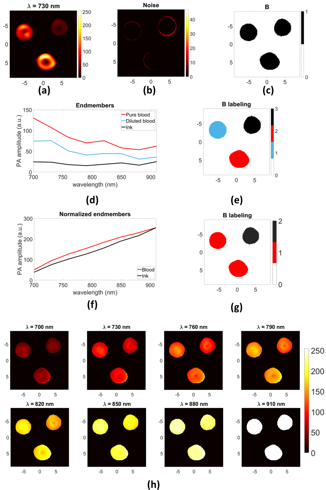
Figure 3.4: Pre-processings and endmembers calculation of Blood-Ink (PAT) dataset. (a) Photoacoustic image at 730 \text{ nm} . (b) Noise removed by the pre-processing threshold. (c) Binary mask \mathbf{B} , the pixels of interest are in black. (d) Endmembers. (e) Labeling of the binary mask \mathbf{B} which corresponds to the ground truth when no normalization is done. (f) Normalized endmembers. (g) Labeling of the binary mask \mathbf{B} when the normalization step is applied. (h) Normalized data. The image axes are in \text{mm} .
