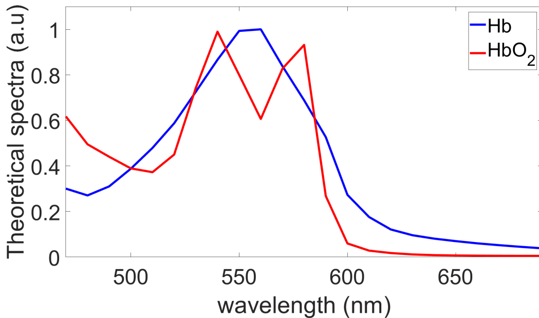
Figure 5.7: Theoretical multispectral absorption evolutions of Hb and HbO 2 used as endmembers in unmixing.
