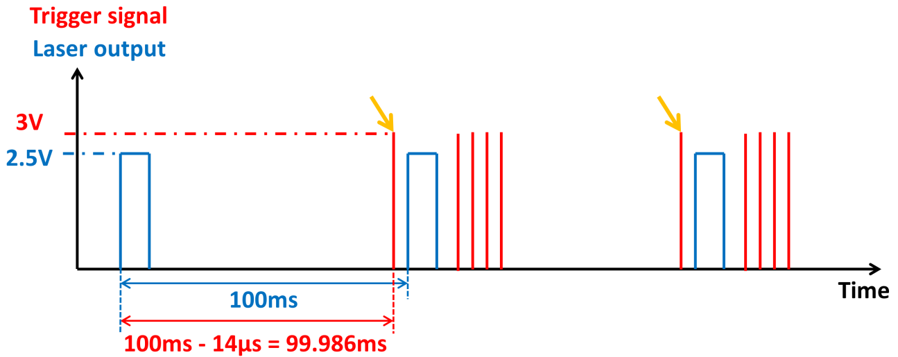
Figure 2.15: Scheme of the ULA-OP256 triggered by the laser pulse. The yellow arrows represent the trigger for passive acquisitions.
