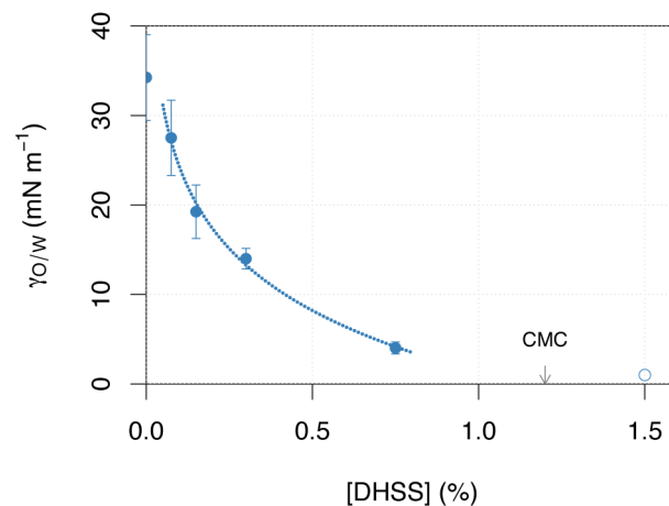
Figure 9.3: Variations of \gamma_{o/w} with DHSS concentration in lab-tests. The dotted line is the logarithmic fit of experimental data. \gamma_{o/w} could not be measured accurately for C_S=1.5\% .
