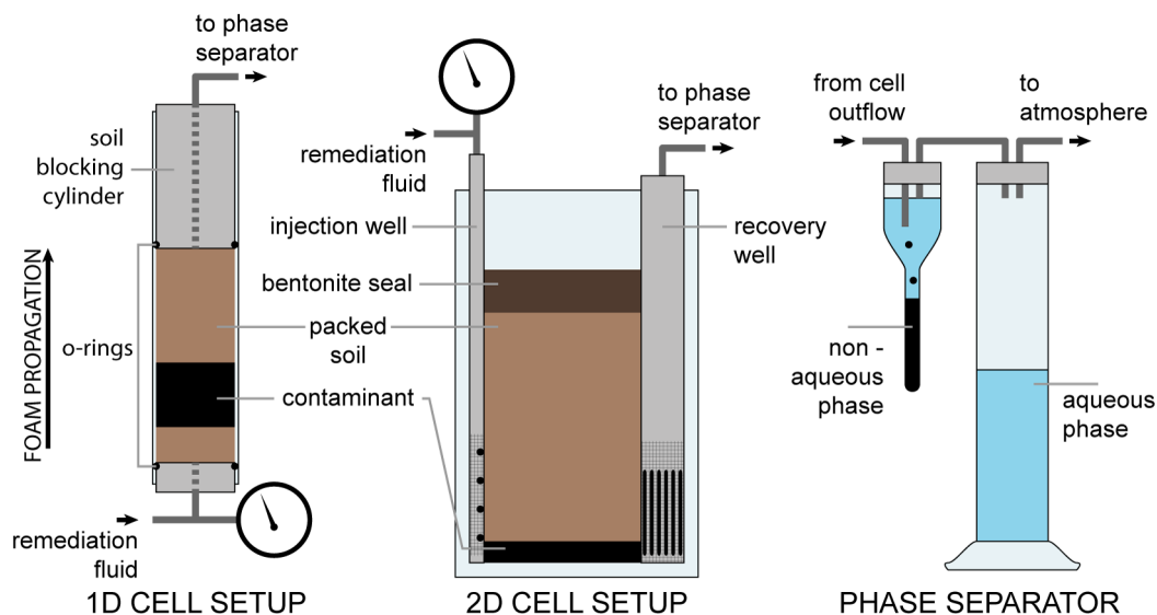
Figure 7.7: Experimental set-up for 1- and 2-D experiments. Contaminant extracted from soil was split whether it was solubilized or not using the phase separator.
