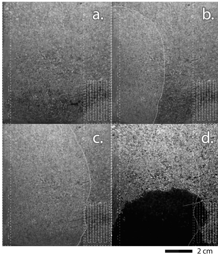
Figure 7.14: a., b., c.: Time lapse photographs (0, 30 and 60 min) of strong foam propagation during 2-D experiments in the presence of DNAPL (darker at the bottom) ( [\text{CAPB-SDS}] = 0.05\% , ex-situ foam, \text{FQ} = 75\% , Q_{\text{foam}} = 40 \text{ cm}^3 \text{ min}^{-1} ). d. Tracer diffusion showing how the solubilizing solution was distributed. Dashed structures are injection and recovery wells on the left and right respectively.
