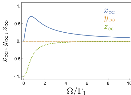
Figure 2.2: Evolution of the steady-state expectation values of \sigma_x (blue, plain), \sigma_y (orange, dashed) and \sigma_z (green, dotted) at zero detuning \delta = 0 with the Rabi drive amplitude \Omega (in unit of \Gamma_1 ) for \Gamma_\varphi = 0 .
