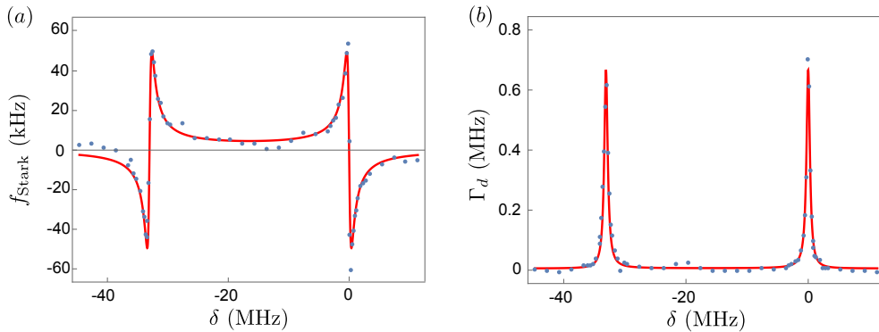
Figure 7.3: a) AC-Stark shift and (b) measurement-induced dephasing of the qubit when the cavity is weakly driven at f_D + \delta so that \alpha_{e,g} \approx 0.5 on resonance (see text). Points are experimental data and solid lines are theoretical evolutions given by Eq. (B.3) and Eq. (B.4) respectively, with \chi - \chi_2 = 33.1 MHz and \kappa/2\pi = 0.77 MHz.
