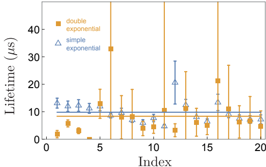
Figure 5.2: Lifetime fluctuations. Evolution of (orange squares) the short decay time T_s for a double exponential fit and (blue triangles) the decay time T_1 for a single exponential fit of the energy decay measurements of the qubit transition with the index of the experiment (related to the time). The duration of the total measurement is about an hour. The mean values of T_s and T_1 are represented by respectively the orange and blue lines.
