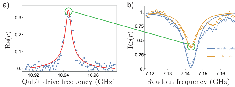
Figure 4.10: Qubit two-tone spectroscopy of fluxonium A. a) Evolution of the real part of the reflection coefficient measured at the readout frequency with the qubit drive frequency, (points) experimental data and (line) theoretical lorentzian response. b) Readout spectroscopy preceded (orange) or not (blue) by a qubit pulse, (point) experiment and (line) theory from Eq. (4.8) with p_0 = 0.96 (blue) and p_0 = 0.62 (orange).
