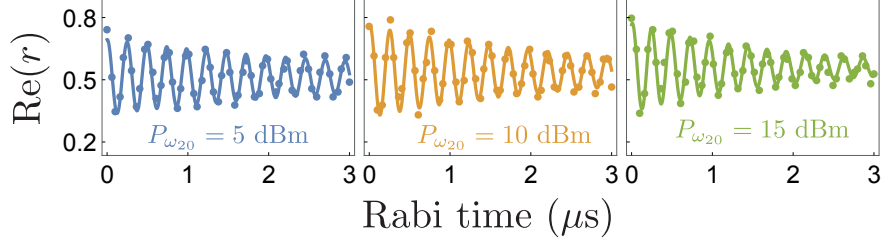
Figure 5.13: Rabi oscillations between |0\rangle and |1\rangle after qubit initialization using a pump on |0\rangle \rightarrow |2\rangle for various values of the pump power (see insets).
