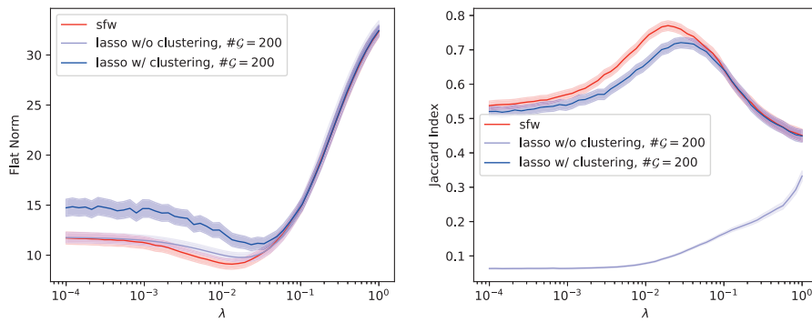
Figure 4.11: Performance comparison in terms of Flat Norm and Jaccard index of FISTA (with 10^4 iterations) with and without clustering. The area around the curves correspond to a 95% confidence interval.
