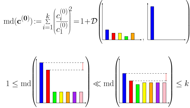
FIGURE 6. A visual representation of the monochromatic distance. At the extremes, when there are only O(1) opinion communities of size \Theta(c_1) , we have \mathbf{md} = \Theta(1) while, when \Theta(k) opinion communities have size \Theta(n/k) , we have \mathbf{md} = \Theta(k) .
