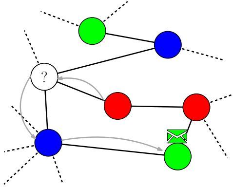
FIGURE 22. A representation of the first phase of the adaptation of the Undecided-State dynamics on expander graphs, in which each node sends a token performing a random walk of at least \bar{t} -hops and thus sampling the opinion of a random node.
