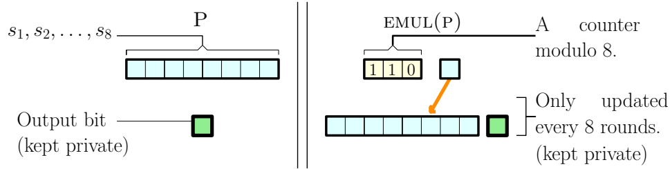
FIGURE 27. On the left is a protocol \Psi using \ell = 8 bits in total and pulling only one node per round ( \eta = 1 ). On the right is the emulated version \text{EMUL}(\Psi) which uses 4 bits only. The bits depicted on the bottom of each panel are kept privately, while the bits on the top are public, that is, appear in the visible part.
