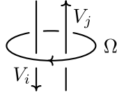
FIGURE 3. Modularity condition.
