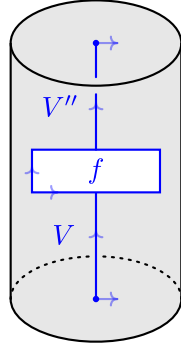
FIGURE 11. The \mathcal{C} -colored ribbon graph T_{D^2 \times I}^f inside D^2 \times I .
