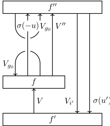
FIGURE 28. The admissible \mathcal{C} -colored closed ribbon graph T_Y^{\varphi_{f, f', f''}} .
