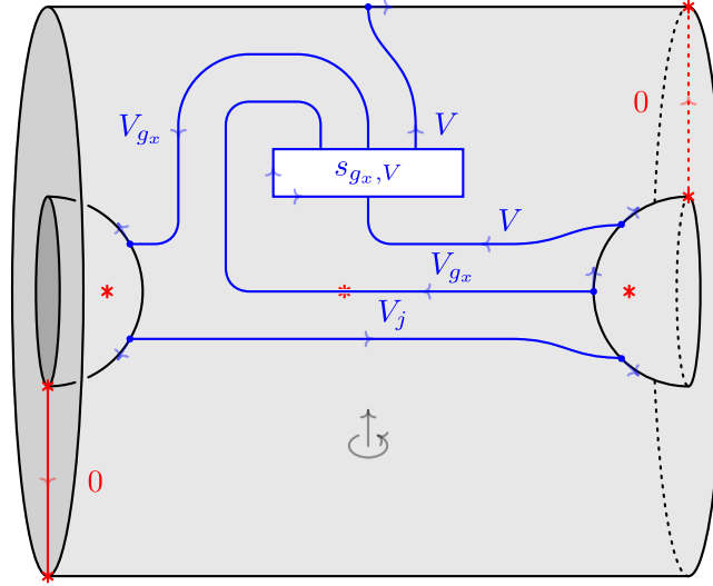
FIGURE 36. The 2-morphism \mathbf{X}_{j, V} of \check{\mathbf{Cob}}_3^{\mathcal{C}} .
