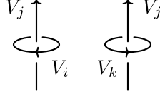
FIGURE 6. The \mathcal{C} -colored ribbon tangles representing f_{ij}^- and f_{jk}^+ .
