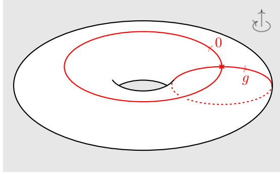
FIGURE 10. The 2-morphism \mathbf{B}_{2,g} . The cohomology class \omega_{\mathbf{b}_{2,g}} is completely determined by \vartheta_{2,g} .
