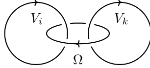
FIGURE 7. The \mathcal{C} -colored framed link representing M_{ik} .
