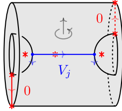
FIGURE 40. The 2-morphism \mathbf{X}_j of \check{\mathbf{Cob}}_3^{\mathcal{C}} .
