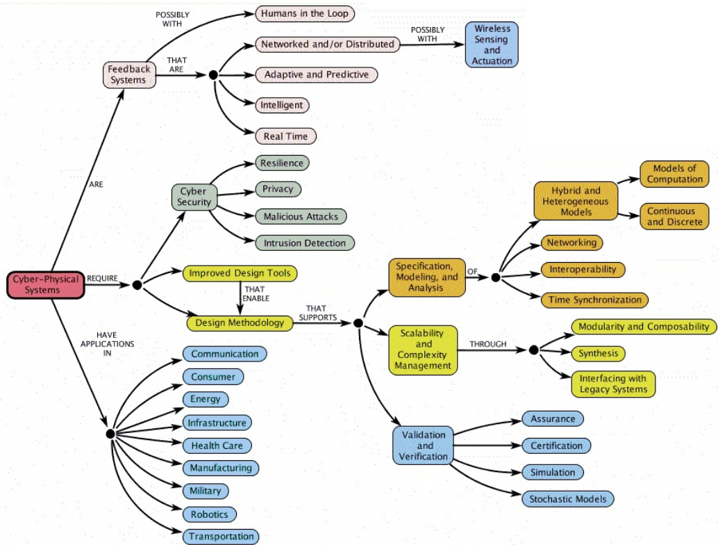
Figure 1.1: Cyber-physical systems - a Concept Map. Image made by Edward A. Lee after a taxonomy given by S. Shyam Sunder [Lee, Edward Ashford, 2012].
