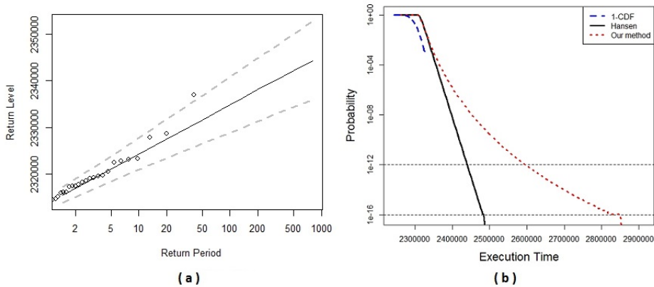
Figure 4.11: Comparison with Hansen’s work: (a) return level plot for Hansen’s method, (b) our pWCET estimation (in red) against the estimation obtained according to adversary method.
