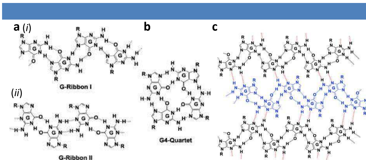
Figure 20 | (a, b). Guanine-containing molecules can form a variety of different self-assembled motifs, including (i) G-ribbon I, (ii) G-ribbon II and (b) the G4-quartet. (c). These ribbons (middle ribbon is blue for differentiation) are stabilized through additional inter-tape hydrogen bonds (shown in red). Reproduced from reference 94.
