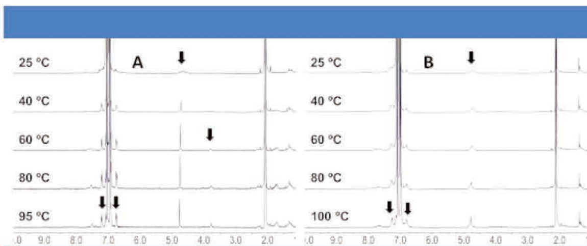
Figure S12 | Variable-temperature ^1\text{H} NMR spectra of TAMG in the absence (A) and in the presence (B) of \text{KPF}_6 (4 mM solution in toluene).
