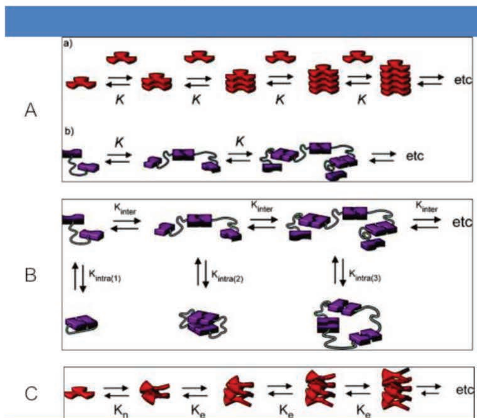
Figure 7 | Schematic representation of A. an isodesmic supramolecular polymerization of a) a rigid discotic molecule into a linear supramolecular polymer and b) a bifunctional monomer in which the two binding groups are connected via a flexible spacer; B. a ring-chain supramolecular polymerization and C. a cooperative ( K_n < K_e ) supramolecular polymerization of a rigid discotic molecule. Reproduced from reference 36 .
