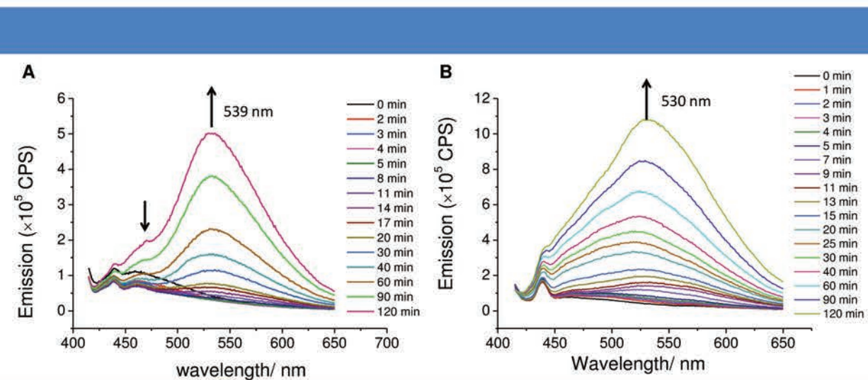
Figure 42 | A. Fluorescence spectra of TAMG for increasing irradiation times ( c = 0.1 mM in chloroform, \lambda_{exc.} = 400 nm). B. Fluorescence spectra of TATT for increasing irradiation times ( c = 0.1 mM in a 5:3 mixture of toluene/methanol with 10 vol% chloroform, \lambda_{exc.} = 400 nm).
