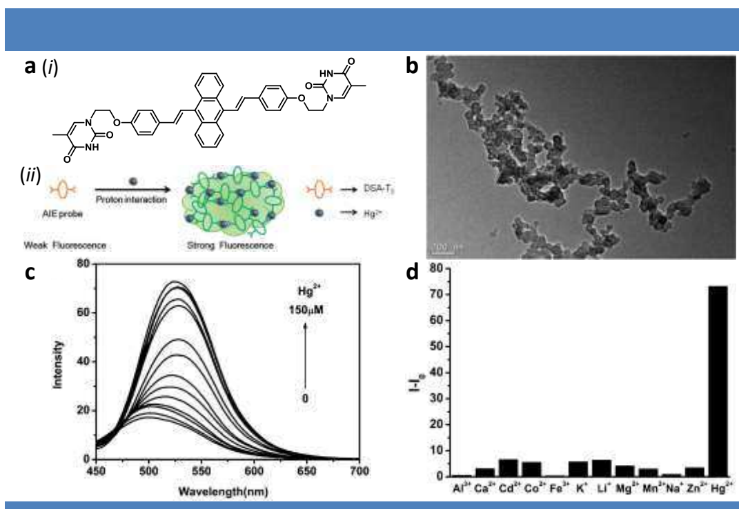
Figure 28 | a. (i) Molecular structure of the distyrylanthracene (DSA-T 2 ) derivative and (ii) design rationale for the \text{Hg}^{2+} chemosensor. b. TEM image of DSA-T 2 ( 1.16 \times 10^{-5} M) in \text{CH}_3\text{CN-H}_2\text{O} (3 : 2, v/v) after addition of \text{Hg}(\text{NO}_3)_2 ( 1 \times 10^{-4} M). c. Fluorescence spectra of DSA-T 2 ( 1.16 \times 10^{-5} M) in \text{CH}_3\text{CN-H}_2\text{O} (3 : 2, v/v) with increasing amounts of \text{Hg}^{2+} , \lambda_{\text{ex}} = 420 nm. d. Normalized fluorescence intensity ( I_{521\text{nm}} ) of DSA-T 2 ( 1.16 \times 10^{-5} M) in \text{CH}_3\text{CN-H}_2\text{O} (3 : 2, v/v) in the presence of different metal ions ( 7 \times 10^{-5} M). Reproduced from reference 151.
