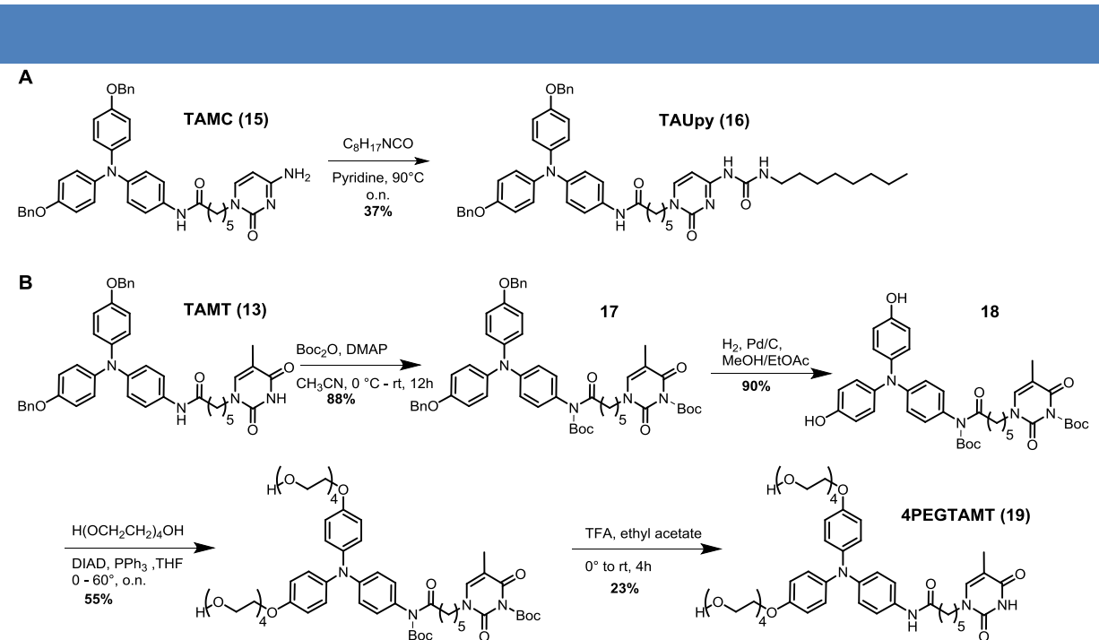
Scheme 2 | Synthesis of A) monotriarylamine-ureidopyrimidinone derivative TAUPy ( 16 ) and B)
