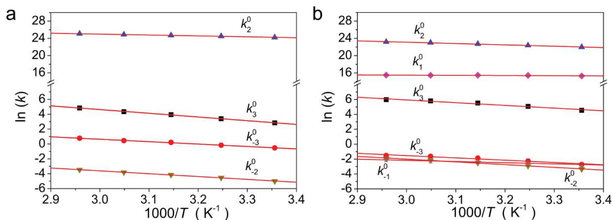
Fig. 3.22 Arrhenius plots of the calculated rate constants for the Volmer ( k_{\pm 3}^0 ), Heyrovsky ( k_{\pm 2}^0 ) and Tafel ( k_{\pm 1}^0 ) elementary steps versus reciprocal temperature for (a) non-activated and (b) EC activated Ni rod.
