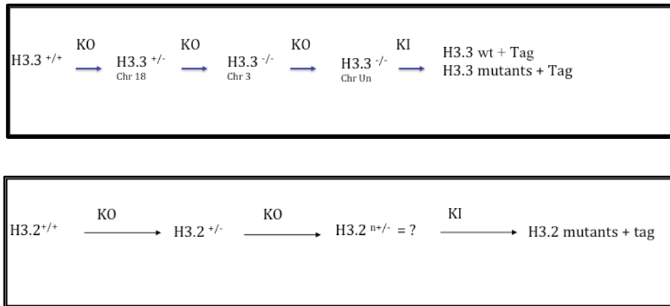
Figure 3.1.1: Strategy for establishing a H3.3 mutant system (upper panel) and H3.2 mutant system (lower panel) using DT40 cell line. H3.2 n+/- is the H3.2 KO clone where ‘n’ represents the minimum number of H3.2 copies with which the DT40 cells will survive.
