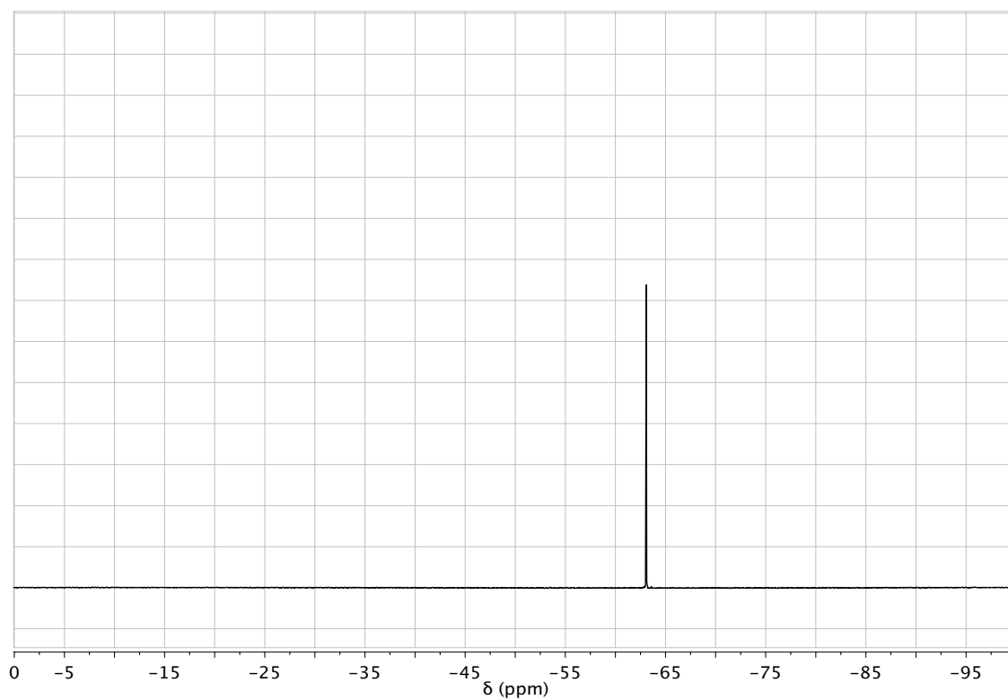
Figure S4b. 19 F NMR spectrum of compound 17 (CD 2 Cl 2 , 376 MHz).
