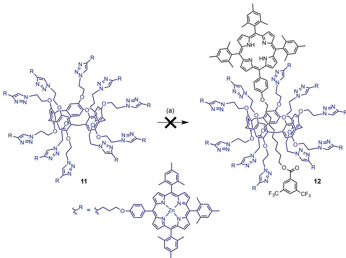
Scheme 2. Attempted preparation of compound 12 from Zn(II)-porphyrin-substituted pillar[5]arene 11 . Reagents and conditions: (a) 6 , 8 , CHCl 3 , Et 3 N, -15°C to rt.
