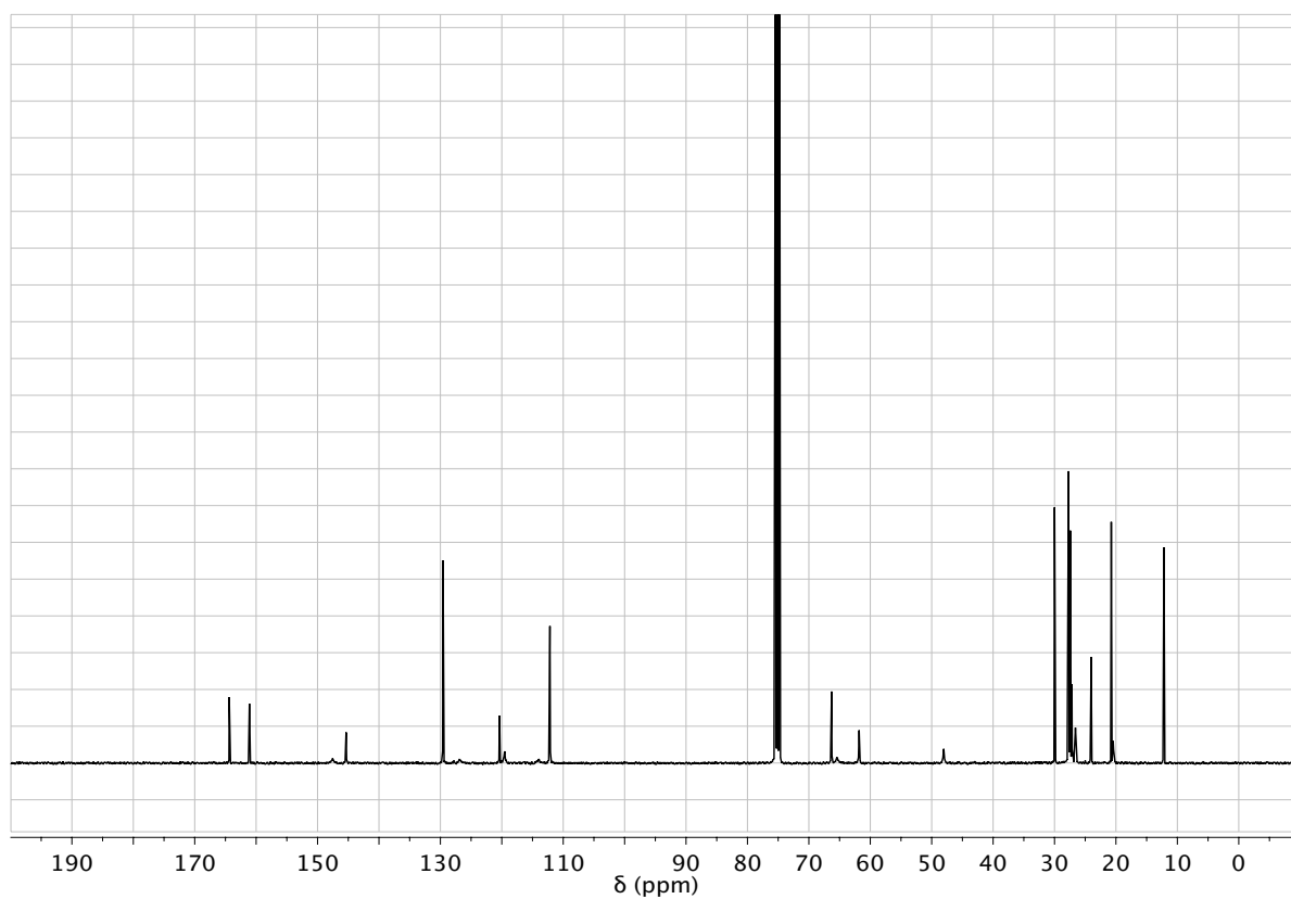
Figure S3b. ^{13}\text{C} NMR spectrum of compound 9 ( \text{CDCl}_3 , 100 MHz).
