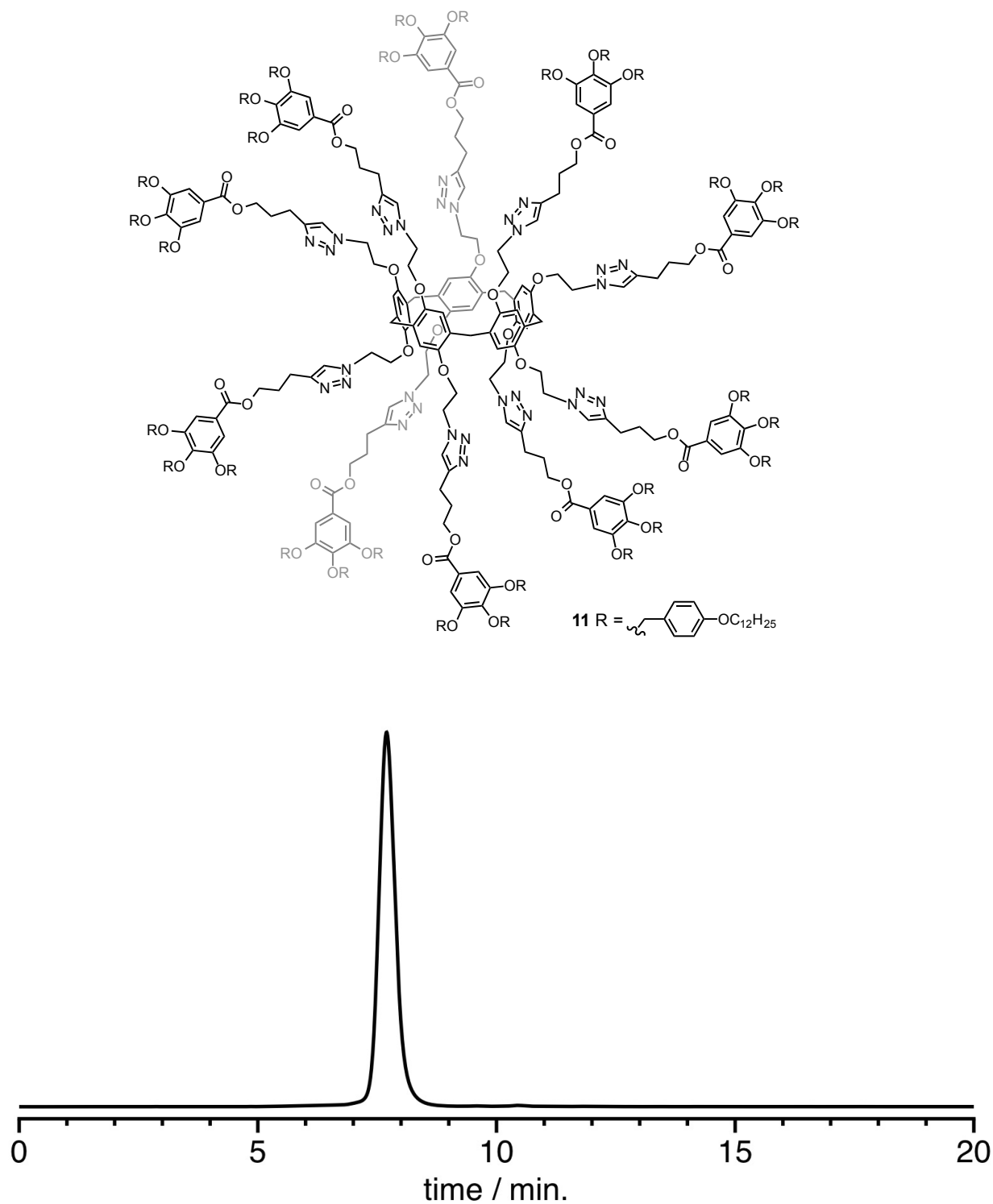
Figure S4e. HPLC trace on a size exclusion column (PLgel, \text{CH}_2\text{Cl}_2 , UV detector at \lambda = 254 nm) obtained for compound 11 .
