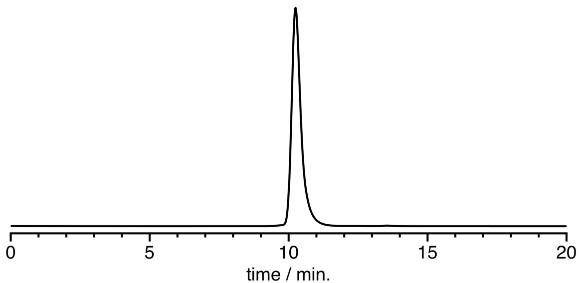
Figure S1f. HPLC trace on a size exclusion column (PLgel, CH 2 Cl 2 , UV detector at \lambda = 254 nm) obtained for compound 3 .
