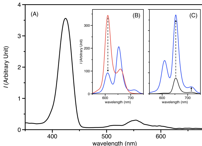
Figure 5. (A) Excitation spectrum recorded for compound 12 in toluene ( \lambda_{em} = 720 nm). (B) Emission spectra of isoabsorbing solutions of compounds 11 (red) and 12 (blue) in toluene ( 25^\circ\text{C} , \lambda_{exc} = 425 nm). (C) Emission spectra of compounds 9 (black) and 12 (blue) in toluene ( 25^\circ\text{C} , \lambda_{exc} = 425 nm), the concentration of the two solutions are identical.
