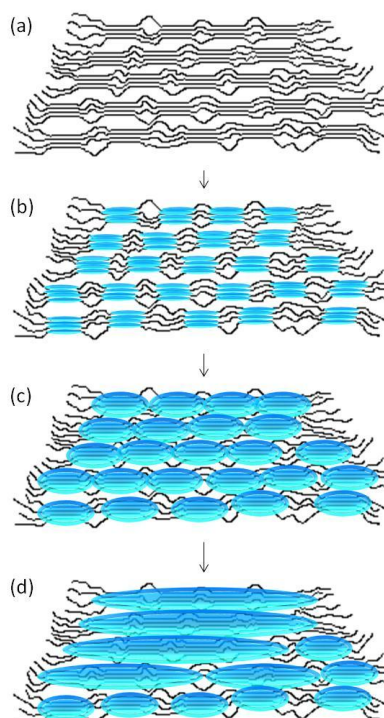
Figure 13: A “bipolaron network”. (a) A semicrystalline doped polymer, where bipolarons are the charge carriers. (b) The same polymer depicted with the \pi -orbitals of the individual doped conjugated chains (in blue). The \pi -orbitals of the various chains recombine (c), extending the \pi -system. Finally, due to the high crystallinity of the doped chains, the various \pi -orbitals overlap, resulting in a much wider \pi -system (d), a bipolaron network. 21,35
