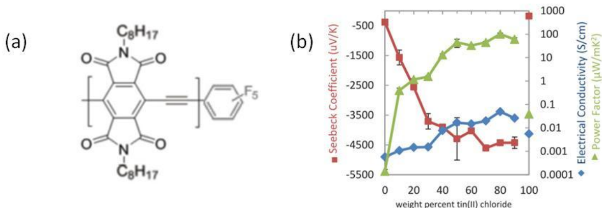
Figure 14: (a) The pyromellitic polymer used by Ireland et al. (b) the resulting Seebeck coefficient, electrical conductivity and Power Factor versus the SnCl 2 weight percent. 52
