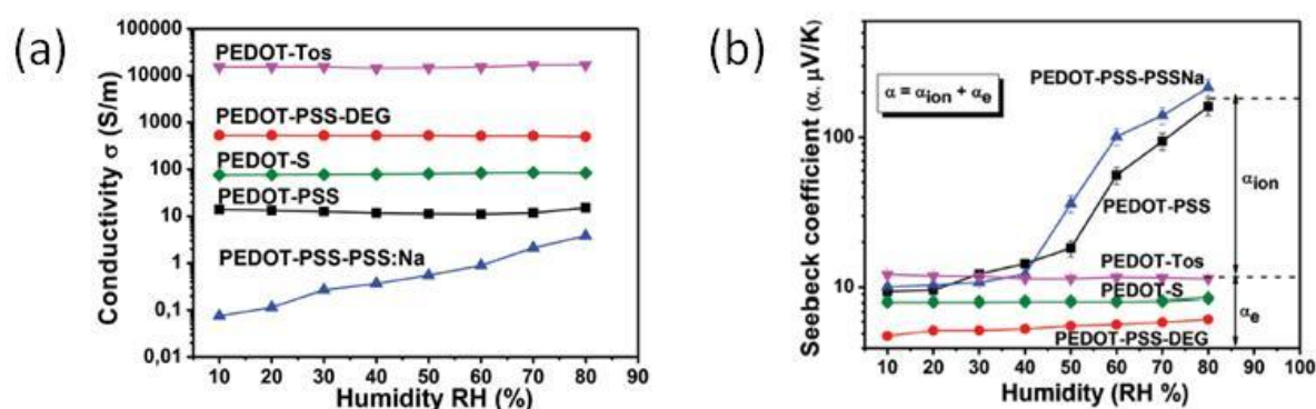
Figure 10: (a) Electrical conductivity and (b) Seebeck coefficient plotted against humidity. 36
