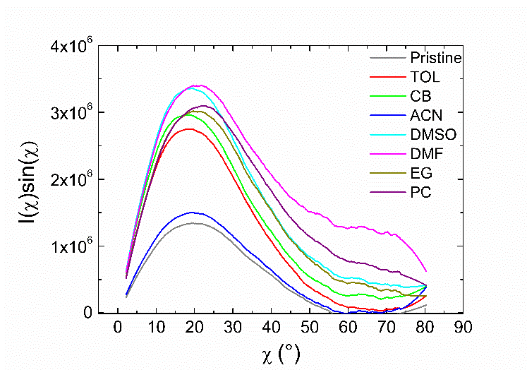
Figure 10. I(\chi)\sin(\chi) vs \chi plots for the (100) peak of the various PEDOT:Tos thin films. The area of the I(\chi)\sin(\chi) vs \chi plots for the (100) peak was subsequently used as a measure of the relative crystallinity considering the PEDOT films as “in-plane powders” (i.e. isotropic in-plane orientation of the crystallites). Additionally an estimation of the edge-on fraction is possible through this plot. Given that I(\chi)\sin(\chi) plot represents the orientation distribution function of the (100) crystallites and considering that edge-on crystallites are oriented with a \chi between 0^\circ and 45^\circ , the fraction of edge-on oriented crystallites can be estimated from the ratio between the I(\chi)\sin(\chi) vs \chi integral from 0^\circ to 45^\circ and the one from 0^\circ to 90^\circ .
