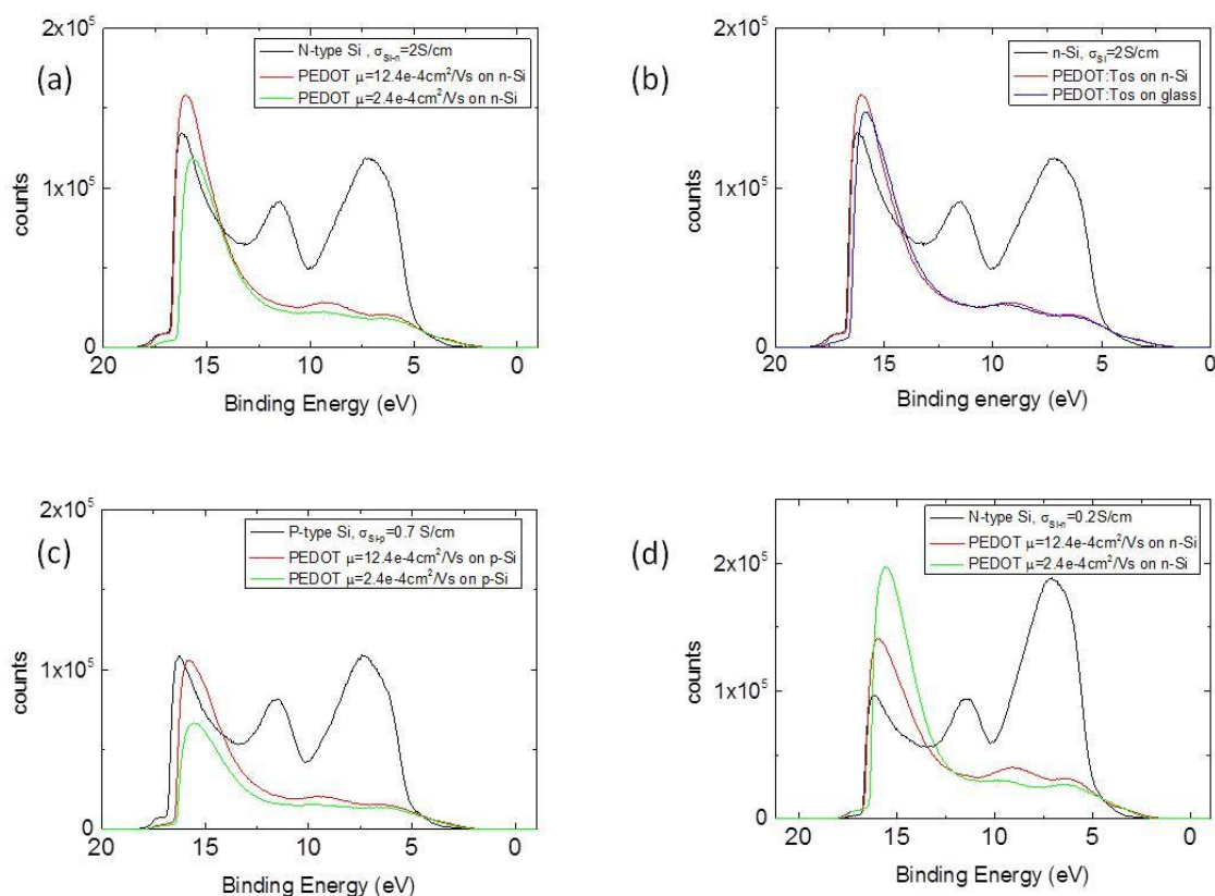
Figure 5: The UPS spectra of the PEDOT:Tos samples on the Silicon substrates with n-doping and \sigma_{Si}=2S/cm (a) and comparatively for PEDOT:Tos ( \mu=12.4 \times 10^{-4} \text{ cm}^2/Vs ) on glass (b) , p-doping and \sigma_{Si}=0.7S/cm (c) and n-doping and \sigma_{Si}=0.2S/cm (d)
