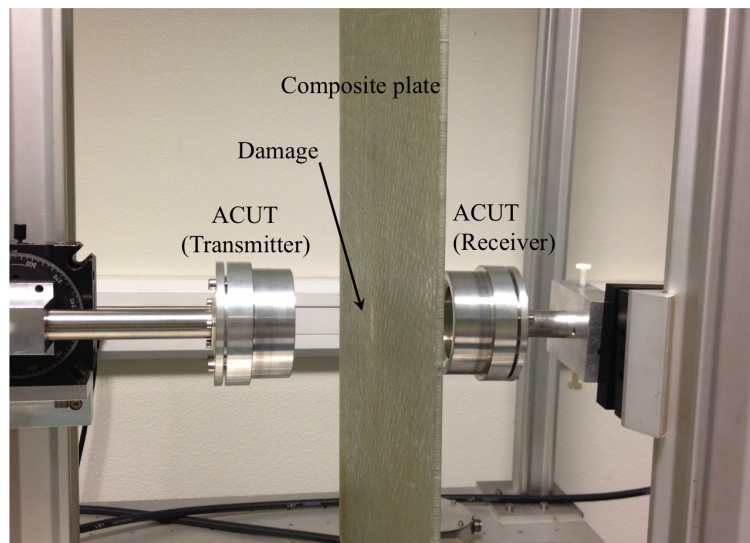
Figure 4.3. Photography of experimental setup: transmitting ACUT, receiving ACUT and composite plate placed between them.
