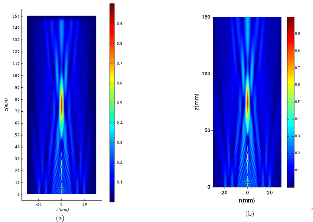
Figure 1.11. Calculated acoustic pressure distribution produced by 3-element annular air-coupled transducer, the elements include centre circular element N°1: r = 9\text{mm} ; annular elements N°2: with inner radius r_{in} = 12\text{mm} and outer radius r_{ou} = 15\text{mm} and N°3: r_{in} = 18\text{mm} and r_{ou} = 21\text{mm} . (a): Axisymmetric acoustic pressure calculated with FEM; (b): Axisymmetric acoustic pressure calculated with KIM. The acoustic pressure amplitudes are normalized for comparison between both methods.
