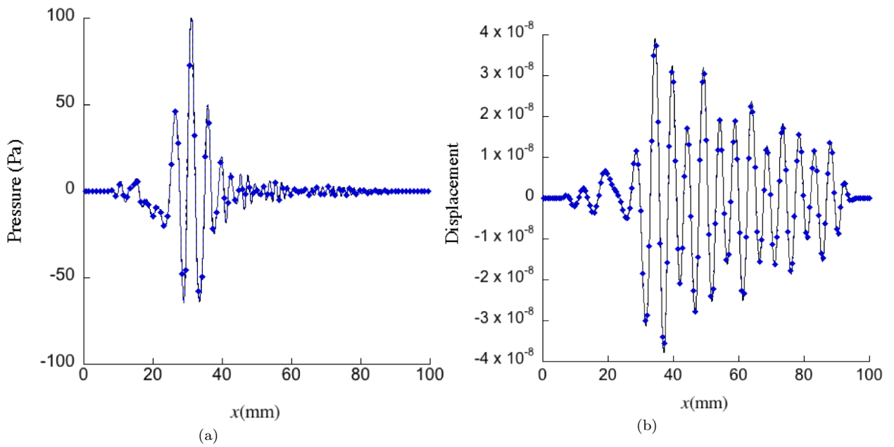
Figure B.10. Comparison of the pressure at front surface (a) and normal displacement at back surface (b) between the FEM model (dashed diamond -\diamond- ) and RIM-FEM-RIM hybrid model (solid line - ).
