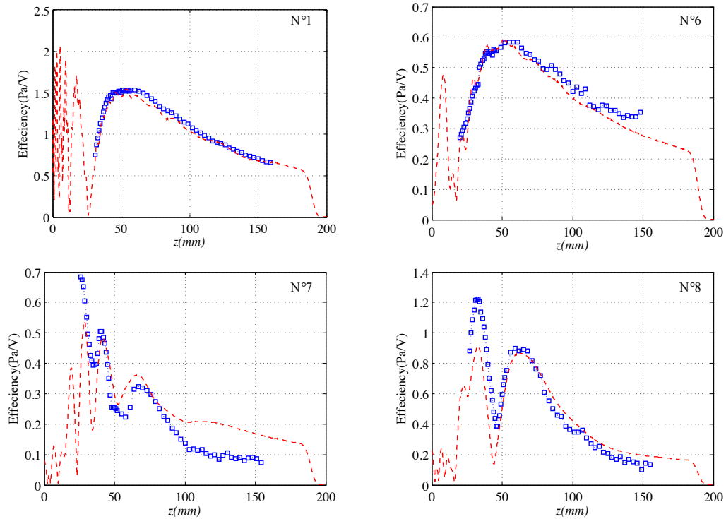
Figure 2.24. Annular MEACUT element acoustic field on-axis pressure measurement: Simulation with finite element method field pressure data (dashed line --- ), on-axis measured pressure amplitude with pulse excitation (non-filling square \square ). Element N°1 (centre circular element), N°6, N°7 and N°8 are demonstrated as the examples.
