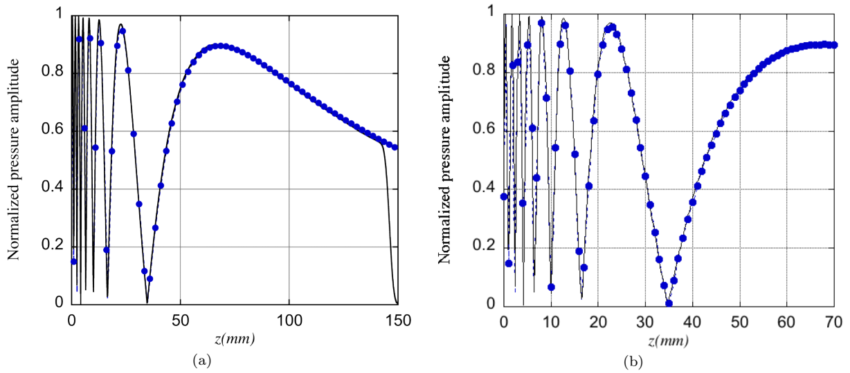
Figure 1.7. Comparison of the on-axis pressure amplitude between axisymmetric FE model (solid line - ) and KIM model (dashed circle - \bullet - ) for circular transducer with radius r = 9\text{mm} at frequency f = 300\text{kHz} . (a): On-axis pressure distribution comparison. (b): The near field comparison between the two models.
