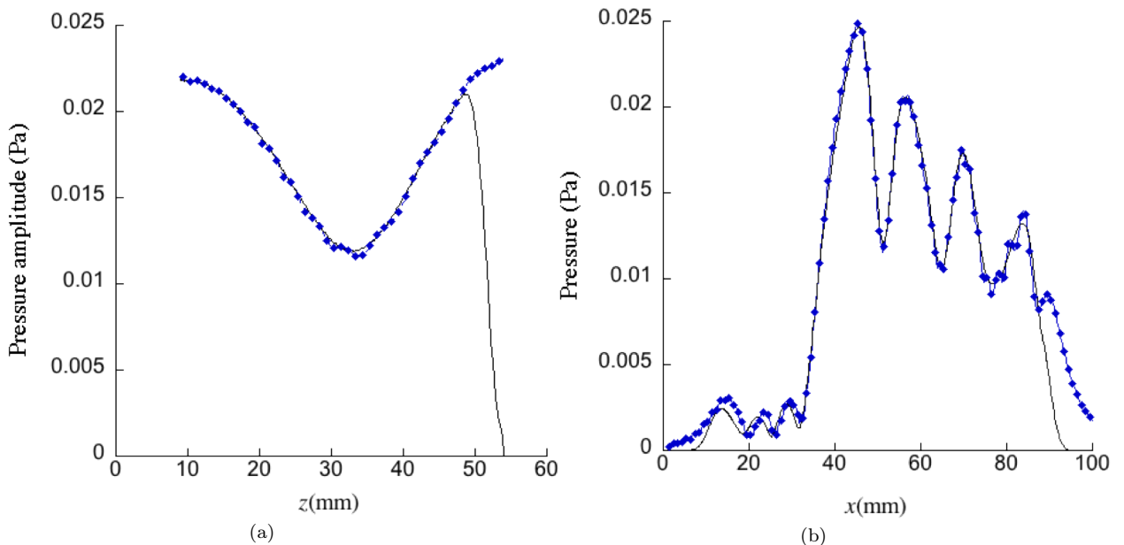
Figure B.11. Comparison of the the pressure amplitude on-axis (a) (along z direction from the centre point of plate) and along direction parallel to the plate at distance z = 35\text{mm} (b) between the FEM model (dashed diamond -\diamond- ) and RIM-FEM-RIM hybrid model (solid line - ).
