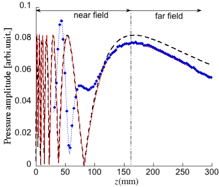
Figure 2.7. On-axis pressure amplitude distribution radiated by a circular transducer versus propagation distance z . Experimental results (dashed diamond -\diamond- ) and Analytical results with (solid line - ) and without (dashed line -- ) attenuation effects.
