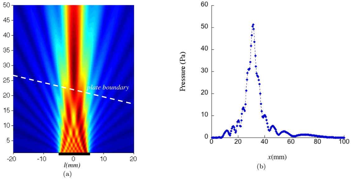
Figure B.6. 2D RIM model for a piston transmitter. (a): Ultrasonic pressure amplitude generated by a line transmitter with length l = 10\text{mm} , the dashed line across the field shows the air-plate interface position. (b): Acoustic pressure amplitude along air-plate interface.
