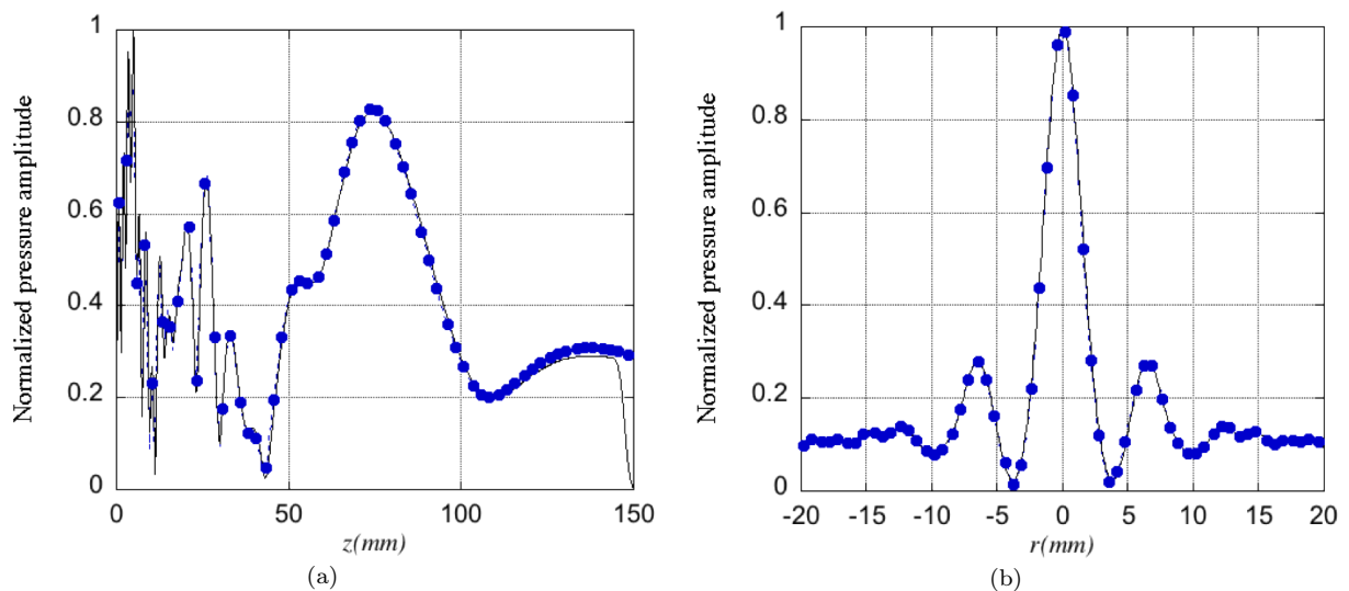
Figure 1.12. Comparison pressure amplitude distribution between axisymmetric FE model (solid line - ) and KIM model (dashed circle - \bullet - ) for 3-element annular array, (a): On-axis acoustic pressure amplitude distribution. (b): Transverse pressure amplitude at distance z = 70\text{mm} .
