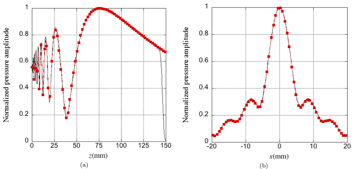
Figure 3.6. Comparison of the pressure amplitude predicted by 3D RIM model (dashed square - \blacksquare - ) and axisymmetric FE model (solid line - ) with non-piston source velocity. the on-axis (a) and transverse at distance z = 100\text{mm} (b).
