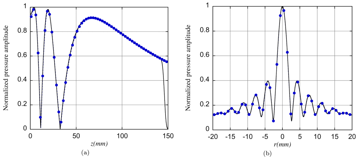
Figure 1.10. Comparison of the on-axis and transverse pressure amplitude between axisymmetric FE model (solid line –) and KIM model (dashed circle – • –) for annular transducer inner radius r_{in} = 12mm and outer radius r_{ou} = 15mm at frequency f = 300kHz . (a): On-axis acoustic pressure amplitude distribution. (b): Transverse pressure amplitude at distance z = 80mm .
