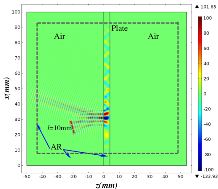
Figure B.3. Air-solid coupling 2D FE model for through-transmission plate inspection: the plate is surrounded by air domains and located between z = 0\text{mm} and z = 4\text{mm} ; the figure shows acoustic pressure in air (real part of complex pressure) and stress in solid.
