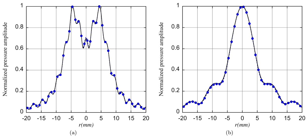
Figure 1.8. Comparison of the transverse pressure amplitude between axisymmetric FE model (solid line - ) and KIM model (dashed circle - \bullet - ) for circular transducer with radius r = 9\text{mm} at frequency f = 300\text{kHz} . (a): Near field transverse pressure amplitude at distance z = 30\text{mm} . (b): Far field transverse pressure amplitude at distance z = 100\text{mm} .
