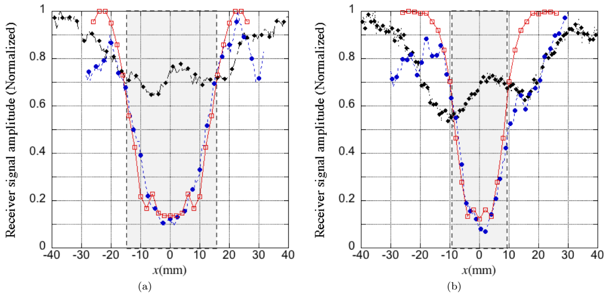
Figure 4.12. Comparison between through-transmission C-scans of the composite plate damaged zone: experimental measurement with a pair of ACUT (dashed diamond -\blacklozenge- ); measurement with MEACUT transmitter/ ACUT receiver (dashed - \bullet - ), simulation with 3D KIM-FEM-RIM hybrid model used for one MEACUT and one ACUT ( -\square ). The C-scan is across the defect along its major axis (a) and minor axis (b). The signal output amplitudes from the receiver are normalized for a clear comparison.
