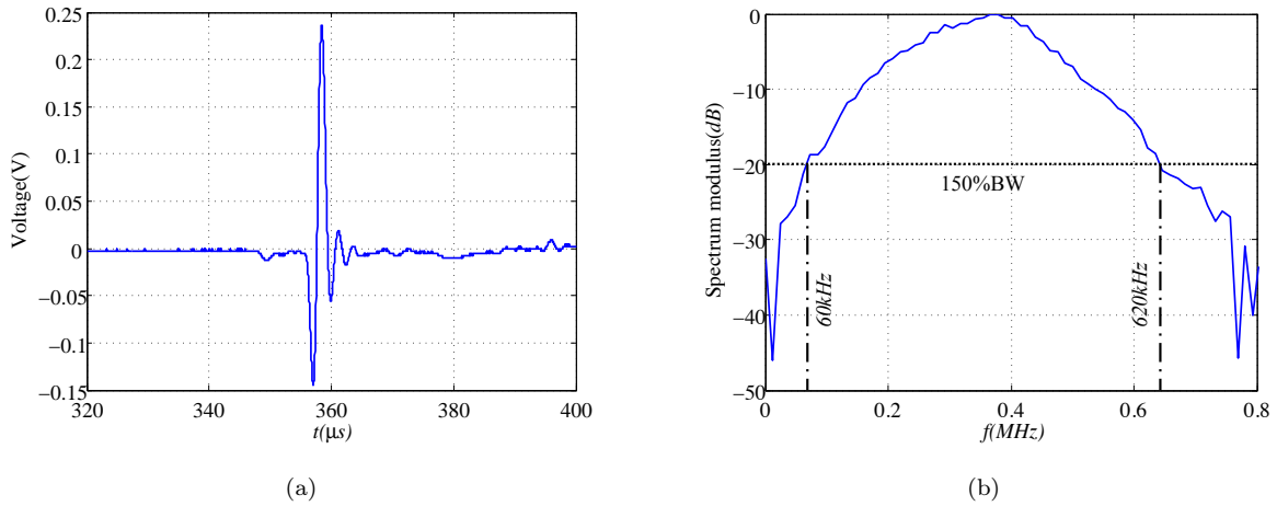
Figure 2.20. Frequency response measurement using pulse excitation for MEACUT. The velocity measurement is at the surface of the membrane with LDV at the focused axis position z = 100mm . (a): Measured temporal output signal of LDV at the testing membrane. (b): MEACUT focused acoustic field frequency response in air.
