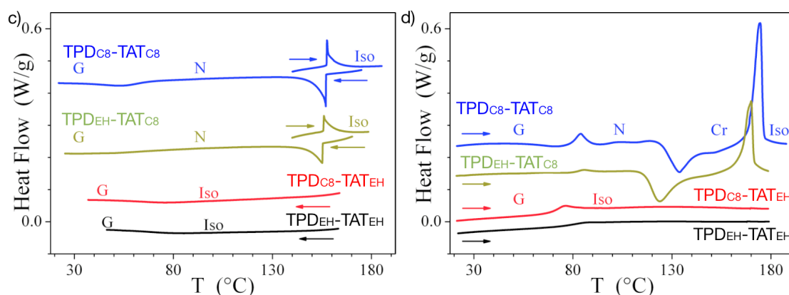
Figure 5-3: POM: typical nematic schlieren textures observed for the liquid-crystalline phase of TPDC 8 -TATC 8 (a) and TPDEH-TATC 8 (b), at 150°C in the fluid state, and at 20°C in the glassy state (half-images left and right, respectively); bottom, DSC: (c) cooling runs from the fluid isotropic liquid state (Iso) and 3 rd heating runs from the fluid nematic phase (N) at 125°C; (d) 2 nd heating runs from glassy nematic or isotropic room temperature states (G); Cr: crystalline phase; ramp conditions: 5°C/min, endotherm up.
