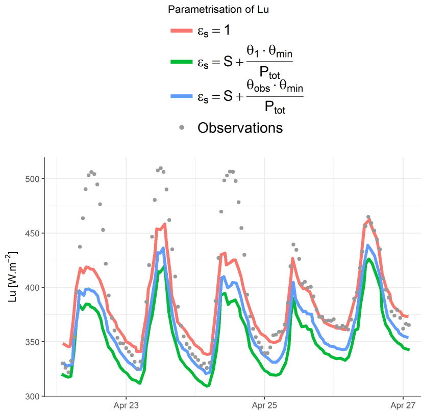
FIGURE 3.8: Comparison of different parametrization of upward long-wave radiation ( Lu ) by modifying the soil emissivity \epsilon_s between 22 and 27 April 2015 in Stein, Switzerland. We set S = 0.9 , \theta_{min} = 0.08 \text{ m}^3 \text{ m}^{-3} , P_{tot} = 0.46 \text{ m}^3 \text{ m}^{-3} , \theta_{sim} simulated volumetric water content at 5 cm with SOPHIA model, \theta_{obs} the volumetric water content observed at 5 cm. The first three days were clear sky days while the last two were rainy.
