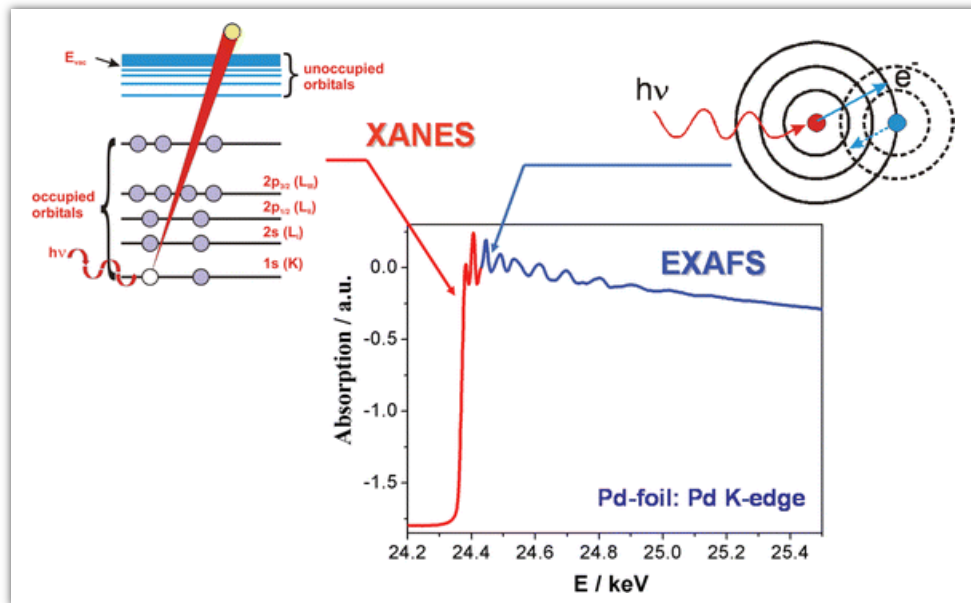
Figure 2.9: Example of XAS spectra around the Pd K-edge and the principle of XANES and EXAFS (Grunwaldt & Baiker, 2005).
