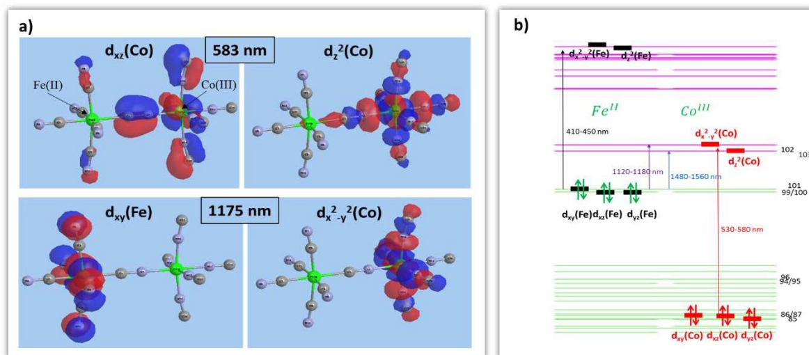
Figure 4.8: a) Characteristic orbitals of hole and particle for \text{Co}^{\text{III}}(\text{LS})\text{Fe}^{\text{II}}(\text{LS}) state obtained by TD-DFT. b) Energy diagram of \text{Co}^{\text{III}}(\text{LS})\text{Fe}^{\text{II}}(\text{LS}) calculated by TDF.
