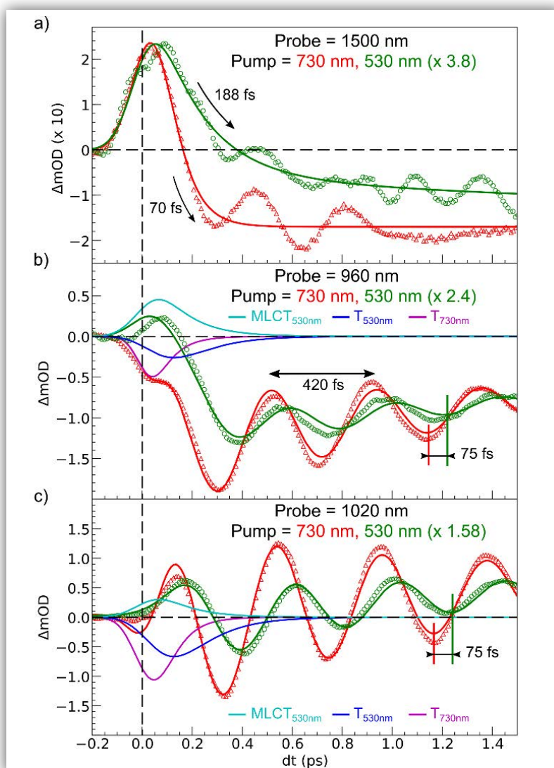
Figure 3.23: Comparison of short time scans of relative OD change at selected probing wavelength upon MLCT LS excitation at 530 nm and d-d LS excitation at 730 nm. The fit for 530 nm excitation includes MLCT and T intermediates, whereas the fit for 730 nm includes T only.
