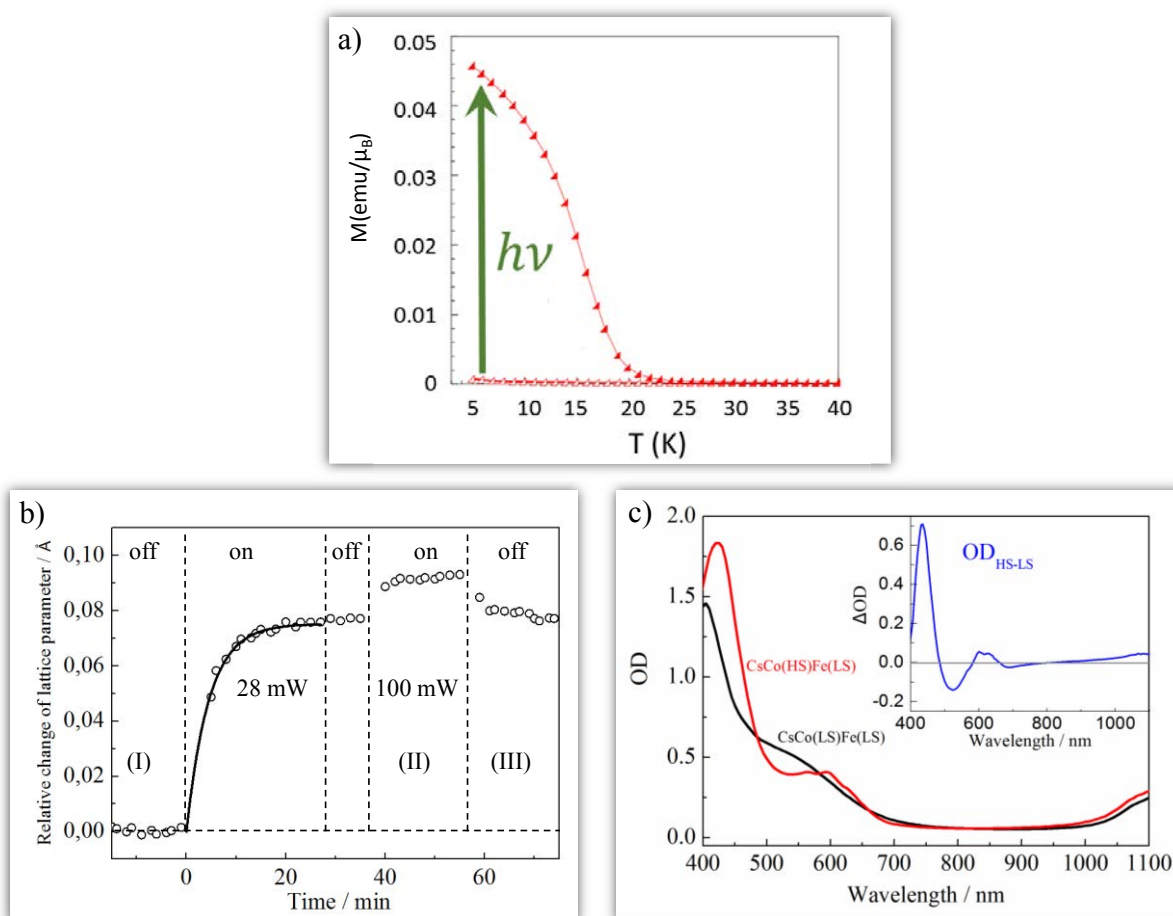
Figure 4.3: a) Temperature dependence of magnetic measurements in \text{CsCoFe}(\text{CN})_6 before and after CW irradiation at 5 K (Dia, 2013). b) Relative change of the lattice parameter \text{CsCoFe}(\text{CN})_6 at 15 K, under 650 nm CW excitation. c) Visible absorption spectra at 15 K, before (black) and after (red) irradiation at 650 nm, in inset (blue) the difference between them (red-black).
